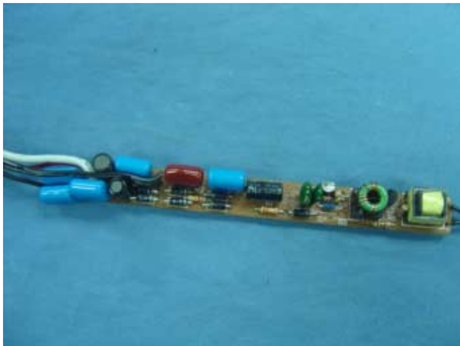
M/N: STRA-T4-6W Figure 20 Main Board, Component Side
