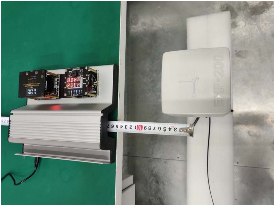
E-Field Position A
