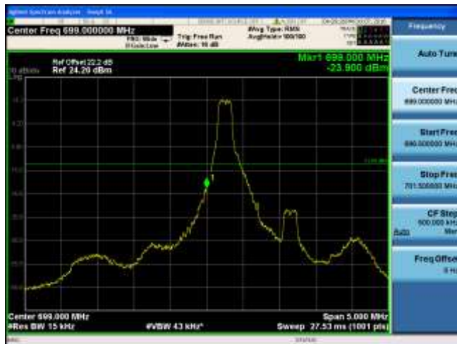
CH23025 (700.5MHz) 16QAM Bandwidth 3MHz 1RB#0
