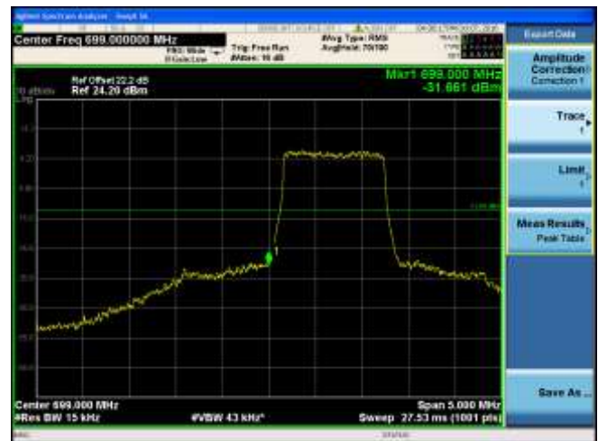
CH23025 (700.5MHz) QPSK Bandwidth 3MHz 15RB#0
