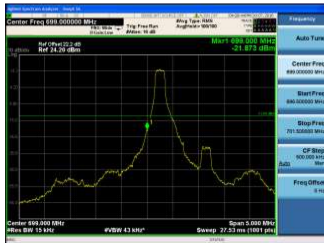
CH23025 (700.5MHz) QPSK Bandwidth 3MHz 1RB#0
