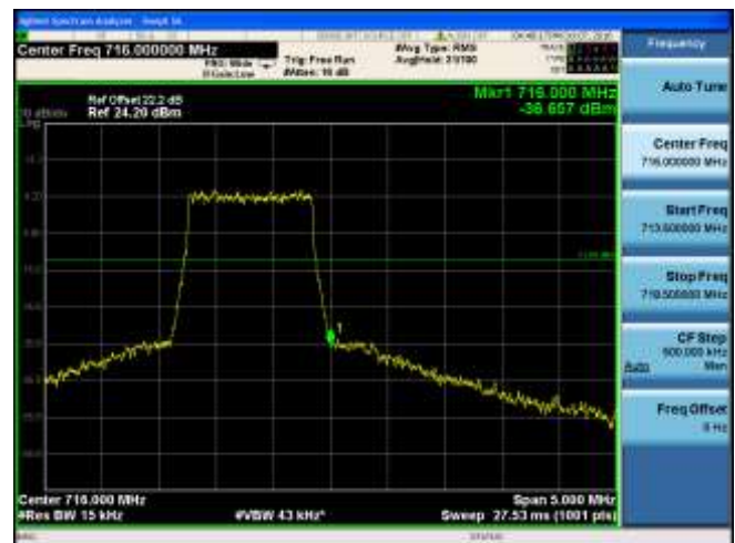
CH23165 (714.5MHz) 16QAM Bandwidth 3MHz 15RB#0
