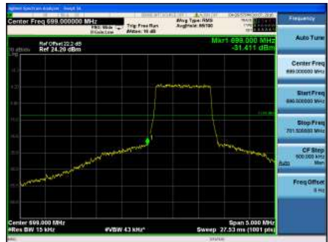
CH23025 (700.5MHz) 16QAM Bandwidth 3MHz 15RB#0
