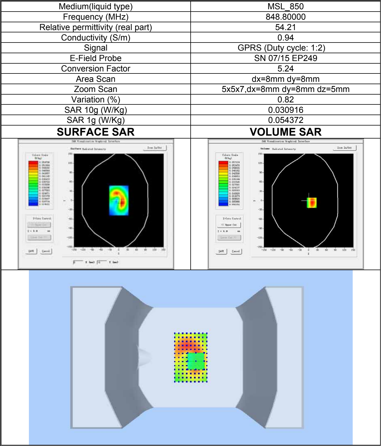
Plot 8: GPRS850MHz, Mid channel(Body-worn, Bottom edge) Product Description: MOBILE PHONE Test Date: 2018-06-14
