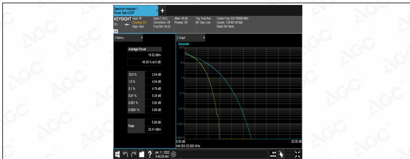
Band5-1.4MHz-QPSK-20525-1RB#0
