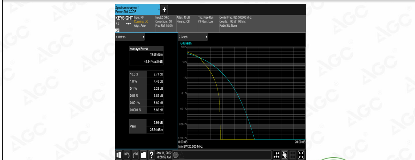
Band5-3MHz-16QAM-20415-1RB#0
