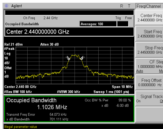
DTS Bandwidth (6dB BW)
