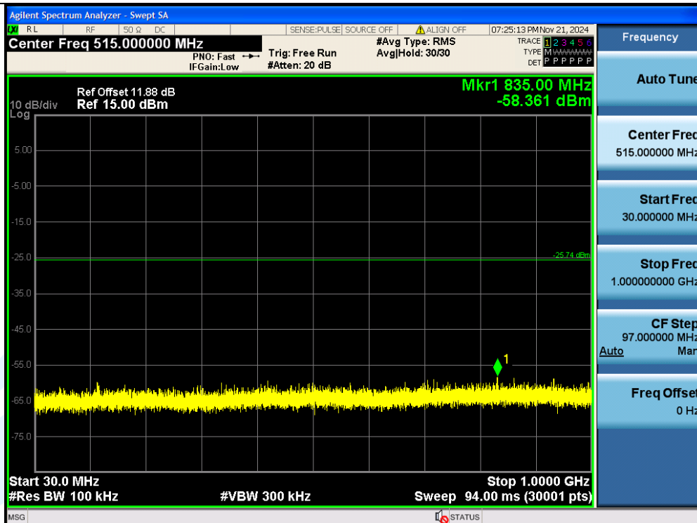
3DH5-Ant1-2441-30~1000-PASS
