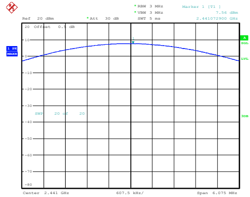
GFSK_Middle 7.56dBm
