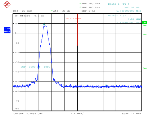
GFSK_High 60.51dB
