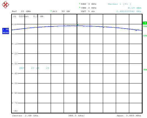
GFSK_High 8.19dBm
