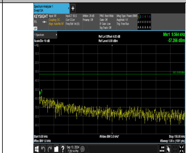
Band26_5MHz_16QAM_27015_1RB#0_0.009~0.15_0.009~0.15
