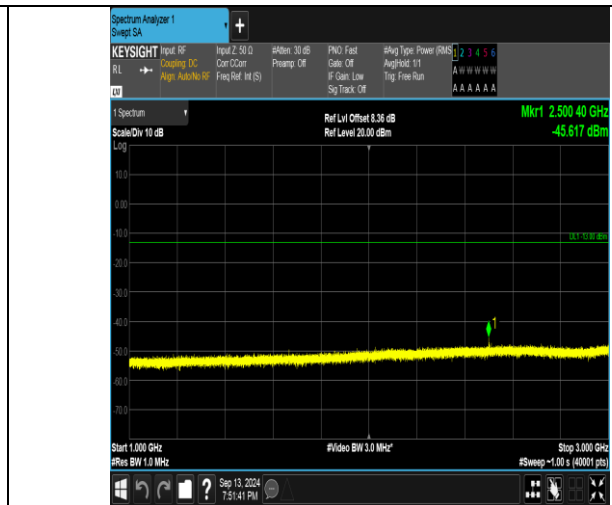
Band26_10MHz_QPSK_26840_1RB#49_1000~3000_1000~3000
