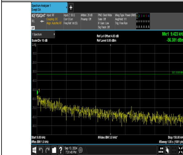
Band26_5MHz_QPSK_27015_25RB#0_0.009~0.15_0.009~0.15
