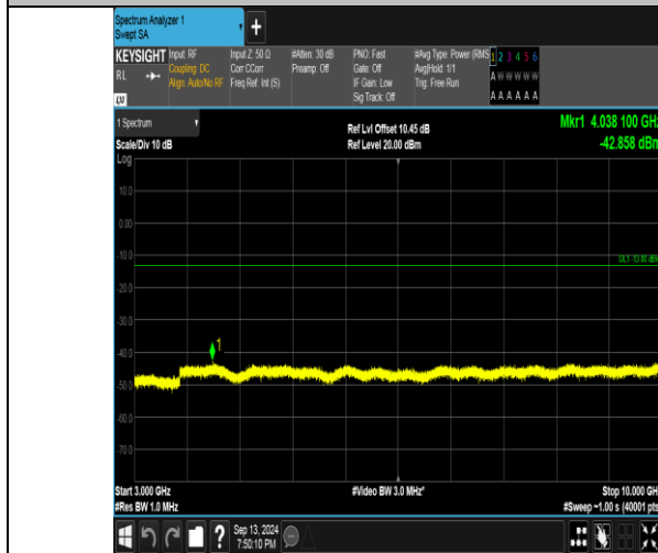
Band26_10MHz_QPSK_26840_1RB#0_3000~10000_3000~10000
