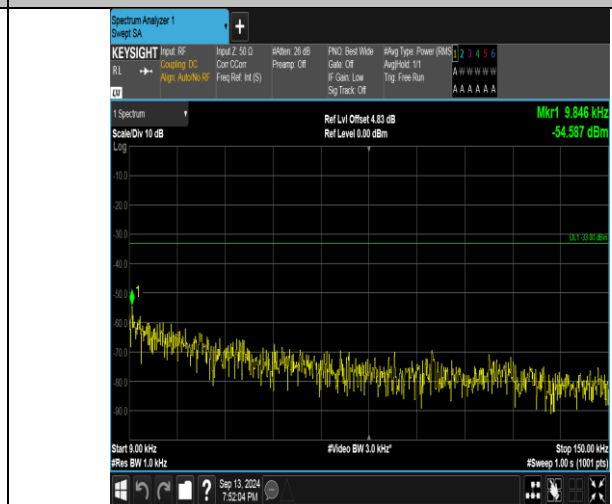
Band26_10MHz_16QAM_26840_1RB#49_0.009~0.15_0.009~0.15
