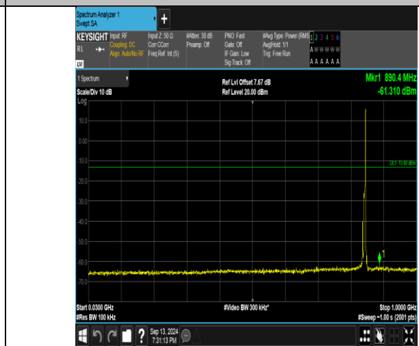
Band26_5MHz_16QAM_27015_1RB#24_30~1000_30~1000
