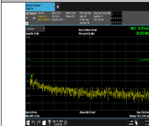
Band26_5MHz_QPSK_26915_1RB#24_0.009~0.15_0.009~0.15
