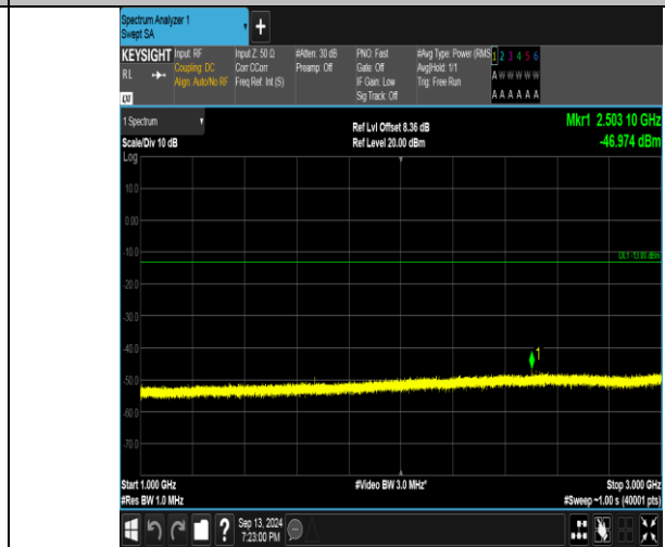
Band26_5MHz_QPSK_26915_1RB#0_1000~3000_1000~3000
