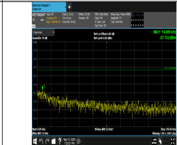
Band26_5MHz_16QAM_26915_1RB#0_0.009~0.15_0.009~0.15
