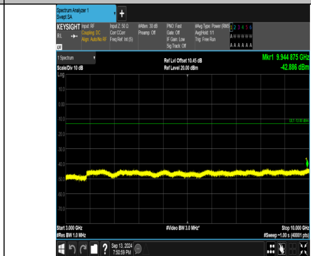
Band26_10MHz_16QAM_26840_1RB#0_3000~10000_3000~10000
