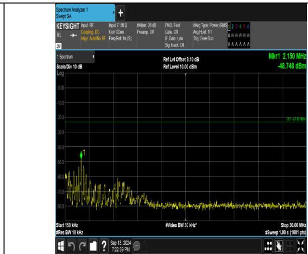
Band26_5MHz_QPSK_26915_1RB#0_0.15~30_0.15~30
