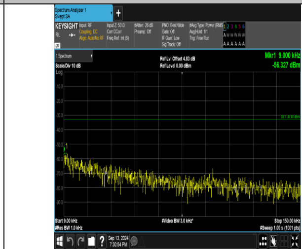
Band26_5MHz_16QAM_27015_1RB#24_0.009~0.15_0.009~0.15
