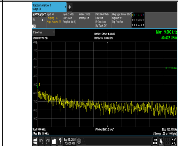
Band26_5MHz_16QAM_26915_1RB#24_0.009~0.15_0.009~0.15
