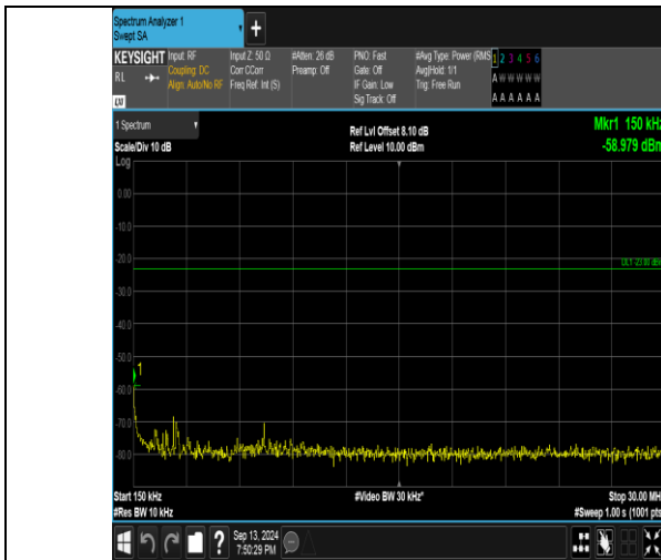
Band26_10MHz_16QAM_26840_1RB#0_0.15~30_0.15~30
