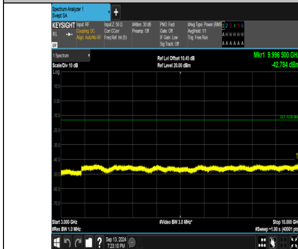
Band26_5MHz_QPSK_26915_1RB#0_3000~10000_3000~10000
