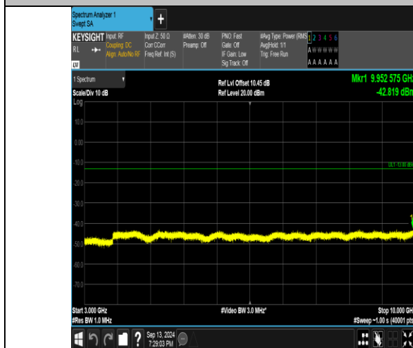
Band26_5MHz_QPSK_27015_1RB#0_3000~10000_3000~10000
