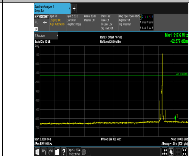
Band26_10MHz_16QAM_26840_1RB#49_30~1000_30~1000
