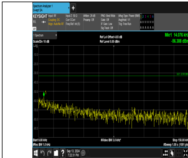
Band26_5MHz_QPSK_26915_1RB#0_0.009~0.15_0.009~0.15
