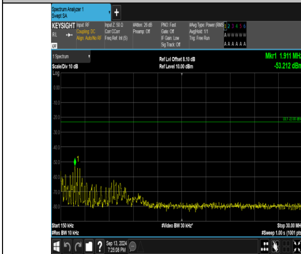
Band26_5MHz_16QAM_26915_1RB#24_0.15~0.30_0.15~0.30
