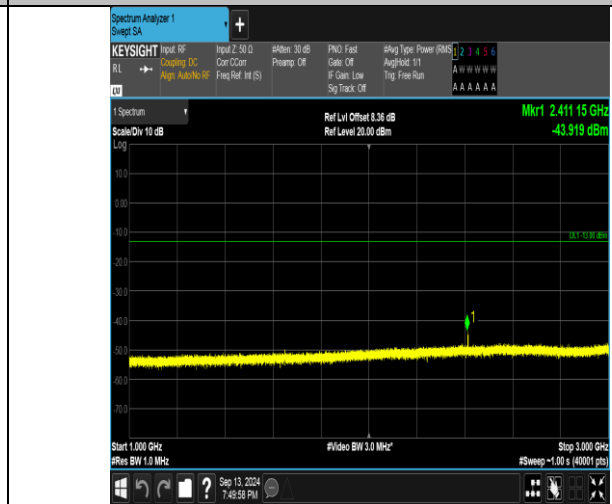
Band26_10MHz_QPSK_26840_1RB#0_1000~3000_1000~3000
