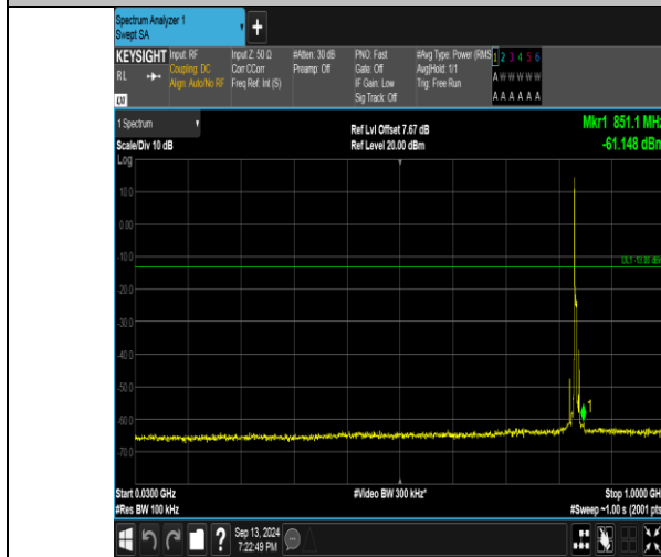
Band26_5MHz_QPSK_26915_1RB#0_30~1000_30~1000
