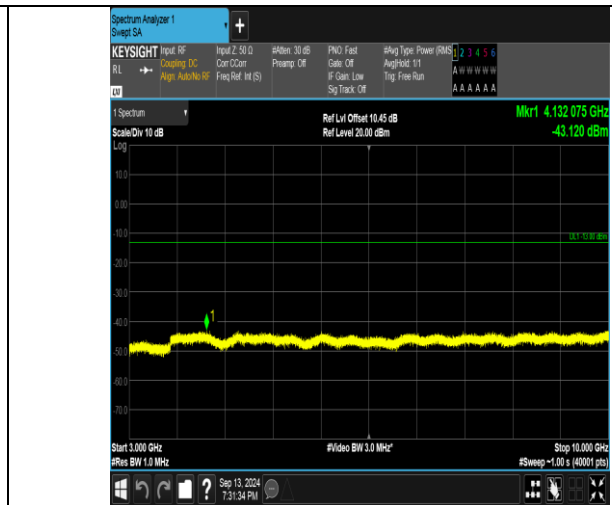
Band26_5MHz_16QAM_27015_1RB#24_3000~10000_3000~10000
