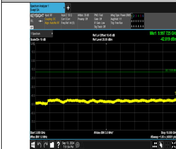
Band26_10MHz_QPSK_26840_1RB#49_3000~10000_3000~10000
