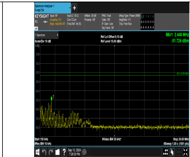
Band26_5MHz_QPSK_27015_1RB#0_0.15~30_0.15~30
