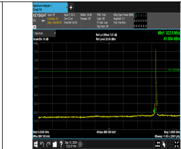
Band26_5MHz_16QAM_26915_1RB#0_30~1000_30~1000
