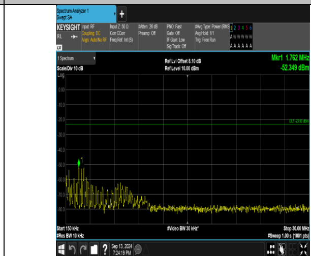
Band26_5MHz_QPSK_26915_1RB#24_0.15~30_0.15~30
