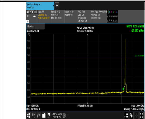
Band26_5MHz_16QAM_26915_1RB#24_30~1000_30~1000
