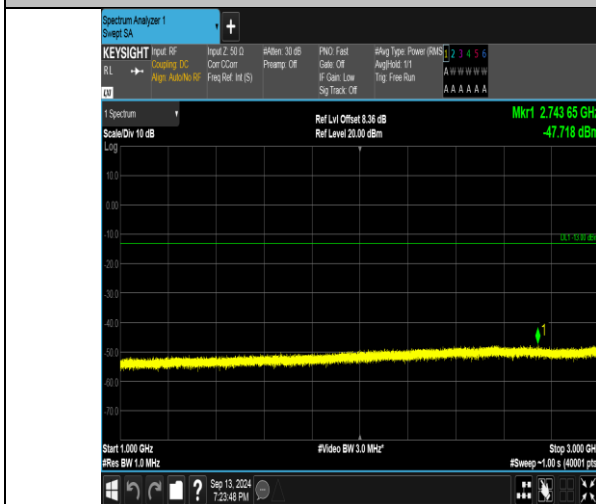
Band26_5MHz_16QAM_26915_1RB#0_1000~3000_1000~3000
