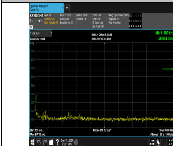
Band26_10MHz_16QAM_26840_1RB#49_0.15~30_0.15~30
