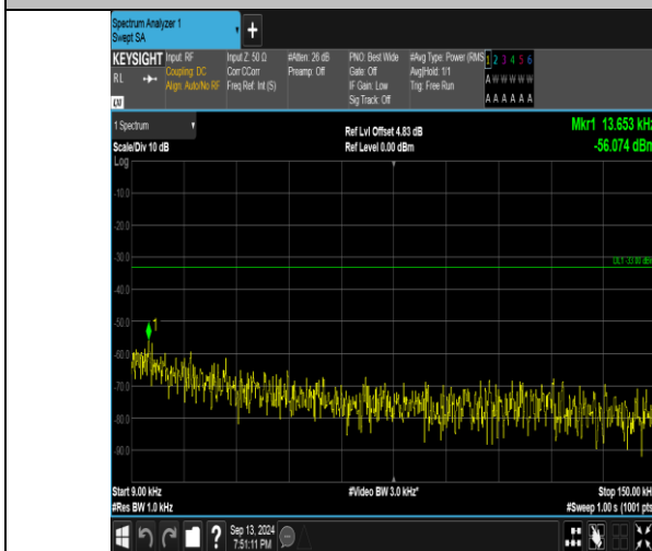
Band26_10MHz_QPSK_26840_1RB#49_0.009~0.15_0.009~0.15
