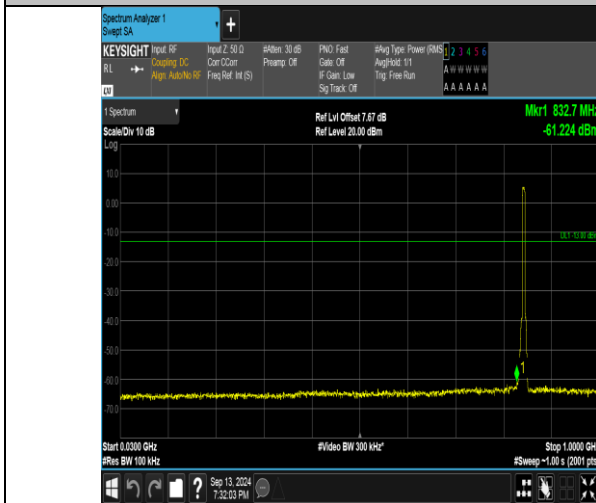
Band26_5MHz_QPSK_27015_25RB#0_30~1000_30~1000
