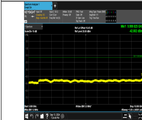
Band26_5MHz_QPSK_26915_1RB#24_3000~10000_3000~10000
