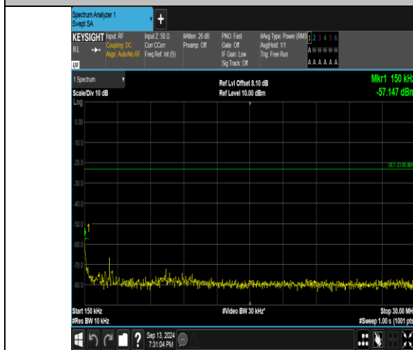
Band26_5MHz_16QAM_27015_1RB#24_0.15~30_0.15~30
