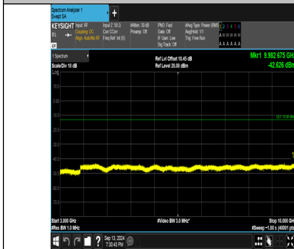
Band26_5MHz_QPSK_27015_1RB#24_3000~10000_3000~10000
