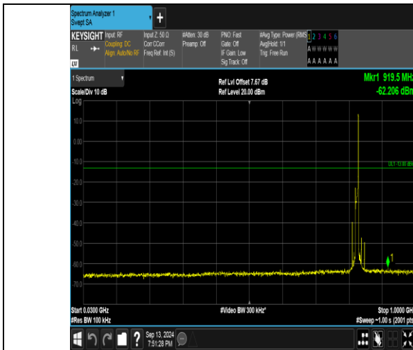
Band26_10MHz_QPSK_26840_1RB#49_30~1000_30~1000
