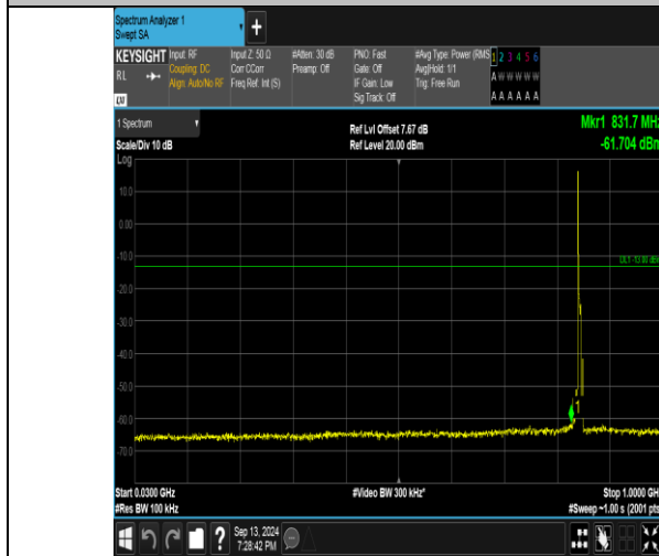
Band26_5MHz_QPSK_27015_1RB#0_30~1000_30~1000
