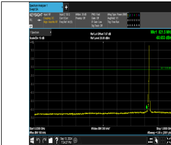
Band26_5MHz_QPSK_26915_1RB#24_30~1000_30~1000
