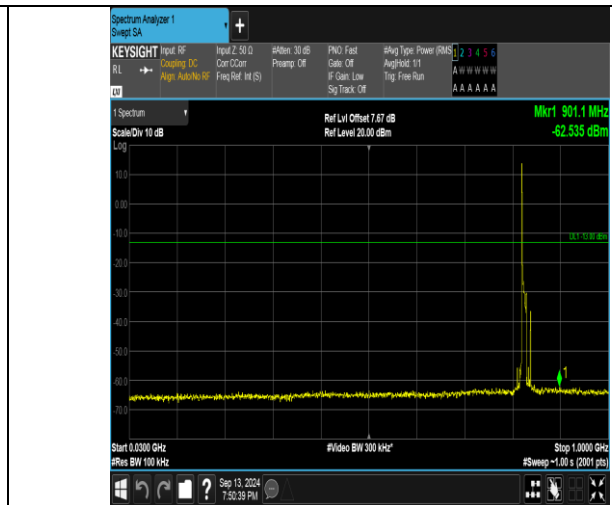
Band26_10MHz_16QAM_26840_1RB#0_30~1000_30~1000
