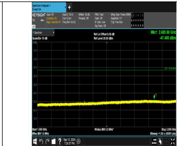
Band26_5MHz_QPSK_26915_1RB#24_1000~3000_1000~3000
