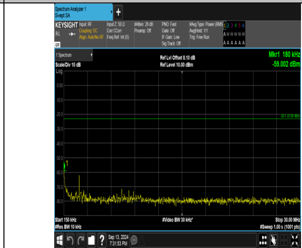
Band26_5MHz_QPSK_27015_25RB#0_0.15~30_0.15~30
