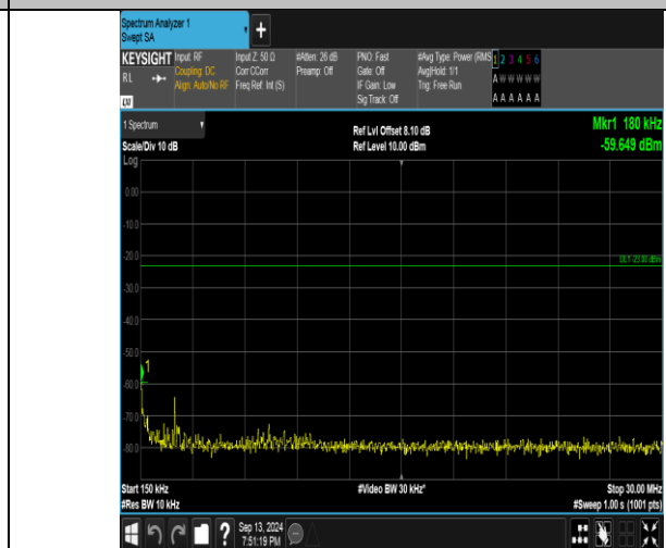
Band26_10MHz_QPSK_26840_1RB#49_0.15~30_0.15~30
