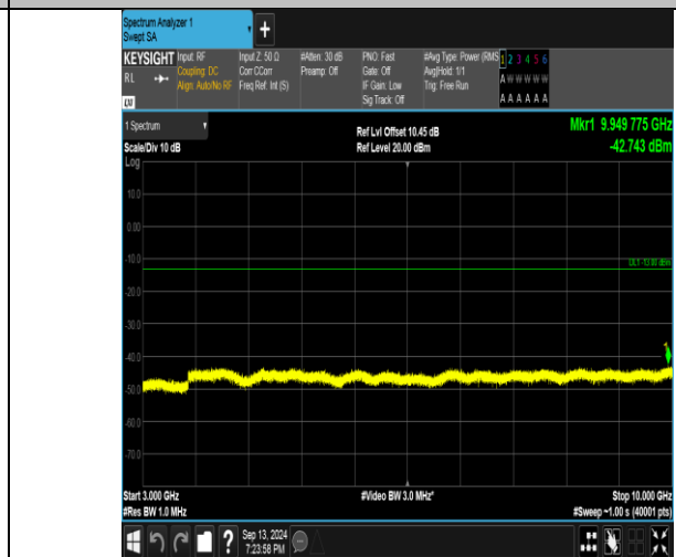
Band26_5MHz_16QAM_26915_1RB#0_3000~10000_3000~10000
