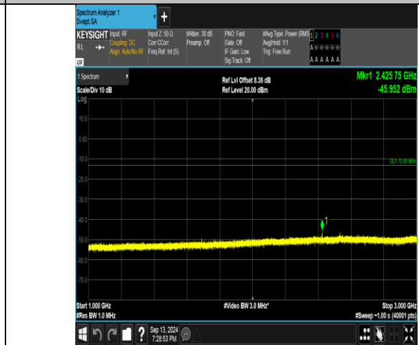
Band26_5MHz_QPSK_27015_1RB#0_1000~3000_1000~3000
