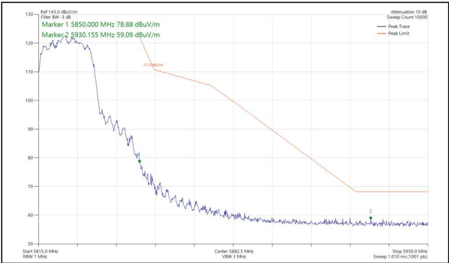
Figure 401 - 802.11n HT20, CDD, Core 0 + Core 1 - 5825 MHz Band Edge Frequency 5850 MHz
