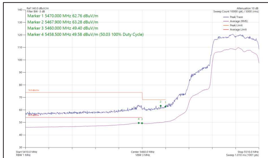
Figure 409 - 802.11ax HE20, SU, SDM, Core 0 + Core 1 - 5500 MHz Band Edge Frequency 5470 MHz
