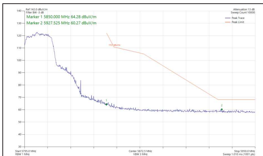
Figure 437 - 802.11ac VHT20, TxBF, Core 0 + Core 1 - 5805 MHz Band Edge Frequency 5850 MHz
