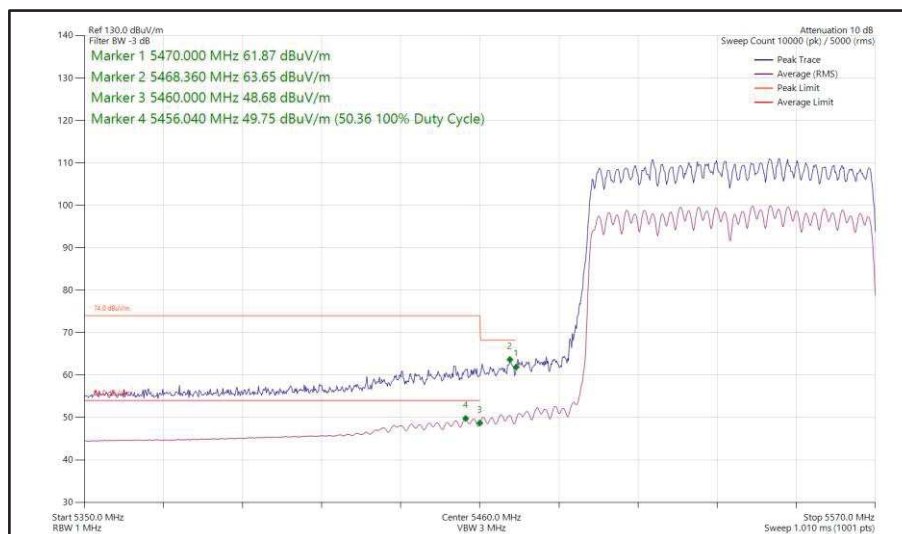
Figure 553 - 802.11ax HE80, SU, CDD, Core 0 + Core 1 - 5530 MHz Band Edge Frequency 5470 MHz
