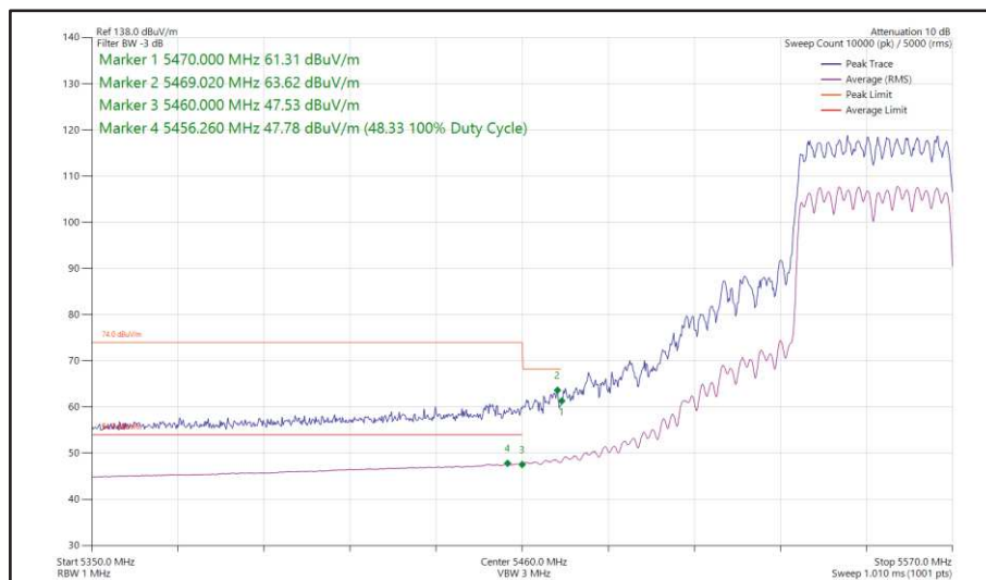
Figure 481 - 802.11ax HE40, SU, CDD, Core 0 + Core 1 - 5550 MHz Band Edge Frequency 5470 MHz
