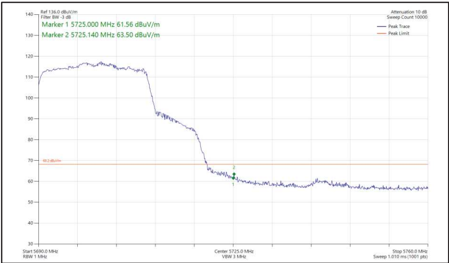
Figure 420 - 802.11ax HE20, SU, SDM, Core 0 + Core 1 - 5700 MHz Band Edge Frequency 5725 MHz
