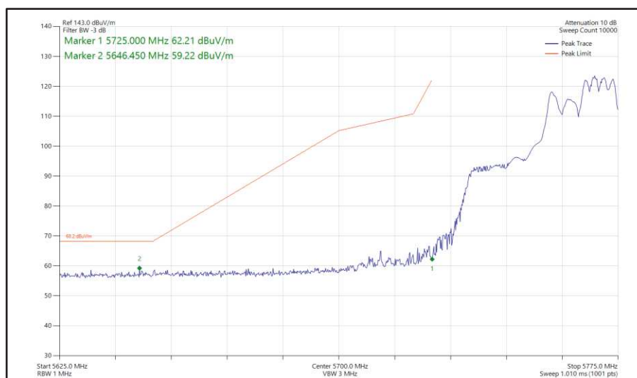
Figure 484 - 802.11ax HE40, RU 106-56, CDD, Core 0 + Core 1 - 5755 MHz Band Edge Frequency 5725 MHz
