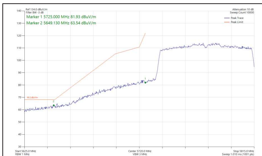
Figure 525 - 802.11ac VHT80, SISO, Core 0 - 5775 MHz Band Edge Frequency 5725 MHz
