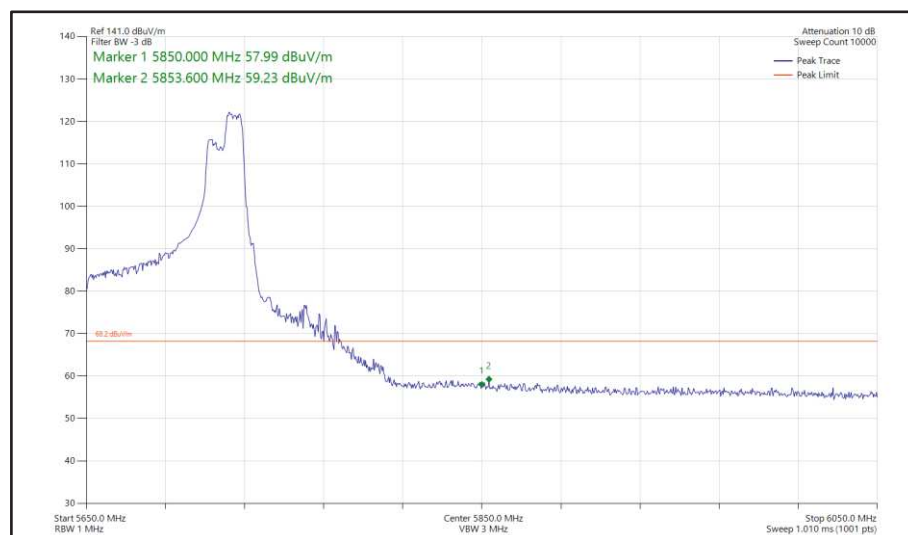
Figure 549 - 802.11ax HE80, RU 106-60, SISO, Core 1 - 5690 MHz Band Edge Frequency 5850 MHz
