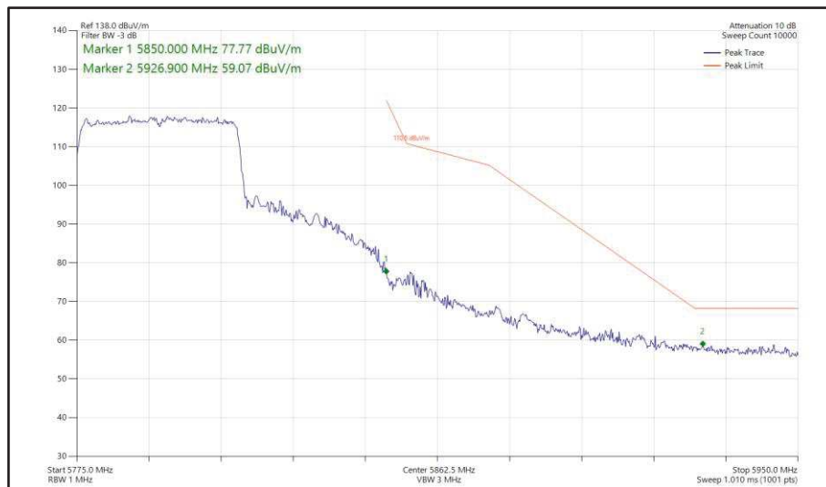
Figure 475 - 802.11ax HE40, SU, SISO, Core 1 - 5795 MHz Band Edge Frequency 5850 MHz
