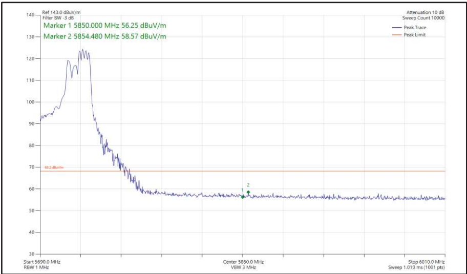
Figure 493 - 802.11ax HE40, RU 106-56, CDD, Core 0 + Core 1 - 5710 MHz Band Edge Frequency 5850 MHz
