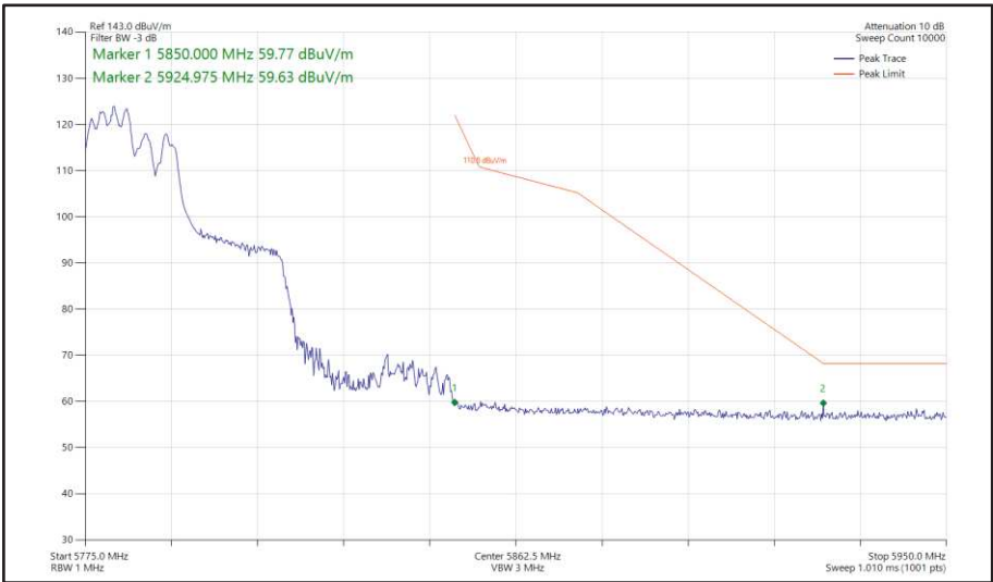
Figure 495 - 802.11ax HE40, RU 106-53, CDD, Core 0 + Core 1 - 5795 MHz Band Edge Frequency 5850 MHz
