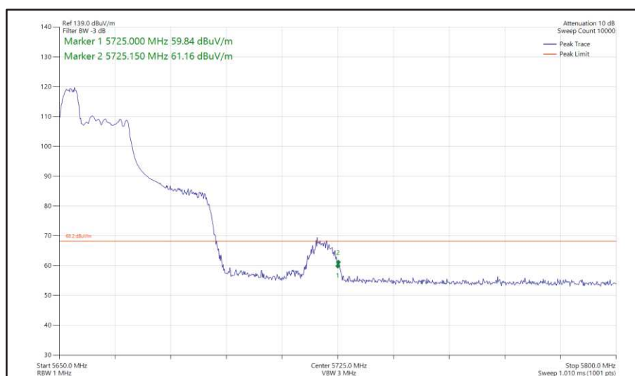
Figure 451 - 802.11ax HE40, RU 52-37, SISO, Core 0 - 5670 MHz Band Edge Frequency 5725 MHz
