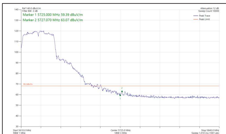
Figure 504 - 802.11n HT40, SDM, Core 0 + Core 1 - 5630 MHz Band Edge Frequency 5725 MHz
