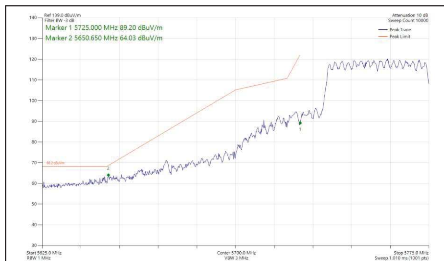
Figure 483 - 802.11ax HE40, SU, CDD, Core 0 + Core 1 - 5755 MHz Band Edge Frequency 5725 MHz
