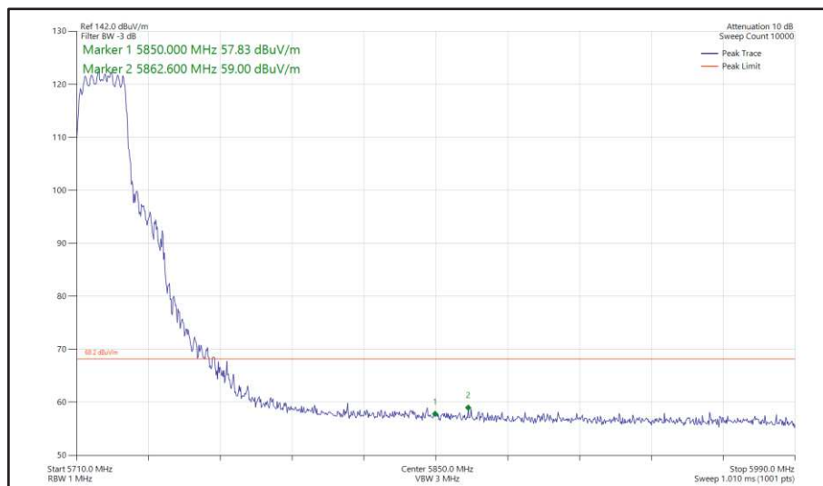
Figure 399 - 802.11n HT20, CDD, Core 0 + Core 1 - 5720 MHz Band Edge Frequency 5850 MHz
