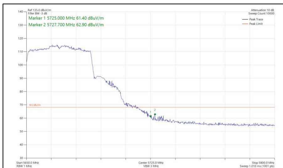
Figure 450 - 802.11ax HE40, SU, SISO, Core 0 - 5670 MHz Band Edge Frequency 5725 MHz
