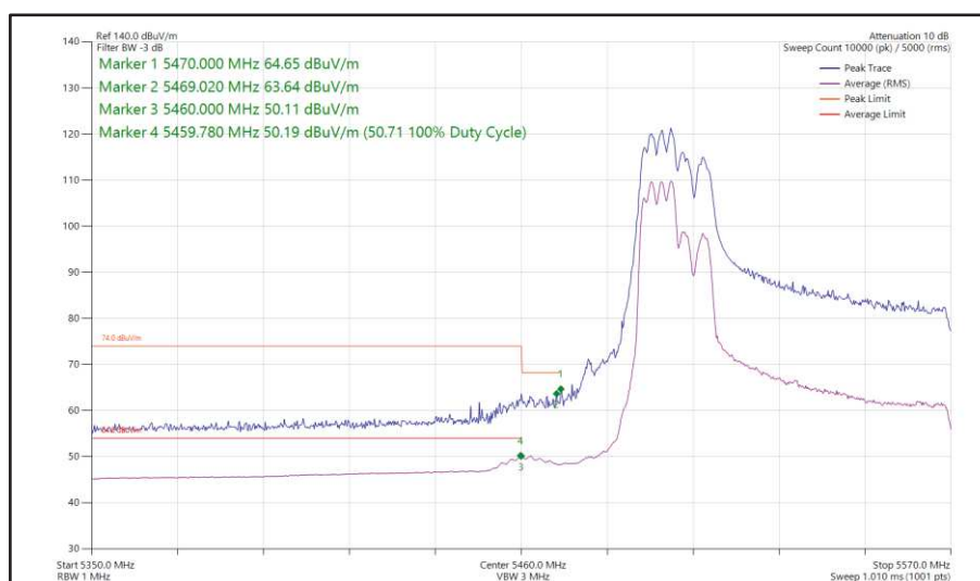
Figure 554 - 802.11ax HE80, RU 106-53, CDD, Core 0 + Core 1 - 5530 MHz Band Edge Frequency 5470 MHz
