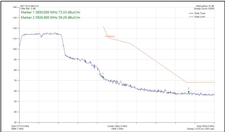
Figure 453 - 802.11n HT40, SISO, Core 0 - 5795 MHz Band Edge Frequency 5850 MHz
