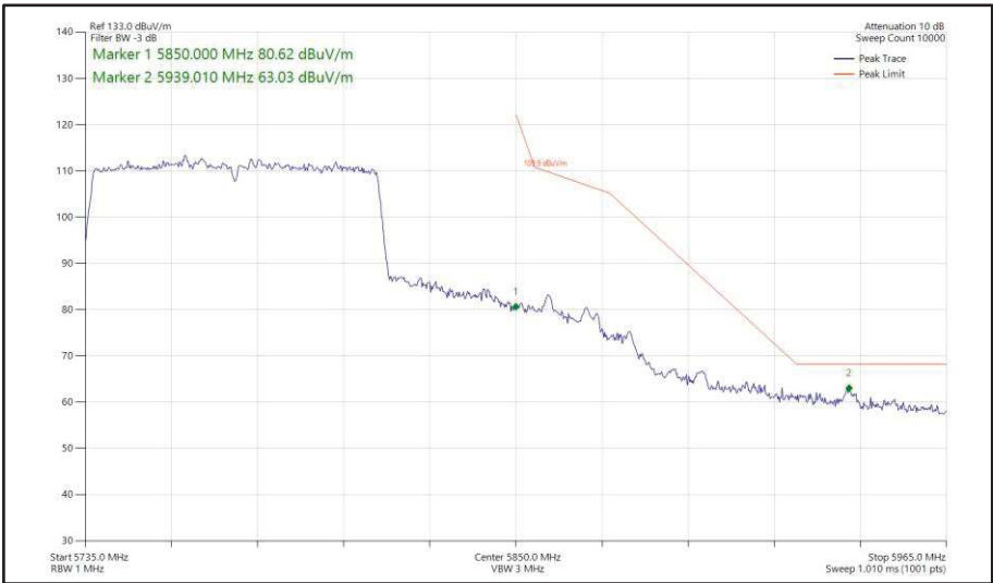
Figure 547 - 802.11ac VHT80, SISO, Core 1 - 5775 MHz Band Edge Frequency 5850 MHz
