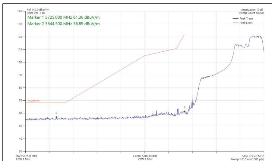
Figure 446 - 802.11ax HE40, RU 106-56, SISO, Core 0 - 5755 MHz Band Edge Frequency 5725 MHz
