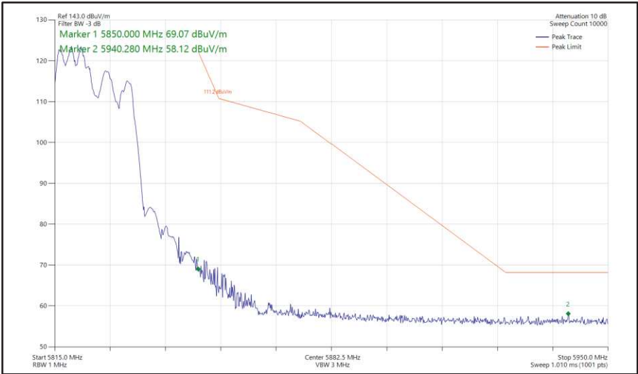
Figure 406 - 802.11ax HE20, RU 106-53, CDD, Core 0 + Core 1 - 5825 MHz Band Edge Frequency 5850 MHz
