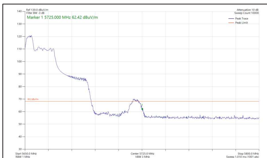
Figure 470 - 802.11ax HE40, RU 52-37, SISO, Core 1 - 5670 MHz Band Edge Frequency 5725 MHz
