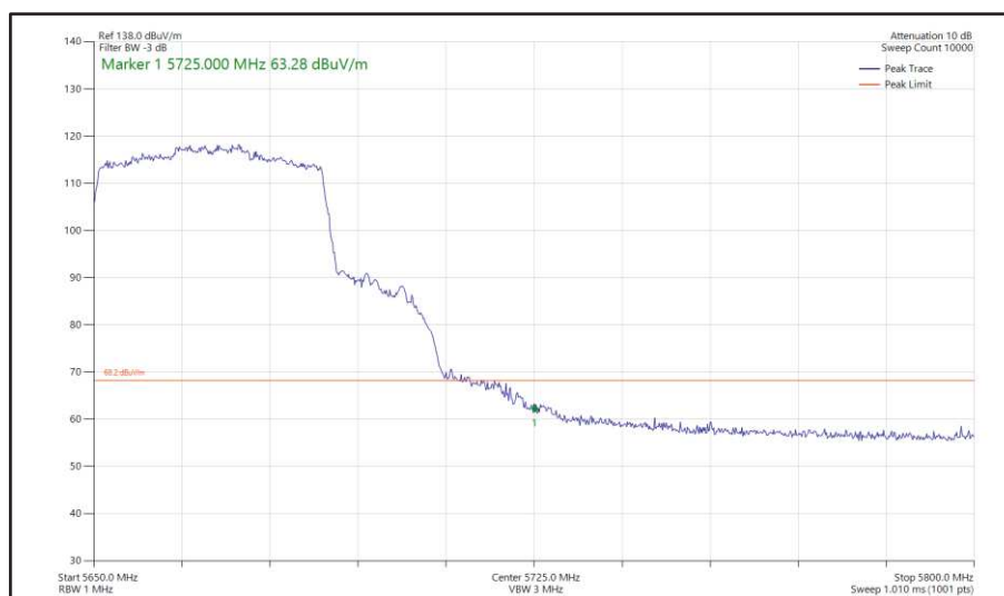
Figure 507 - 802.11ax HE40, SU, SDM, Core 0 + Core 1 - 5670 MHz Band Edge Frequency 5725 MHz
