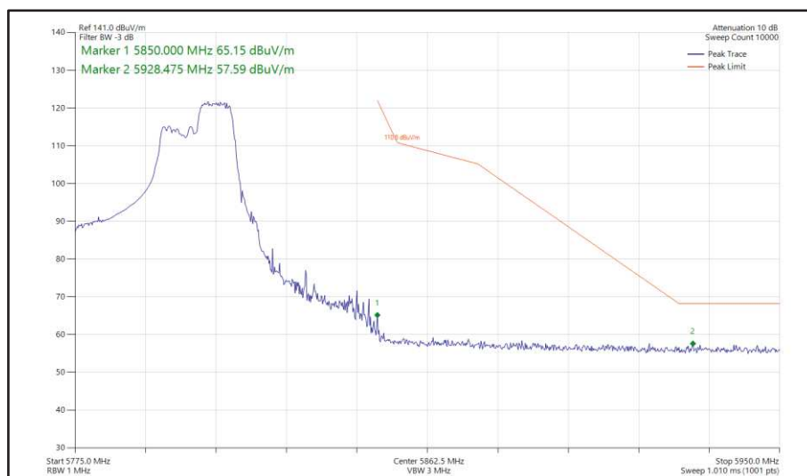
Figure 476 - 802.11ax HE40, RU 106-56, SISO, Core 1 - 5795 MHz Band Edge Frequency 5850 MHz
