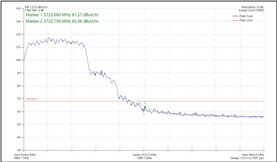
Figure 486 - 802.11n HT40, CDD, Core 0 + Core 1 - 5670 MHz Band Edge Frequency 5725 MHz
