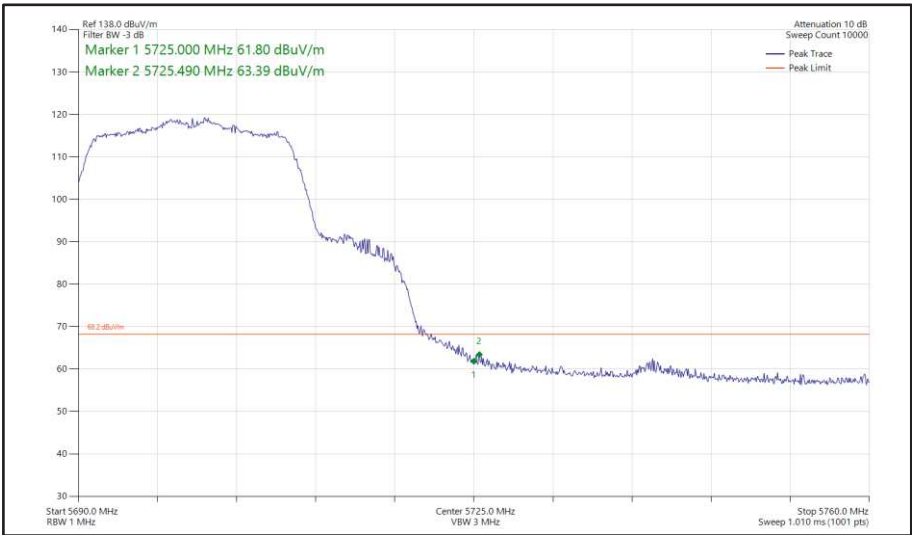
Figure 418 - 802.11n HT20, SDM, Core 0 + Core 1 - 5700 MHz Band Edge Frequency 5725 MHz
