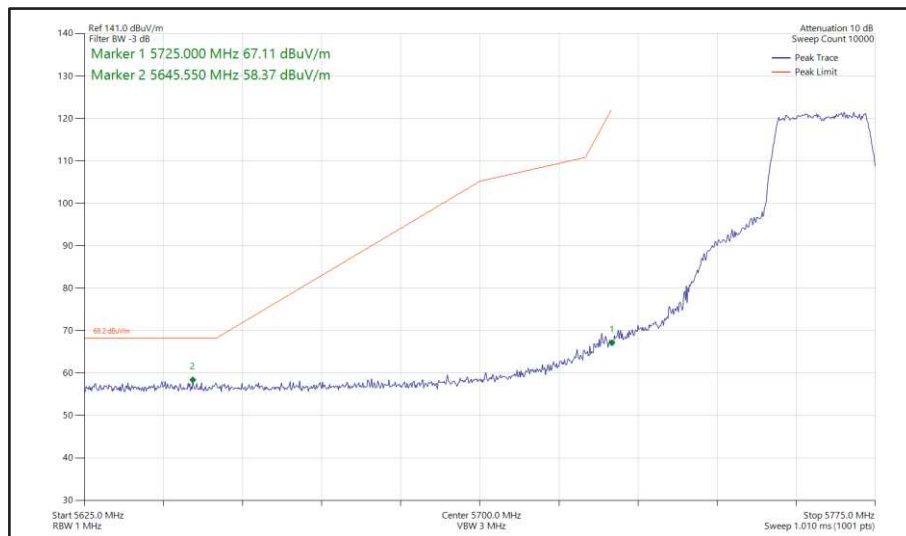
Figure 413 - 802.11n HT20, SDM, Core 0 + Core 1 - 5765 MHz Band Edge Frequency 5725 MHz
