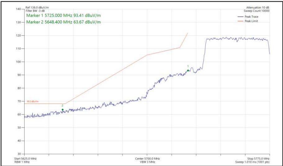
Figure 502 - 802.11ax HE40, SU, SDM, Core 0 + Core 1 - 5755 MHz Band Edge Frequency 5725 MHz
