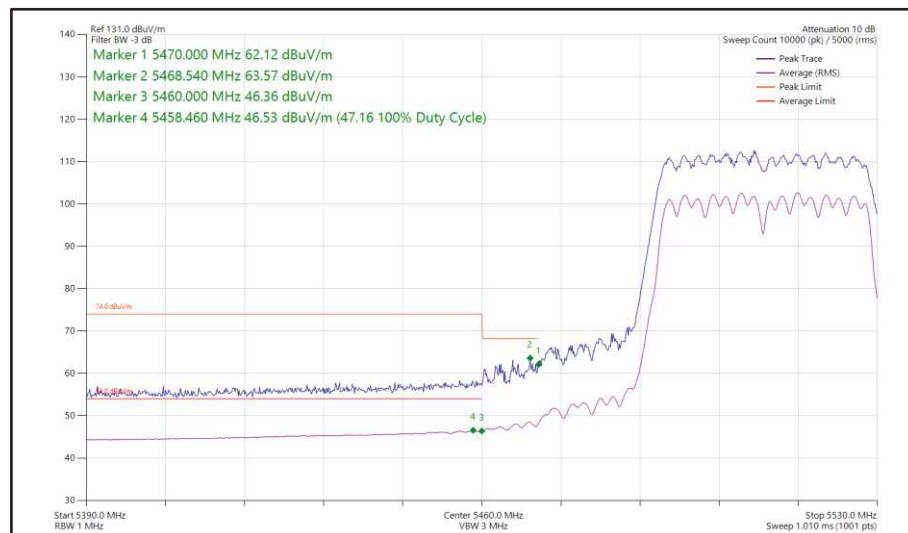
Figure 477 - 802.11n HT40, CDD, Core 0 + Core 1 - 5510 MHz Band Edge Frequency 5470 MHz
