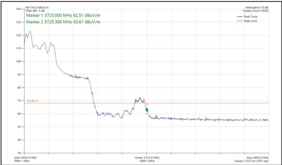
Figure 489 - 802.11ax HE40, RU 52-37, CDD, Core 0 + Core 1 - 5670 MHz Band Edge Frequency 5725 MHz
