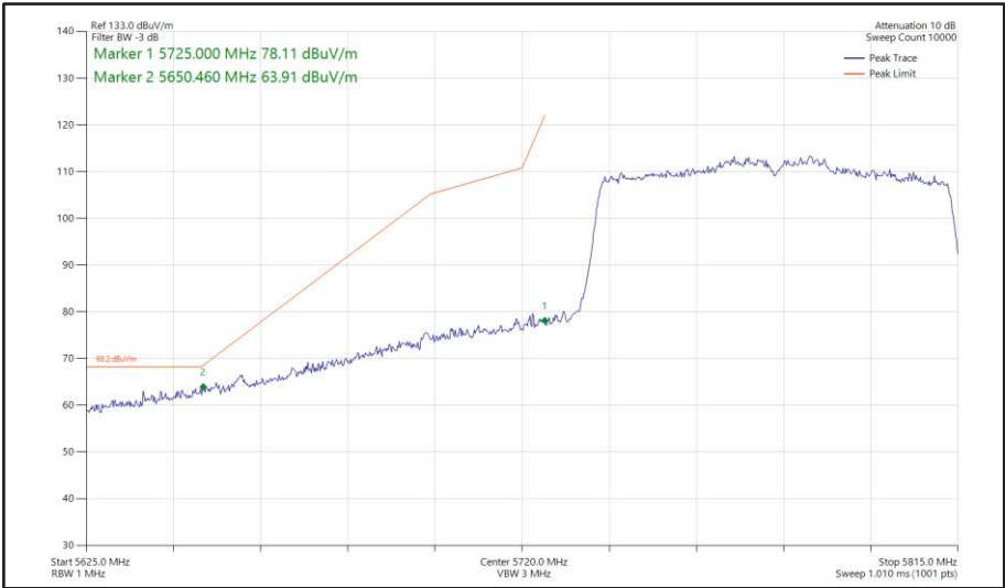
Figure 540 - 802.11ac VHT80, SISO, Core 1 - 5775 MHz Band Edge Frequency 5725 MHz
