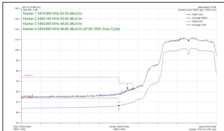
Figure 439 - 802.11n HT40, SISO, Core 0 - 5510 MHz Band Edge Frequency 5470 MHz
