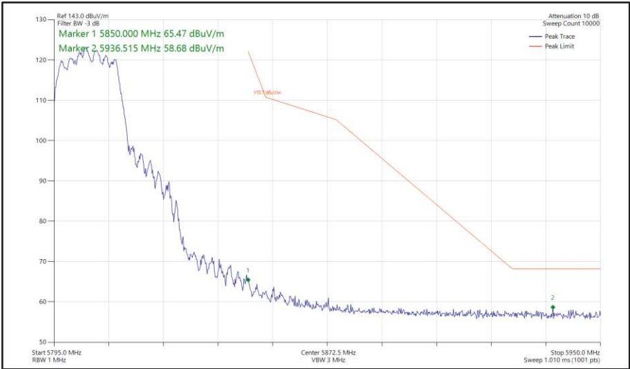
Figure 400 - 802.11n HT20, CDD, Core 0 + Core 1 - 5805 MHz Band Edge Frequency 5850 MHz
