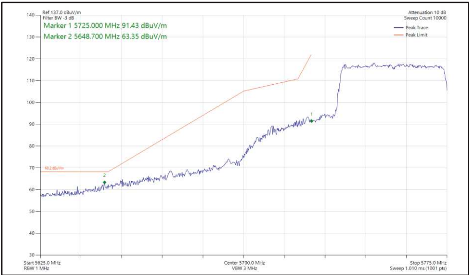
Figure 464 - 802.11ax HE40, SU, SISO, Core 1 - 5755 MHz Band Edge Frequency 5725 MHz
