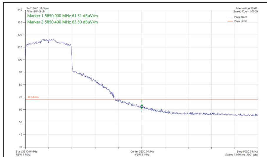
Figure 548 - 802.11ax HE80, SU, SISO, Core 1 - 5690 MHz Band Edge Frequency 5850 MHz
