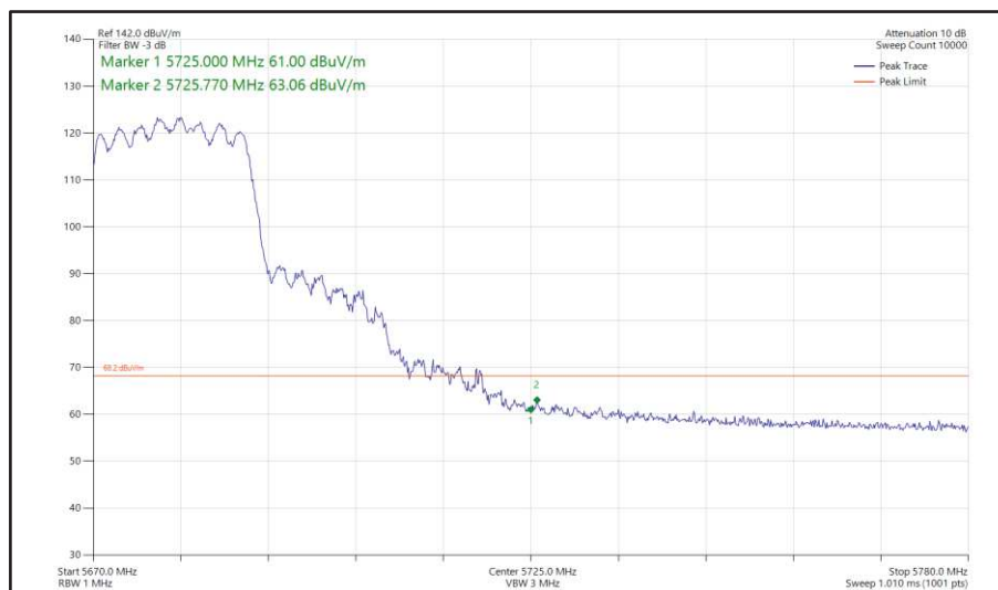
Figure 396 - 802.11ax HE20, SU, CDD, Core 0 + Core 1 - 5680 MHz Band Edge Frequency 5725 MHz
