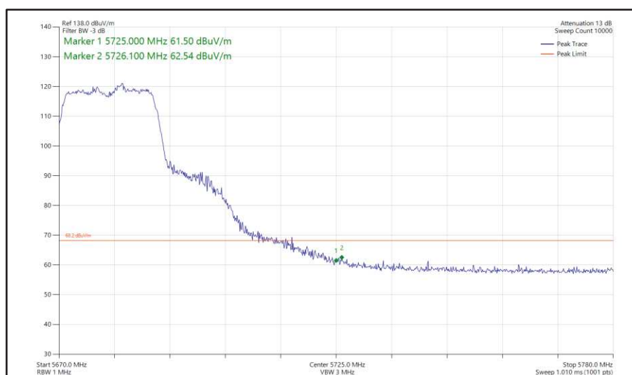
Figure 434 - 802.11ac VHT20, TxBF, Core 0 + Core 1 - 5680 MHz Band Edge Frequency 5725 MHz
