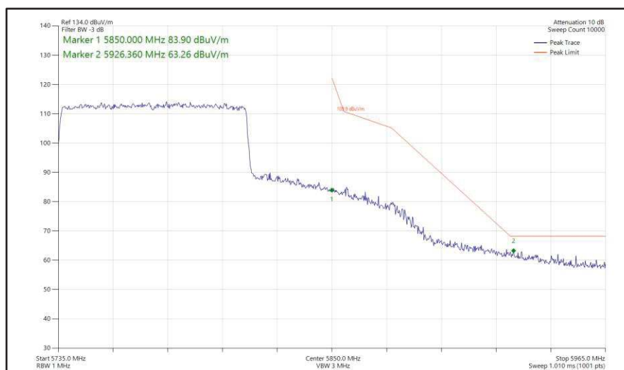
Figure 550 - 802.11ax HE80, SU, SISO, Core 1 - 5775 MHz Band Edge Frequency 5850 MHz
