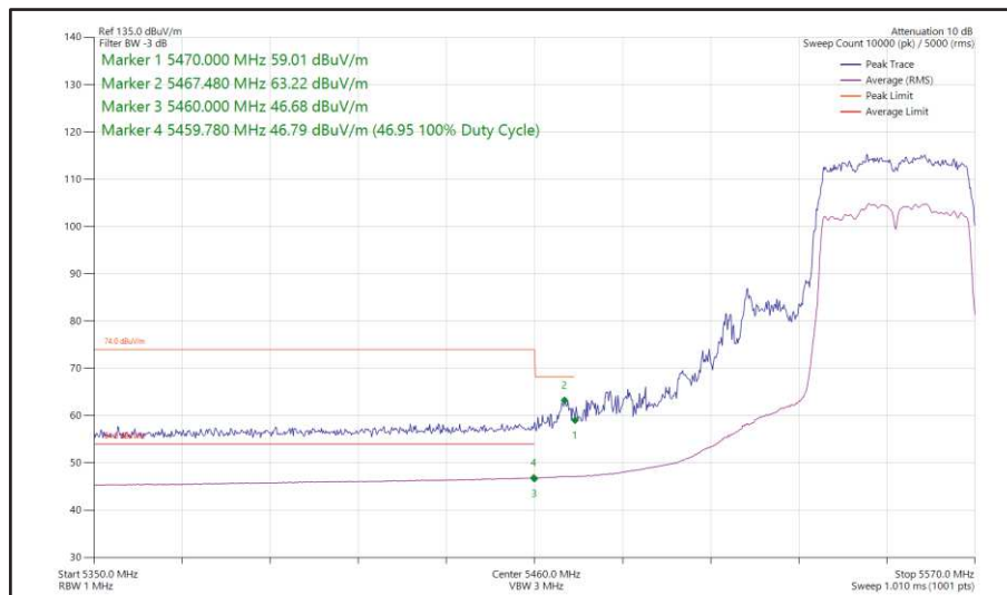
Figure 516 - 802.11ac VHT40, TxBF, Core 0 + Core 1 - 5550 MHz Band Edge Frequency 5470 MHz
