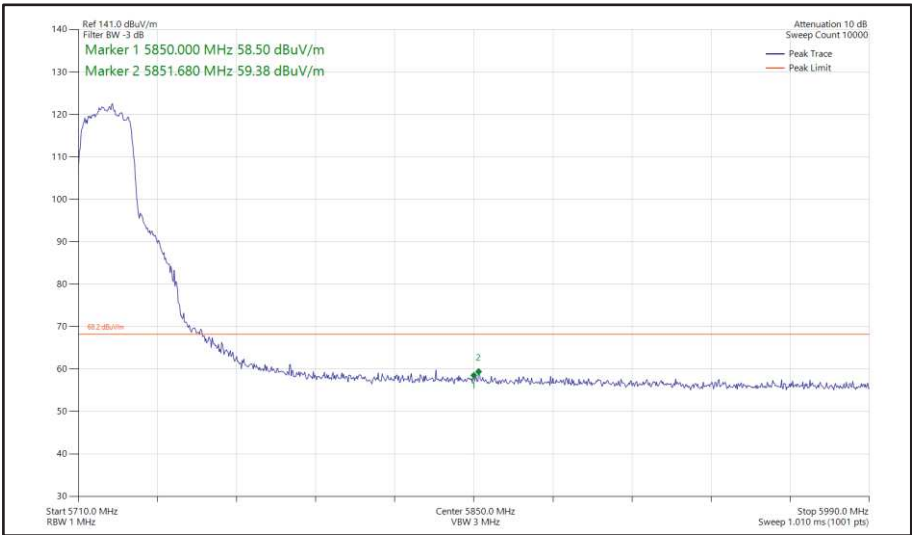
Figure 422 - 802.11n HT20, SDM, Core 0 + Core 1 - 5720 MHz Band Edge Frequency 5850 MHz
