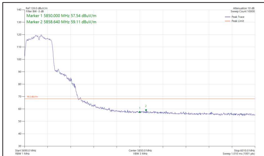
Figure 509 - 802.11n HT40, SDM, Core 0 + Core 1 - 5710 MHz Band Edge Frequency 5850 MHz
