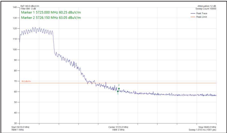
Figure 487 - 802.11ax HE40, SU, CDD, Core 0 + Core 1 - 5630 MHz Band Edge Frequency 5725 MHz
