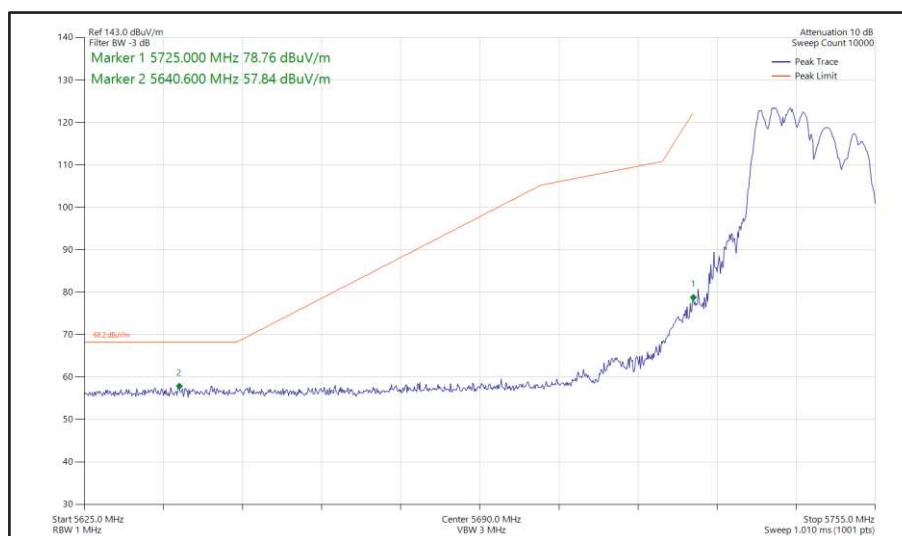
Figure 415 - 802.11ax HE20, RU 106-53, SDM, Core 0 + Core 1 - 5745 MHz Band Edge Frequency 5725 MHz
