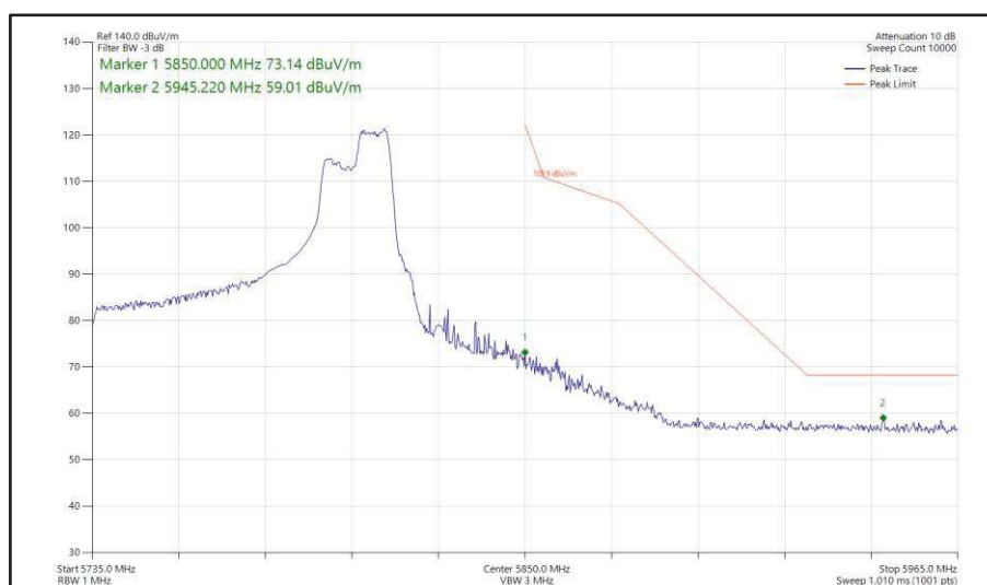
Figure 551 - 802.11ax HE80, RU 106-60, SISO, Core 1 - 5775 MHz Band Edge Frequency 5850 MHz
