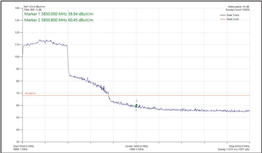
Figure 533 - 802.11ax HE80, SU, SISO, Core 0 - 5690 MHz Band Edge Frequency 5850 MHz
