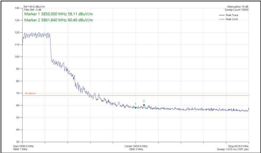
Figure 492 - 802.11ax HE40, SU, CDD, Core 0 + Core 1 - 5710 MHz Band Edge Frequency 5850 MHz
