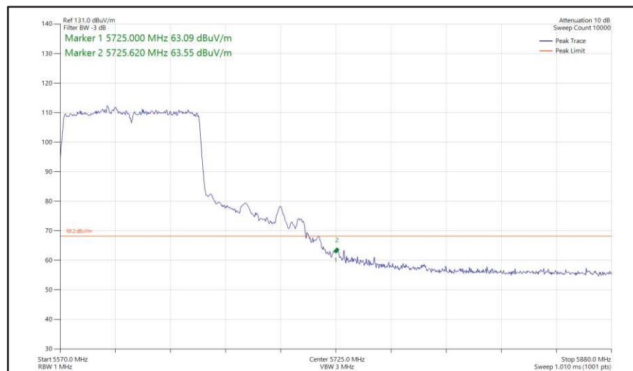
Figure 543 - 802.11ac VHT80, SISO, Core 1 - 5610 MHz Band Edge Frequency 5725 MHz
