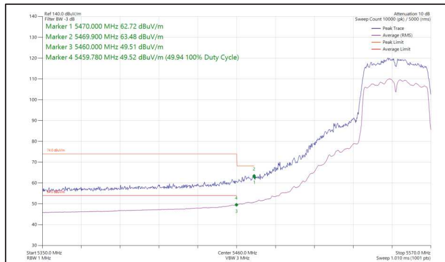
Figure 497 - 802.11n HT40, SDM, Core 0 + Core 1 - 5550 MHz Band Edge Frequency 5470 MHz
