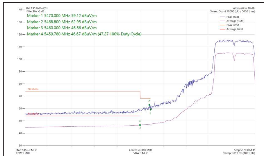
Figure 459 - 802.11n HT40, SISO, Core 1 - 5550 MHz Band Edge Frequency 5470 MHz
