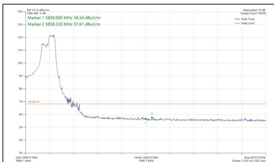
Figure 474 - 802.11ax HE40, RU 106-56, SISO, Core 1 - 5710 MHz Band Edge Frequency 5850 MHz
