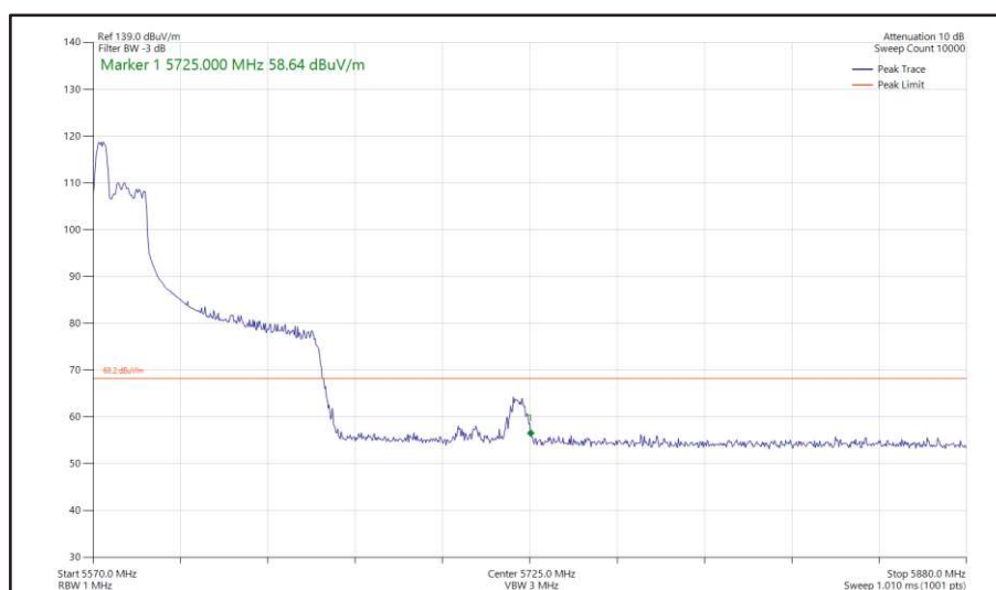
Figure 530 - 802.11ax HE80, RU 52-37, SISO, Core 0 - 5610 MHz Band Edge Frequency 5725 MHz
