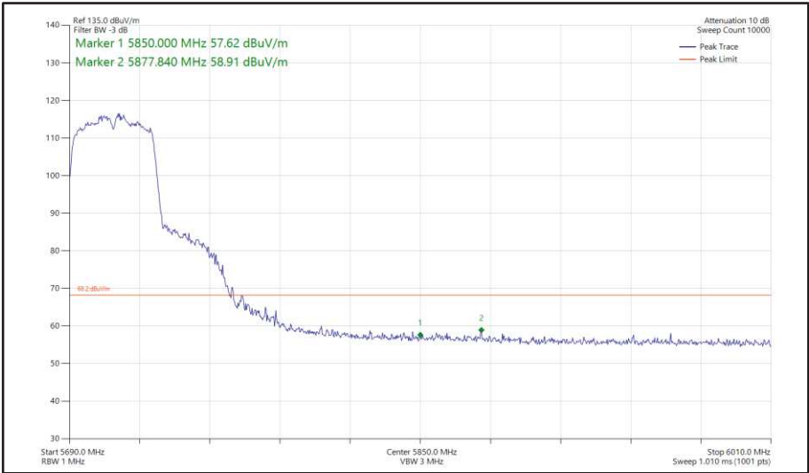
Figure 452 - 802.11n HT40, SISO, Core 0 - 5710 MHz Band Edge Frequency 5850 MHz
