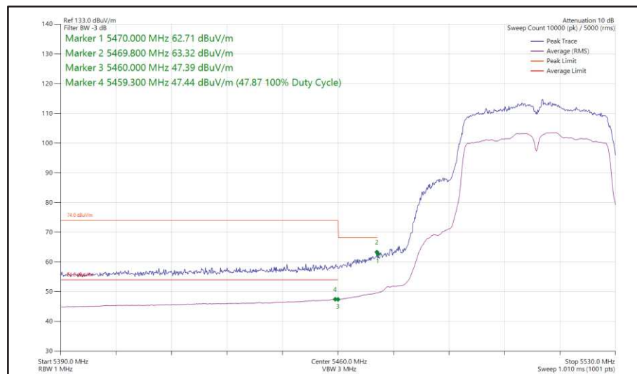
Figure 458 - 802.11n HT40, SISO, Core 1 - 5510 MHz Band Edge Frequency 5470 MHz
