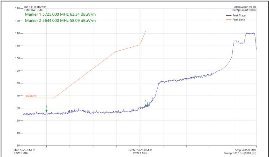
Figure 527 - 802.11ax HE80, RU 106-60, SISO, Core 0 - 5775 MHz Band Edge Frequency 5725 MHz
