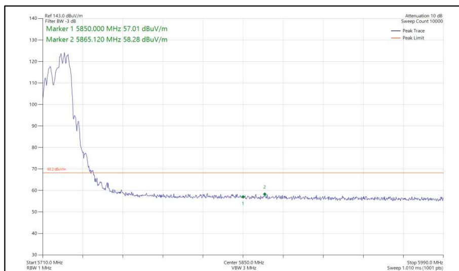
Figure 426 - 802.11ax HE20, RU 106-54, SDM, Core 0 + Core 1 - 5720 MHz Band Edge Frequency 5850 MHz
