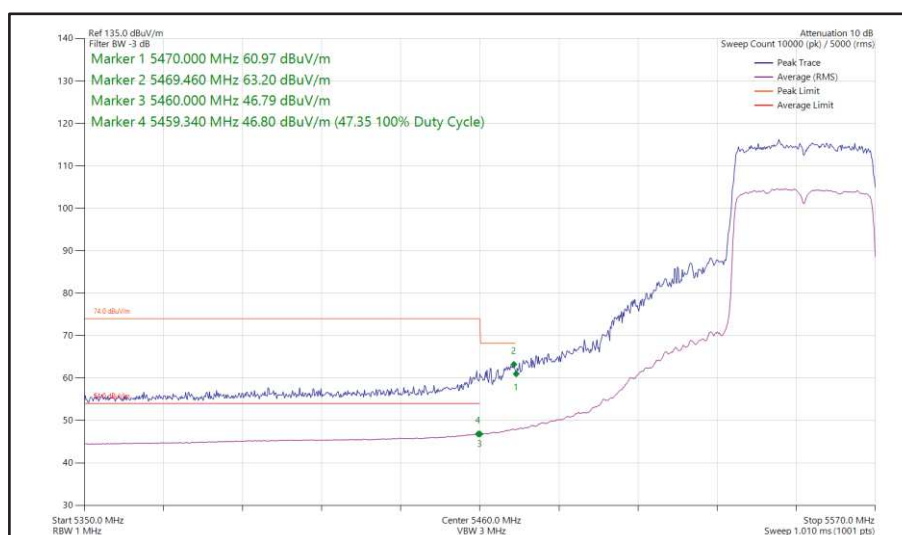
Figure 462 - 802.11ax HE40, SU, SISO, Core 1 - 5550 MHz Band Edge Frequency 5470 MHz
