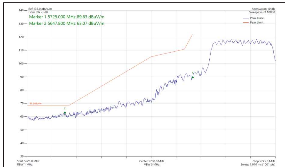
Figure 482 - 802.11n HT40, CDD, Core 0 + Core 1 - 5755 MHz Band Edge Frequency 5725 MHz
