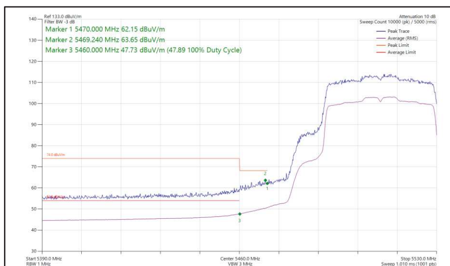
Figure 441 - 802.11ax HE40, SU, SISO, Core 0 - 5510 MHz Band Edge Frequency 5470 MHz
