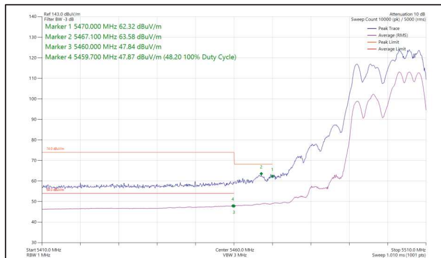
Figure 410 - 802.11ax HE20, RU 106-54, SDM, Core 0 + Core 1 - 5500 MHz Band Edge Frequency 5470 MHz
