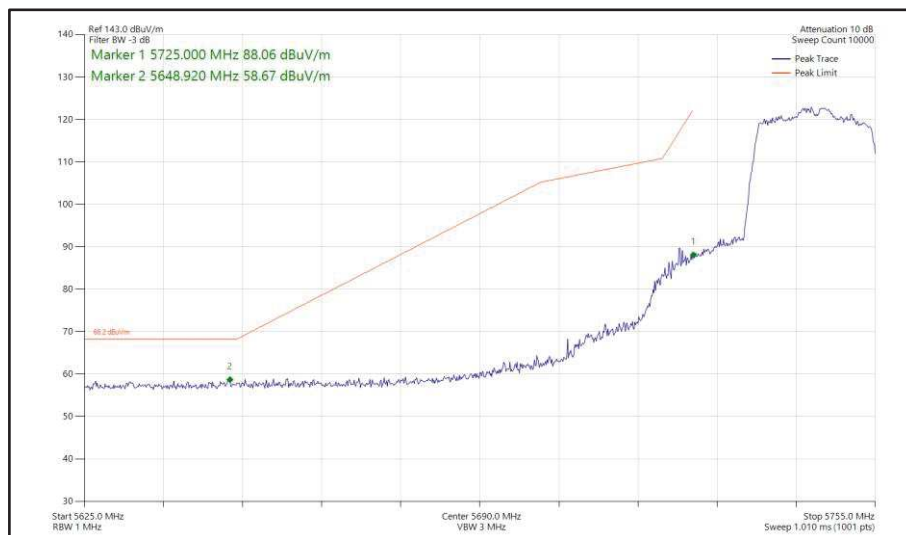
Figure 414 - 802.11ax HE20, SU, SDM, Core 0 + Core 1 - 5745 MHz Band Edge Frequency 5725 MHz
