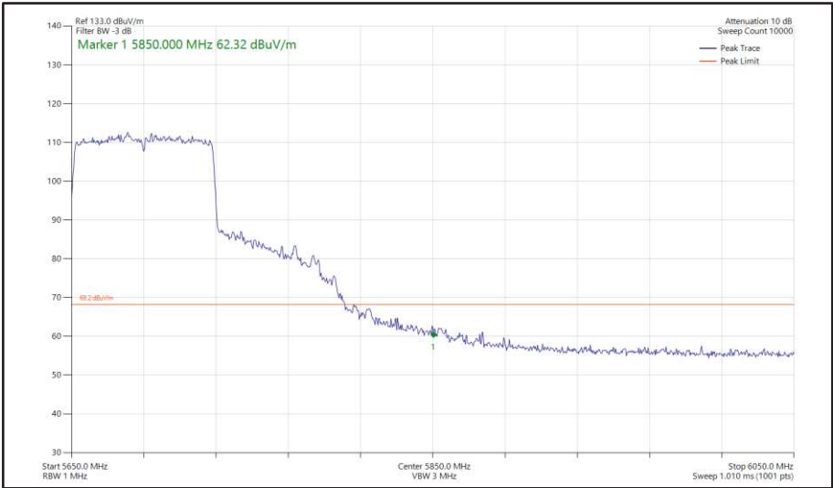
Figure 531 - 802.11ac VHT80, SISO, Core 0 - 5690 MHz Band Edge Frequency 5850 MHz
