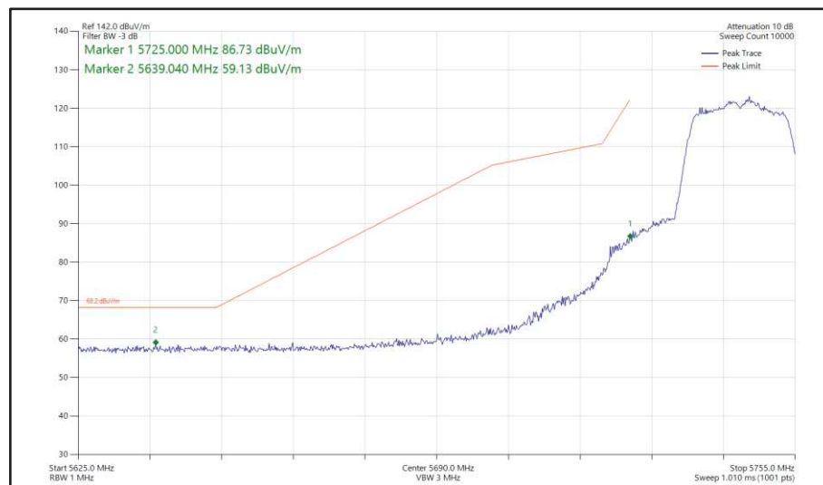
Figure 412 - 802.11n HT20, SDM, Core 0 + Core 1 - 5745 MHz Band Edge Frequency 5725 MHz
