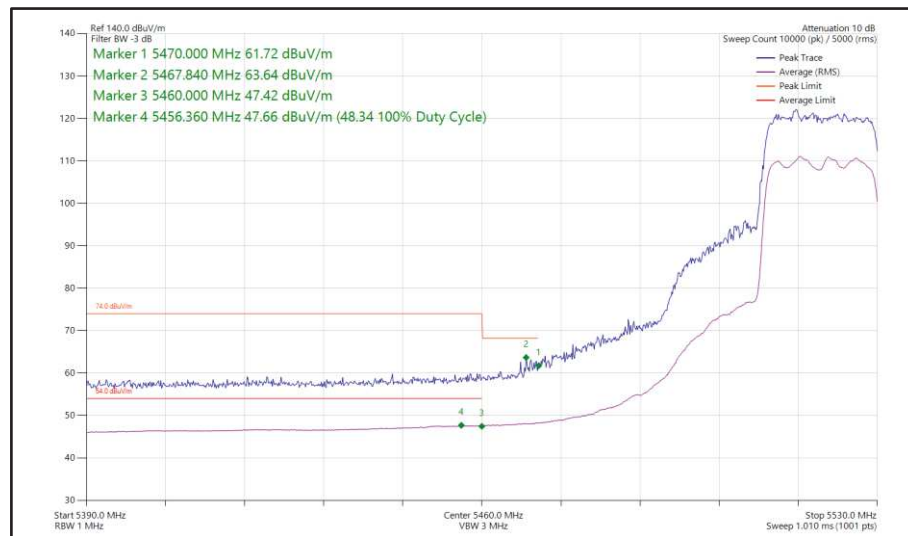
Figure 411 - 802.11ax HE20, SU, SDM, Core 0 + Core 1 - 5520 MHz Band Edge Frequency 5470 MHz
