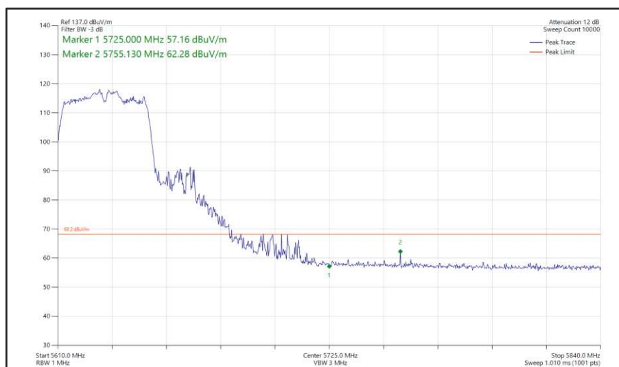
Figure 518 - 802.11ac VHT40, TxBF, Core 0 + Core 1 - 5630 MHz Band Edge Frequency 5725 MHz
