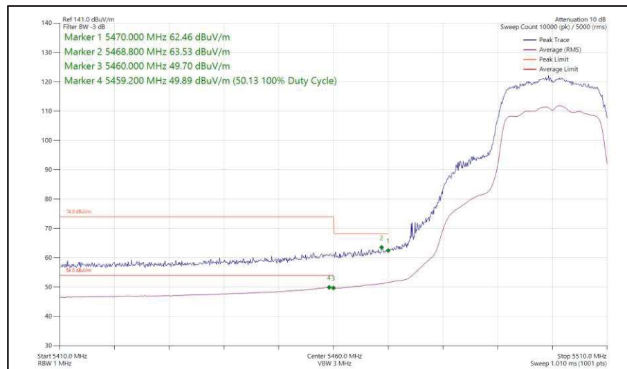
Figure 407 - 802.11n HT20, SDM, Core 0 + Core 1 - 5500 MHz Band Edge Frequency 5470 MHz
