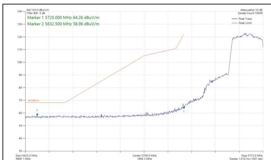
Figure 416 - 802.11ax HE20, SU, SDM, Core 0 + Core 1 - 5765 MHz Band Edge Frequency 5725 MHz
