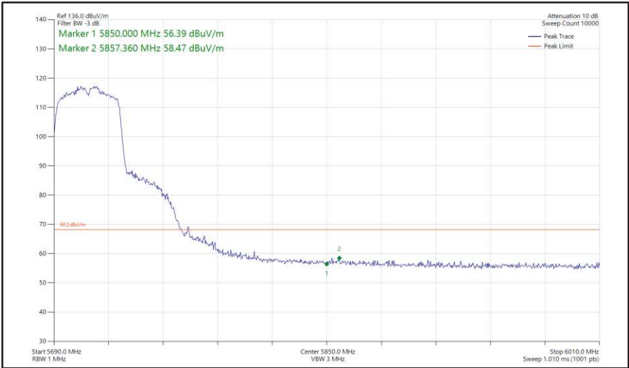
Figure 471 - 802.11n HT40, SISO, Core 1 - 5710 MHz Band Edge Frequency 5850 MHz
