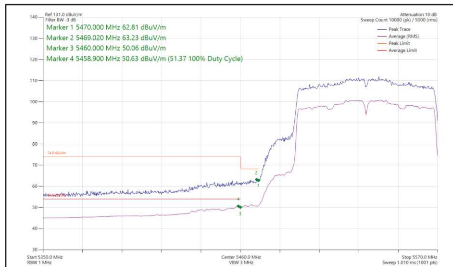
Figure 537 - 802.11ac VHT80, SISO, Core 1 - 5530 MHz Band Edge Frequency 5470 MHz
