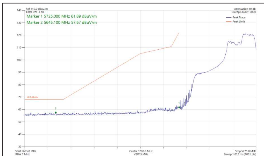
Figure 465 - 802.11ax HE40, RU 106-56, SISO, Core 1 - 5755 MHz Band Edge Frequency 5725 MHz
