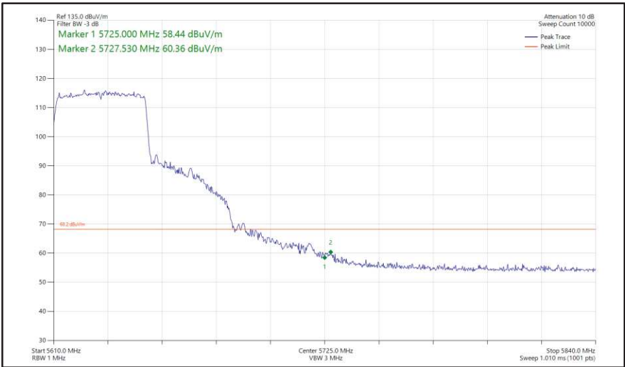
Figure 449 - 802.11ax HE40, SU, SISO, Core 0 - 5630 MHz Band Edge Frequency 5725 MHz
