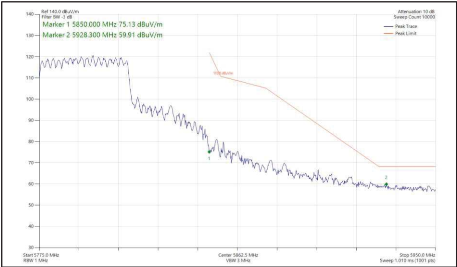
Figure 494 - 802.11ax HE40, SU, CDD, Core 0 + Core 1 - 5795 MHz Band Edge Frequency 5850 MHz
