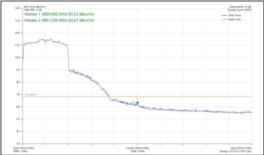
Figure 546 - 802.11ac VHT80, SISO, Core 1 - 5690 MHz Band Edge Frequency 5850 MHz
