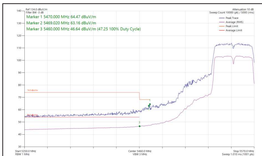
Figure 440 - 802.11n HT40, SISO, Core 0 - 5550 MHz Band Edge Frequency 5470 MHz
