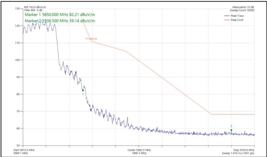
Figure 405 - 802.11ax HE20, SU, CDD, Core 0 + Core 1 - 5825 MHz Band Edge Frequency 5850 MHz
