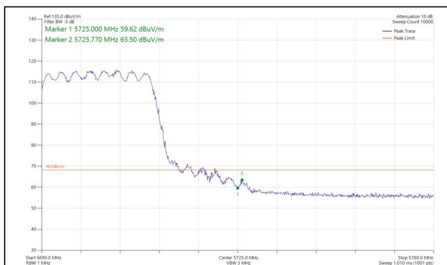
Figure 397 - 802.11ax HE20, SU, CDD, Core 0 + Core 1 - 5700 MHz Band Edge Frequency 5725 MHz
