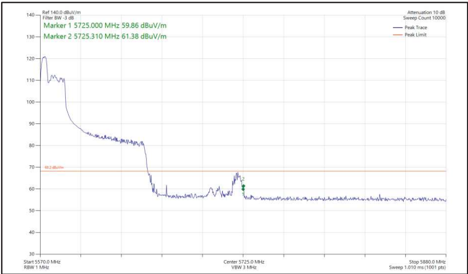
Figure 545 - 802.11ax HE80, RU 52-37, SISO, Core 1 - 5610 MHz Band Edge Frequency 5725 MHz
