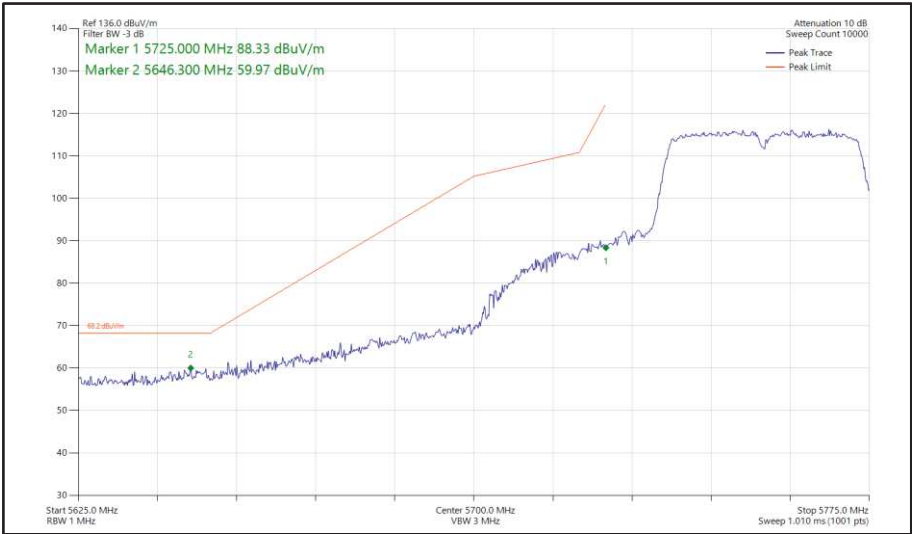
Figure 444 - 802.11n HT40, SISO, Core 0 - 5755 MHz Band Edge Frequency 5725 MHz
