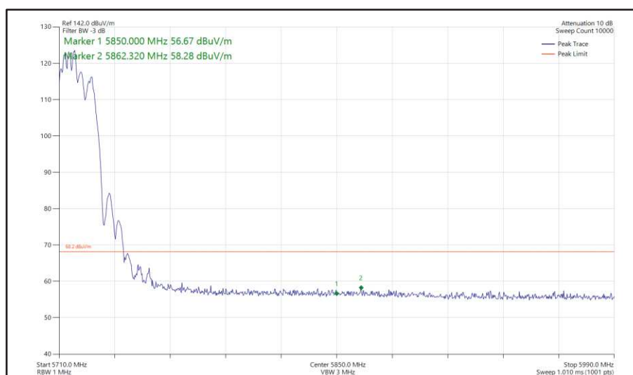
Figure 403 - 802.11ax HE20, RU 106-53, CDD, Core 0 + Core 1 - 5720 MHz Band Edge Frequency 5850 MHz
