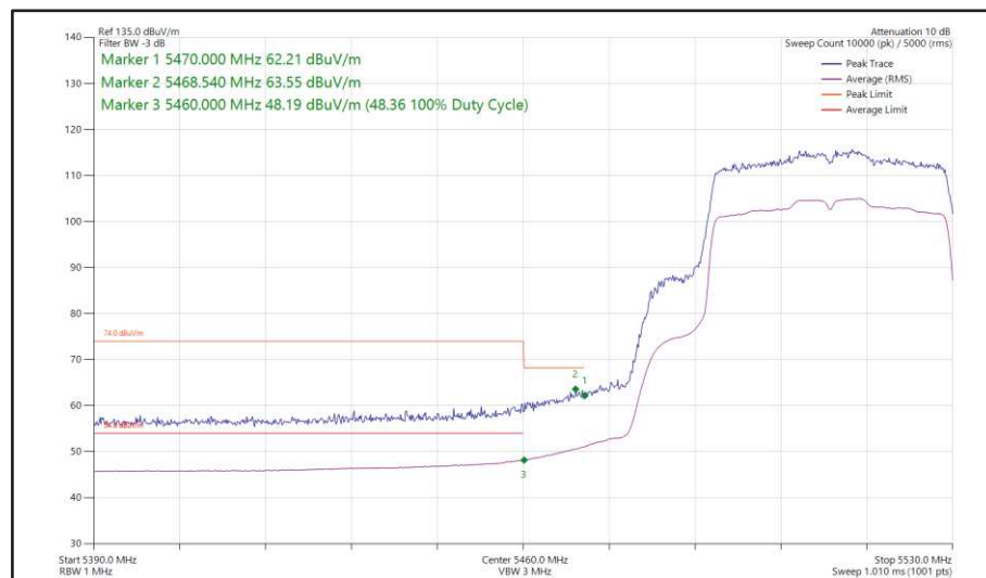
Figure 460 - 802.11ax HE40, SU, SISO, Core 1 - 5510 MHz Band Edge Frequency 5470 MHz
