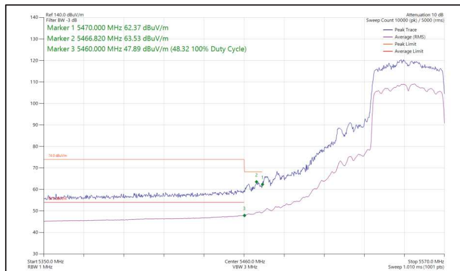
Figure 500 - 802.11ax HE40, SU, SDM, Core 0 + Core 1 - 5550 MHz Band Edge Frequency 5470 MHz
