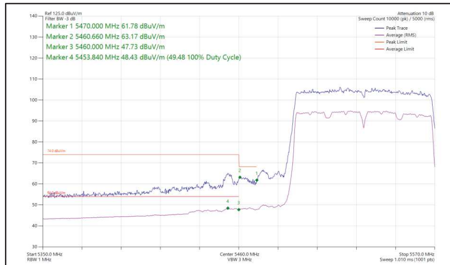
Figure 522 - 802.11ac VHT80, SISO, Core 0 - 5530 MHz Band Edge Frequency 5470 MHz
