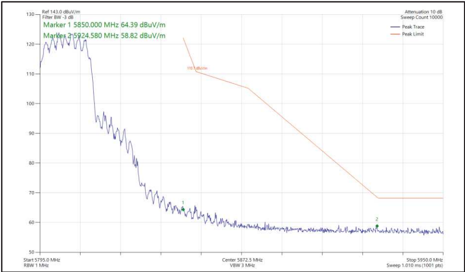
Figure 404 - 802.11ax HE20, SU, CDD, Core 0 + Core 1 - 5805 MHz Band Edge Frequency 5850 MHz
