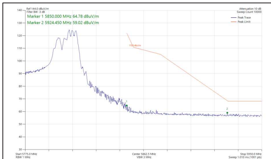
Figure 514 - 802.11ax HE40, RU 106-56, SDM, Core 0 + Core 1 - 5795 MHz Band Edge Frequency 5850 MHz
