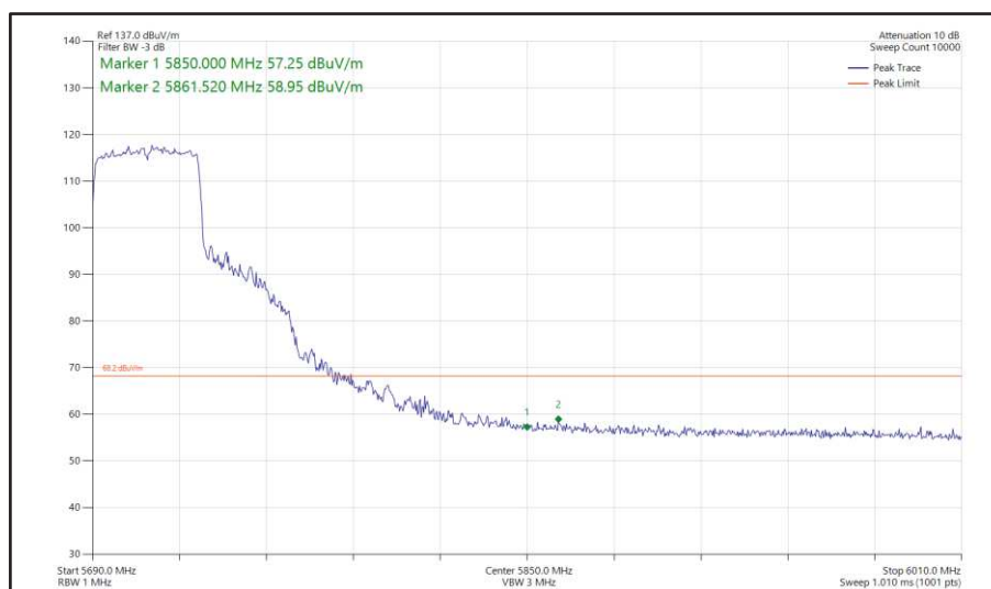
Figure 473 - 802.11ax HE40, SU, SISO, Core 1 - 5710 MHz Band Edge Frequency 5850 MHz
