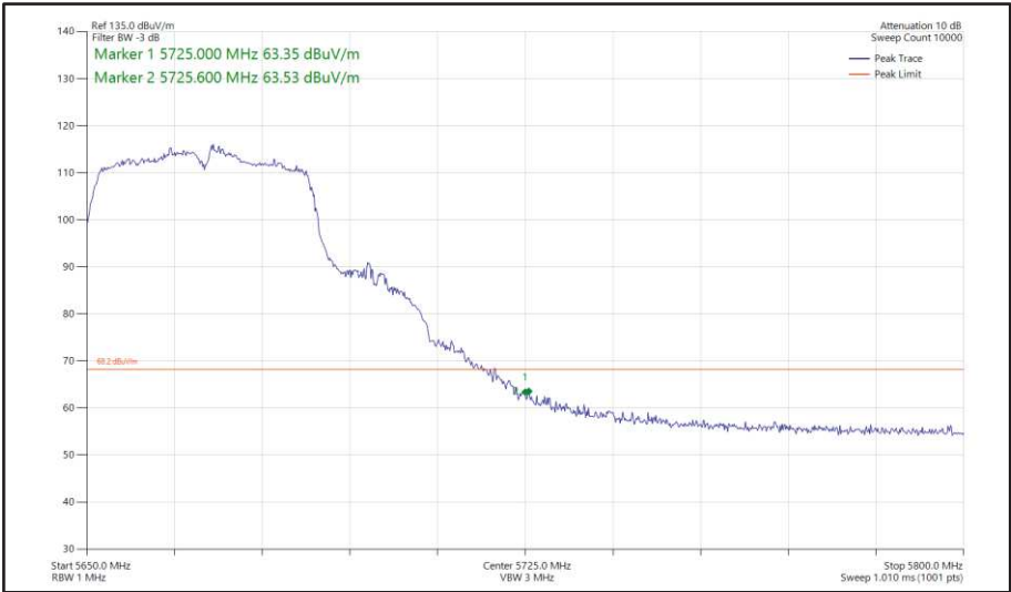
Figure 448 - 802.11n HT40, SISO, Core 0 - 5670 MHz Band Edge Frequency 5725 MHz
