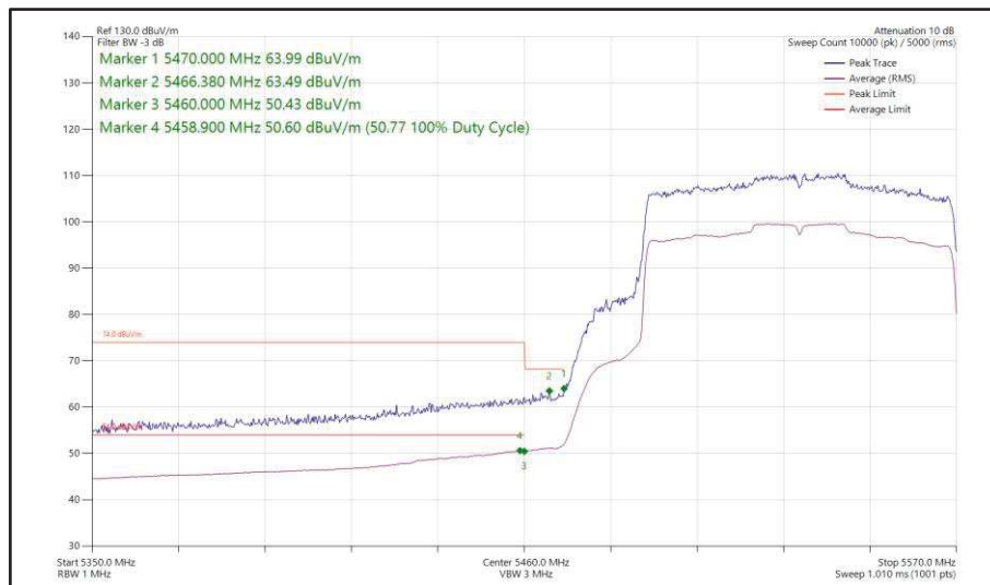
Figure 523 - 802.11ax HE80, SU, SISO, Core 0 - 5530 MHz Band Edge Frequency 5470 MHz
