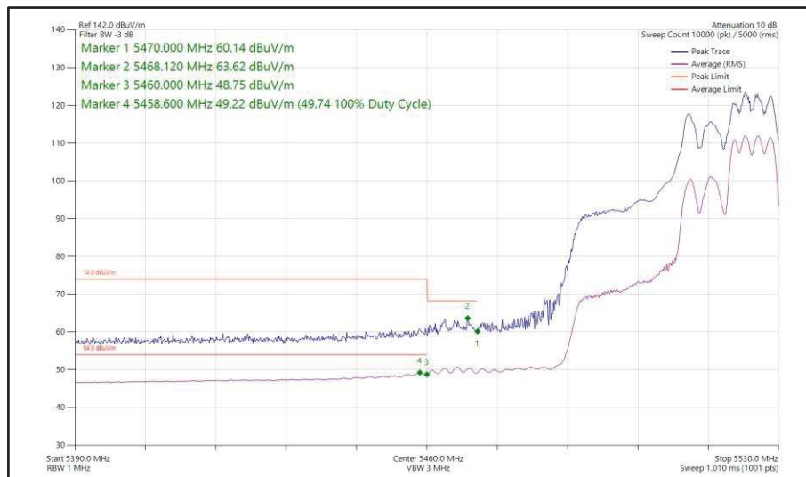
Figure 480 - 802.11ax HE40, RU 106-56, CDD, Core 0 + Core 1 - 5510 MHz Band Edge Frequency 5470 MHz
