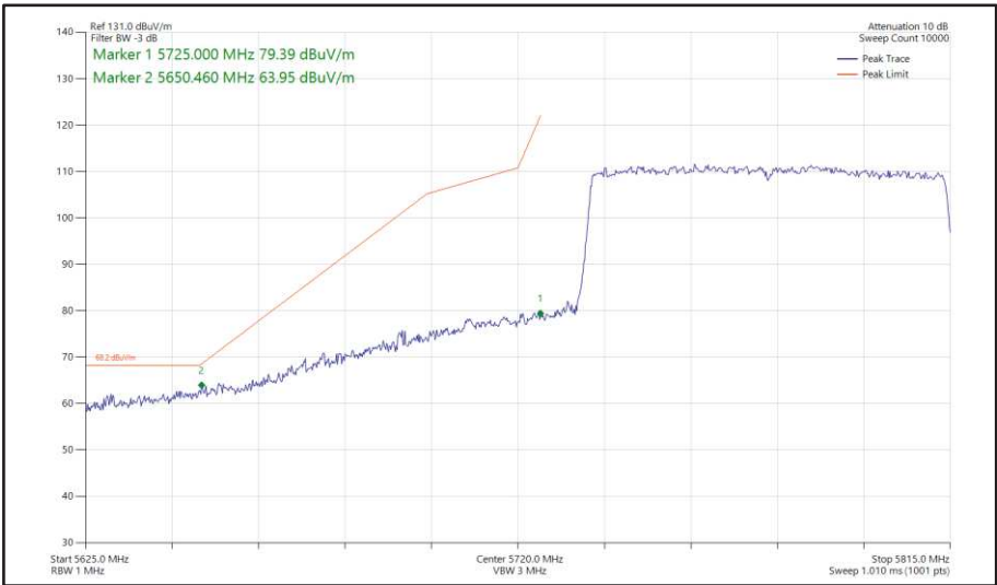
Figure 541 - 802.11ax HE80, SU, SISO, Core 1 - 5775 MHz Band Edge Frequency 5725 MHz
