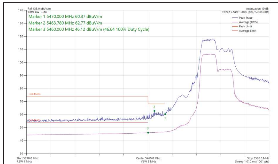
Figure 442 - 802.11ax HE40, RU 106-53, SISO, Core 0 - 5510 MHz Band Edge Frequency 5470 MHz
