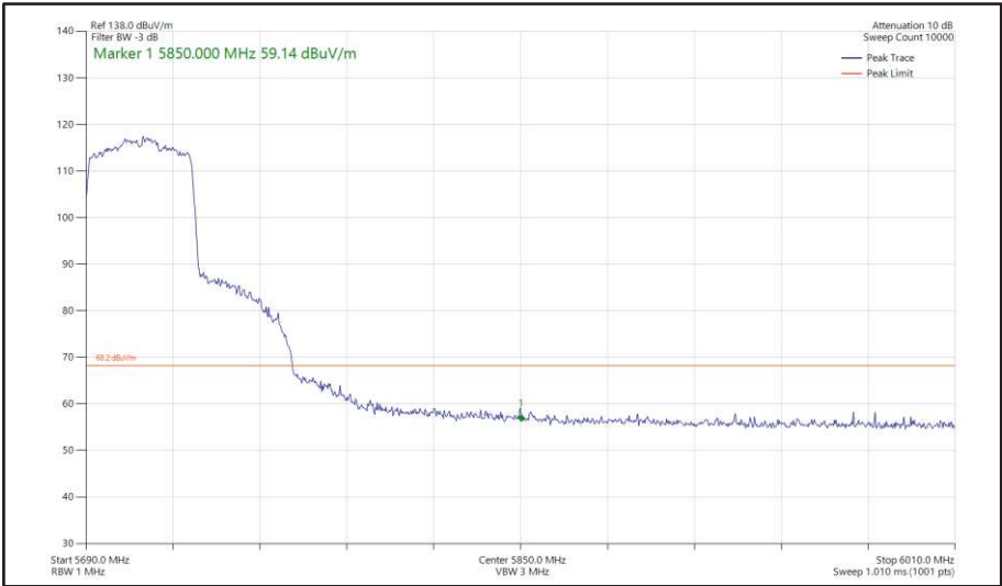
Figure 454 - 802.11ax HE40, SU, SISO, Core 0 - 5710 MHz Band Edge Frequency 5850 MHz
