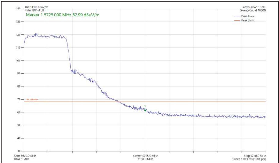
Figure 419 - 802.11ax HE20, SU, SDM, Core 0 + Core 1 - 5680 MHz Band Edge Frequency 5725 MHz
