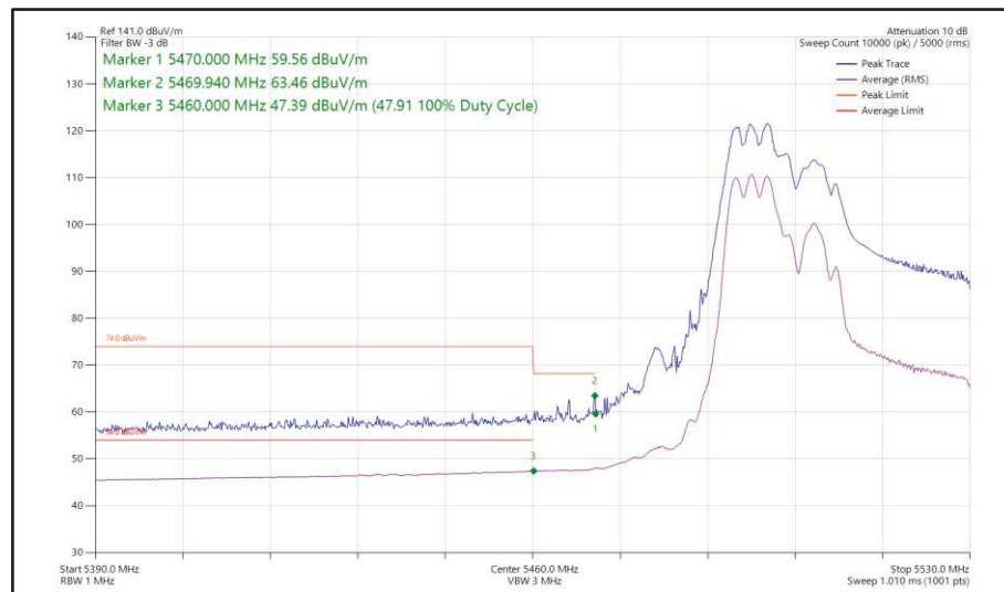
Figure 499 - 802.11ax HE40, RU 106-53, SDM, Core 0 + Core 1 - 5510 MHz Band Edge Frequency 5470 MHz
