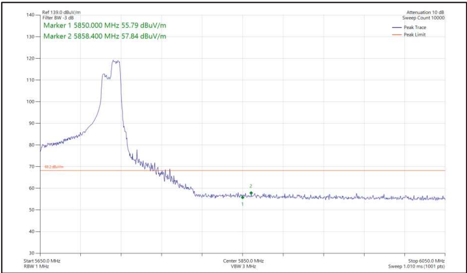
Figure 534 - 802.11ax HE80, RU 106-60, SISO, Core 0 - 5690 MHz Band Edge Frequency 5850 MHz
