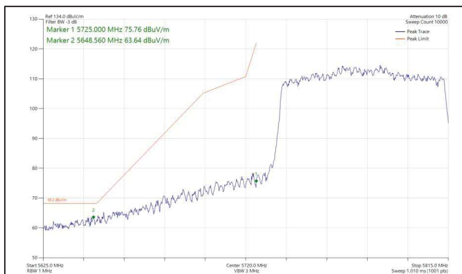
Figure 555 - 802.11ac VHT80, CDD, Core 0 + Core 1 - 5775 MHz Band Edge Frequency 5725 MHz
