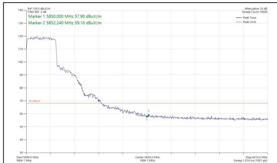
Figure 511 - 802.11ax HE40, SU, SDM, Core 0 + Core 1 - 5710 MHz Band Edge Frequency 5850 MHz
