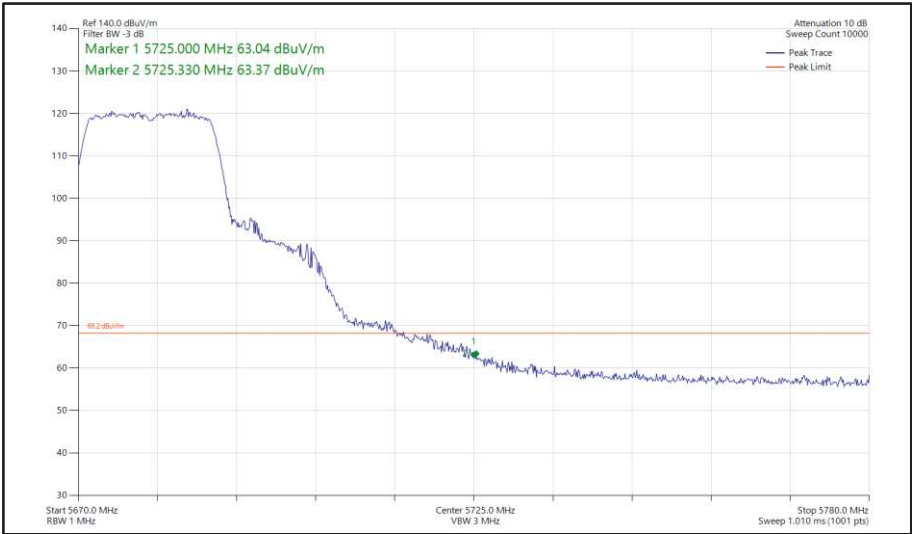
Figure 417 - 802.11n HT20, SDM, Core 0 + Core 1 - 5680 MHz Band Edge Frequency 5725 MHz
