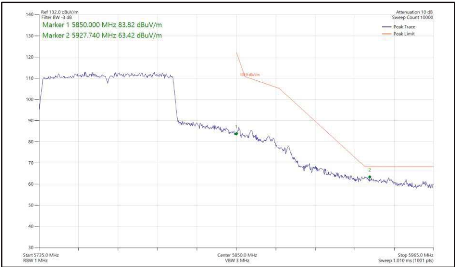
Figure 532 - 802.11ac VHT80, SISO, Core 0 - 5775 MHz Band Edge Frequency 5850 MHz
