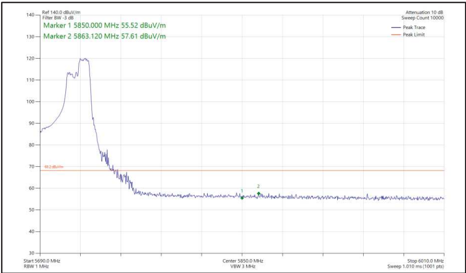
Figure 455 - 802.11ax HE40, RU 106-56, SISO, Core 0 - 5710 MHz Band Edge Frequency 5850 MHz
