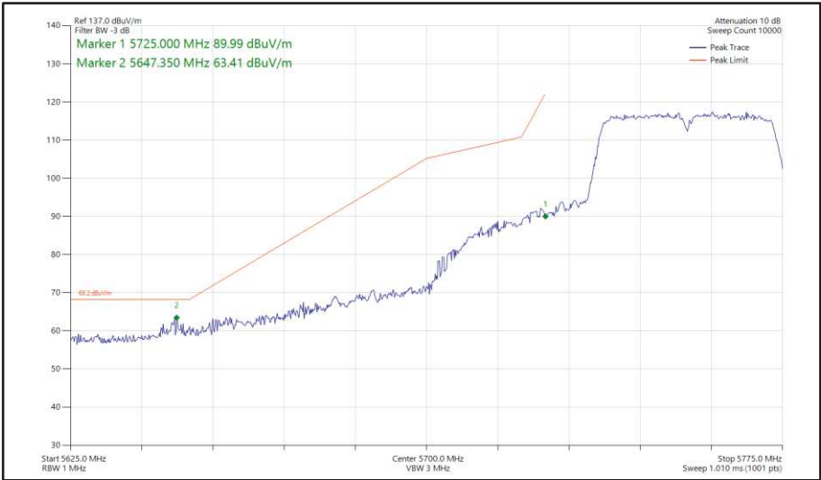
Figure 463 - 802.11n HT40, SISO, Core 1 - 5755 MHz Band Edge Frequency 5725 MHz
