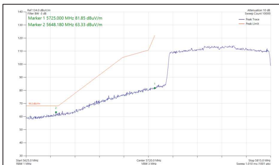
Figure 526 - 802.11ax HE80, SU, SISO, Core 0 - 5775 MHz Band Edge Frequency 5725 MHz
