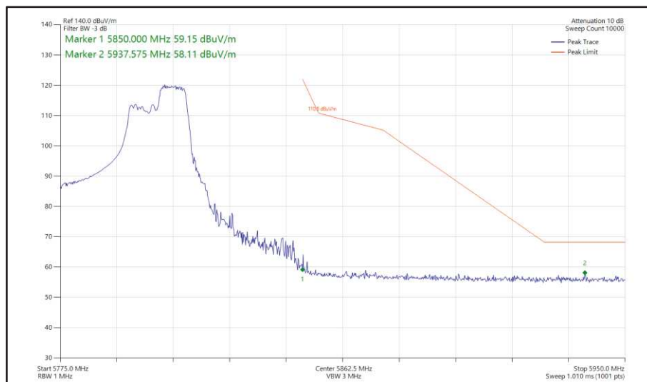
Figure 457 - 802.11ax HE40, RU 106-56, SISO, Core 0 - 5795 MHz Band Edge Frequency 5850 MHz
