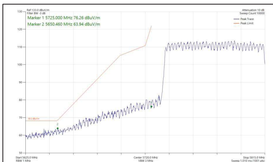
Figure 556 - 802.11ax HE80, SU, CDD, Core 0 + Core 1 - 5775 MHz Band Edge Frequency 5725 MHz
