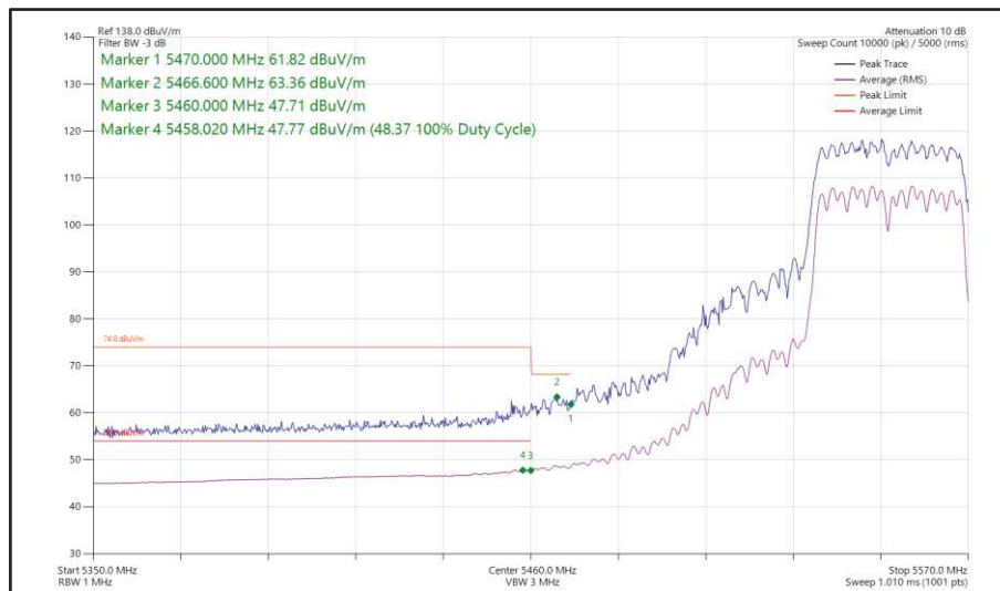
Figure 478 - 802.11n HT40, CDD, Core 0 + Core 1 - 5550 MHz Band Edge Frequency 5470 MHz
