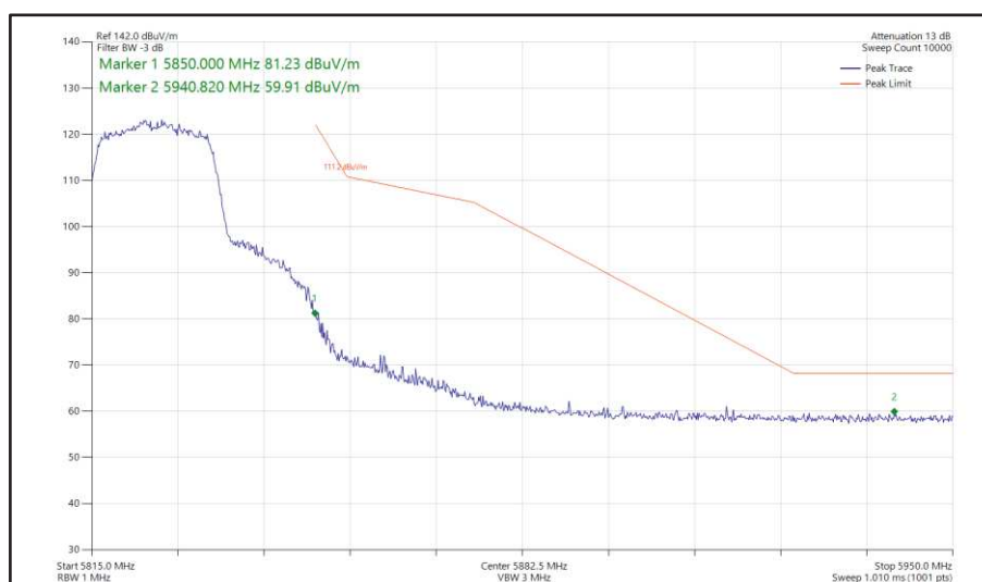
Figure 438 - 802.11ac VHT20, TxBF, Core 0 + Core 1 - 5825 MHz Band Edge Frequency 5850 MHz
