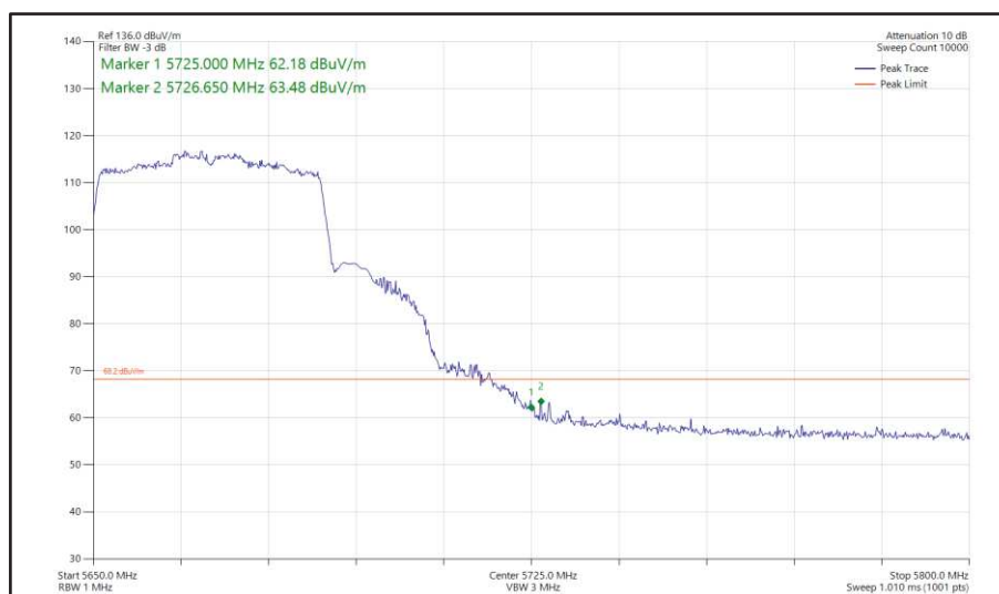
Figure 469 - 802.11ax HE40, SU, SISO, Core 1 - 5670 MHz Band Edge Frequency 5725 MHz
