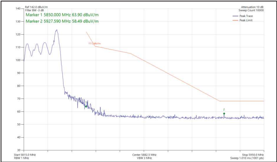
Figure 429 - 802.11ax HE20, RU 26-8, SDM, Core 0 + Core 1 - 5825 MHz Band Edge Frequency 5850 MHz
