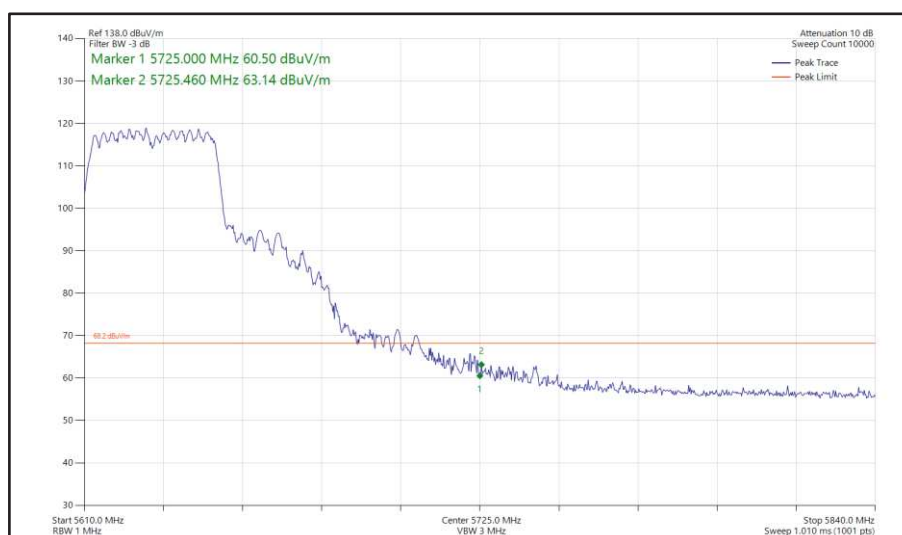
Figure 485 - 802.11n HT40, CDD, Core 0 + Core 1 - 5630 MHz Band Edge Frequency 5725 MHz
