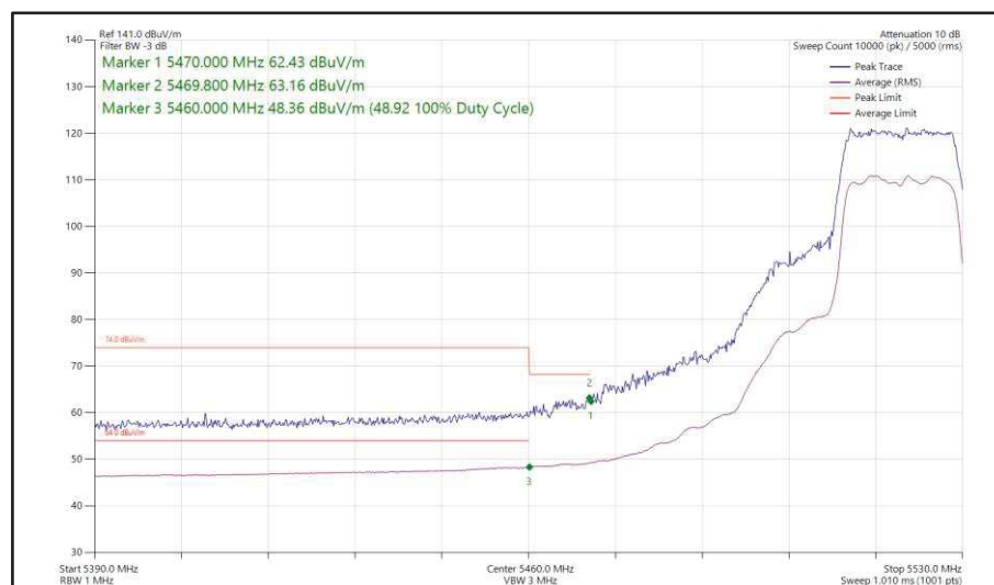
Figure 408 - 802.11n HT20, SDM, Core 0 + Core 1 - 5520 MHz Band Edge Frequency 5470 MHz
