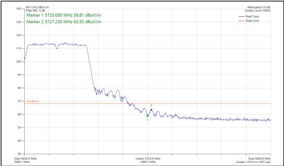
Figure 505 - 802.11n HT40, SDM, Core 0 + Core 1 - 5670 MHz Band Edge Frequency 5725 MHz
