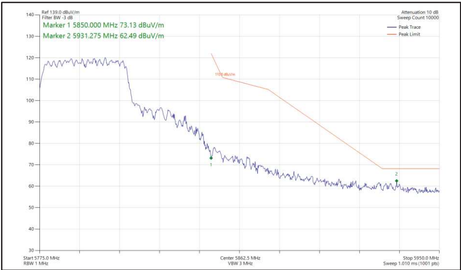
Figure 491 - 802.11n HT40, CDD, Core 0 + Core 1 - 5795 MHz Band Edge Frequency 5850 MHz
