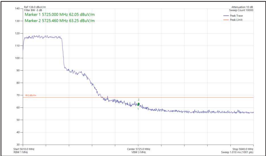
Figure 506 - 802.11ax HE40, SU, SDM, Core 0 + Core 1 - 5630 MHz Band Edge Frequency 5725 MHz
