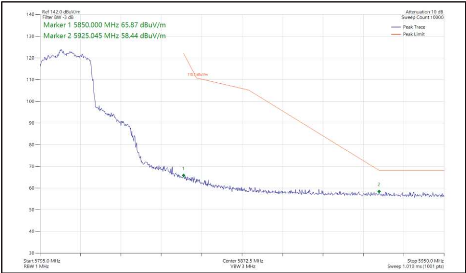
Figure 427 - 802.11ax HE20, SU, SDM, Core 0 + Core 1 - 5805 MHz Band Edge Frequency 5850 MHz
