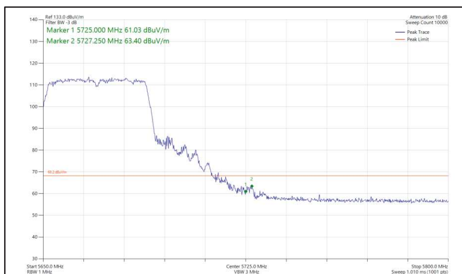
Figure 519 - 802.11ac VHT40, TxBF, Core 0 + Core 1 - 5670 MHz Band Edge Frequency 5725 MHz
