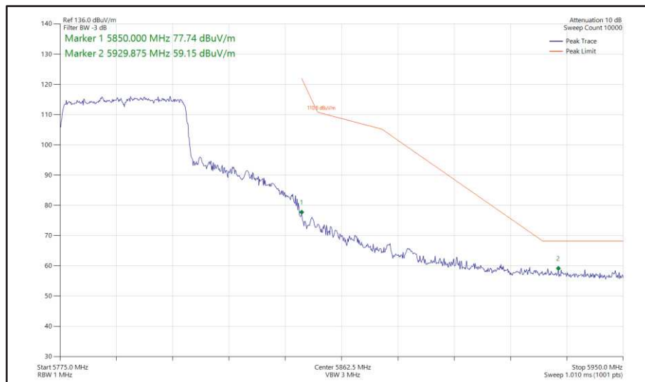
Figure 456 - 802.11ax HE40, SU, SISO, Core 0 - 5795 MHz Band Edge Frequency 5850 MHz
