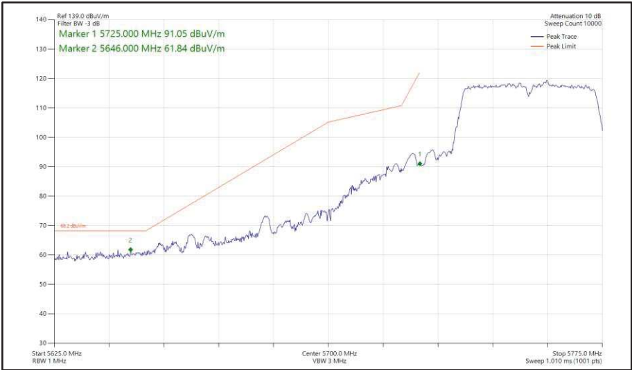
Figure 501 - 802.11n HT40, SDM, Core 0 + Core 1 - 5755 MHz Band Edge Frequency 5725 MHz
