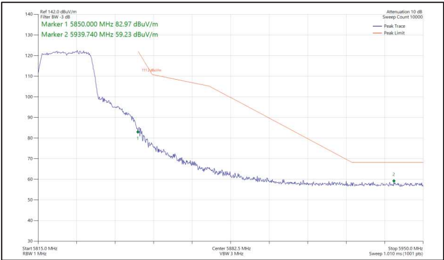
Figure 424 - 802.11n HT20, SDM, Core 0 + Core 1 - 5825 MHz Band Edge Frequency 5850 MHz
