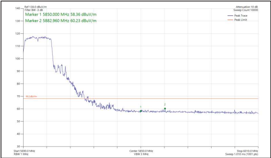
Figure 520 - 802.11ac VHT40, TxBF, Core 0 + Core 1 - 5710 MHz Band Edge Frequency 5850 MHz
