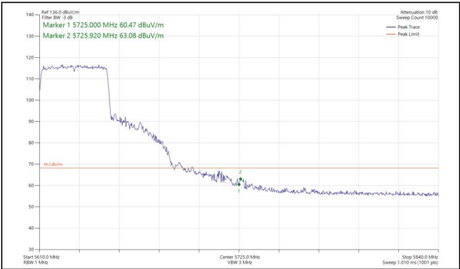
Figure 468 - 802.11ax HE40, SU, SISO, Core 1 - 5630 MHz Band Edge Frequency 5725 MHz
