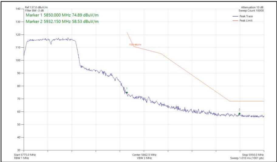
Figure 472 - 802.11n HT40, SISO, Core 1 - 5795 MHz Band Edge Frequency 5850 MHz
