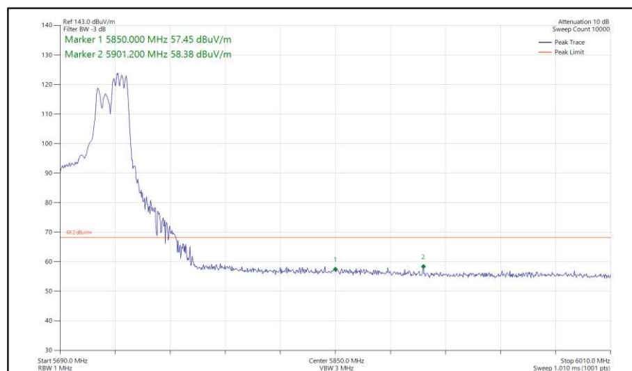
Figure 512 - 802.11ax HE40, RU 106-56, SDM, Core 0 + Core 1 - 5710 MHz Band Edge Frequency 5850 MHz
