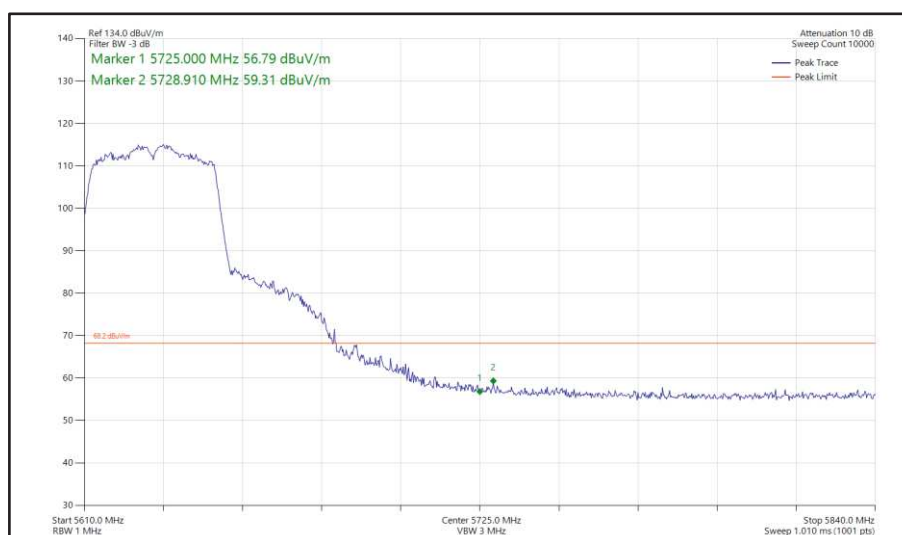
Figure 447 - 802.11n HT40, SISO, Core 0 - 5630 MHz Band Edge Frequency 5725 MHz
