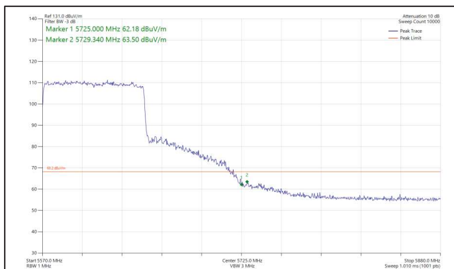
Figure 529 - 802.11ax HE80, SU, SISO, Core 0 - 5610 MHz Band Edge Frequency 5725 MHz
