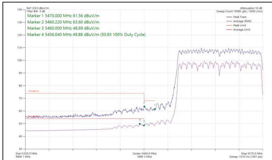
Figure 552 - 802.11ac VHT80, CDD, Core 0 + Core 1 - 5530 MHz Band Edge Frequency 5470 MHz
