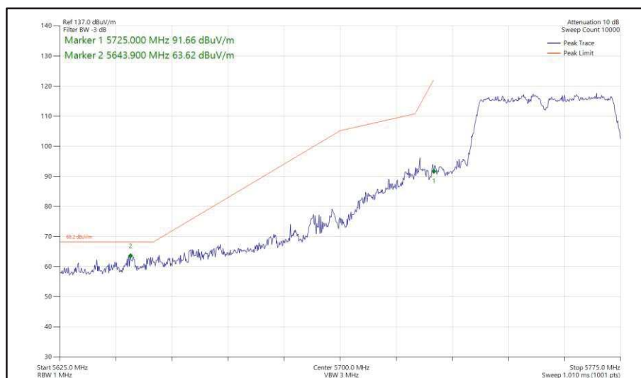
Figure 517 - 802.11ac VHT40, TxBF, Core 0 + Core 1 - 5755 MHz Band Edge Frequency 5725 MHz
