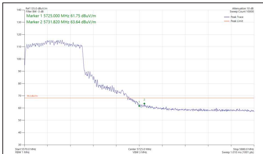
Figure 558 - 802.11ac VHT80, CDD, Core 0 + Core 1 - 5610 MHz Band Edge Frequency 5725 MHz
