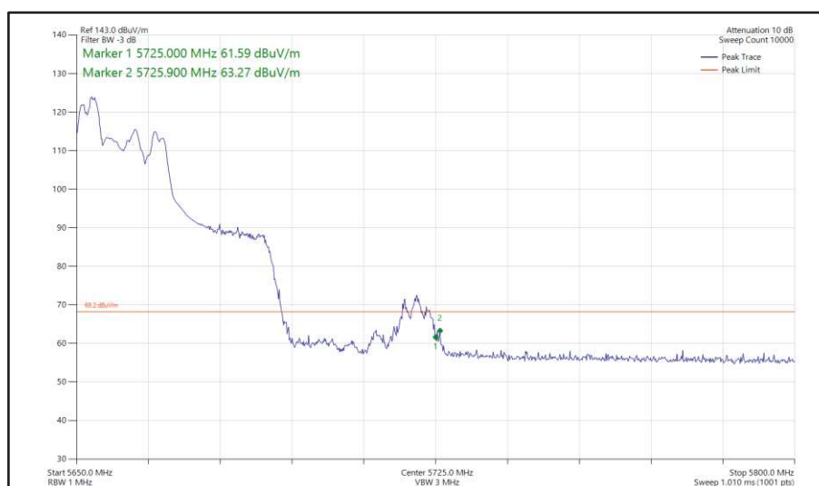
Figure 508 - 802.11ax HE40, RU 52-37, SDM, Core 0 + Core 1 - 5670 MHz Band Edge Frequency 5725 MHz
