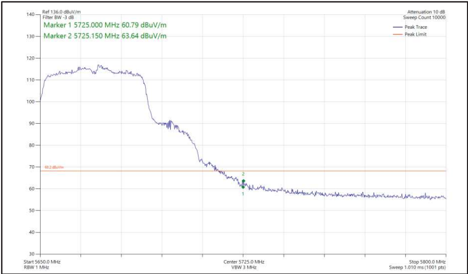
Figure 467 - 802.11n HT40, SISO, Core 1 - 5670 MHz Band Edge Frequency 5725 MHz
