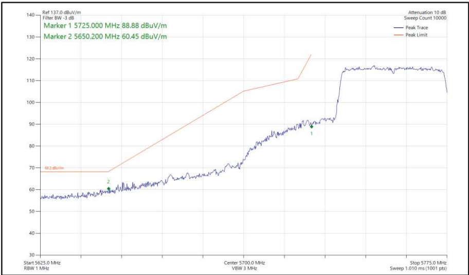
Figure 445 - 802.11ax HE40, SU, SISO, Core 0 - 5755 MHz Band Edge Frequency 5725 MHz
