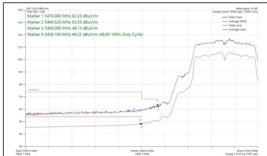
Figure 496 - 802.11n HT40, SDM, Core 0 + Core 1 - 5510 MHz Band Edge Frequency 5470 MHz
