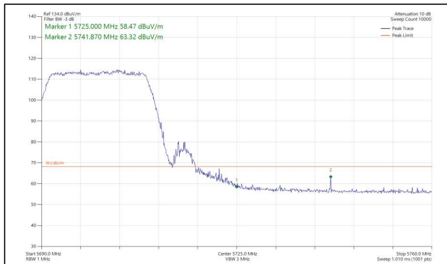
Figure 435 - 802.11ac VHT20, TxBF, Core 0 + Core 1 - 5700 MHz Band Edge Frequency 5725 MHz
