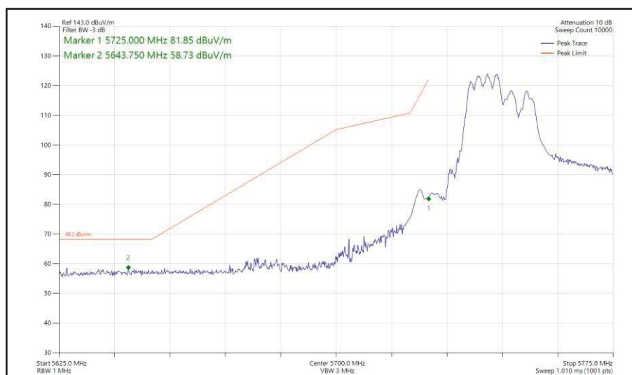
Figure 503 - 802.11ax HE40, RU 106-53, SDM, Core 0 + Core 1 - 5755 MHz Band Edge Frequency 5725 MHz
