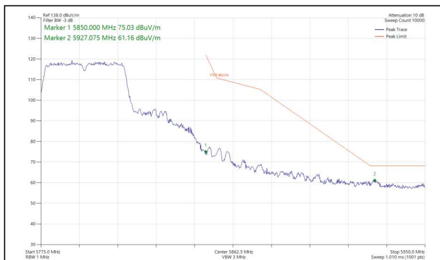
Figure 510 - 802.11n HT40, SDM, Core 0 + Core 1 - 5795 MHz Band Edge Frequency 5850 MHz
