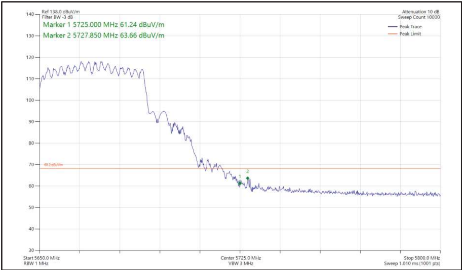
Figure 488 - 802.11ax HE40, SU, CDD, Core 0 + Core 1 - 5670 MHz Band Edge Frequency 5725 MHz
