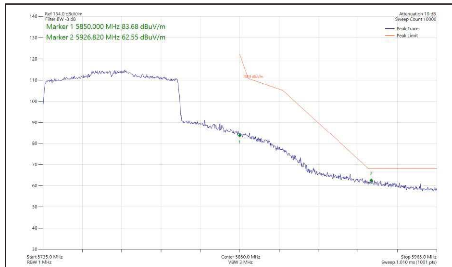
Figure 535 - 802.11ax HE80, SU, SISO, Core 0 - 5775 MHz Band Edge Frequency 5850 MHz
