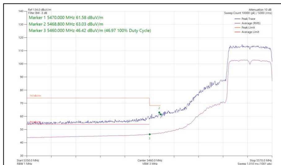
Figure 443 - 802.11ax HE40, SU, SISO, Core 0 - 5550 MHz Band Edge Frequency 5470 MHz
