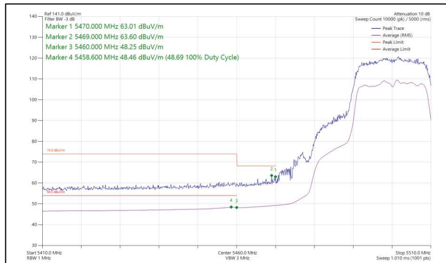
Figure 430 - 802.11ac VHT20, TxBF, Core 0 + Core 1 - 5500 MHz Band Edge Frequency 5470 MHz
