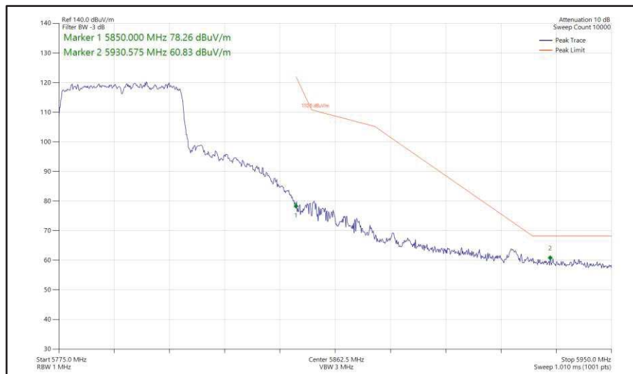
Figure 513 - 802.11ax HE40, SU, SDM, Core 0 + Core 1 - 5795 MHz Band Edge Frequency 5850 MHz
