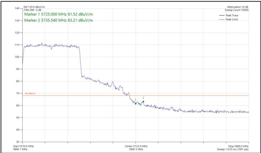
Figure 528 - 802.11ac VHT80, SISO, Core 0 - 5610 MHz Band Edge Frequency 5725 MHz
