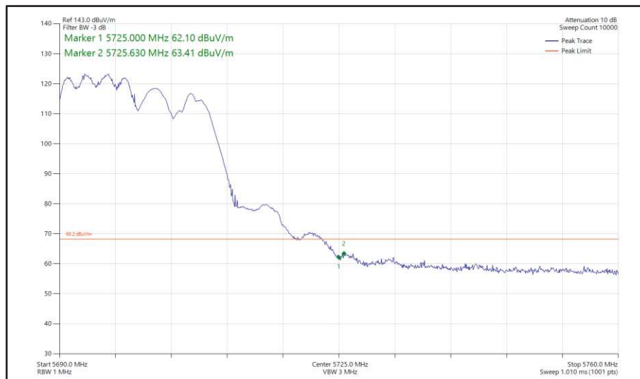
Figure 398 - 802.11ax HE20, RU 106-53, CDD, Core 0 + Core 1 - 5700 MHz Band Edge Frequency 5725 MHz
