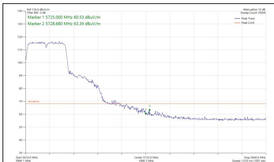
Figure 466 - 802.11n HT40, SISO, Core 1 - 5630 MHz Band Edge Frequency 5725 MHz
