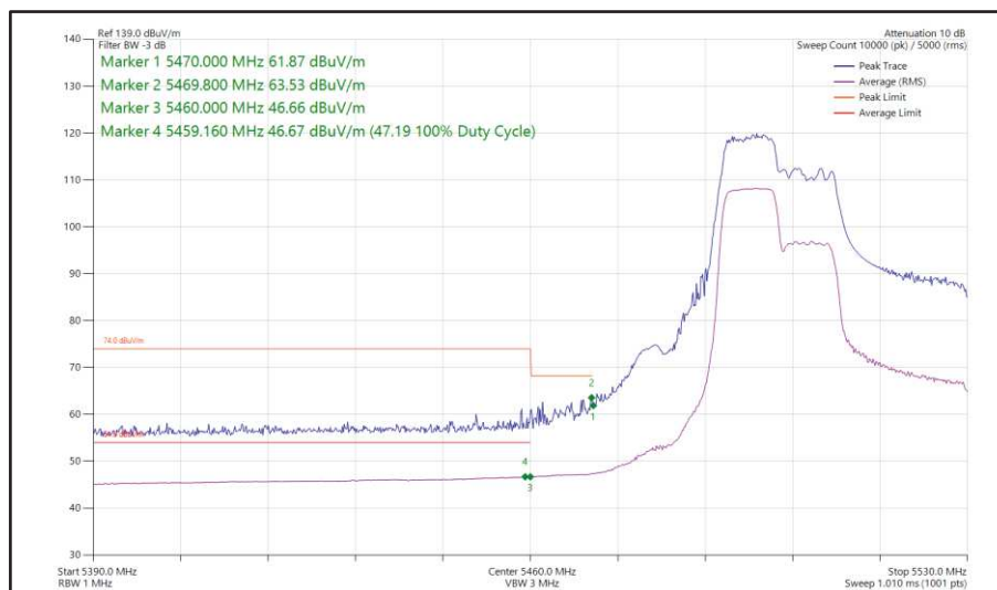
Figure 461 - 802.11ax HE40, RU 106-53, SISO, Core 1 - 5510 MHz Band Edge Frequency 5470 MHz
