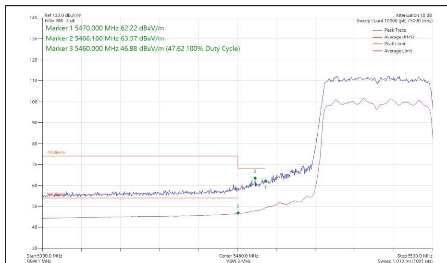
Figure 498 - 802.11ax HE40, SU, SDM, Core 0 + Core 1 - 5510 MHz Band Edge Frequency 5470 MHz
