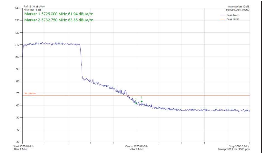
Figure 544 - 802.11ax HE80, SU, SISO, Core 1 - 5610 MHz Band Edge Frequency 5725 MHz
