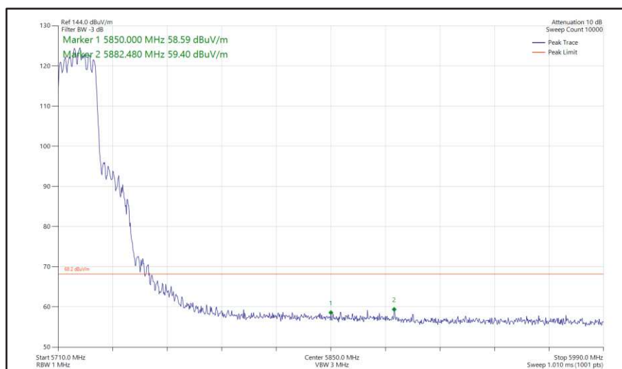
Figure 402 - 802.11ax HE20, SU, CDD, Core 0 + Core 1 - 5720 MHz Band Edge Frequency 5850 MHz
