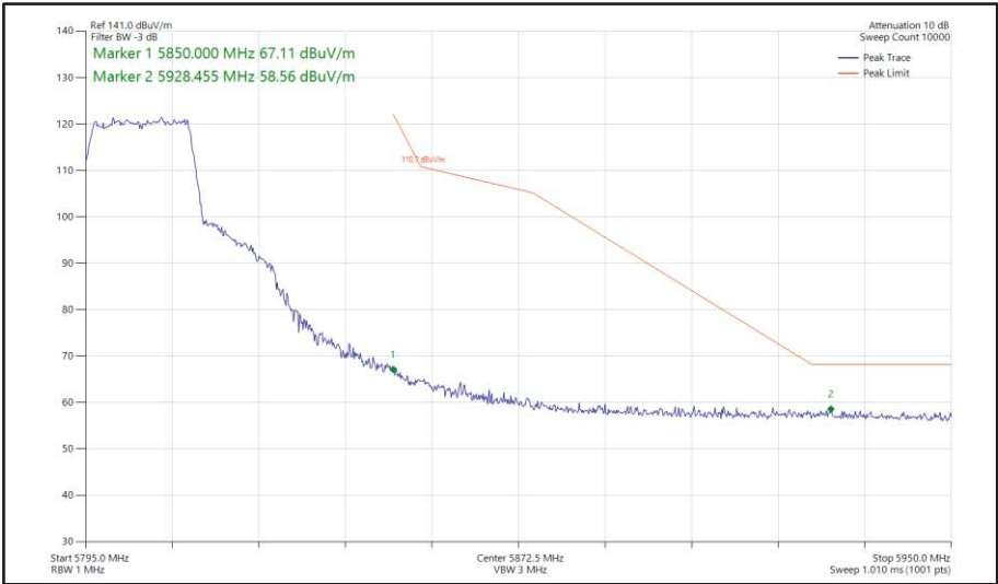
Figure 423 - 802.11n HT20, SDM, Core 0 + Core 1 - 5805 MHz Band Edge Frequency 5850 MHz
