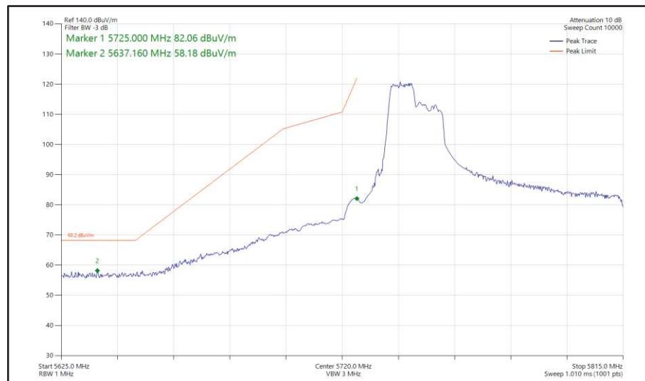
Figure 542 - 802.11ax HE80, RU 106-53, SISO, Core 1 - 5775 MHz Band Edge Frequency 5725 MHz
