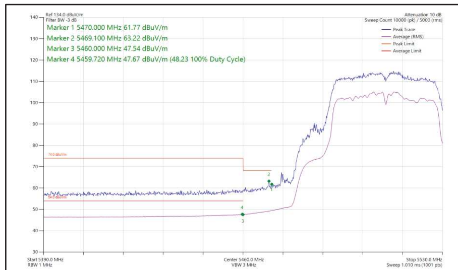
Figure 515 - 802.11ac VHT40, TxBF, Core 0 + Core 1 - 5510 MHz Band Edge Frequency 5470 MHz
