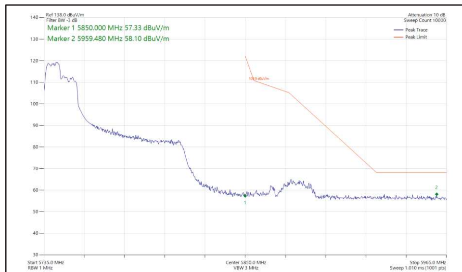
Figure 536 - 802.11ax HE80, RU 106-53, SISO, Core 0 - 5775 MHz Band Edge Frequency 5850 MHz
