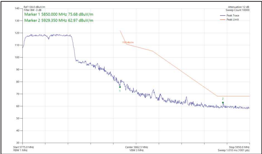
Figure 521 - 802.11ac VHT40, TxBF, Core 0 + Core 1 - 5795 MHz Band Edge Frequency 5850 MHz
