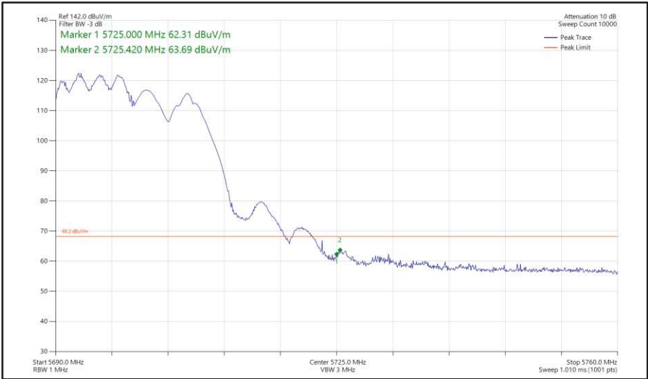
Figure 421 - 802.11ax HE20, RU 106-53, SDM, Core 0 + Core 1 - 5700 MHz Band Edge Frequency 5725 MHz
