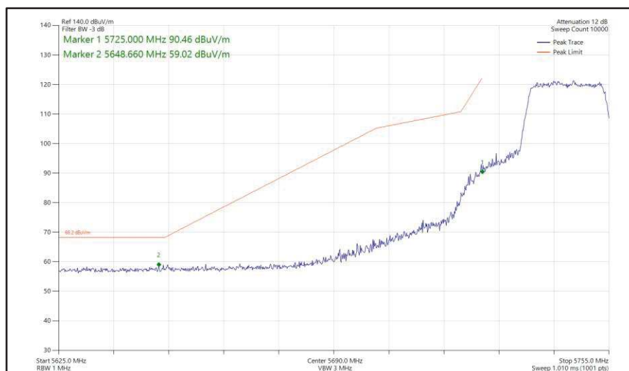
Figure 432 - 802.11ac VHT20, TxBF, Core 0 + Core 1 - 5745 MHz Band Edge Frequency 5725 MHz
