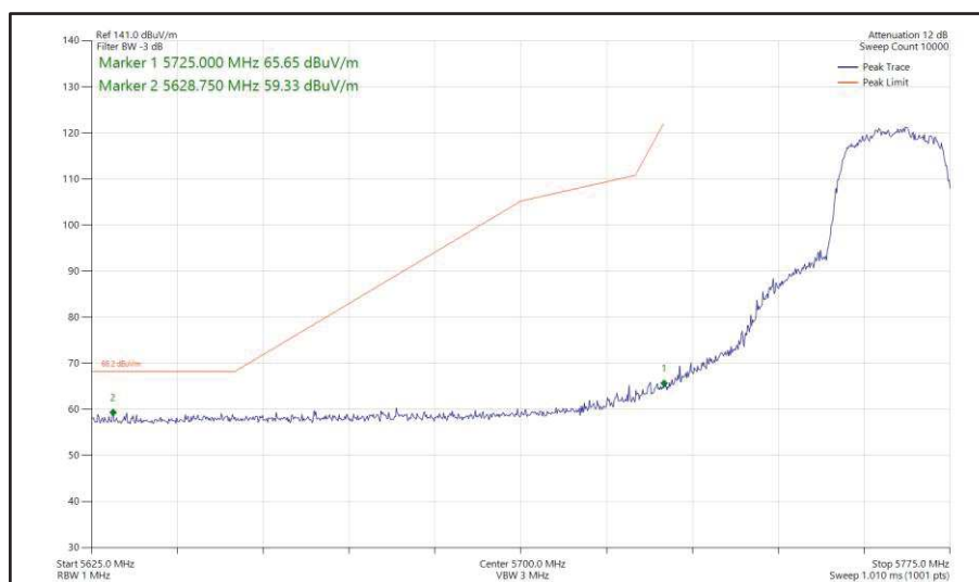
Figure 433 - 802.11ac VHT20, TxBF, Core 0 + Core 1 - 5765 MHz Band Edge Frequency 5725 MHz
