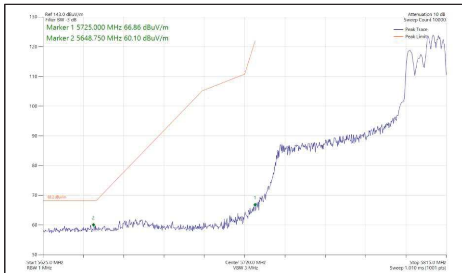
Figure 557 - 802.11ax HE80, RU 106-60, CDD, Core 0 + Core 1 - 5775 MHz Band Edge Frequency 5725 MHz
