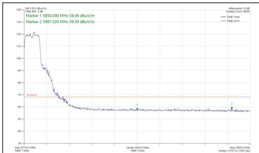
Figure 436 - 802.11ac VHT20, TxBF, Core 0 + Core 1 - 5720 MHz Band Edge Frequency 5850 MHz
