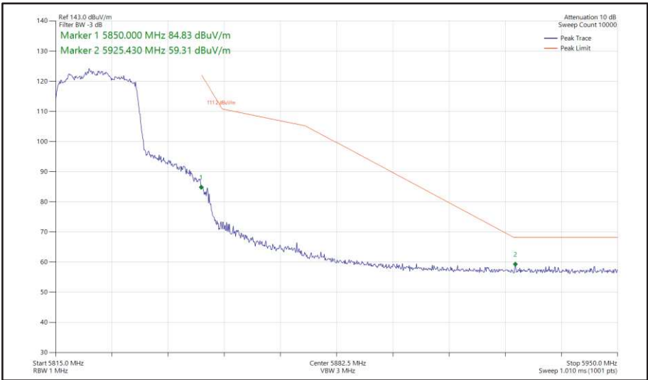
Figure 428 - 802.11ax HE20, SU, SDM, Core 0 + Core 1 - 5825 MHz Band Edge Frequency 5850 MHz
