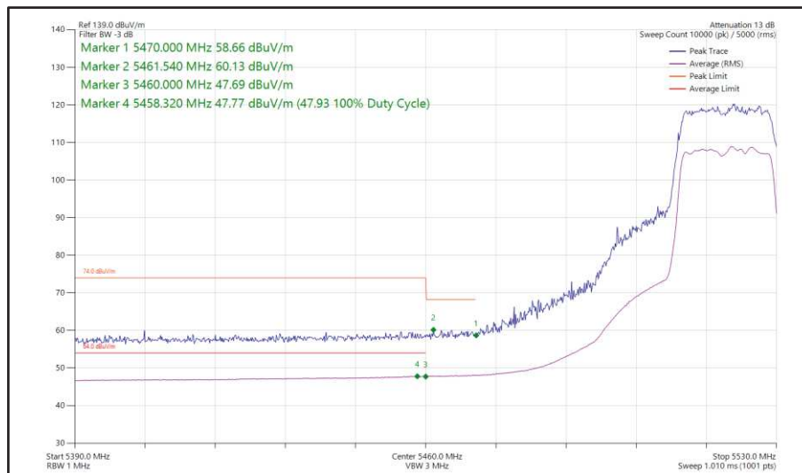
Figure 431 - 802.11ac VHT20, TxBF, Core 0 + Core 1 - 5520 MHz Band Edge Frequency 5470 MHz
