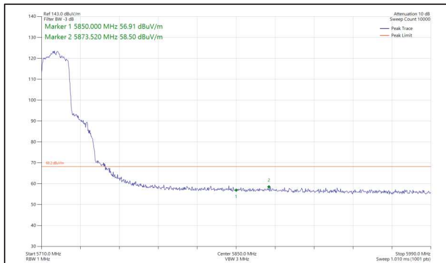
Figure 425 - 802.11ax HE20, SU, SDM, Core 0 + Core 1 - 5720 MHz Band Edge Frequency 5850 MHz
