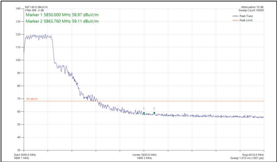
Figure 490 - 802.11n HT40, CDD, Core 0 + Core 1 - 5710 MHz Band Edge Frequency 5850 MHz
