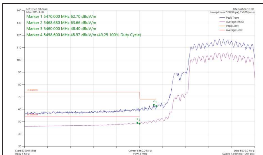
Figure 479 - 802.11ax HE40, SU, CDD, Core 0 + Core 1 - 5510 MHz Band Edge Frequency 5470 MHz
