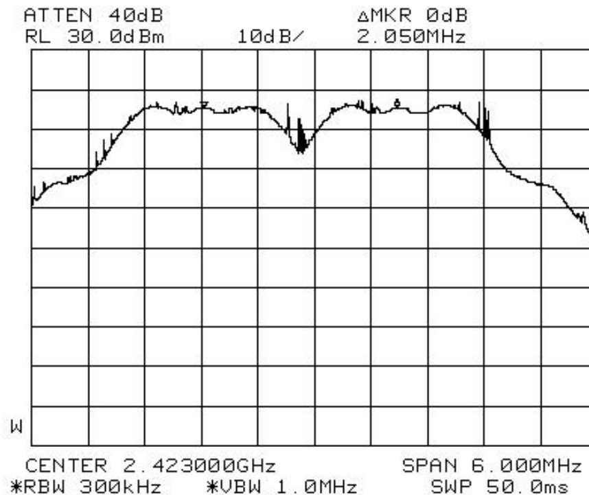
Plot 2 – Carrier Frequency Separation – Flat Speaker
