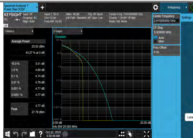
Band38-10MHz-16QAM-38200-50RB#0
