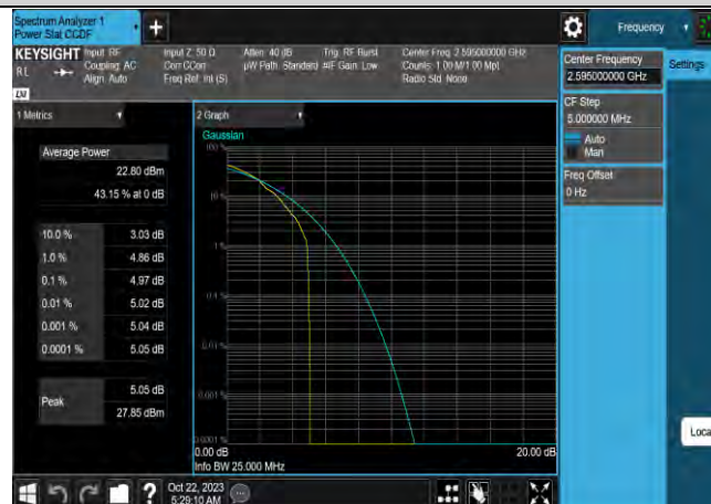
Band38-10MHz-16QAM-38000-50RB#0
