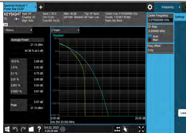
Band38-10MHz-16QAM-38000-1RB#0
