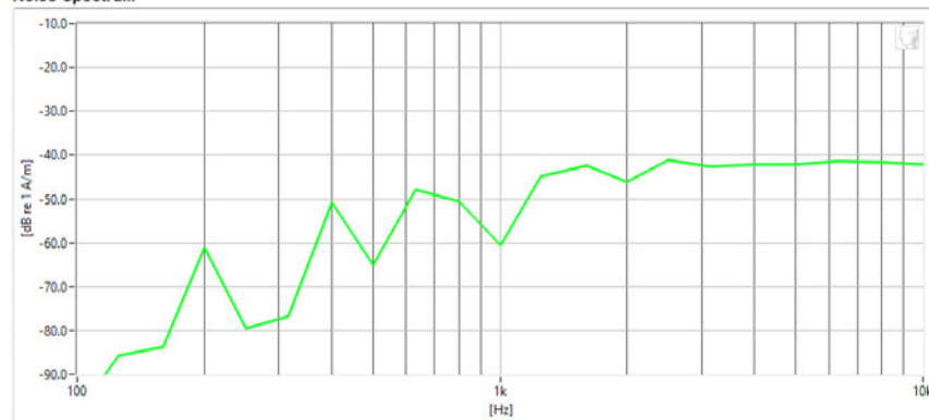
Noise Spectrum
