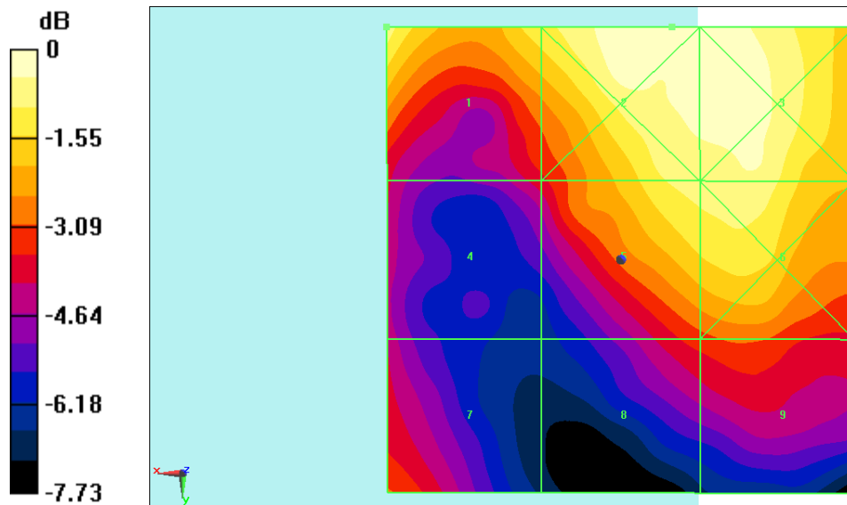
Fig B.4 HAC RF E-Field LTE Band41 PC3
