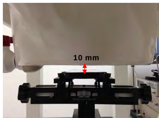
Fig.10 EUT front to flat phantom
