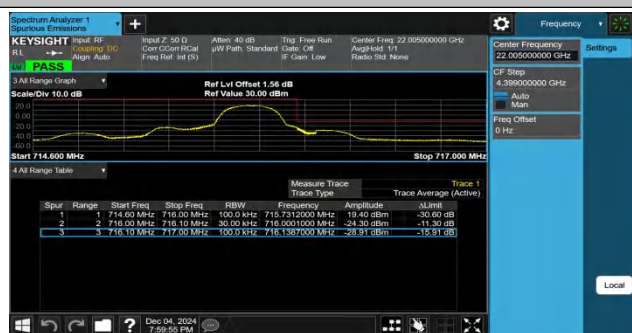
Band12-1.4MHz-QPSK-23173-1RB#5-PASS
