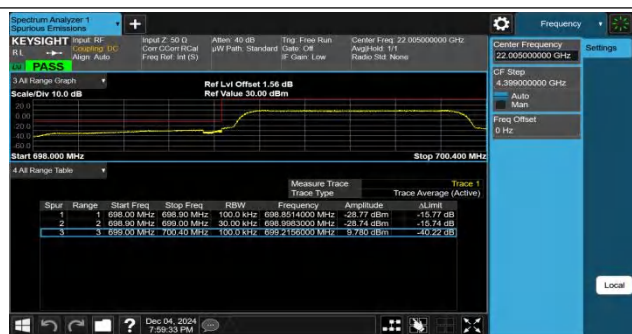
Band12-1.4MHz-QPSK-23017-6RB#0-PASS
