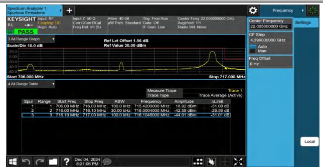
Band12-10MHz-QPSK-23130-1RB#49-PASS
