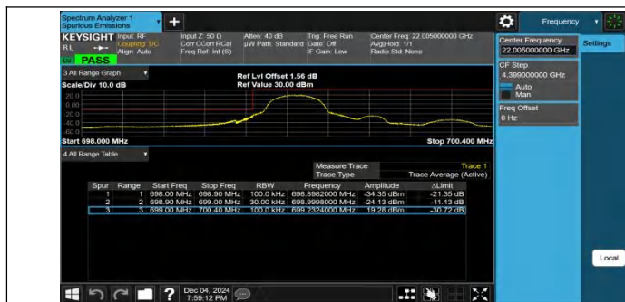
Band12-1.4MHz-QPSK-23017-1RB#0-PASS
