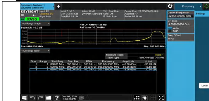
Band12-3MHz-QPSK-23025-1RB#14-PASS
