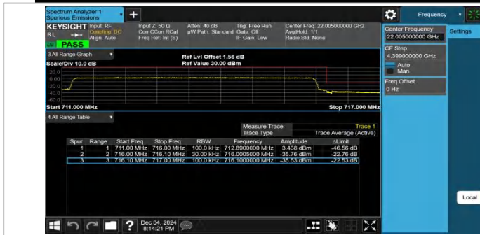
Band12-5MHz-QPSK-23155-25RB#0-PASS
