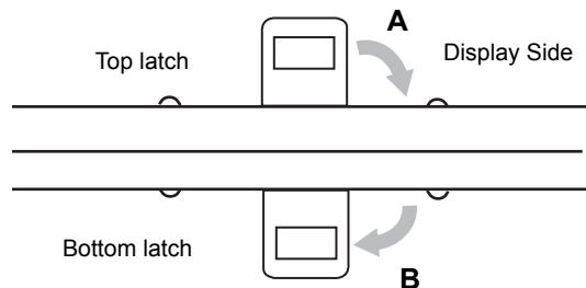
Figure 2-12. Latching/Unlatching
