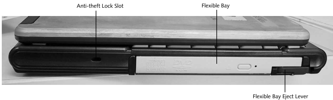
Figure 2-6. LifeBook T Series Tablet PC right-side panel
