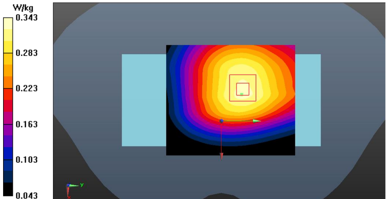
Fig.8 WCDMA Band 5 Body
