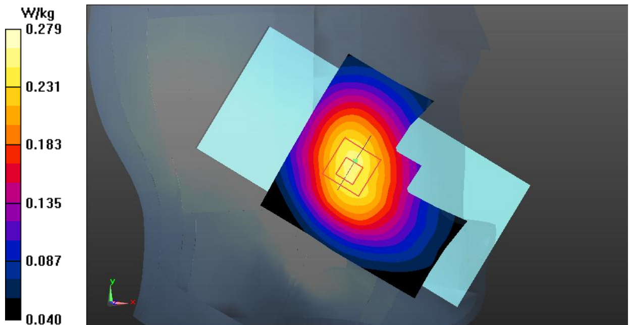
Fig.1 GSM 850 Head
