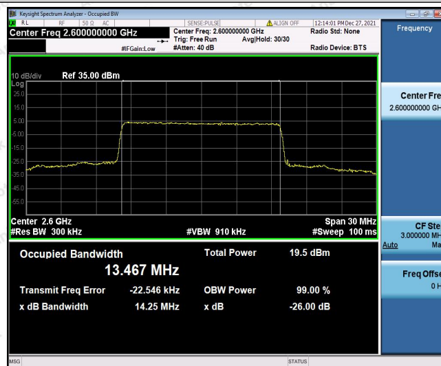
Band41-15MHz-16QAM-41065-75RB#0
