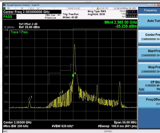
Band41-10MHz-QPSK-40390-1RB#49
