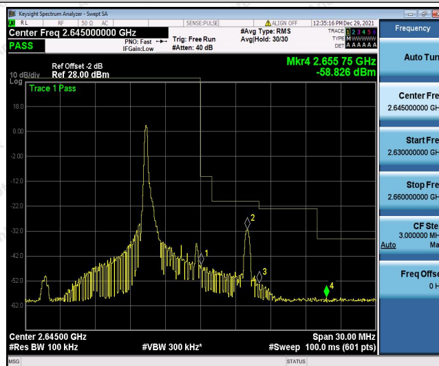
Band41-5MHz-QPSK-41115-1RB#24
