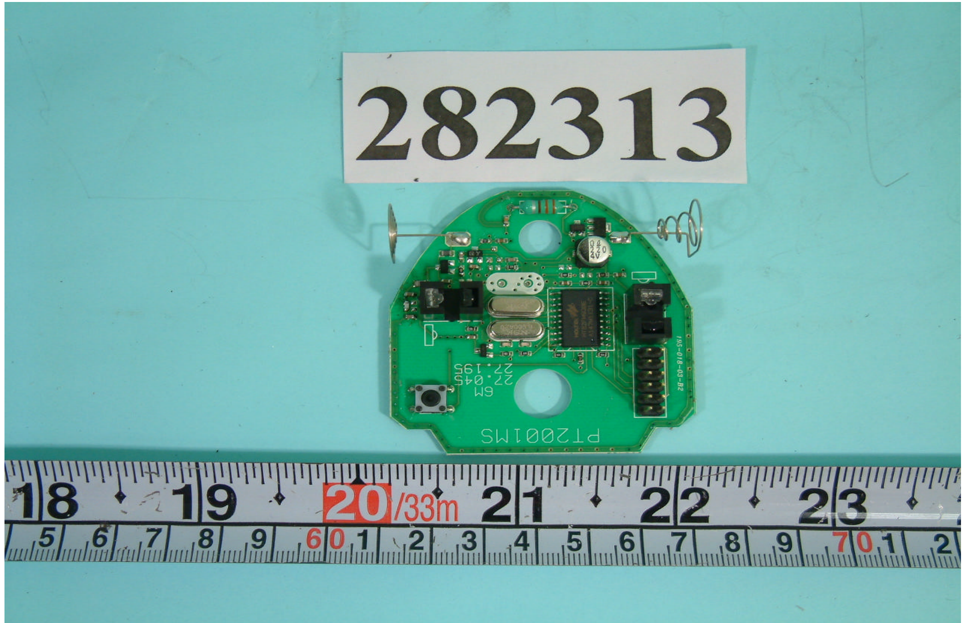
Front side of Main Board Of Mouse
