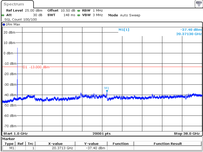
90MHz_30kHz_3745MHz_DFT-s-OFDM QPSK_RB1@244 -37.40 dBm
