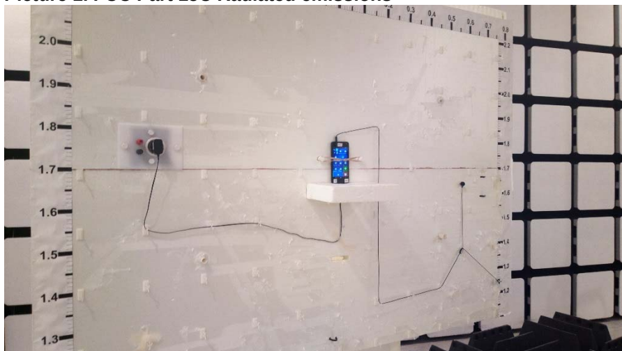
Picture 1. FCC Part 15C Radiated emissions
