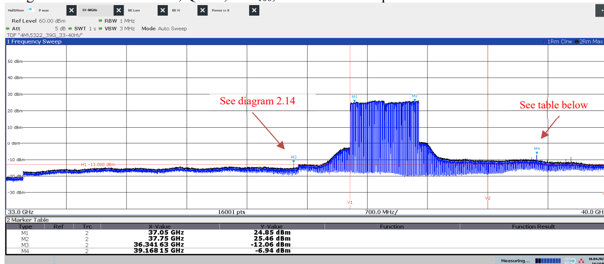
Diagram 2.17a: 33 – 40 GHz, QPSK, BL 8100 , EIRP Horizontal polarization
