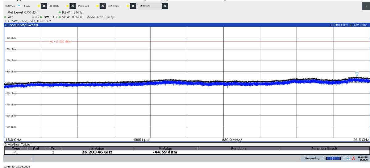
Diagram 2.7b: Pre scan 18 – 26.5 GHz, BL 50 , EIRP Vertical polarization
