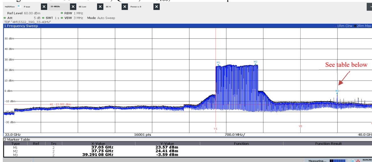
Diagram 2.17b: 33 – 40 GHz, QPSK, BL 8100 , EIRP Vertical polarization
