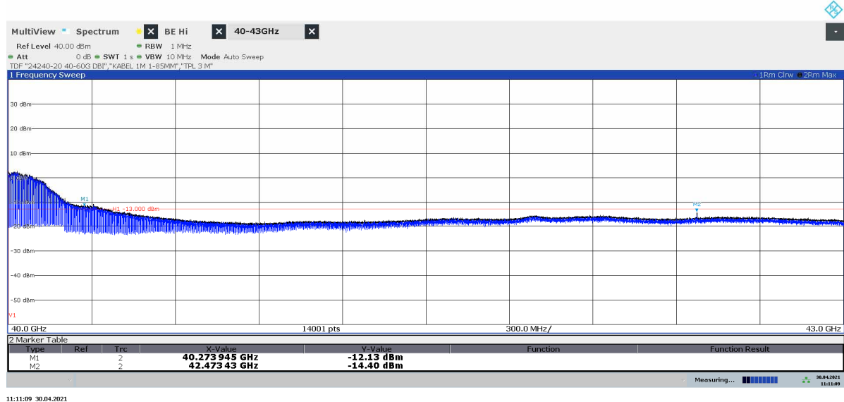
Diagram 2.22a: 40 – 43 GHz, QPSK, TH 8100 , EIRP Horizontal polarization
