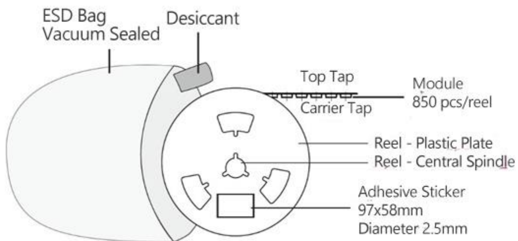
Fig 7 Packaging
