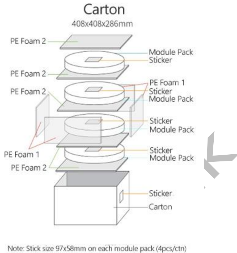
Fig 8 Carton
