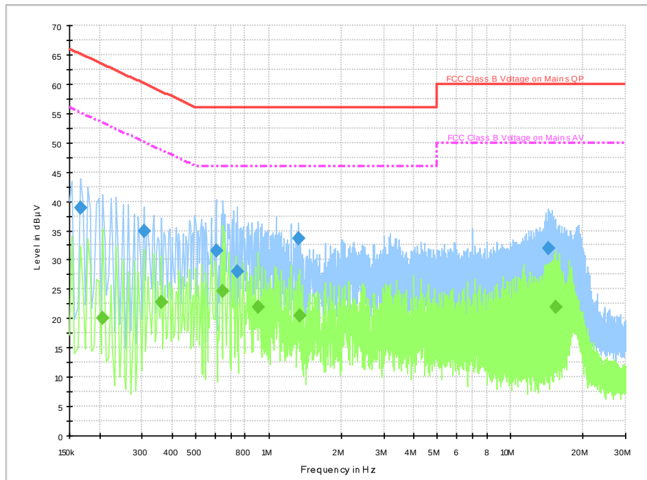
Fig.B.10.1 AC Powerline Conducted Emission-blueooth
