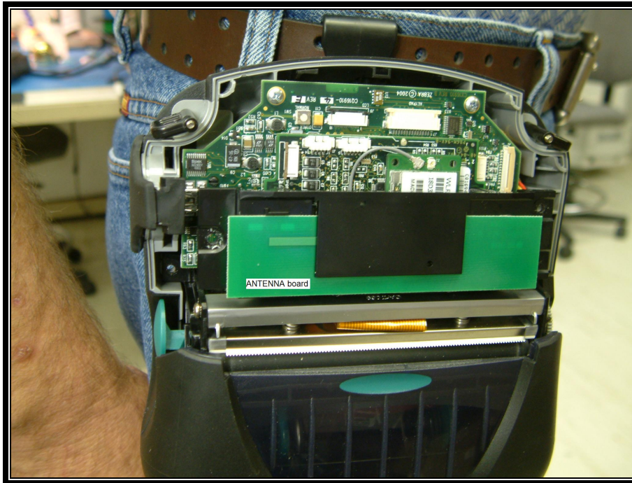
Photograph 5: Front view RW Antenna
