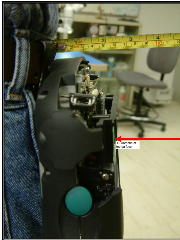
Photograph 6: RW420 side view showing separation distance between antenna and body
