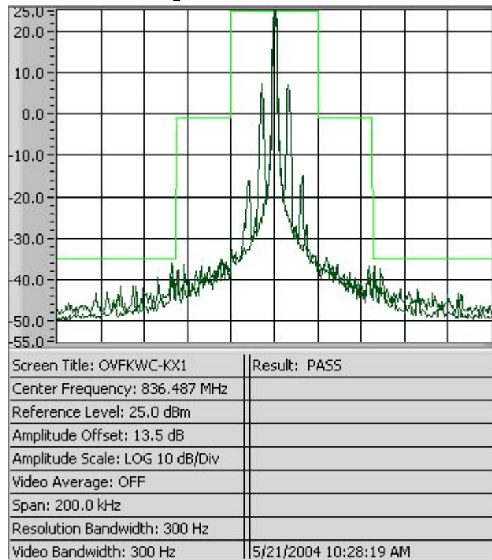
Figure 8-2 AMPS SAT
