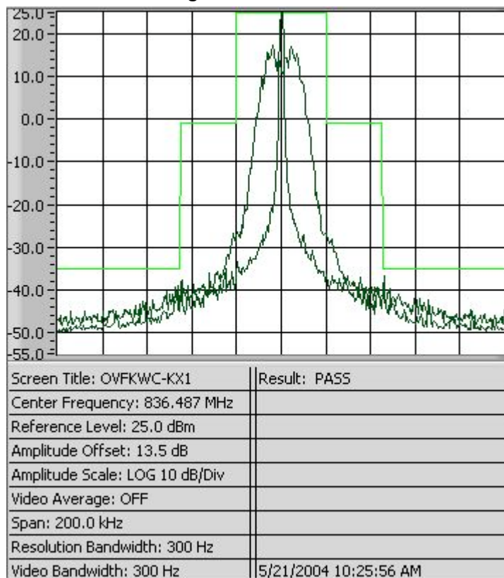
Figure 8-1 AMPS Voice
