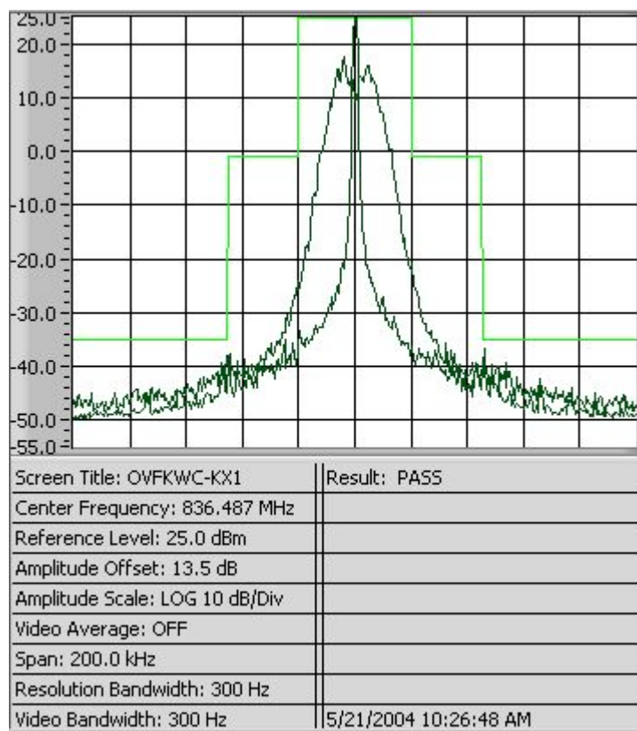
Figure 8-4 AMPS ST
