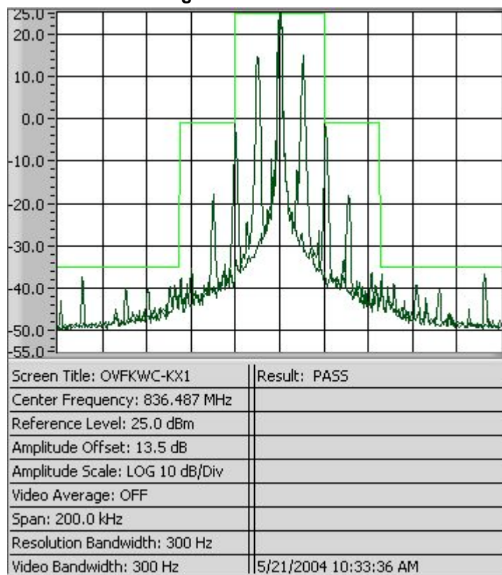
Figure 8-4 AMPS ST
