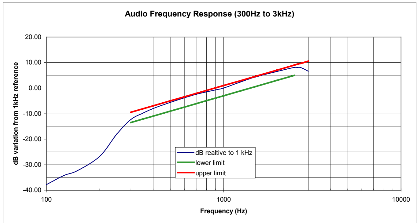
Figure 7.1 Audio Filter Characteristics (300-3000Hz)
