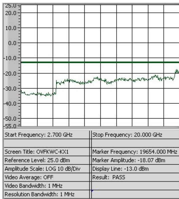
Figure 9-13b CDMA 1900 - Conducted Spurious Emission (CH 25)
