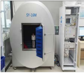
SY-16M Test System
