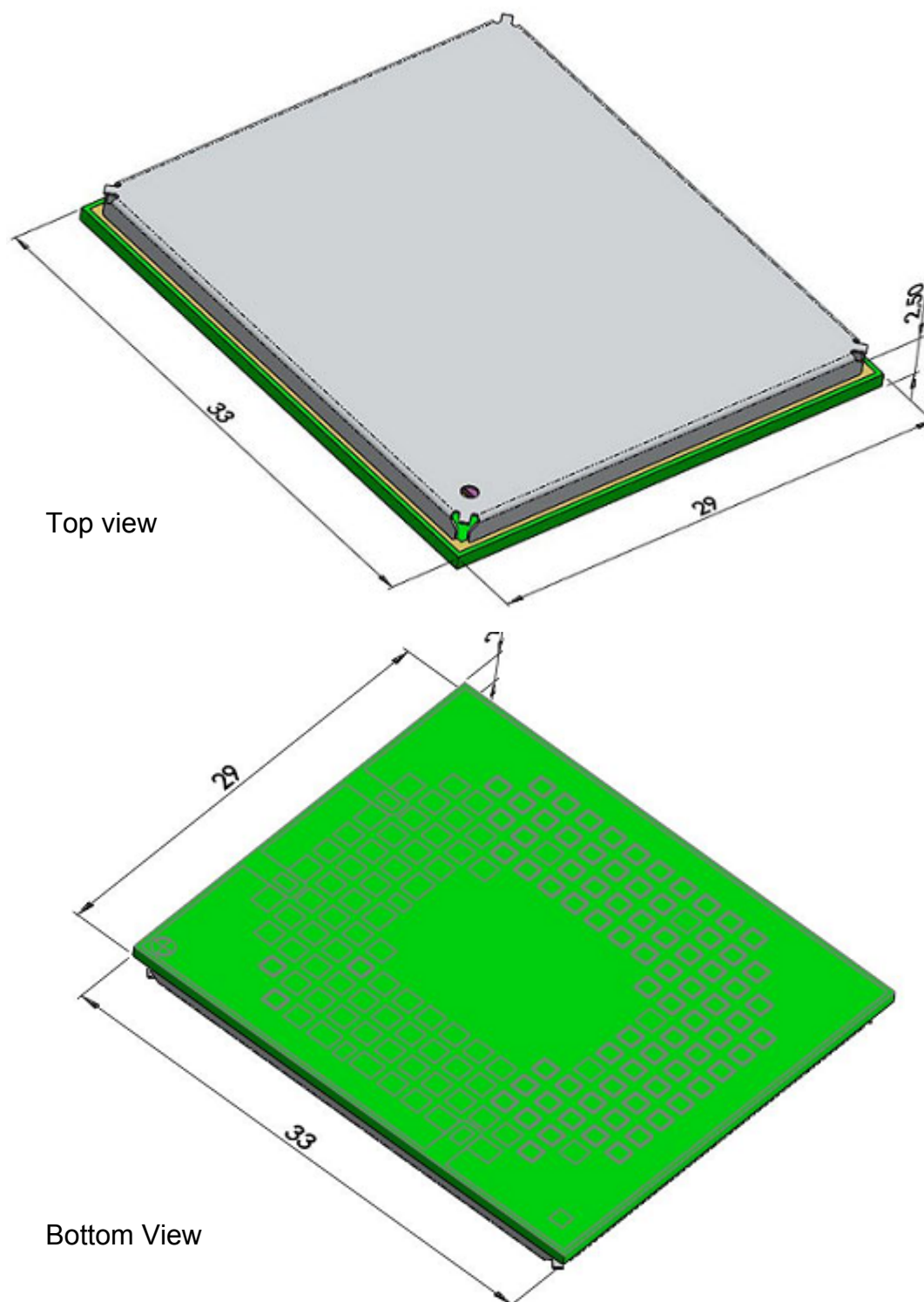
Figure 30: PLSx3– top and bottom view
