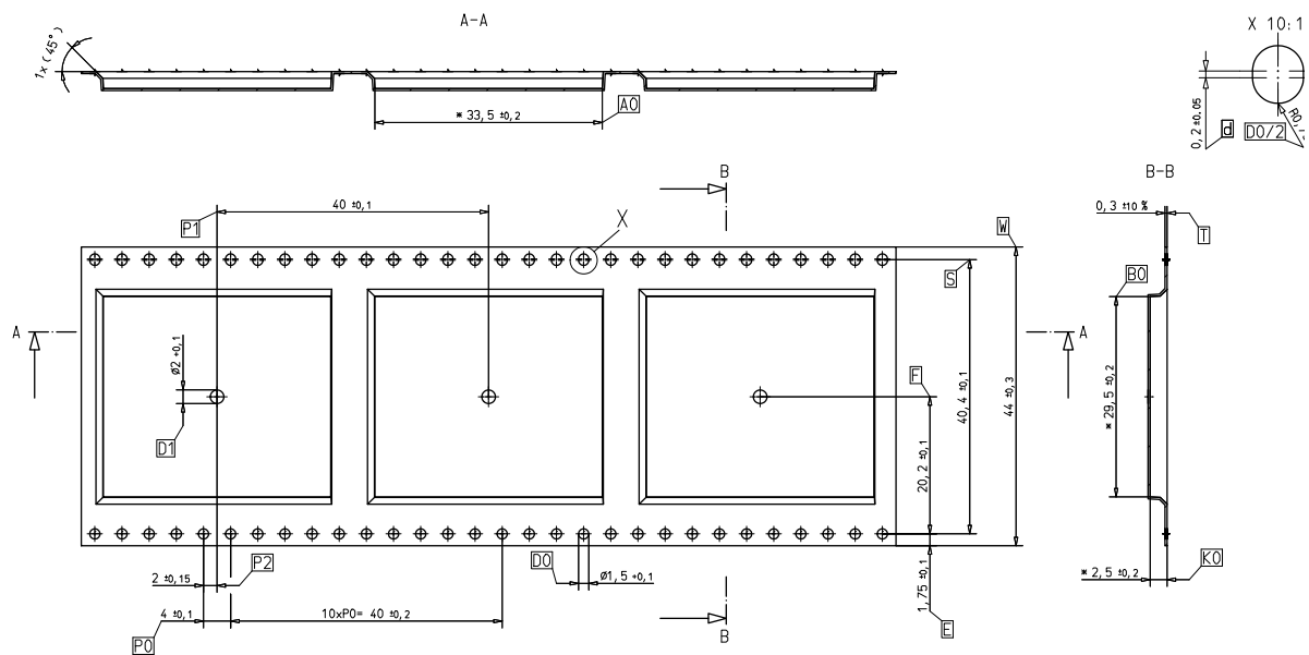
Figure 37: Carrier tape
