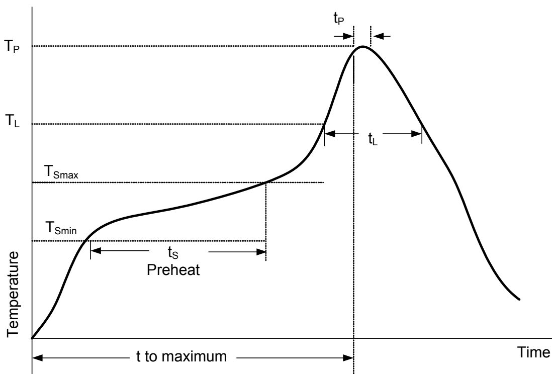
Figure 36: Reflow Profile
