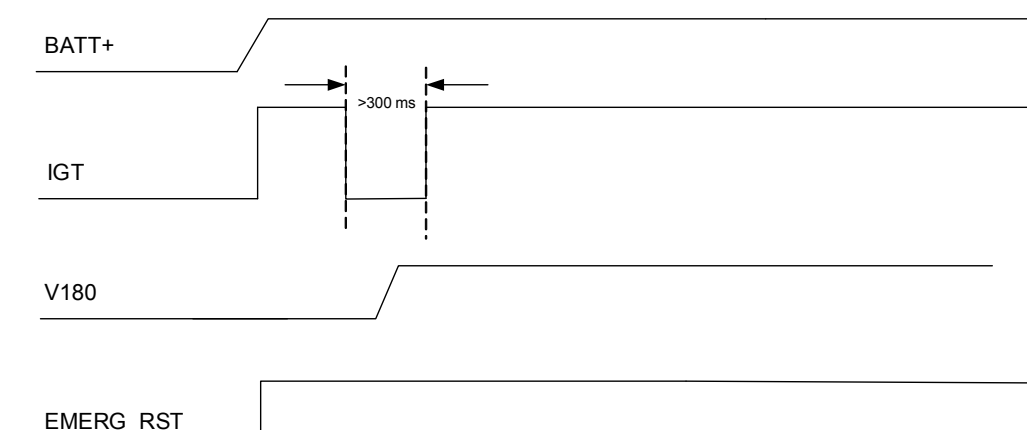
Figure 23: IGT timing
