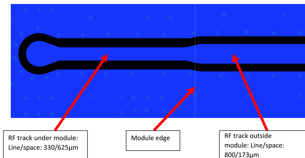
Figure 19: Routing Detail
