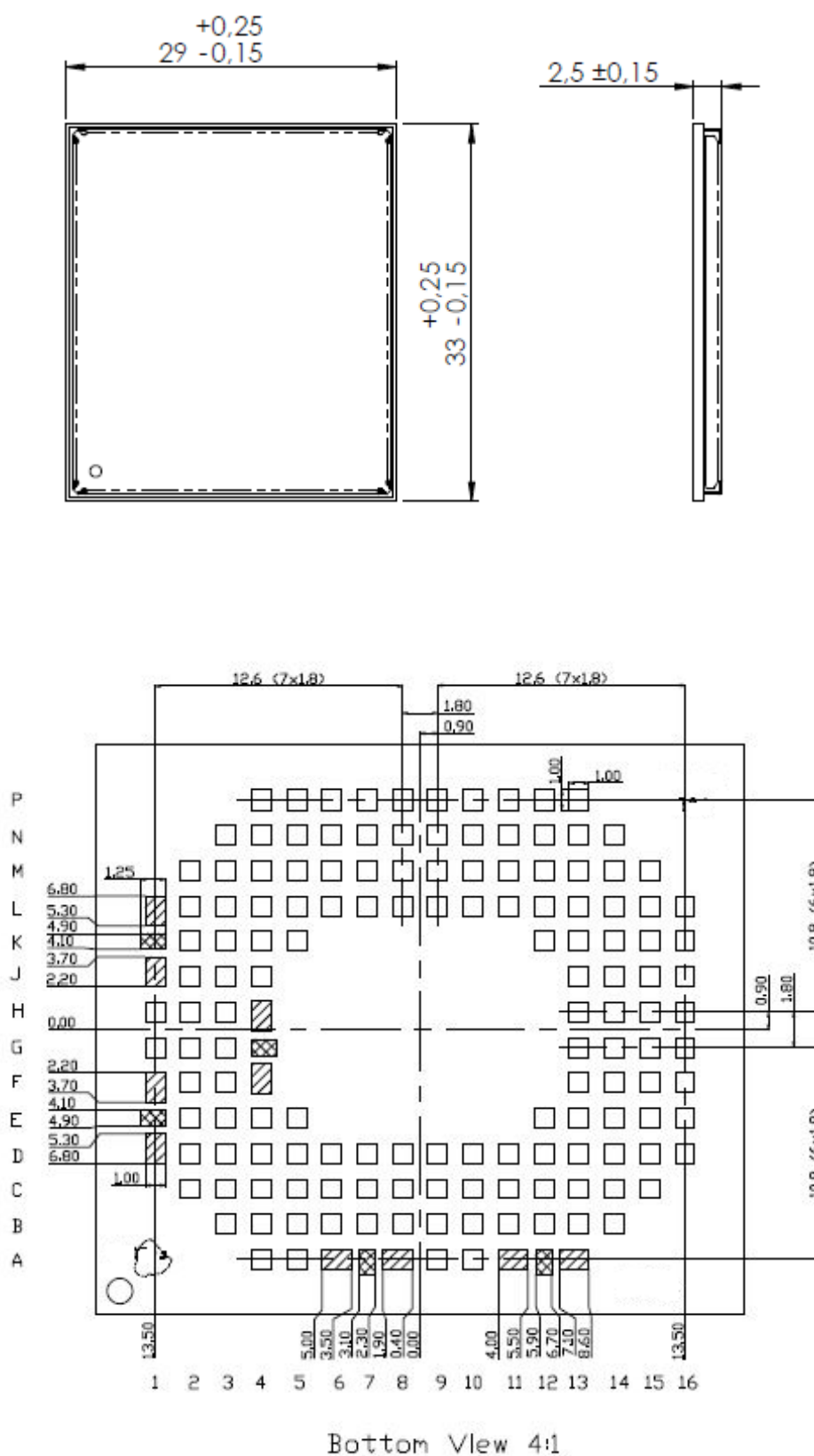
Figure 31: Dimensions of PLSx3 (all dimensions in mm)
