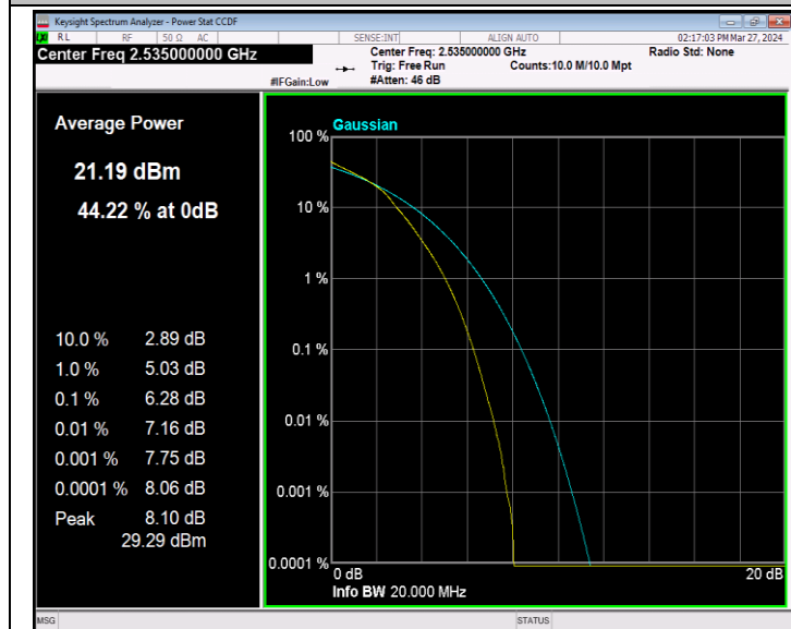
Band7-20MHz-16QAM-21100-100RB#0-PASS
