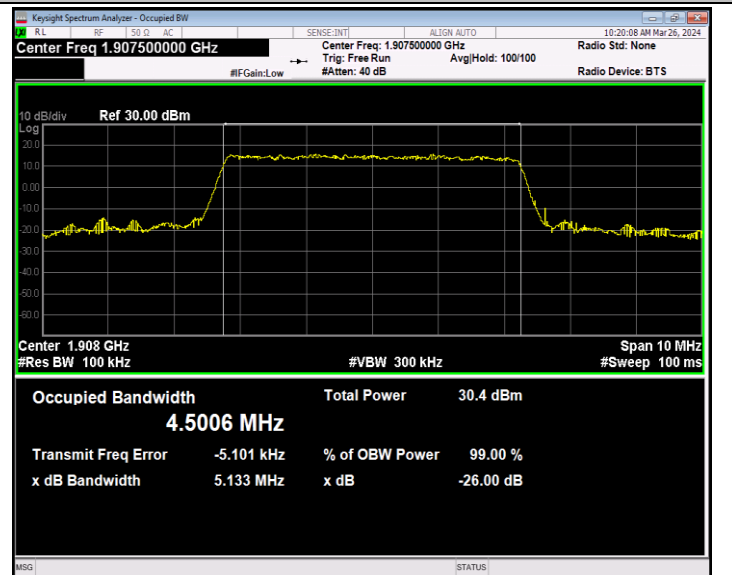
Band2-5MHz-16QAM-19175-25RB#0-PASS
