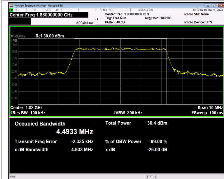
Band2-5MHz-16QAM-18900-25RB#0-PASS
