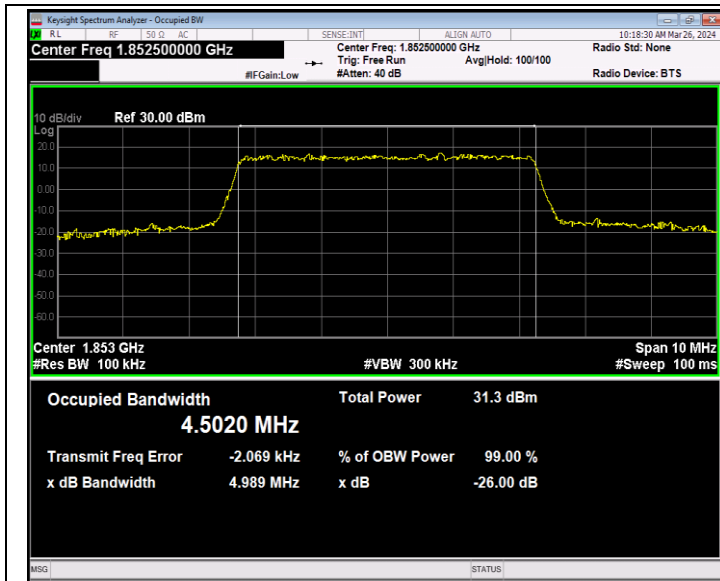
Band2-5MHz-64QAM-18625-25RB#0-PASS
