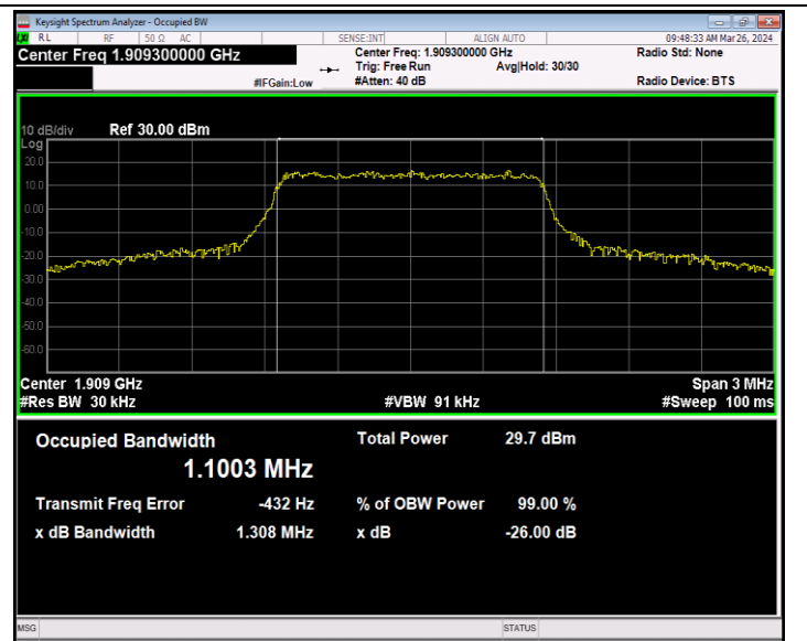
Band2-1.4MHz-16QAM-19193-6RB#0-PASS
