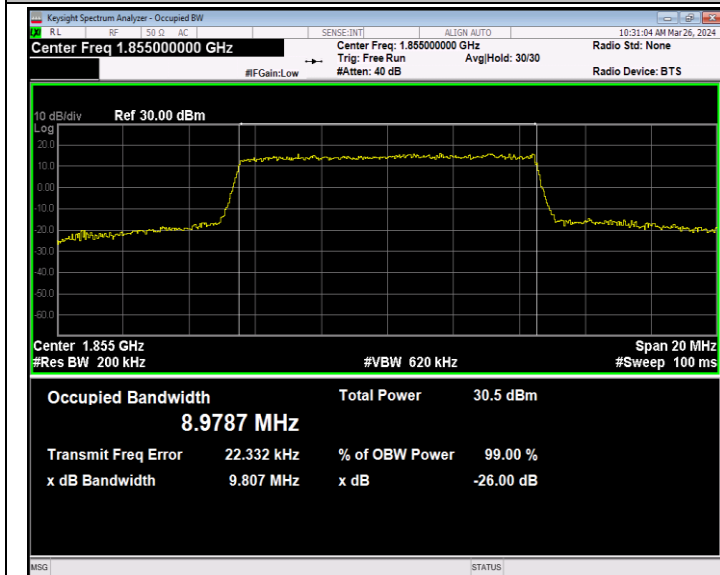
Band2-10MHz-16QAM-18650-50RB#0-PASS
