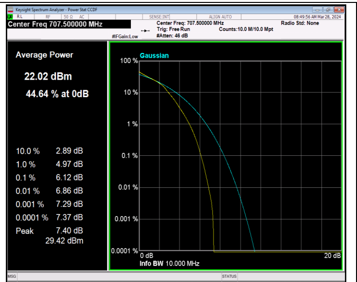
Band12-10MHz-16QAM-23095-50RB#0-PASS
