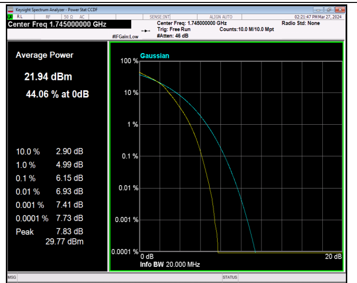
Band66-20MHz-16QAM-132322-100RB#0-PASS
