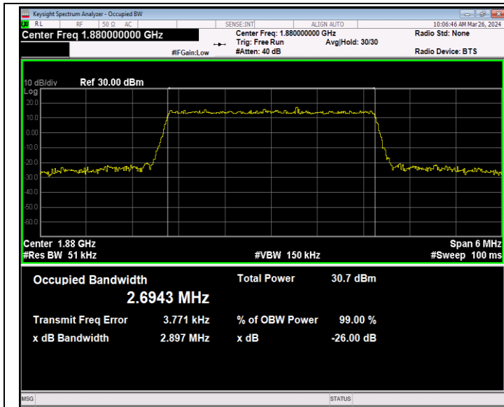
Band2-3MHz-64QAM-18900-15RB#0-PASS
