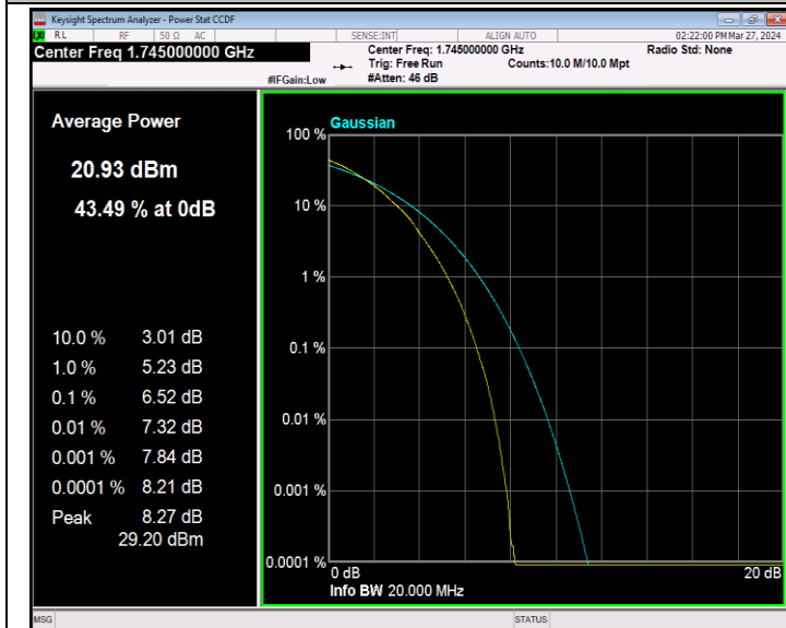
Band66-20MHz-64QAM-132322-100RB#0-PASS
