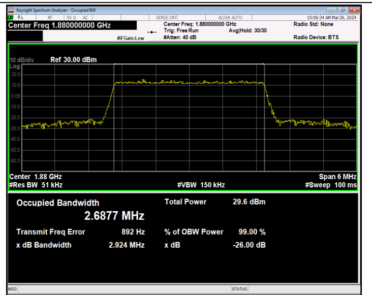
Band2-3MHz-16QAM-18900-15RB#0-PASS
