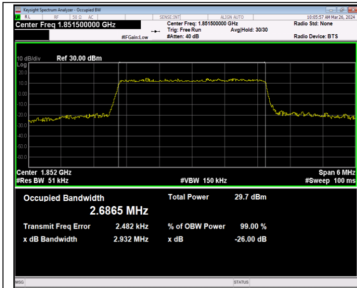
Band2-3MHz-16QAM-18615-15RB#0-PASS
