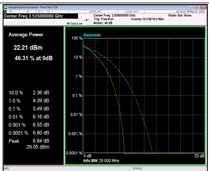
Band7-20MHz-QPSK-21100-100RB#0-PASS
