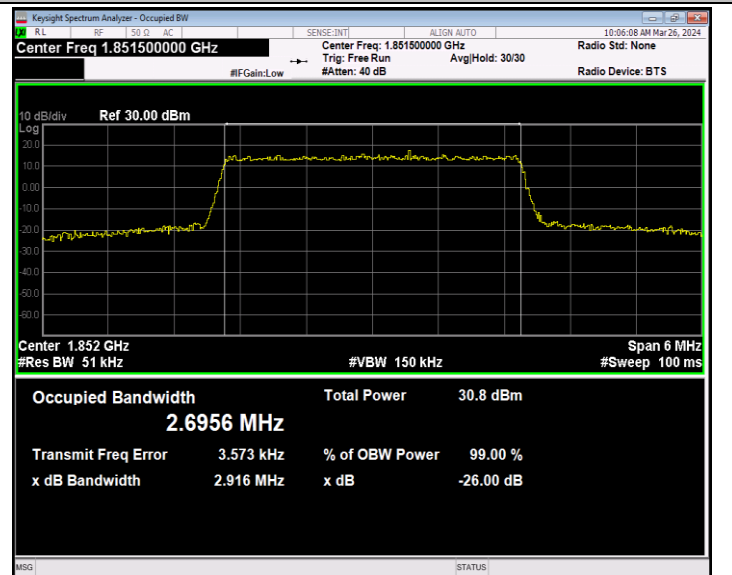
Band2-3MHz-64QAM-18615-15RB#0-PASS
