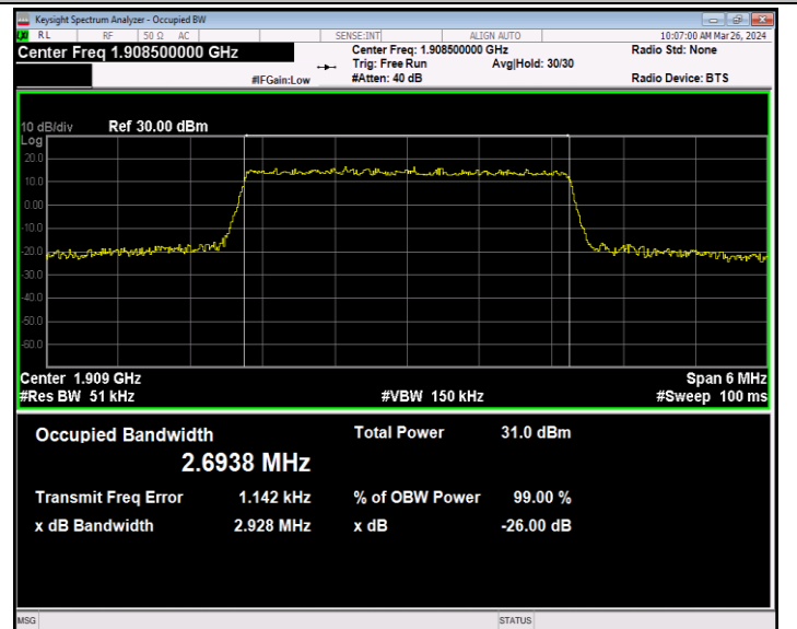
Band2-3MHz-QPSK-19185-15RB#0-PASS
