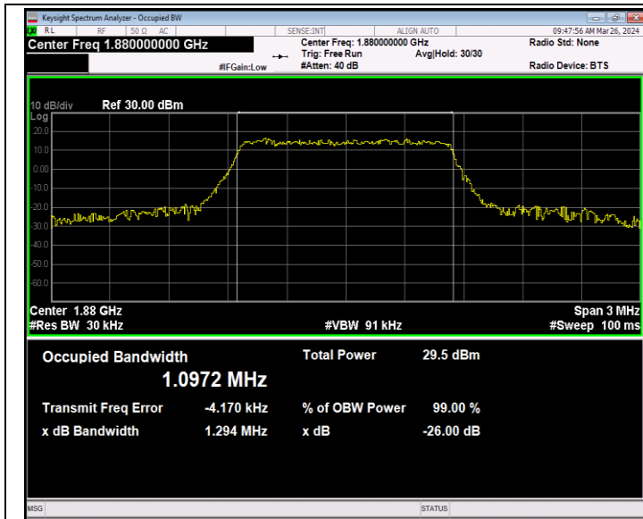
Band2-1.4MHz-16QAM-18900-6RB#0-PASS
