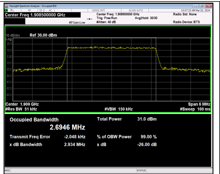
Band2-3MHz-64QAM-19185-15RB#0-PASS
