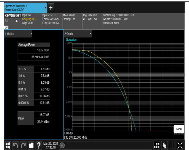
42(3450-3550)-20MHz-QPSK-42590-100RB#0-PASS
