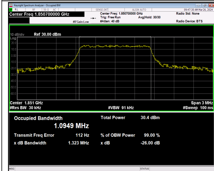
Band2-1.4MHz-64QAM-18607-6RB#0-PASS
