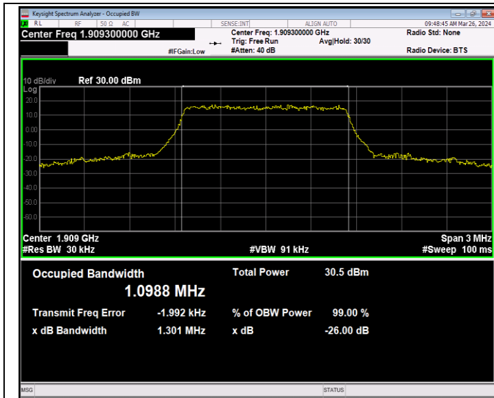
Band2-1.4MHz-64QAM-19193-6RB#0-PASS
