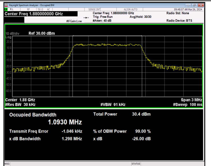
Band2-1.4MHz-64QAM-18900-6RB#0-PASS
