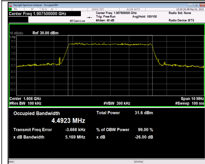
Band2-5MHz-64QAM-19175-25RB#0-PASS
