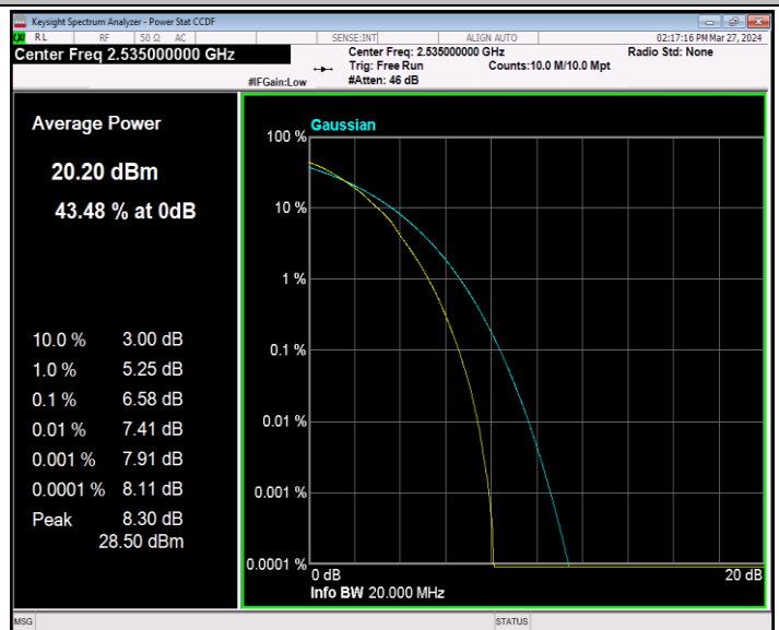
Band7-20MHz-64QAM-21100-100RB#0-PASS
