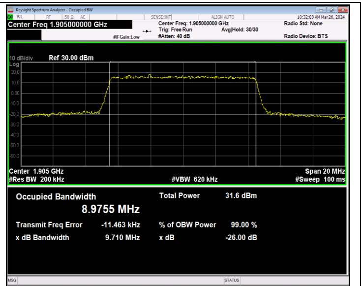
Band2-10MHz-QPSK-19150-50RB#0-PASS
