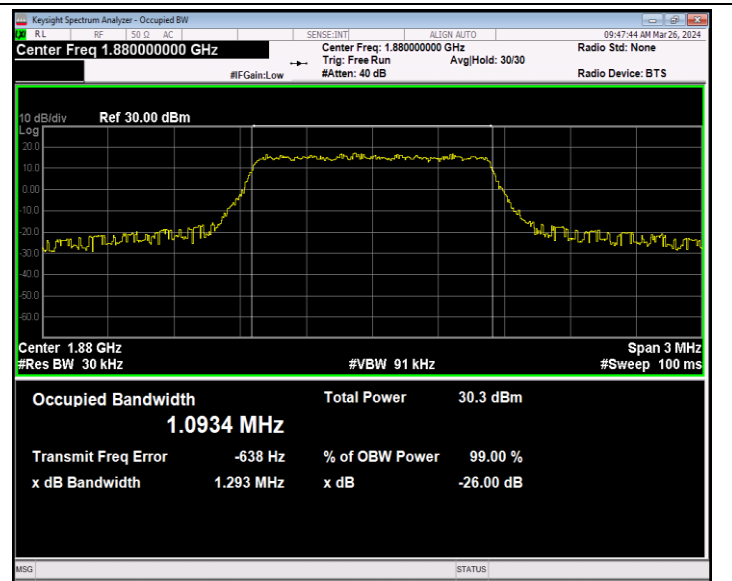
Band2-1.4MHz-QPSK-18900-6RB#0-PASS
