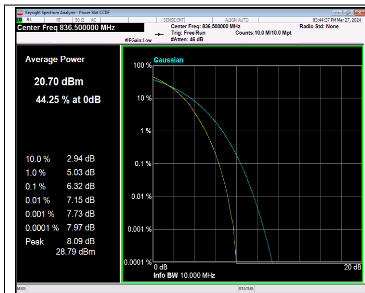
Band5-10MHz-64QAM-20525-50RB#0-PASS
