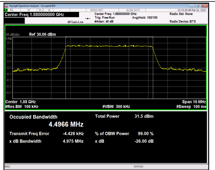
Band2-5MHz-64QAM-18900-25RB#0-PASS
