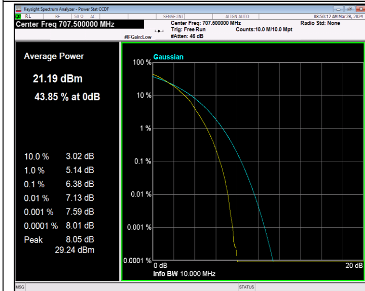
Band12-10MHz-64QAM-23095-50RB#0-PASS
