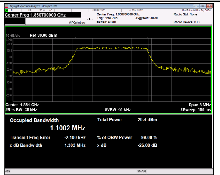
Band2-1.4MHz-16QAM-18607-6RB#0-PASS
