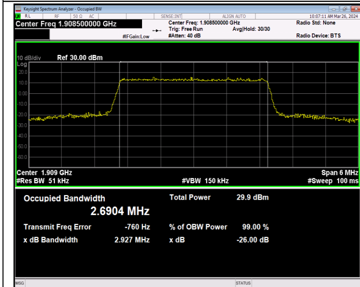
Band2-3MHz-16QAM-19185-15RB#0-PASS
