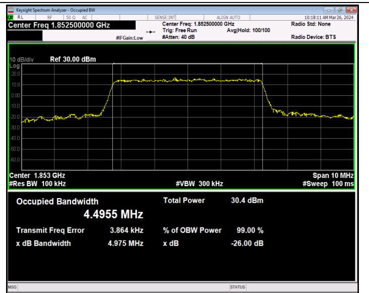
Band2-5MHz-16QAM-18625-25RB#0-PASS
