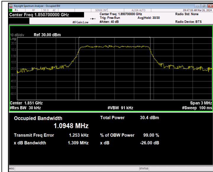
Band2-1.4MHz-QPSK-18607-6RB#0-PASS
