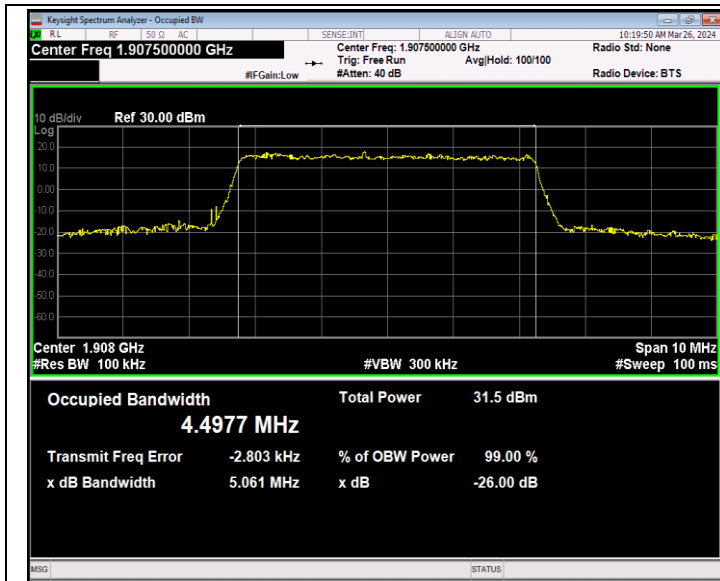
Band2-5MHz-QPSK-19175-25RB#0-PASS
