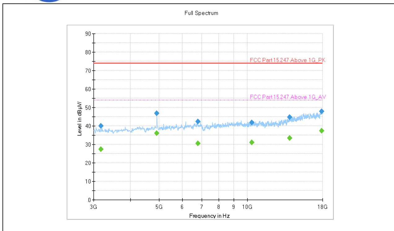
(802.11b _2462MHz, Antenna Horizontal, 3GHz to 18GHz)
