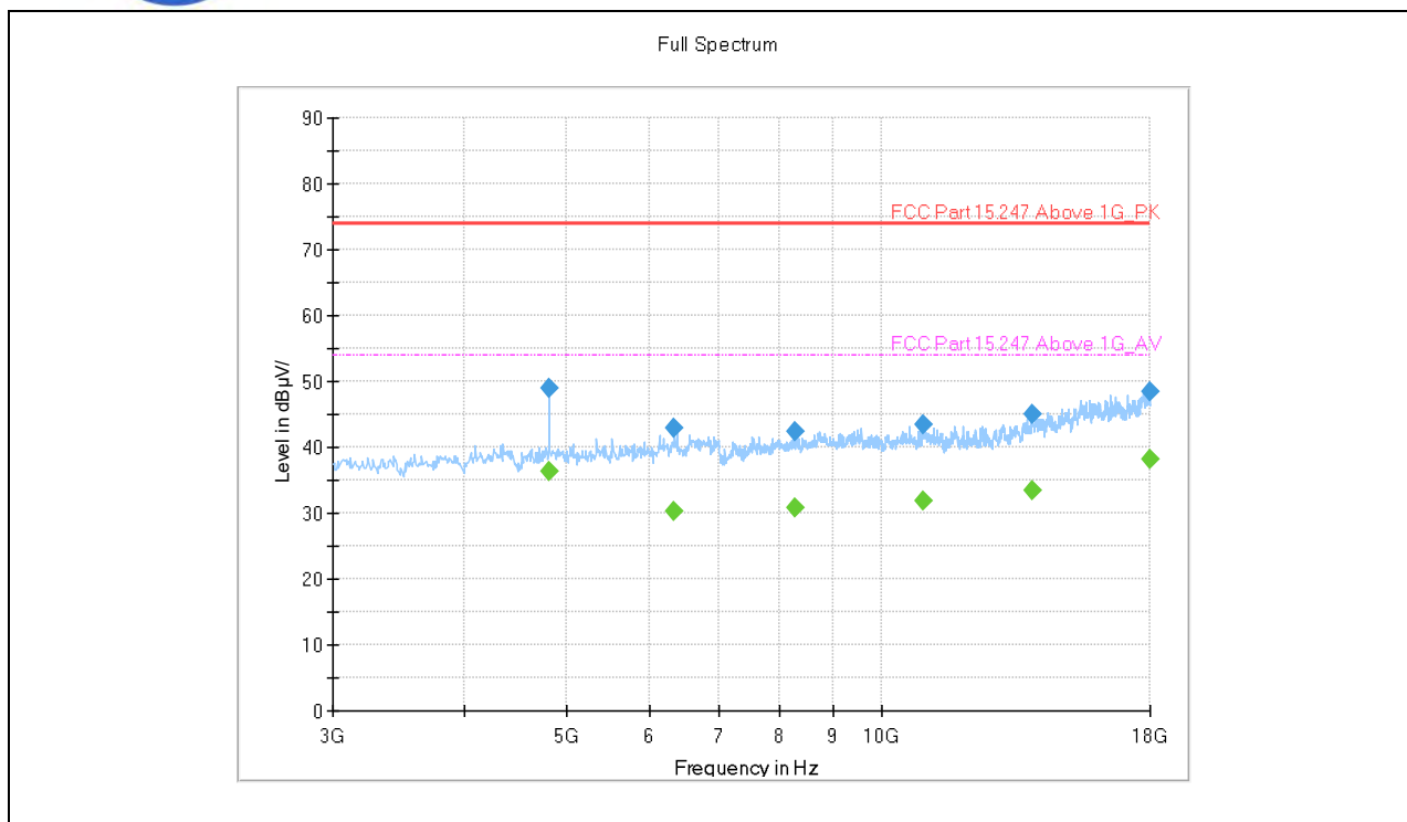
(802.11b _2412MHz, Antenna Horizontal, 3GHz to 18GHz)
