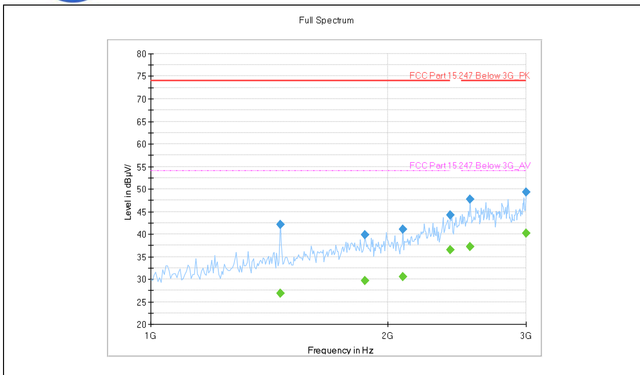
(802.11b _2412MHz, Antenna Vertical , 1GHz to 3GHz)
