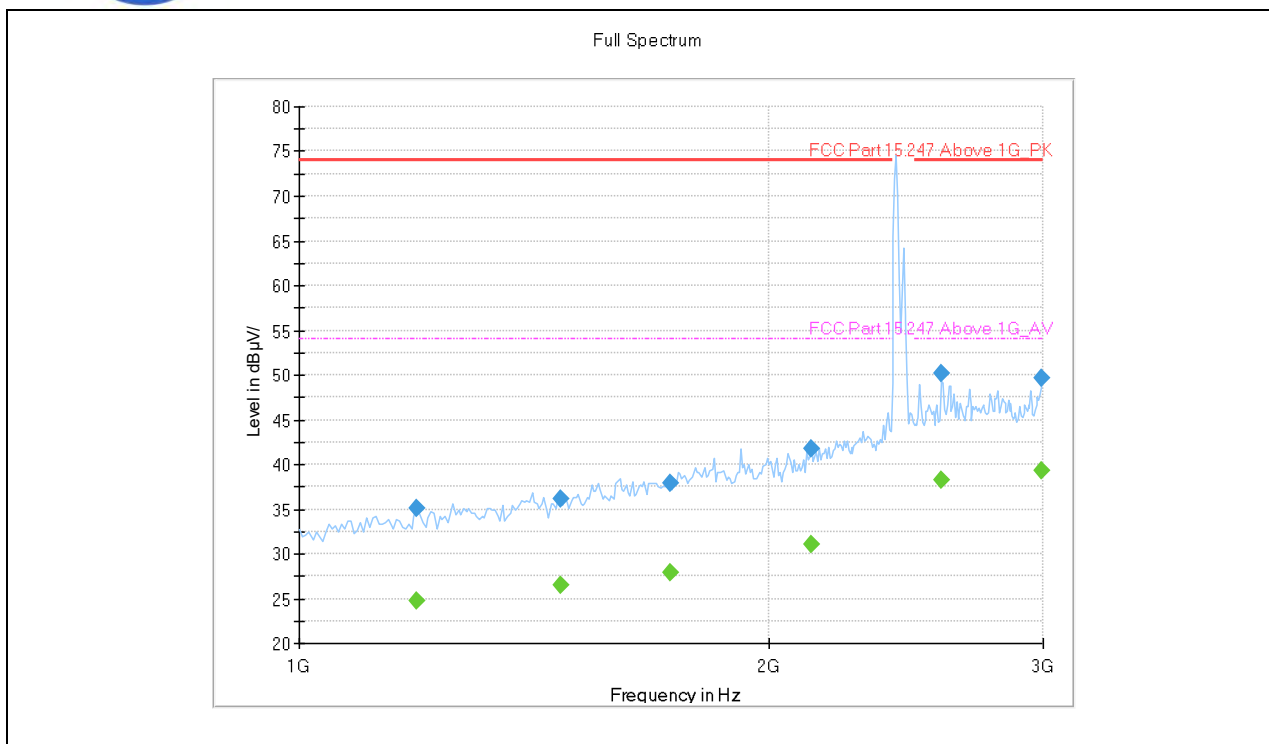
(802.11b _2437MHz, Antenna Horizontal, 1GHz to 3GHz)
