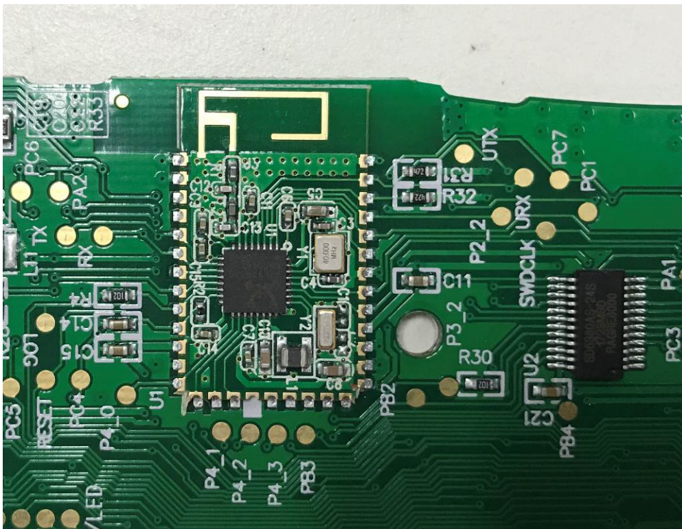
Internal View (Philips SRP2017B)
