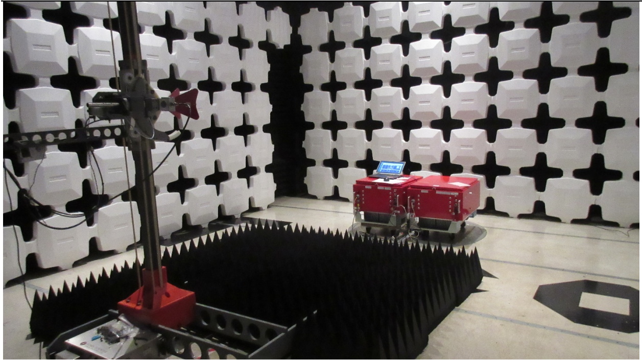
Testing, Above 1 GHz at 1.5m
