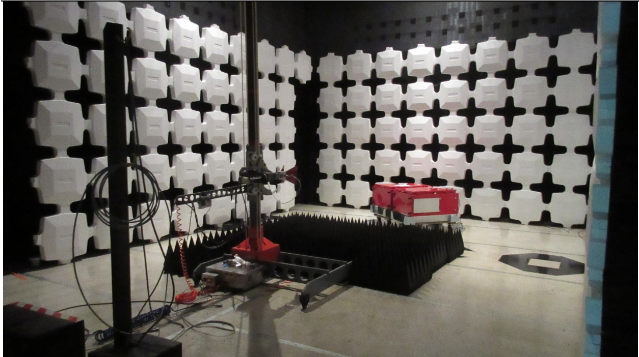
Testing, Above 1 GHz at 1m
