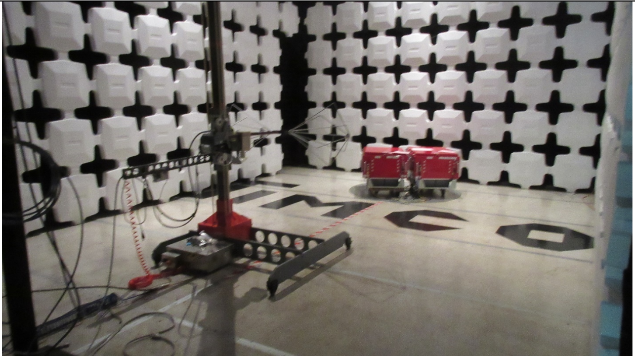
Radiated Testing, Below 1 GHz, #1
