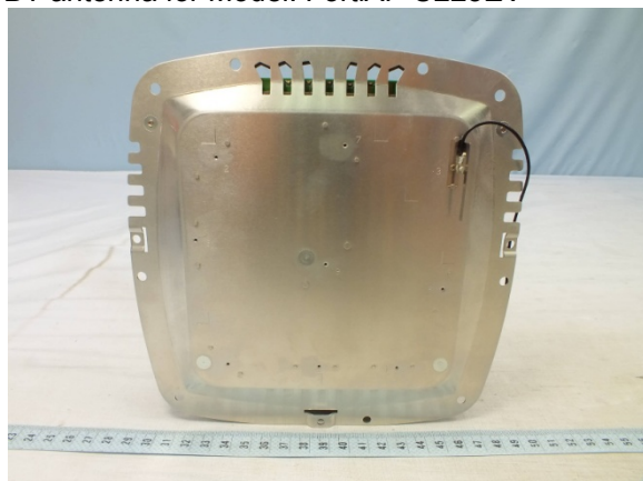
BT antenna for Model: FortiAP U223EV
