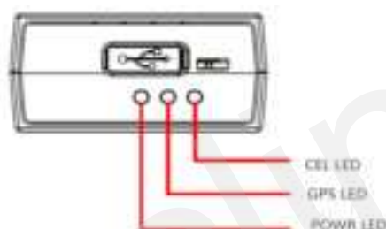
Figure 2. GV300LAU LEDs
