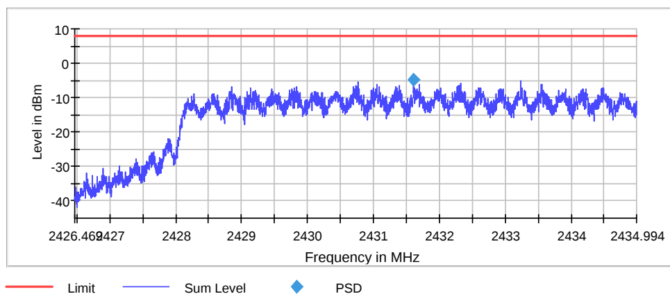
Peak Power Spectral Density 2nd
