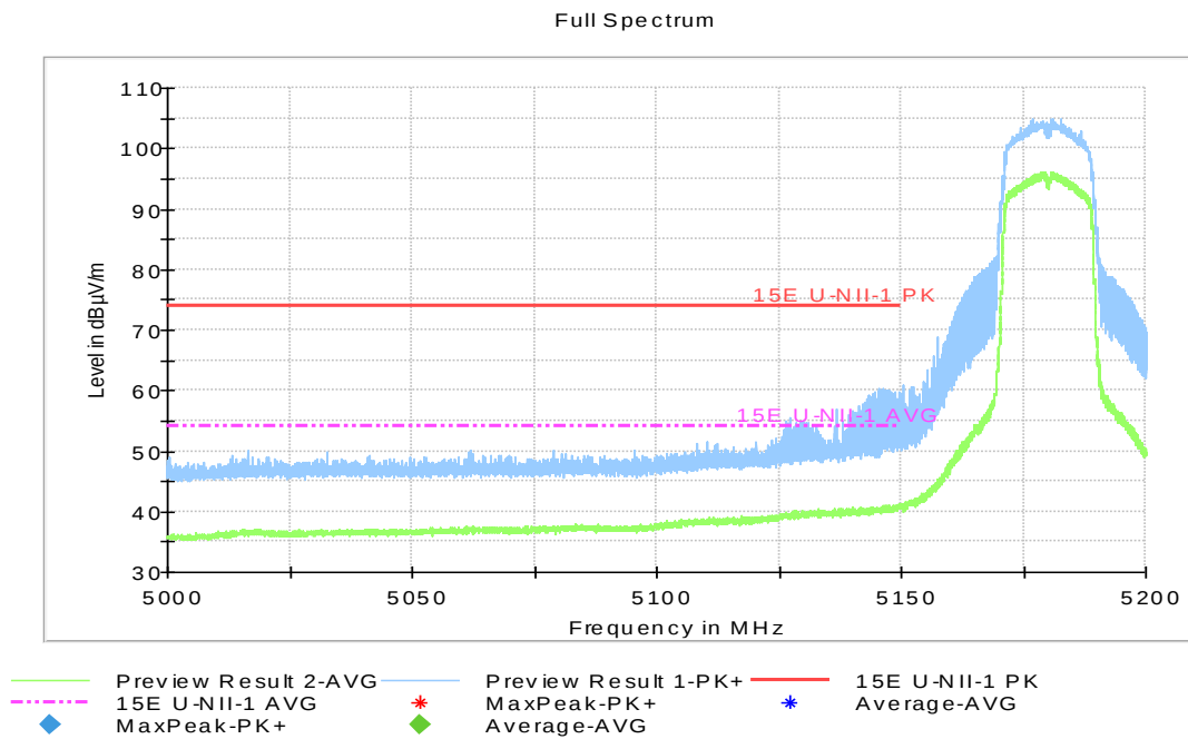
Fig.38 Band Edges (802.11n-HT20, 5180MHz)
