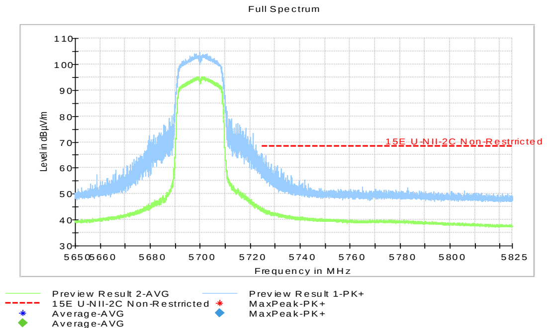
Fig.49 Band Edges (802.11ac-HT20, 5700MHz)
