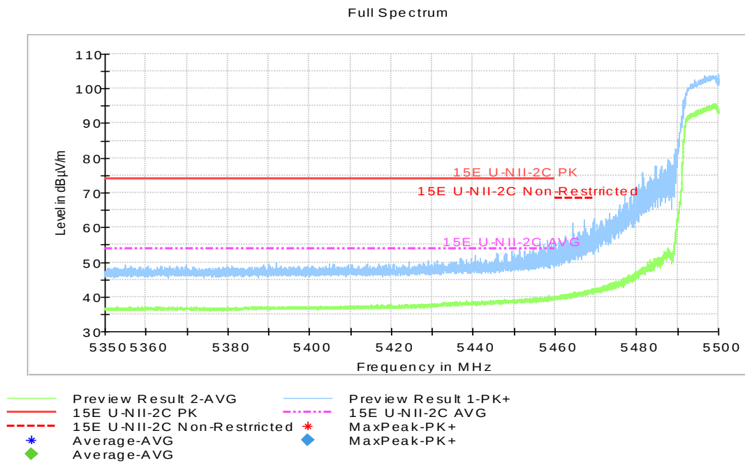
Fig.36 Band Edges (802.11a, 5500MHz)
