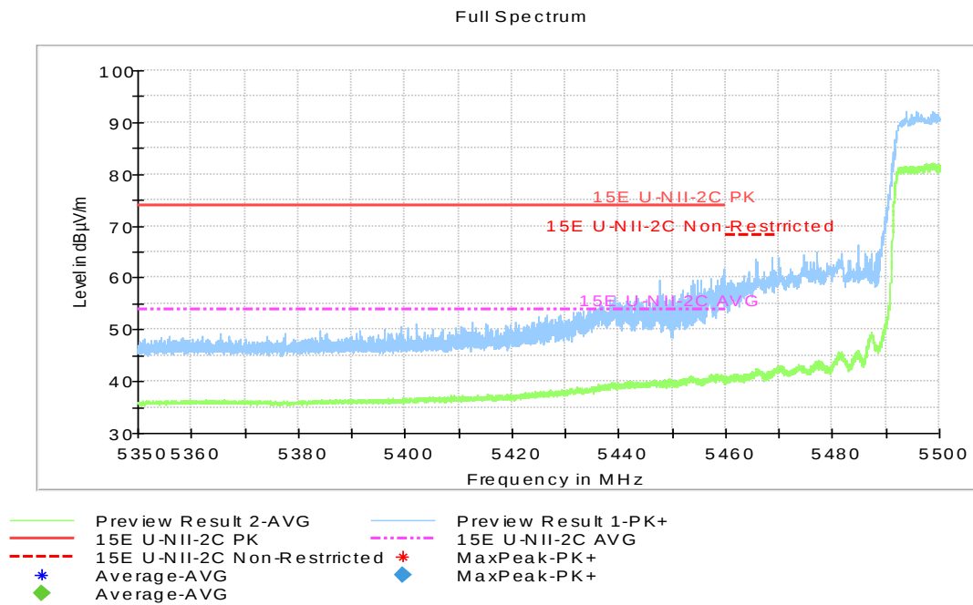
Fig.56 Band Edges (802.11ac-HT80, 5530MHz)
