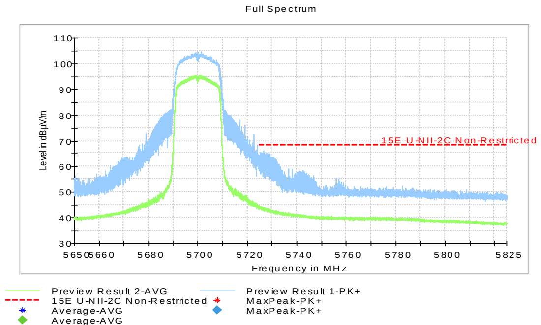
Fig.41 Band Edges (802.11n-HT20, 5700MHz)
