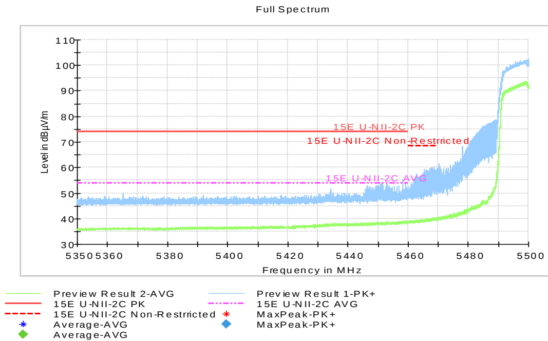
Fig.40 Band Edges (802.11n-HT20, 5500MHz)
