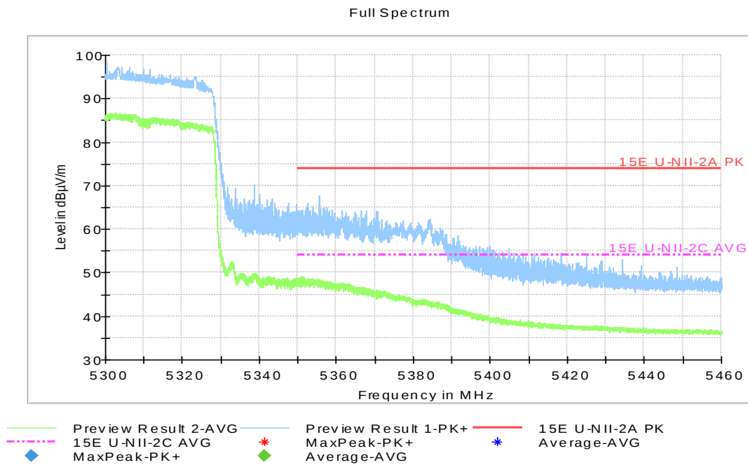
Fig.55 Band Edges (802.11ac-HT80, 5290MHz)
