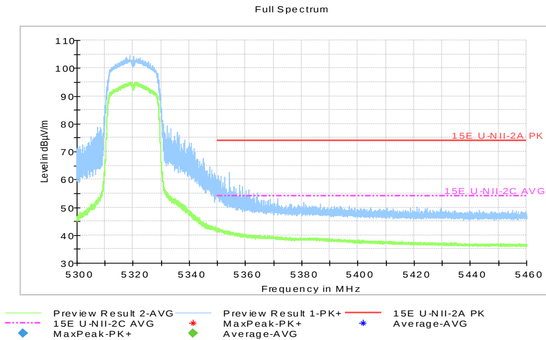
Fig.47 Band Edges (802.11ac-HT20, 5320MHz)
