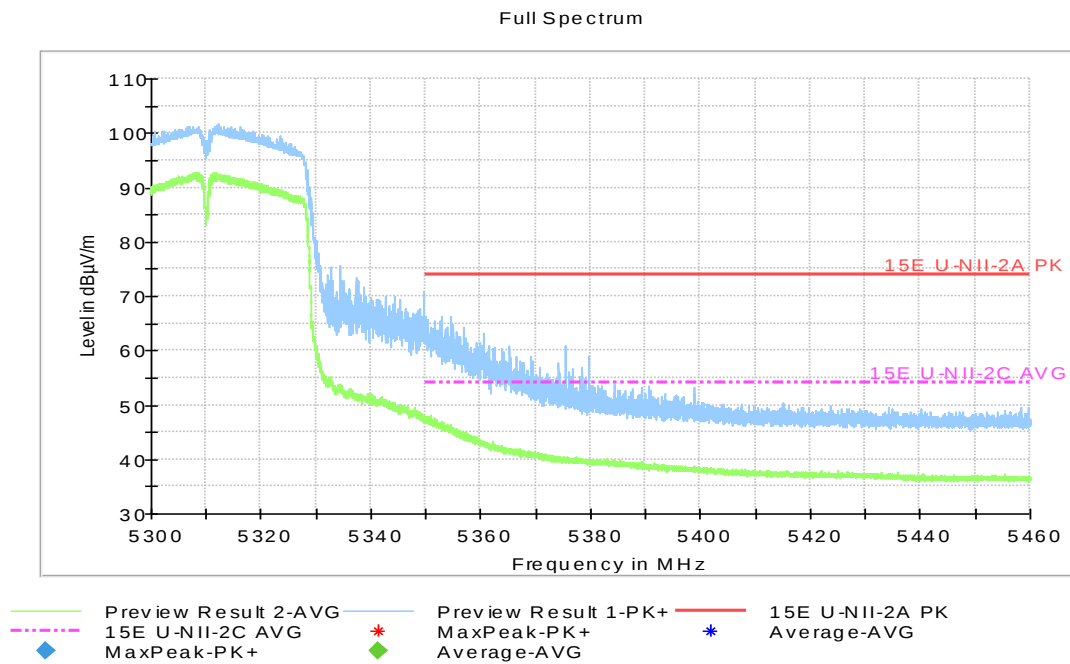
Fig.51 Band Edges (802.11ac-HT40, 5310MHz)
