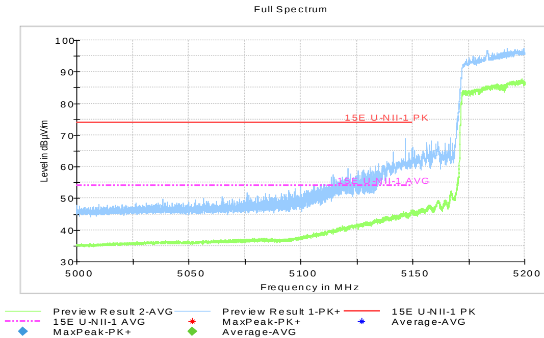
Fig.54 Band Edges (802.11ac-HT80, 5210MHz)
