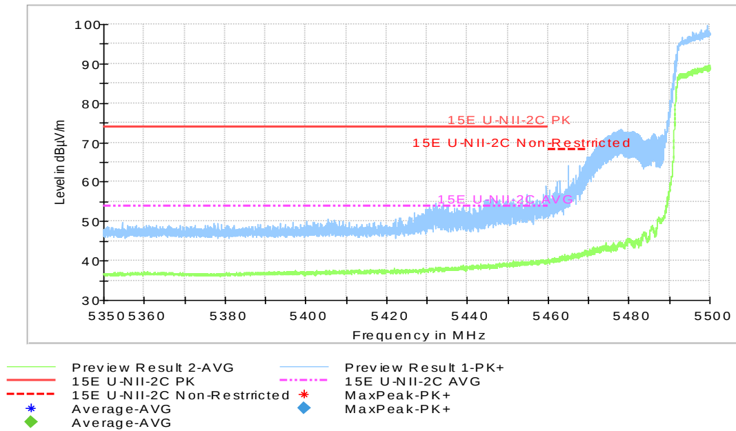
Fig.44 Band Edges (802.11n-HT40, 5510MHz)
