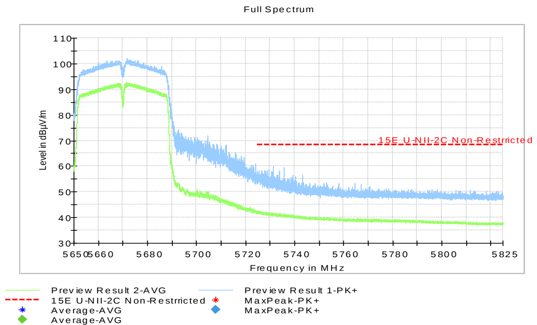
Fig.53 Band Edges (802.11ac-HT40, 5670MHz)
