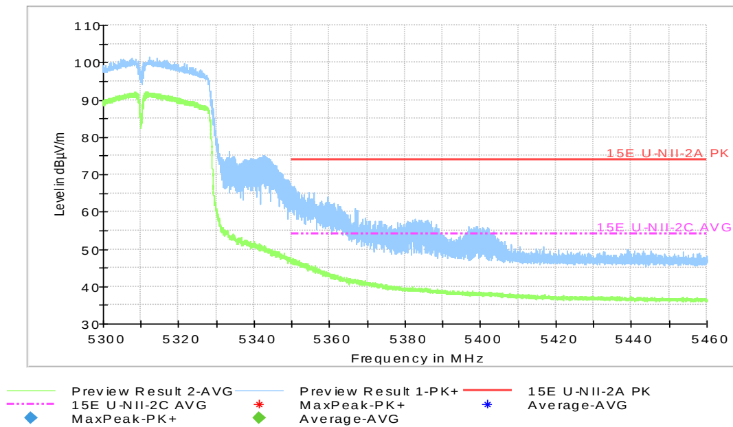
Fig.43 Band Edges (802.11n-HT40, 5310MHz)
