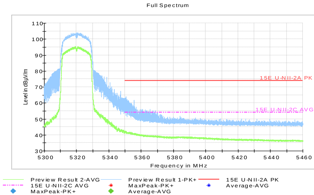
Fig.39 Band Edges (802.11n-HT20, 5320MHz)
