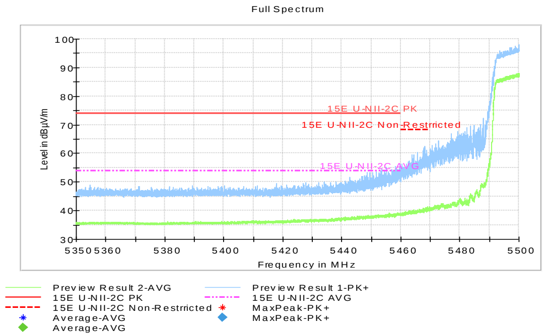
Fig.52 Band Edges (802.11ac-HT40, 5510MHz)
