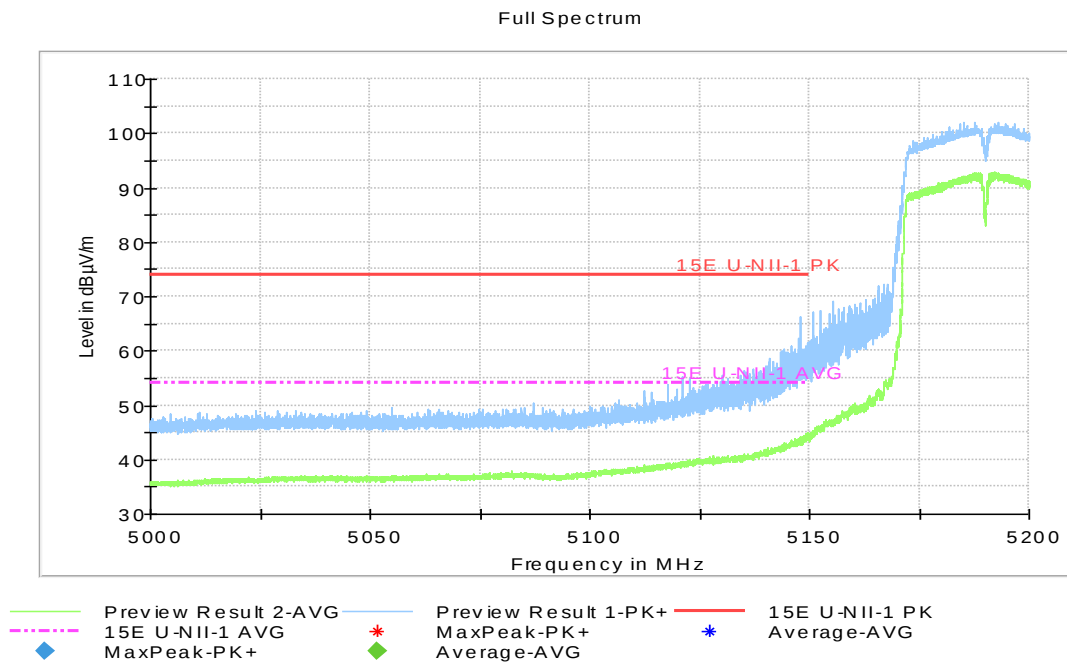
Fig.50 Band Edges (802.11ac-HT40, 5190MHz)
