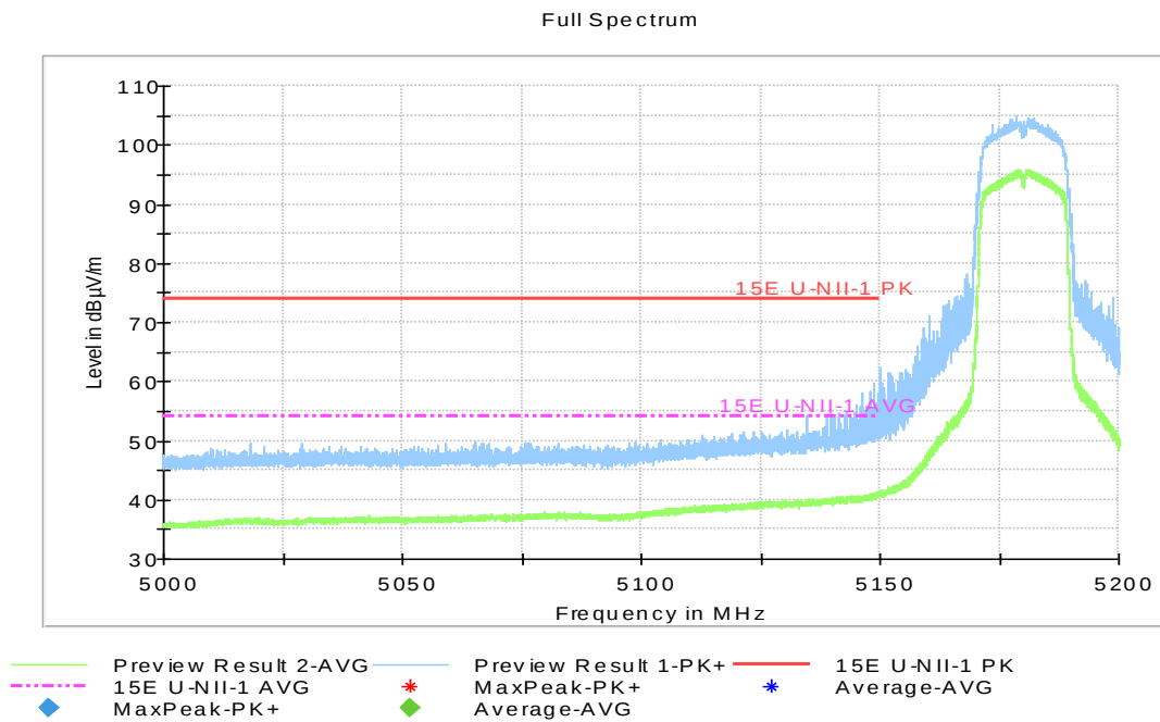
Fig.46 Band Edges (802.11ac-HT20, 5180MHz)
