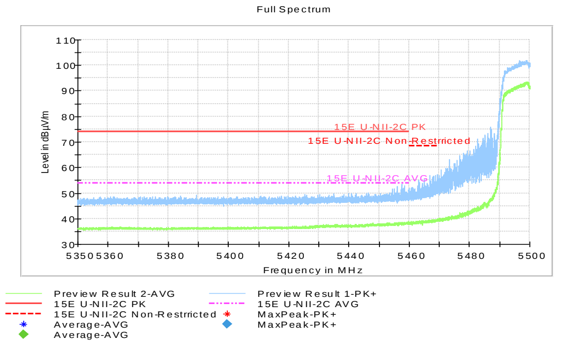
Fig.48 Band Edges (802.11ac-HT20, 5500MHz)
