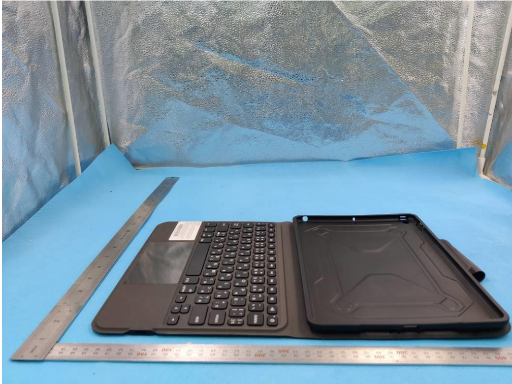
The series model name is UAG-BTKB-02-UK WHOLE VIEW OF EUT
