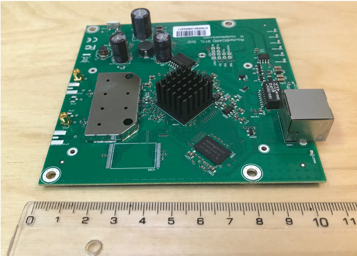
Internal Photos of EUT
