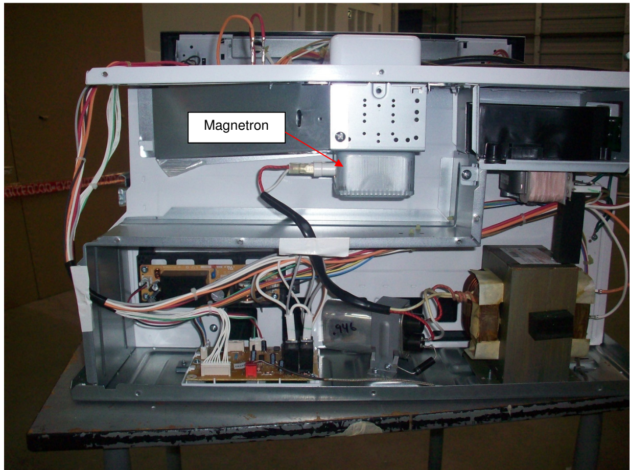
Figure 3. Magnetron Location
