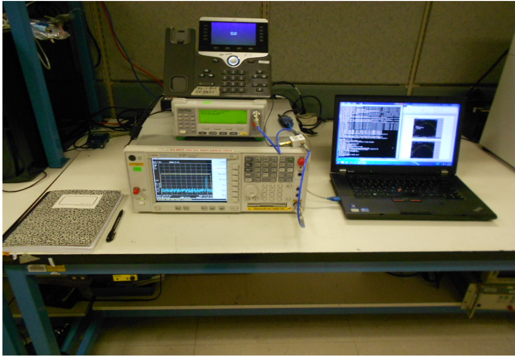
Title: Bluetooth & RF Conducted Test Setup
