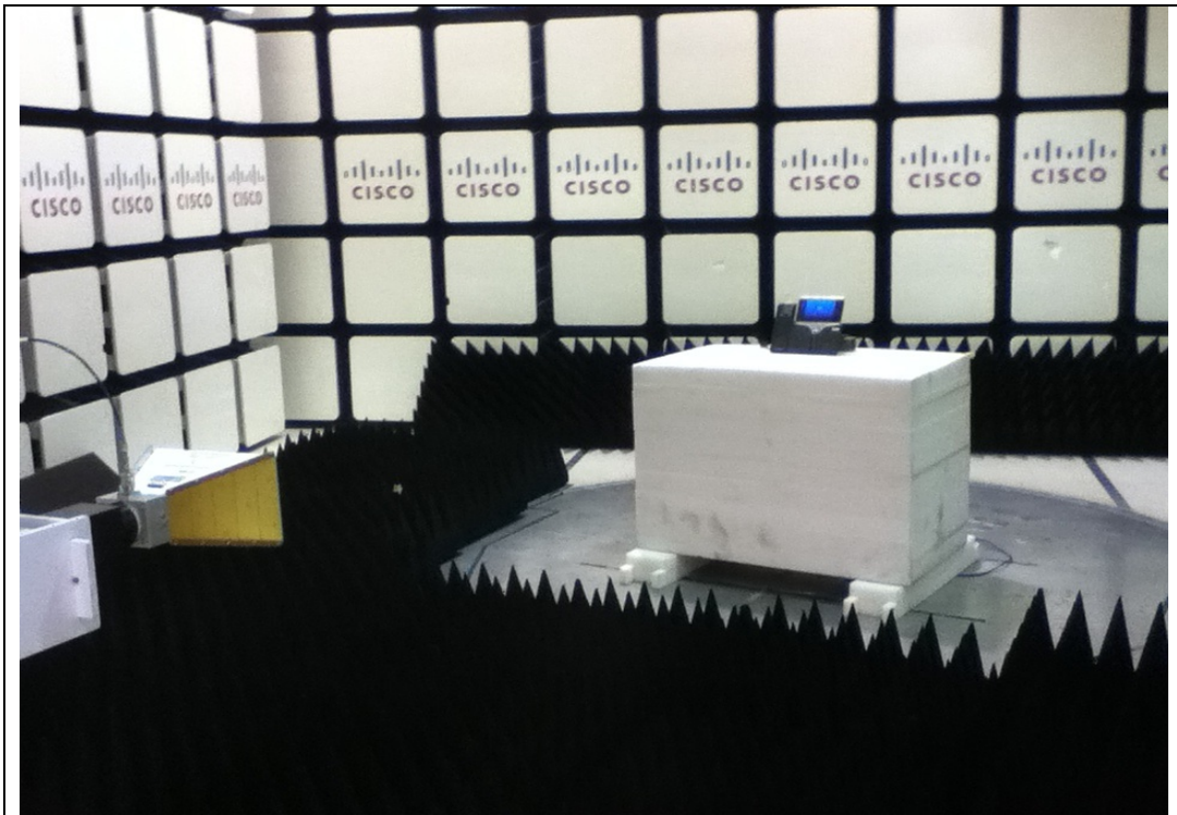
Title: Radiated Test Configuration from 1 - 18GHz
