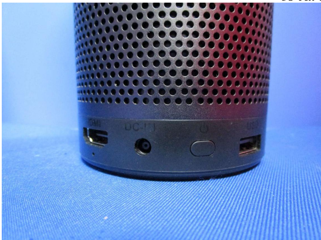
Figure 10 I/O Port of the EUT
