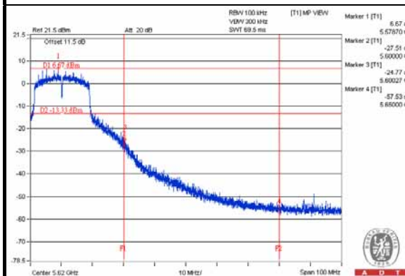
802.11n (HT20) OFDM MODULATION (CH 116: 5580MHz)
