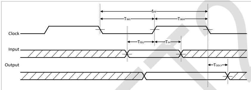
SDIO Protocol Timing Diagram – Default Speed Mode (V SD 3.3 V)
