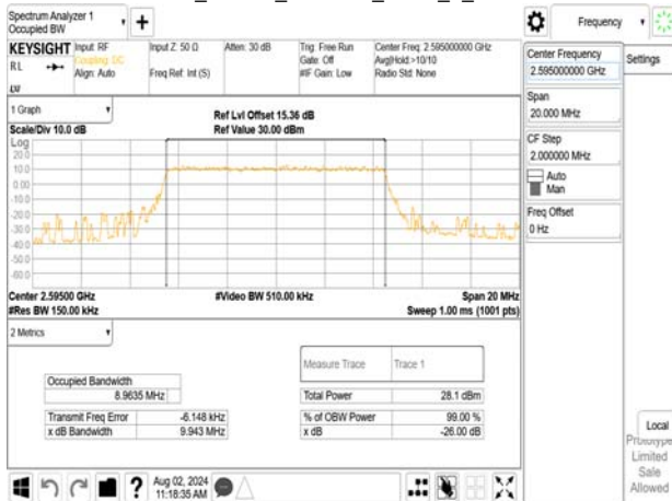
Band38_10MHz_256QAM_RB50_0_CH38200
