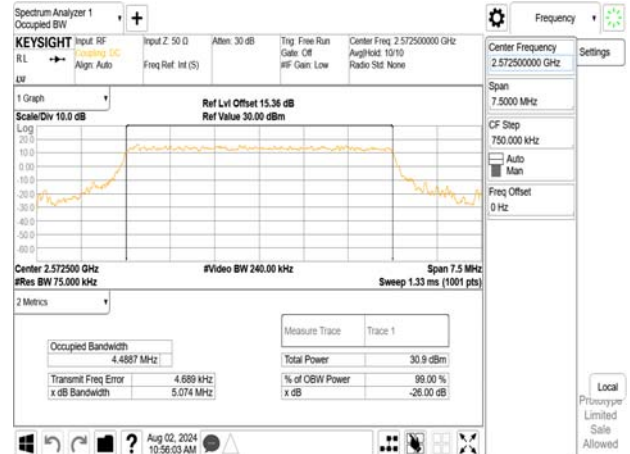
Band38_5MHz_16QAM_RB25_0_CH37775
