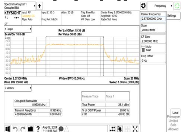
Band38_10MHz_256QAM_RB50_0_CH37800
