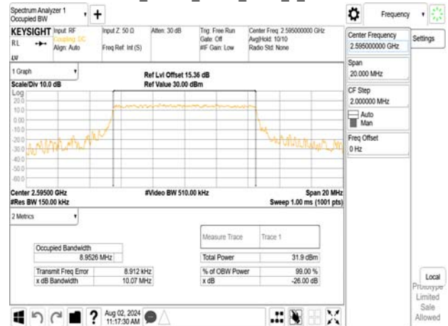
Band38_10MHz_QPSK_RB50_0_CH38200
