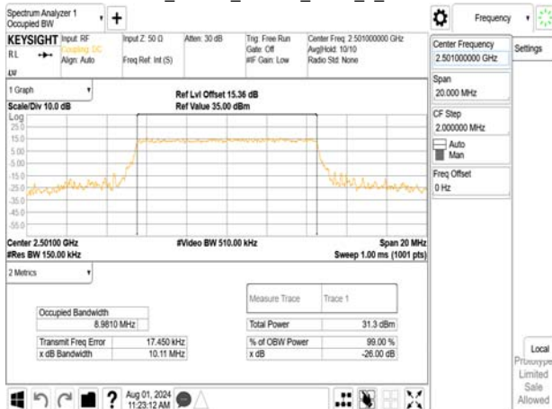
Band41_10MHz_64QAM_RB50_0_CH39700
