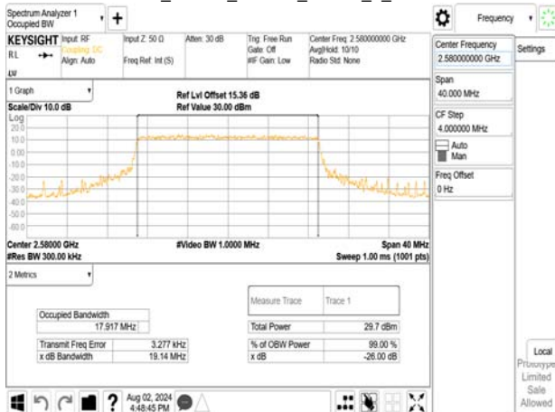
Band38_20MHz_64QAM_RB100_0_CH37850
