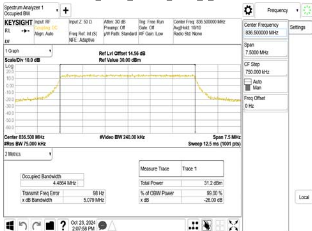
Band26_5MHz_16QAM_RB25_0_CH26915
