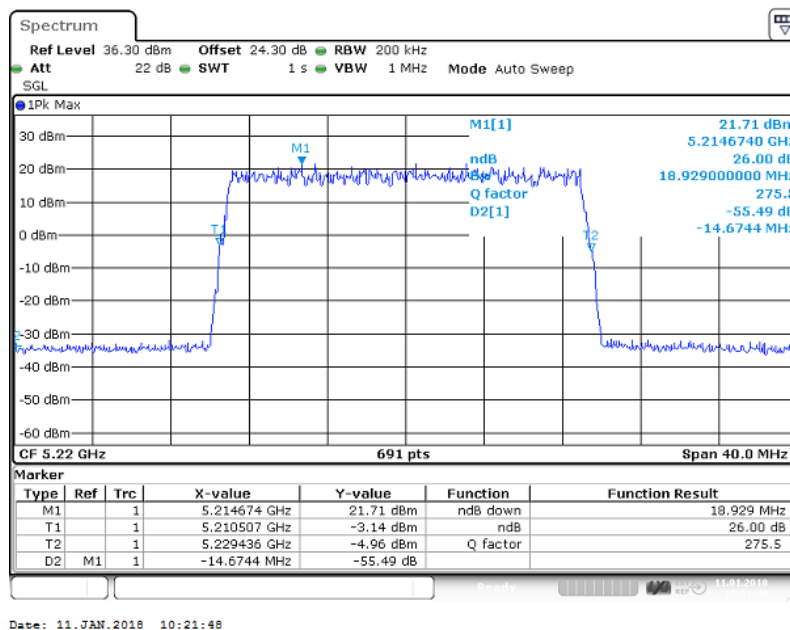
Figure 39 Occupied Bandwidth – 16QAM (5220.0 MHz) (20MHz Channel BW)
