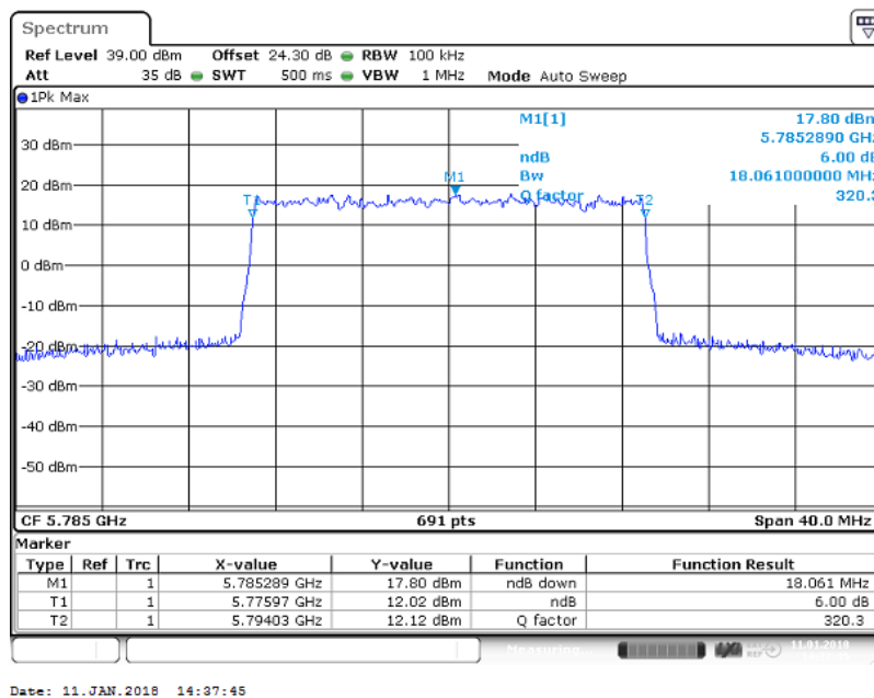
Figure 55 Occupied Bandwidth – 16QAM (5785.0 MHz) (20MHz Channel BW)
