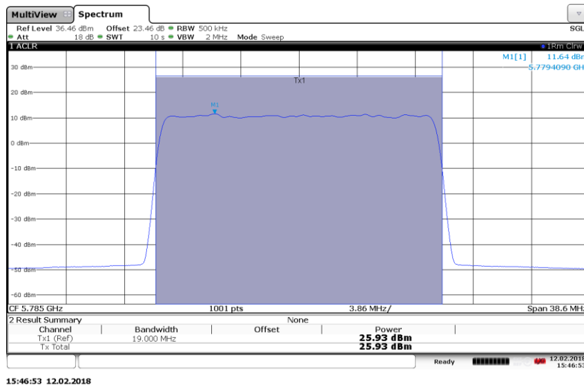
Figure 27 Output Power and Power Spectral Density – 16QAMQPSK (5785.0 MHz) (20MHz Channel BW)
