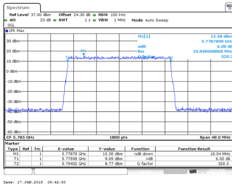
Figure 58 Occupied Bandwidth – 64QAM (5785.0 MHz) (20MHz Channel BW)
