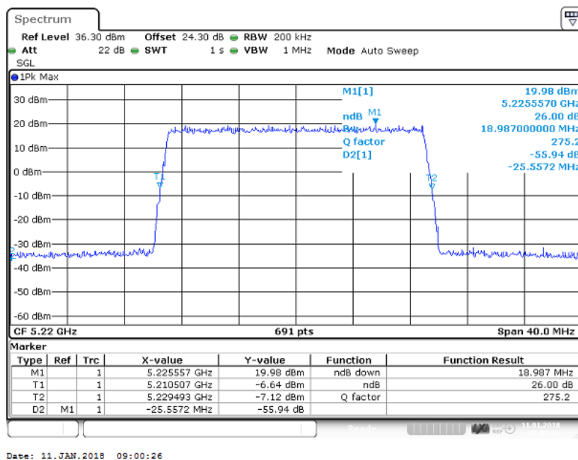
Figure 40 Occupied Bandwidth – 256QAM (5220.0 MHz) (20MHz Channel BW)
