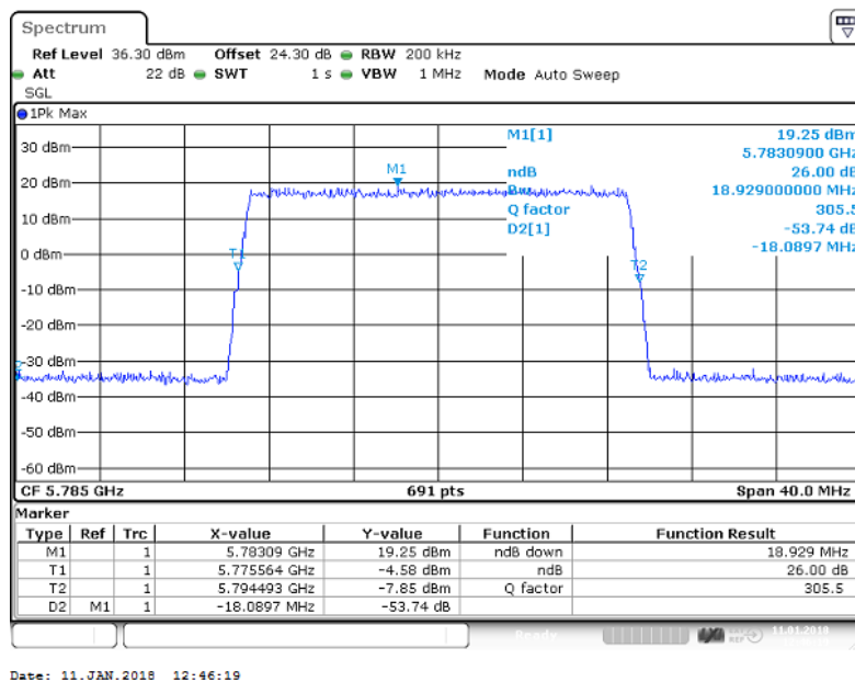
Figure 48 Occupied Bandwidth – 256QAM (5785.0 MHz) (20MHz Channel BW)
