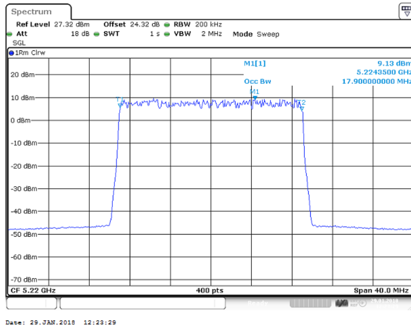
Figure 31 Occupied Bandwidth – 16QAM (5220.0 MHz) (20MHz Channel BW)
