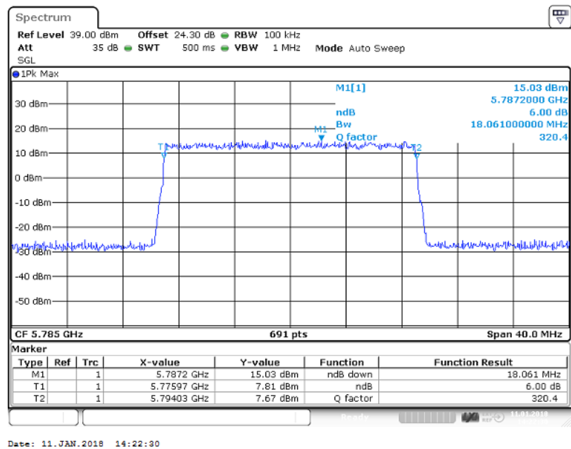
Figure 54 Occupied Bandwidth – 64QAM (5785.0 MHz) (20MHz Channel BW)
