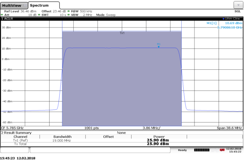
Figure 26 Output Power and Power Spectral Density – 64QAMQPSK (5785.0 MHz) (20MHz Channel BW)
