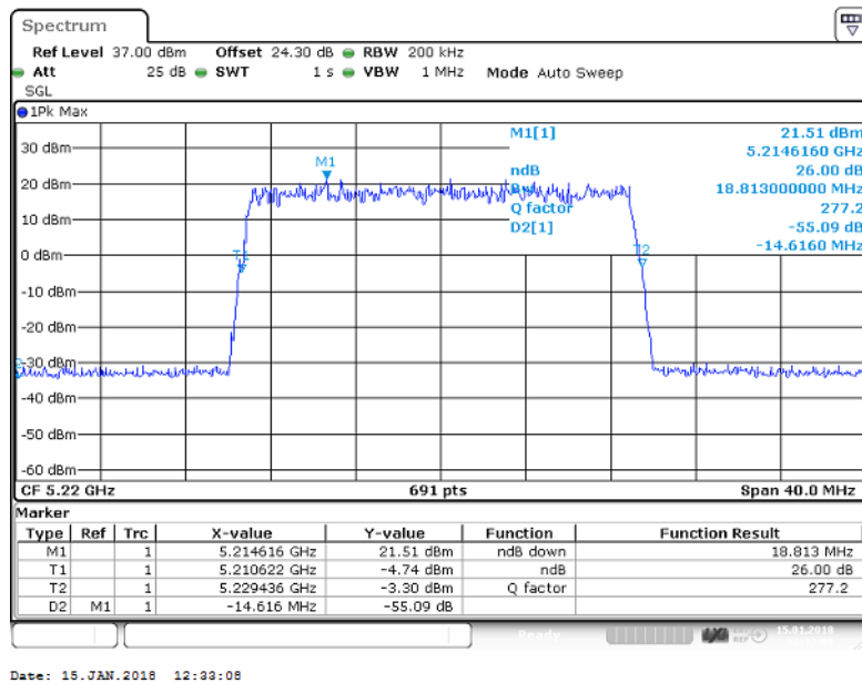
Figure 43 Occupied Bandwidth – 16QAM (5220.0 MHz) (20MHz Channel BW)
