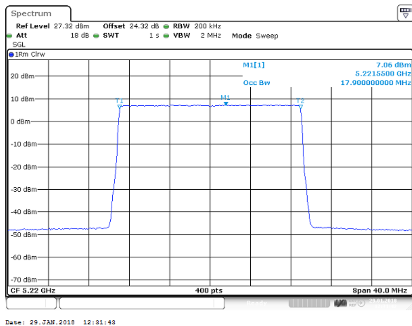
Figure 34 Occupied Bandwidth – 64QAM (5220.0 MHz) (20MHz Channel BW)
