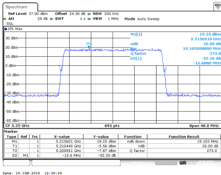
Figure 44 Occupied Bandwidth – 256QAM (5220.0 MHz) (20MHz Channel BW)
