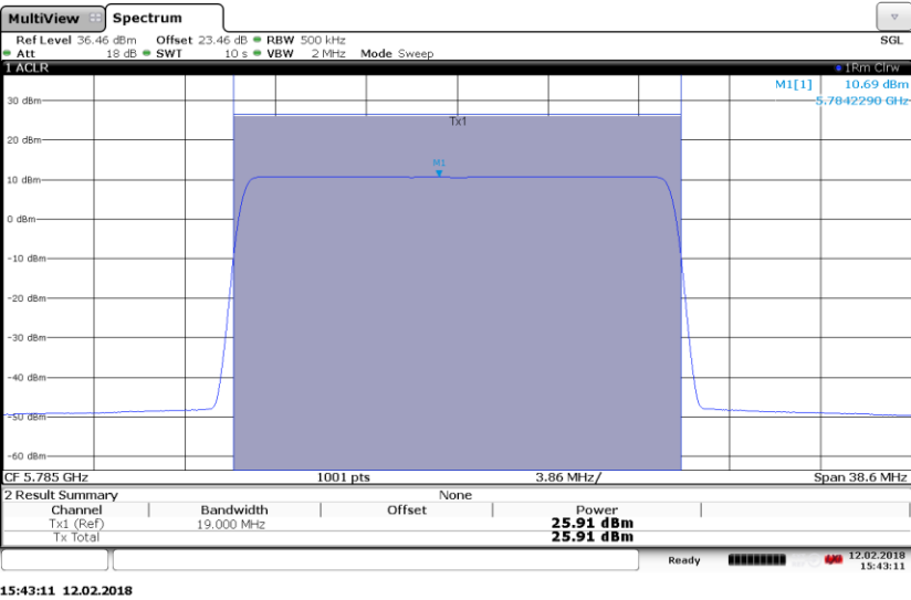
Figure 25 Output Power and Power Spectral Density – QPSK (5785.0 MHz) (20MHz Channel BW)
