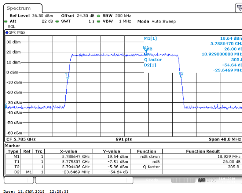
Figure 46 Occupied Bandwidth – 64QAM (5785.0 MHz) (20MHz Channel BW)
