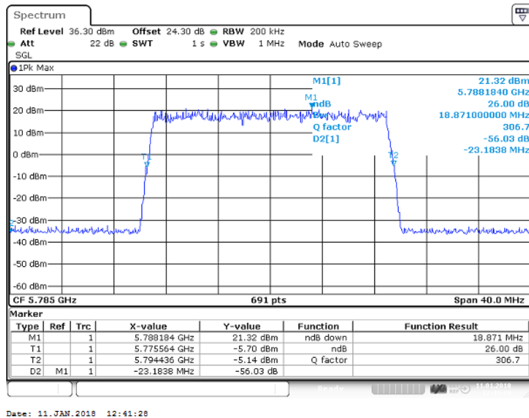
Figure 47 Occupied Bandwidth – 16QAM (5785.0 MHz) (20MHz Channel BW)
