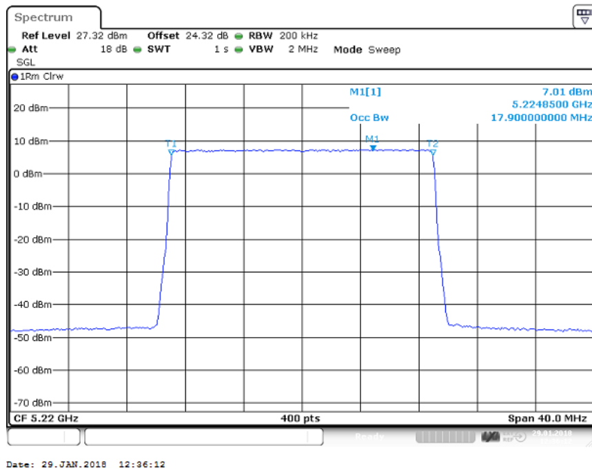
Figure 36 Occupied Bandwidth – 256QAM (5220.0 MHz) (20MHz Channel BW)
