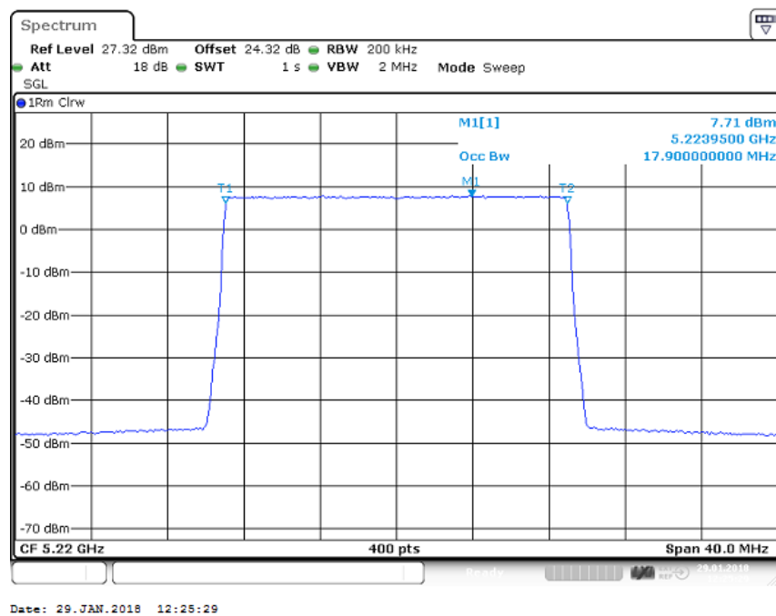
Figure 32 Occupied Bandwidth – 256QAM (5220.0 MHz) (20MHz Channel BW)
