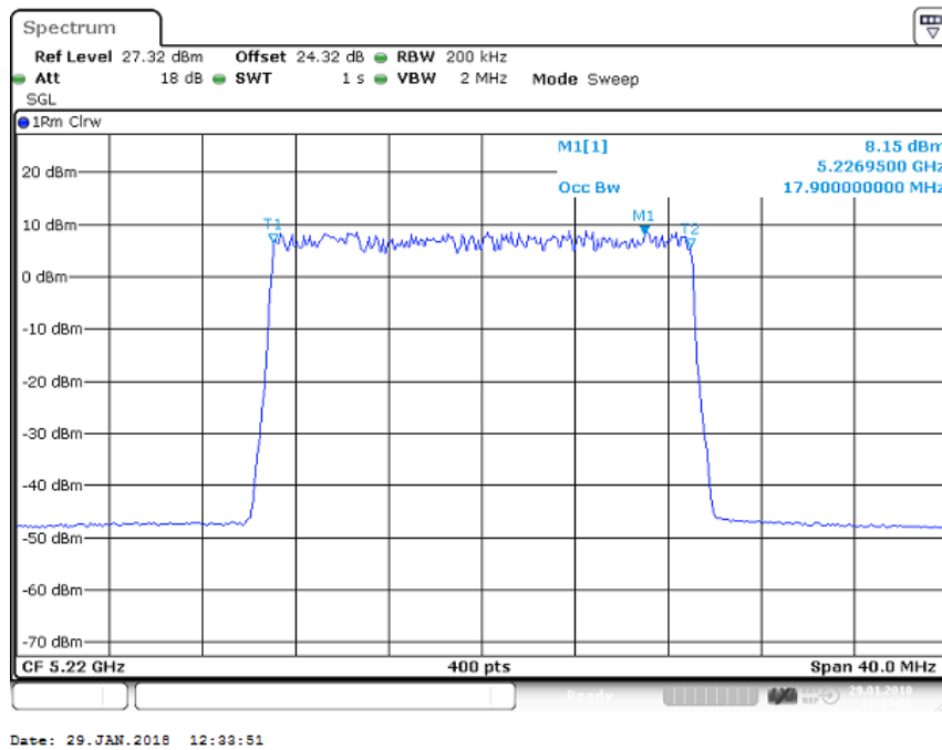
Figure 35 Occupied Bandwidth – 16QAM (5220.0 MHz) (20MHz Channel BW)
