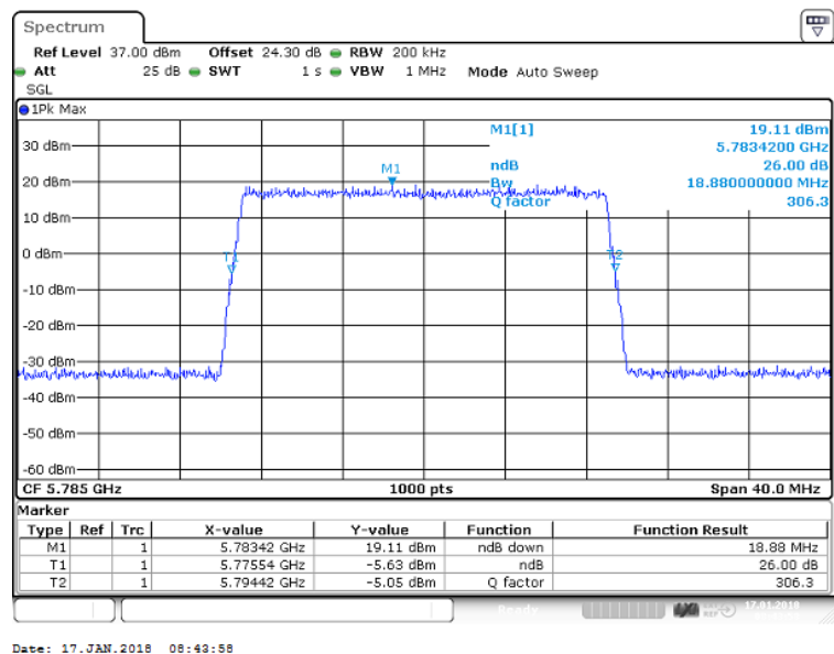
Figure 50 Occupied Bandwidth – 64QAM (5785.0 MHz) (20MHz Channel BW)
