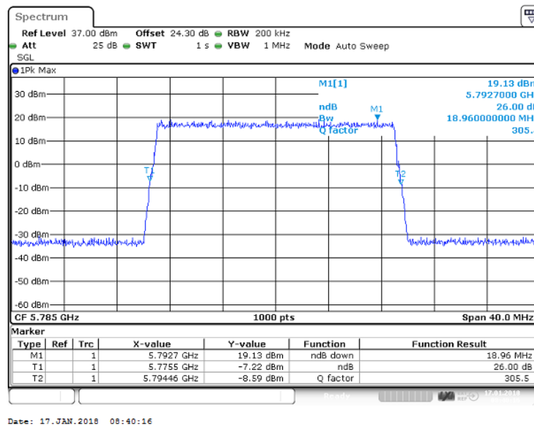
Figure 49 Occupied Bandwidth – QPSK (5785.0 MHz) (20MHz Channel BW)
