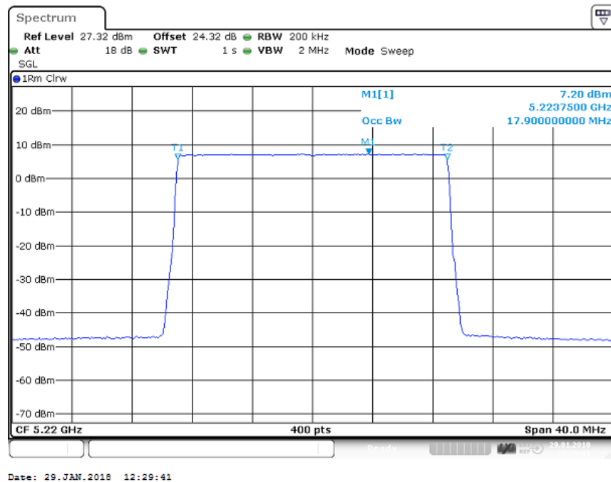
Figure 33 Occupied Bandwidth – QPSK (5220.0 MHz) (20MHz Channel BW)
