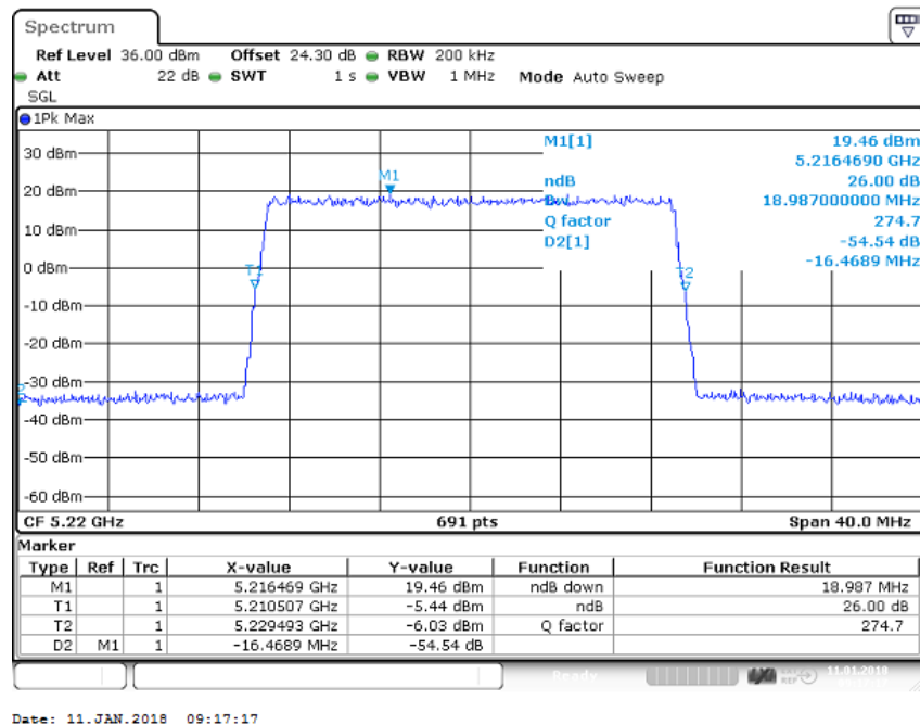
Figure 37 Occupied Bandwidth – QPSK (5220.0 MHz) (20MHz Channel BW)
