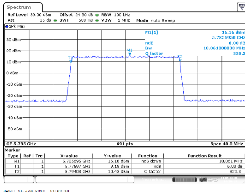
Figure 53 Occupied Bandwidth – QPSK (5785.0 MHz) (20MHz Channel BW)
