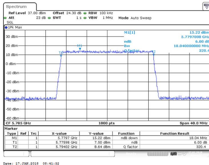
Figure 57 Occupied Bandwidth – QPSK (5785.0 MHz) (20MHz Channel BW)
