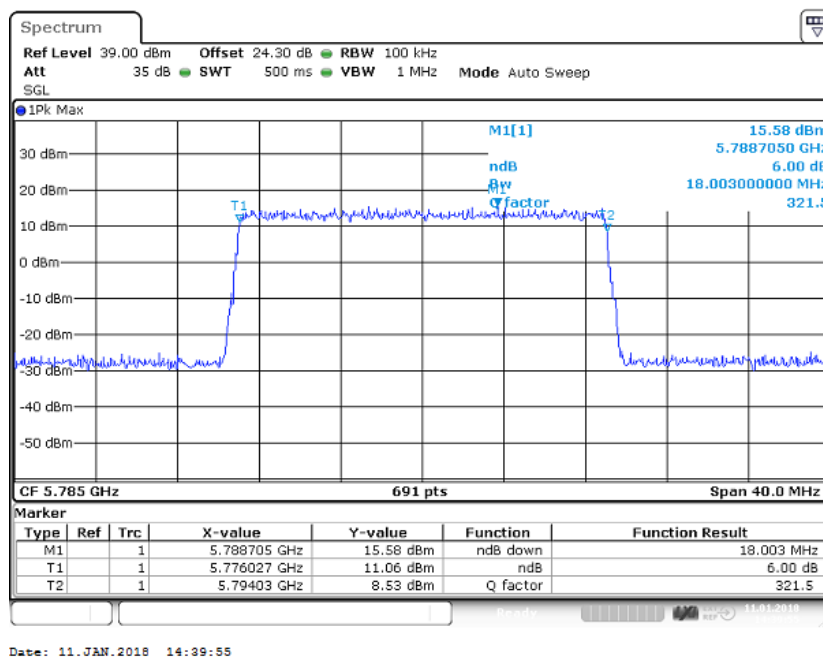
Figure 56 Occupied Bandwidth – 256QAM (5785.0 MHz) (20MHz Channel BW)
