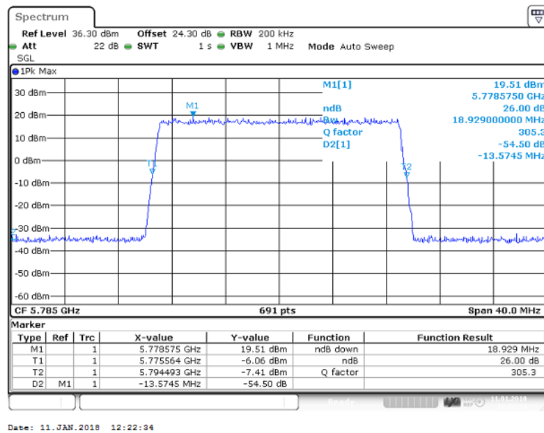
Figure 45 Occupied Bandwidth – QPSK (5785.0 MHz) (20MHz Channel BW)
