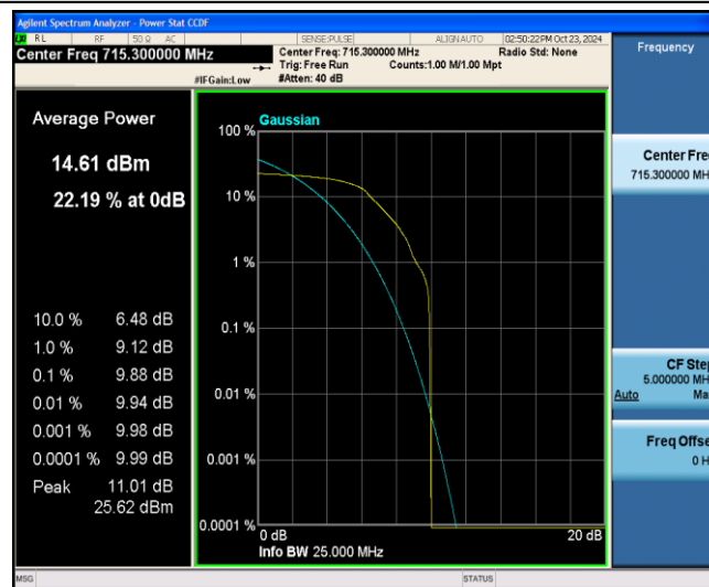
Band12-1.4MHz-QPSK-23173-1-0-Low-9.88-&lt;=13-PASS
