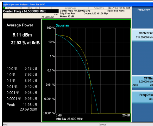
Band12-3MHz-QPSK-23165-6-0-Low-8.91-=&lt;=13-PASS
