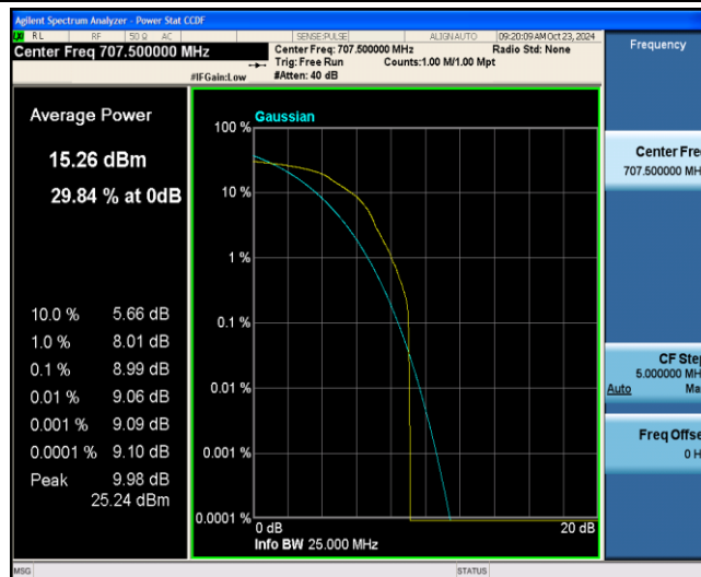
Band12-1.4MHz-16QAM-23095-1-0-Low-8.99-&lt;=13-PASS
