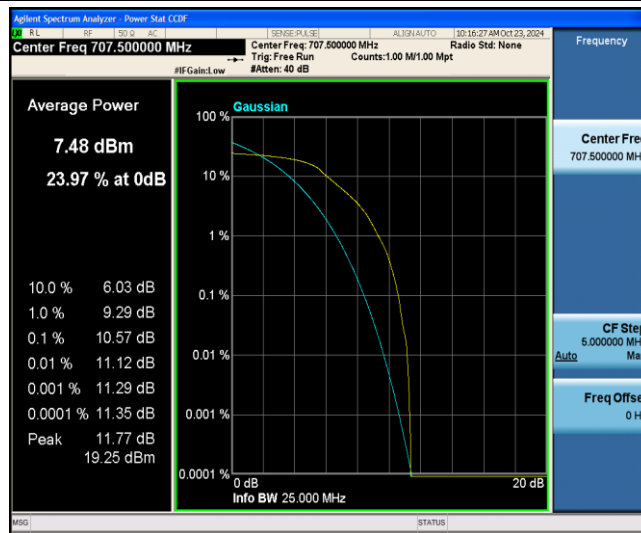
Band12-3MHz-QPSK-23095-6-0-Low-10.57-=&lt;=13-PASS
