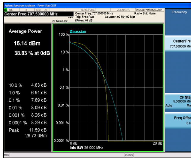
Band12-1.4MHz-QPSK-23095-6-0-Low-7.69-&lt;=13-PASS
