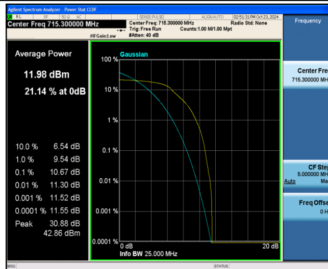
Band12-1.4MHz-QPSK-23173-6-0-Low-10.67-&lt;=13-PASS
