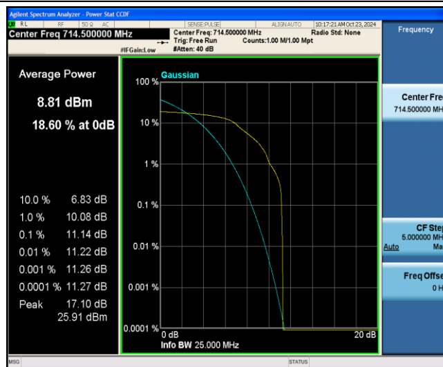
Band12-3MHz-QPSK-23165-1-0-Low-11.14-=&lt;=13-PASS
