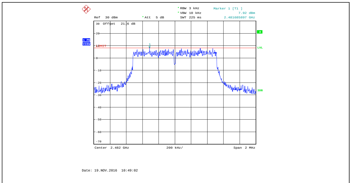
Plot 5.6.4.39. Power Spectral Density, Bandwidth: 1 MHz, TX Gain Setting: 43, Data Rate 5, 2482 MHz
