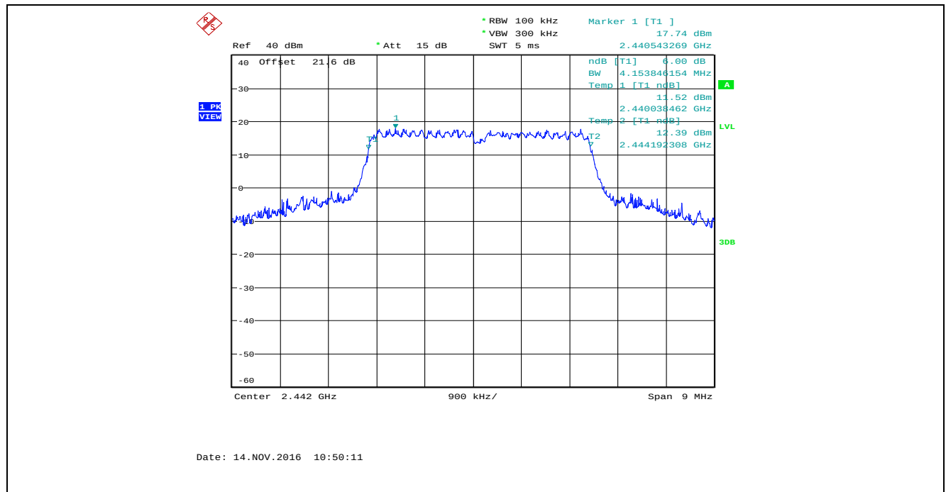
Plot 5.2.4.59. 6 dB Bandwidth, Bandwidth: 4 MHz, TX Gain: 50, Data Rate 4, 2442 MHz
