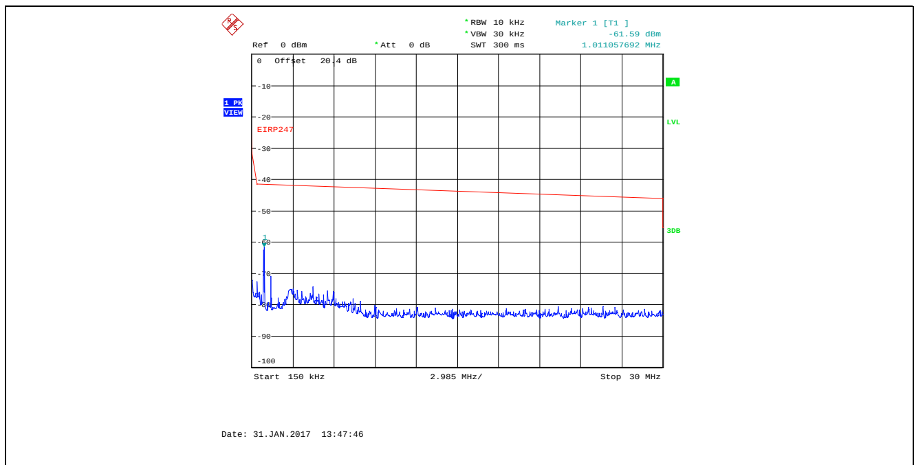
Plot 5.4.4.4.31. Conducted Spurious Emissions in Restricted Frequency Bands Bandwidth: 8 MHz, TX Gain Setting 25, Data Rate 4, 2477 MHz, 150 kHz - 30 MHz, Peak Detector
