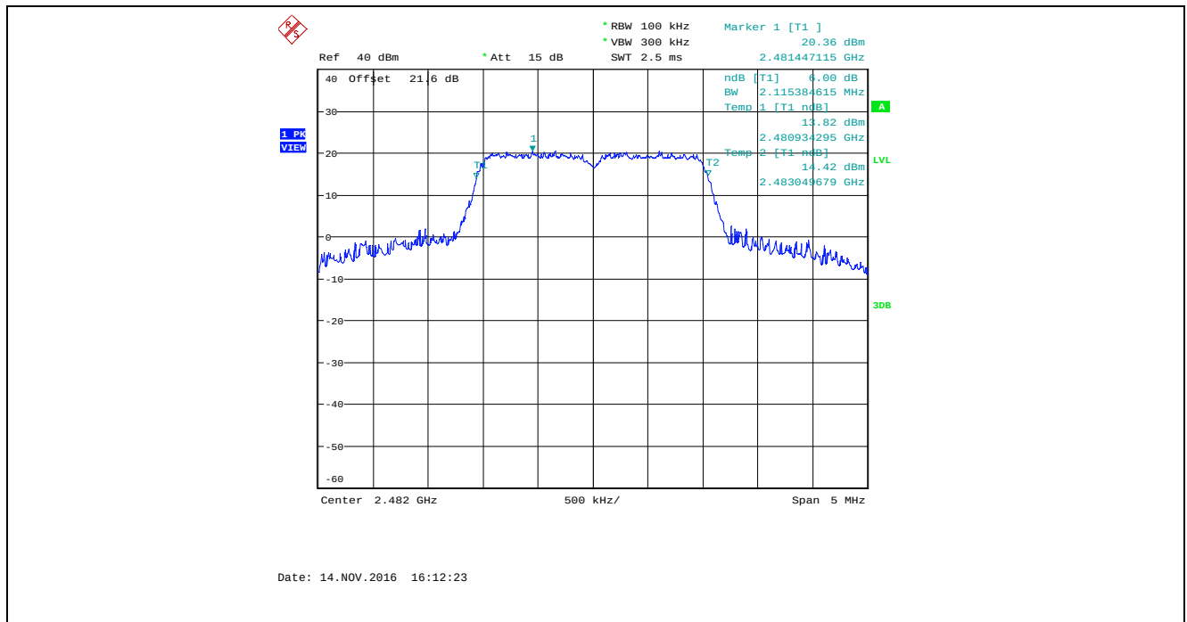
Plot 5.2.4.48. 6 dB Bandwidth, Bandwidth: 2 MHz, TX Gain: 45, Data Rate 4, 2482 MHz
