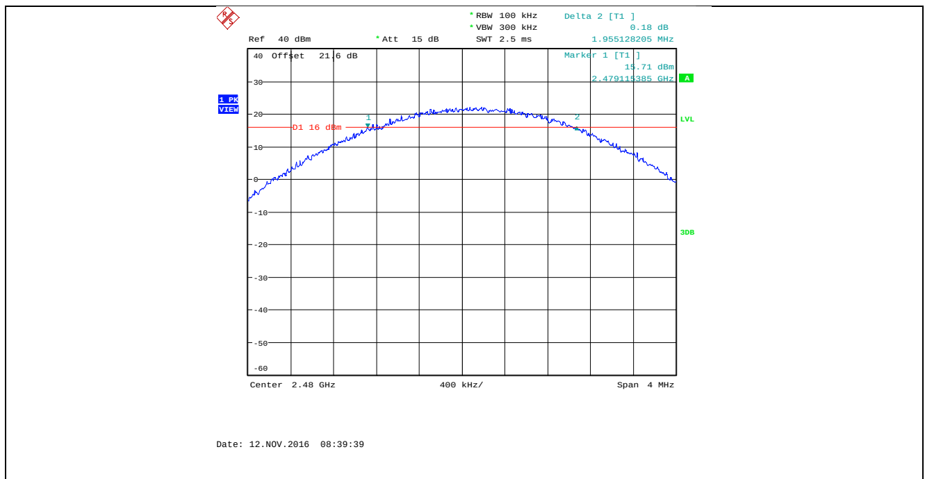
Plot 5.2.4.24. 6 dB Bandwidth, Bandwidth: 4 MHz, TX Gain: 43, Data Rate 3, 2480 MHz
