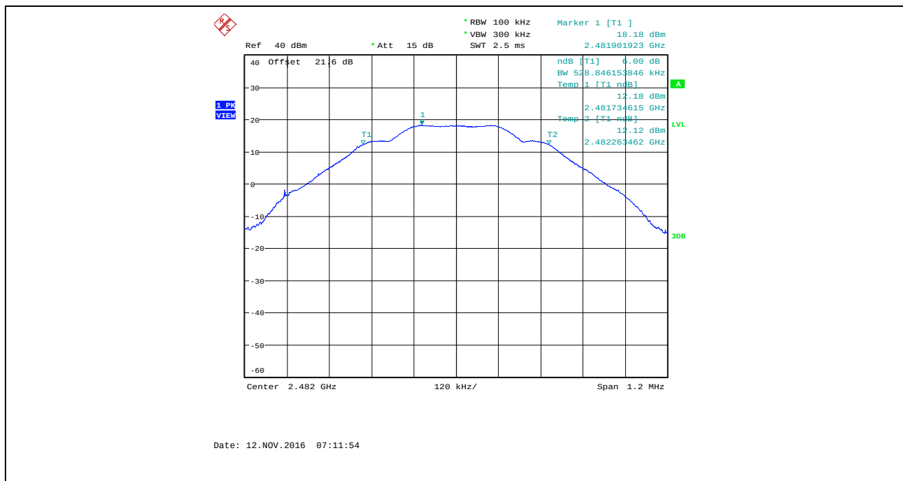
Plot 5.2.4.6. 6 dB Bandwidth, Bandwidth: 1 MHz, TX Gain: 26, Data Rate 2, 2482 MHz
