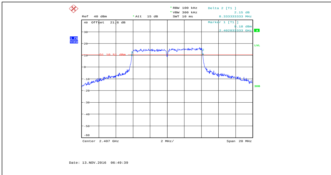
Plot 5.2.4.79. 6 dB Bandwidth, Bandwidth: 8 MHz, TX Gain: 55, Data Rate 7, 2407 MHz
