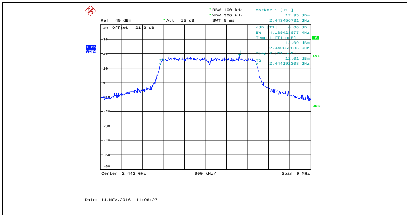
Plot 5.2.4.62. 6 dB Bandwidth, Bandwidth: 4 MHz, TX Gain: 50, Data Rate 5, 2442 MHz
