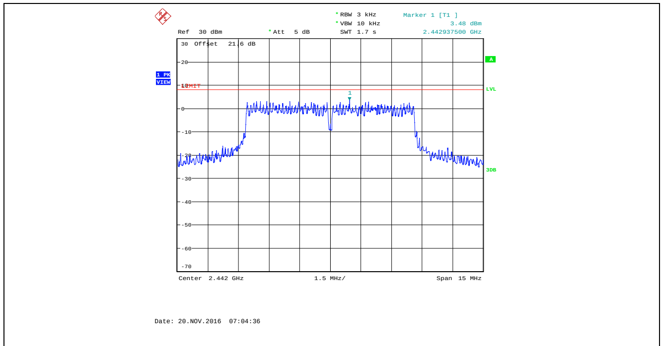
Plot 5.6.4.71. Power Spectral Density, Bandwidth: 8 MHz, TX Gain Setting: 55, Data Rate 4, 2442 MHz
