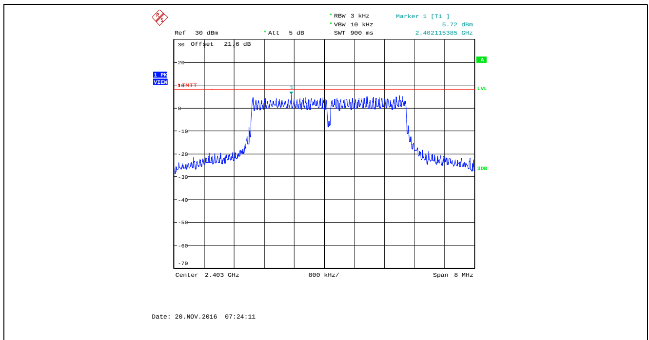
Plot 5.6.4.67. Power Spectral Density, Bandwidth: 4 MHz, TX Gain Setting: 50, Data Rate 7, 2403 MHz
