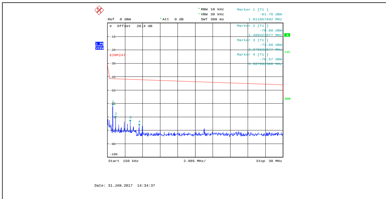
Plot 5.4.4.4.7. Conducted Spurious Emissions in Restricted Frequency Bands Bandwidth: 8 MHz, TX Gain Setting 25, Data Rate 1, 2442 MHz, 150 kHz - 30 MHz, Peak Detector
