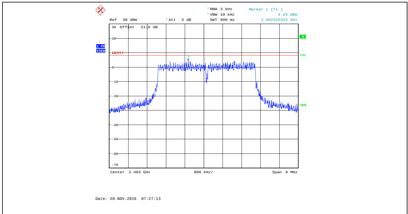
Plot 5.6.4.64. Power Spectral Density, Bandwidth: 4 MHz, TX Gain Setting: 50, Data Rate 6, 2403 MHz
