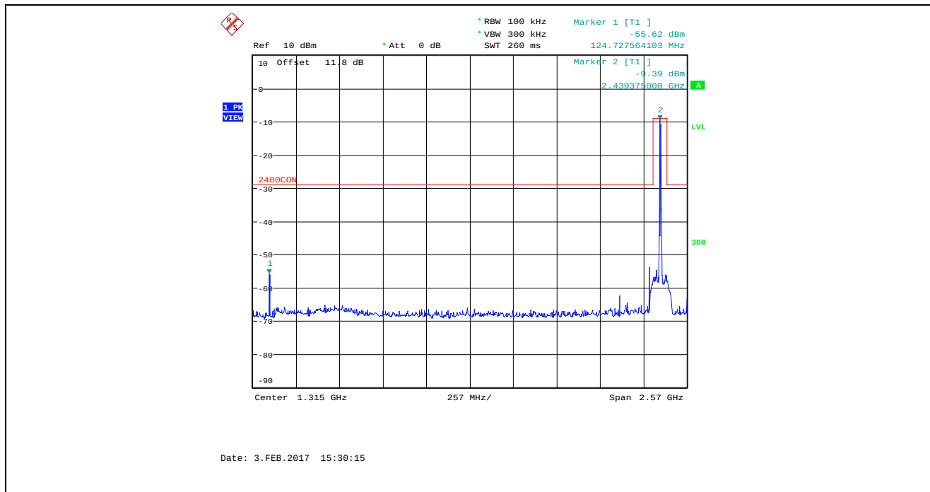
Plot 5.4.4.2.21. Conducted Spurious Emissions in Non-restricted Frequency Bands Bandwidth: 8 MHz, TX Gain: 0, Data Rate 4, 2442 MHz, 30 MHz – 2.6 GHz
