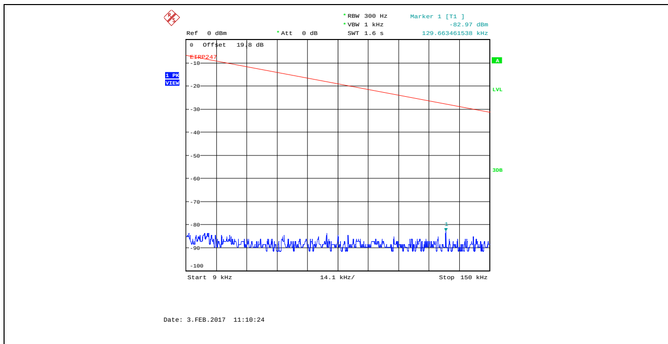
Plot 5.4.4.3.16. Conducted Spurious Emissions in Restricted Frequency Bands Bandwidth: 8 MHz, TX Gain Setting 55, Data Rate 4, 2407 MHz, 9 kHz - 150 kHz, Peak Detector
