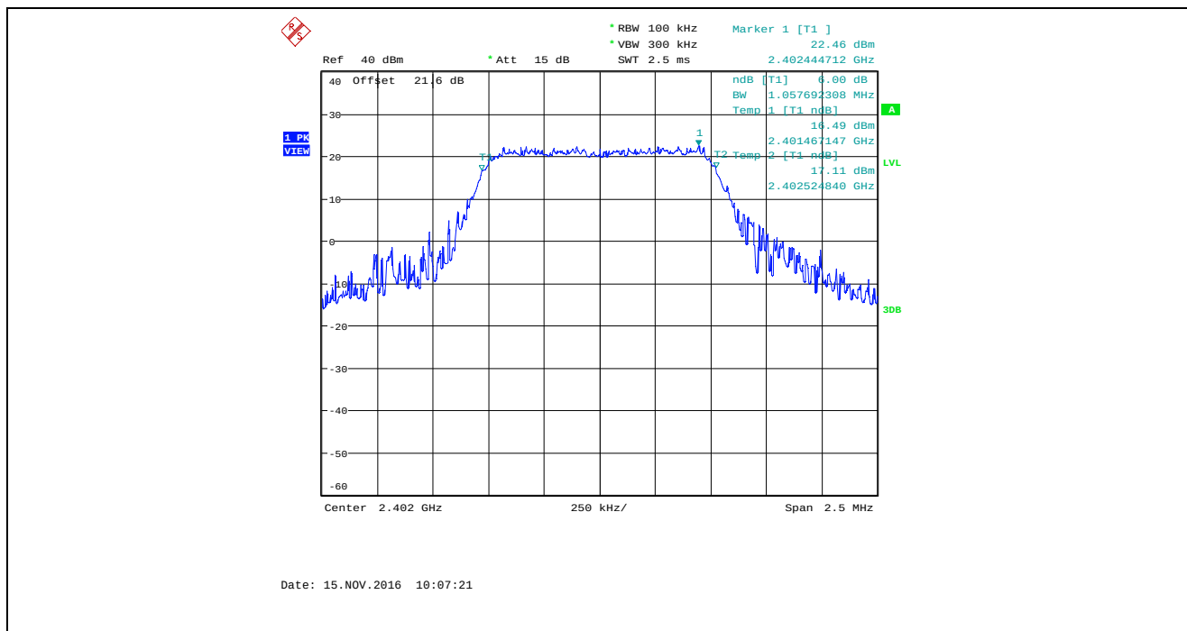
Plot 5.2.4.40. 6 dB Bandwidth, Bandwidth: 1 MHz, TX Gain: 43, Data Rate 6, 2402 MHz
