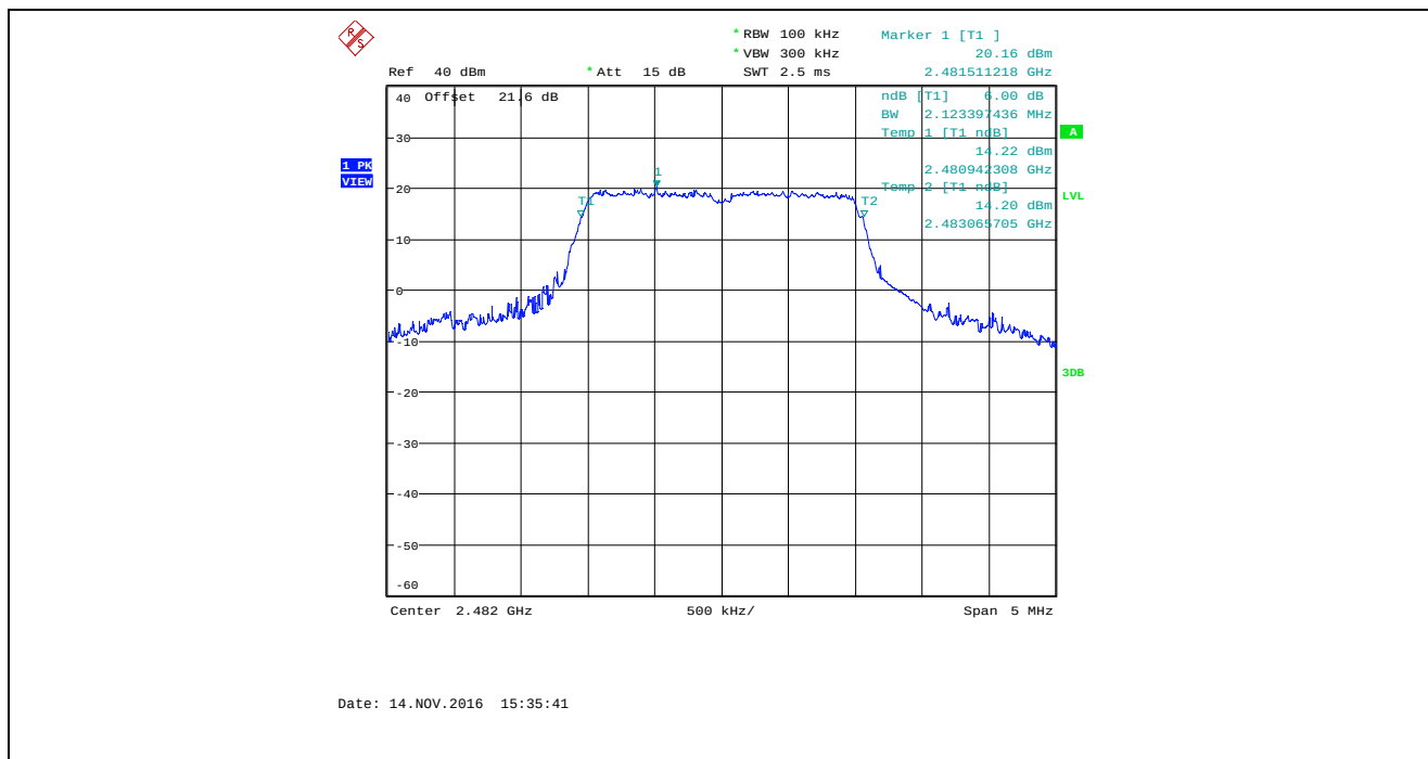
Plot 5.2.4.54. 6 dB Bandwidth, Bandwidth: 2 MHz, TX Gain: 45, Data Rate 6, 2482 MHz
