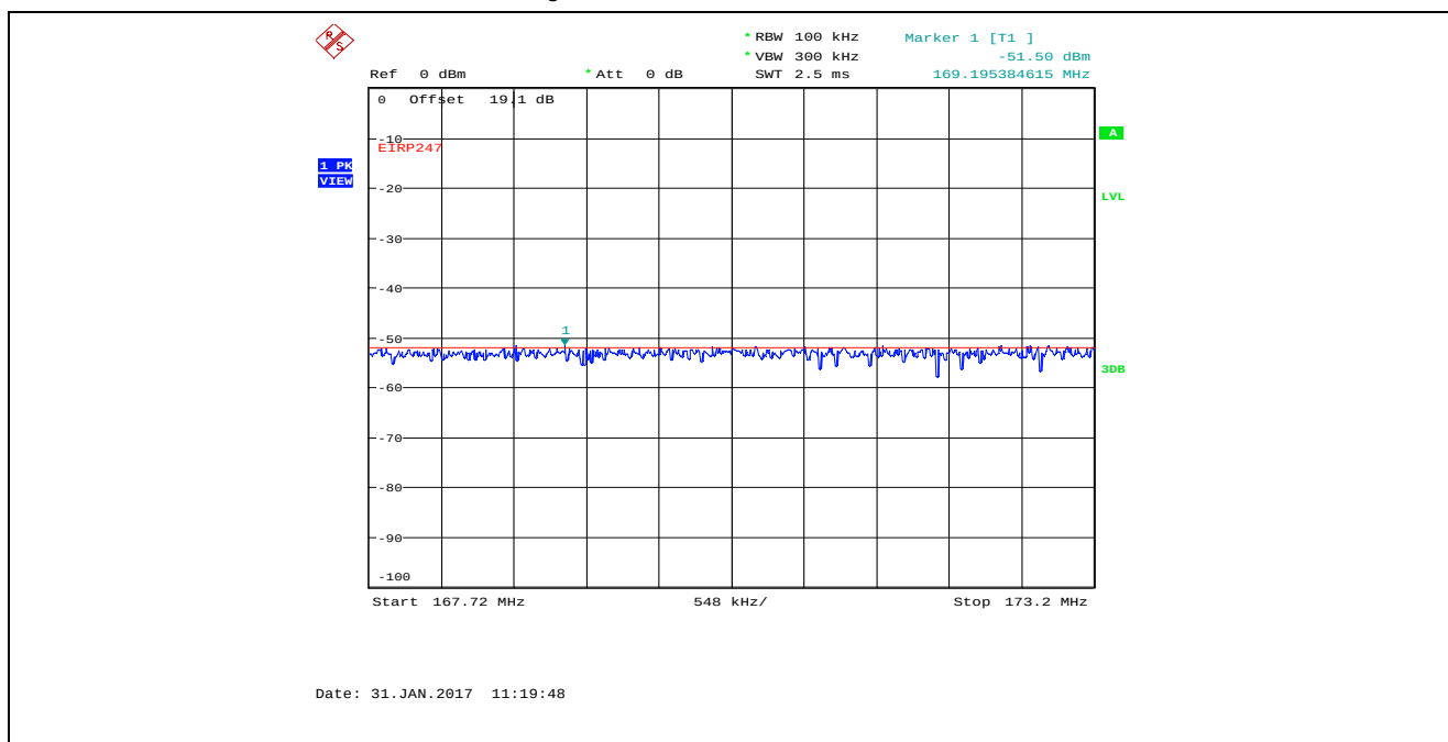
Plot 5.4.4.26. Conducted Spurious Emissions in Restricted Frequency Bands Bandwidth: 8 MHz, TX Gain Setting 25, Data Rate 4, 2442 MHz, RB 167.72-173.2 MHz, QP Detector
