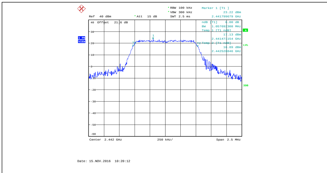
Plot 5.2.4.41. 6 dB Bandwidth, Bandwidth: 1 MHz, TX Gain: 43, Data Rate 6, 2442 MHz
