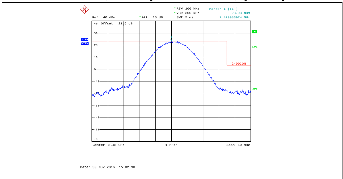
Plot 5.4.4.1.6. Band-Edge RF Conducted Emissions Bandwidth: 4 MHz, TX Gain Setting : 43, Data Rate 3, 2480 MHz, Higher Band-edge
