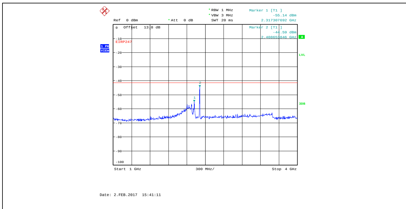
Plot 5.4.4.3.4. Conducted Spurious Emissions in Restricted Frequency Bands Bandwidth: 8 MHz, TX Gain Setting 50, Data Rate 1, 2407 MHz, 1 GHz - 4 GHz, Peak Detector
