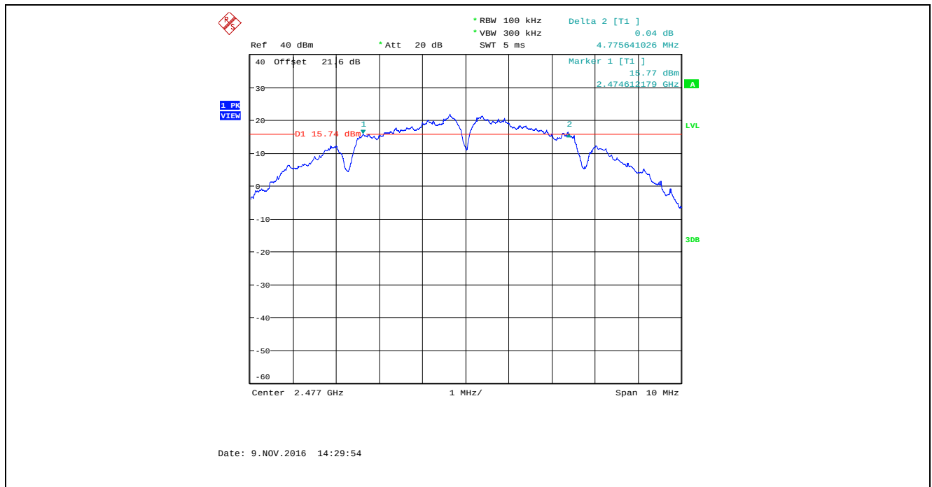
Plot 5.2.4.30. 6 dB Bandwidth, Bandwidth: 8 MHz, TX Gain: 50, Data Rate 2, 2477 MHz
