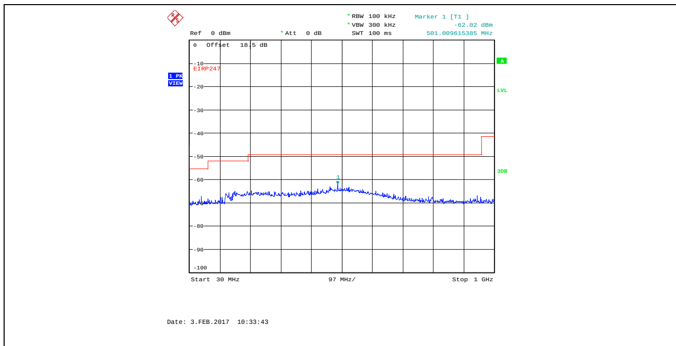
Plot 5.4.4.3.3. Conducted Spurious Emissions in Restricted Frequency Bands Bandwidth: 8 MHz, TX Gain Setting 50, Data Rate 1, 2407 MHz, 30 MHz - 1 GHz, Peak Detector
