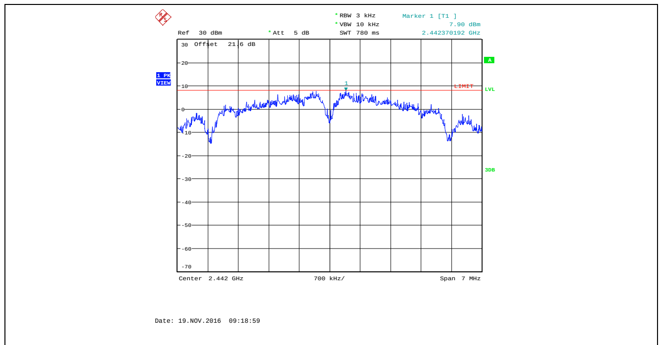
Plot 5.6.4.26. Power Spectral Density, Bandwidth: 8 MHz, TX Gain Setting: 50, Data Rate 1, 2442 MHz
