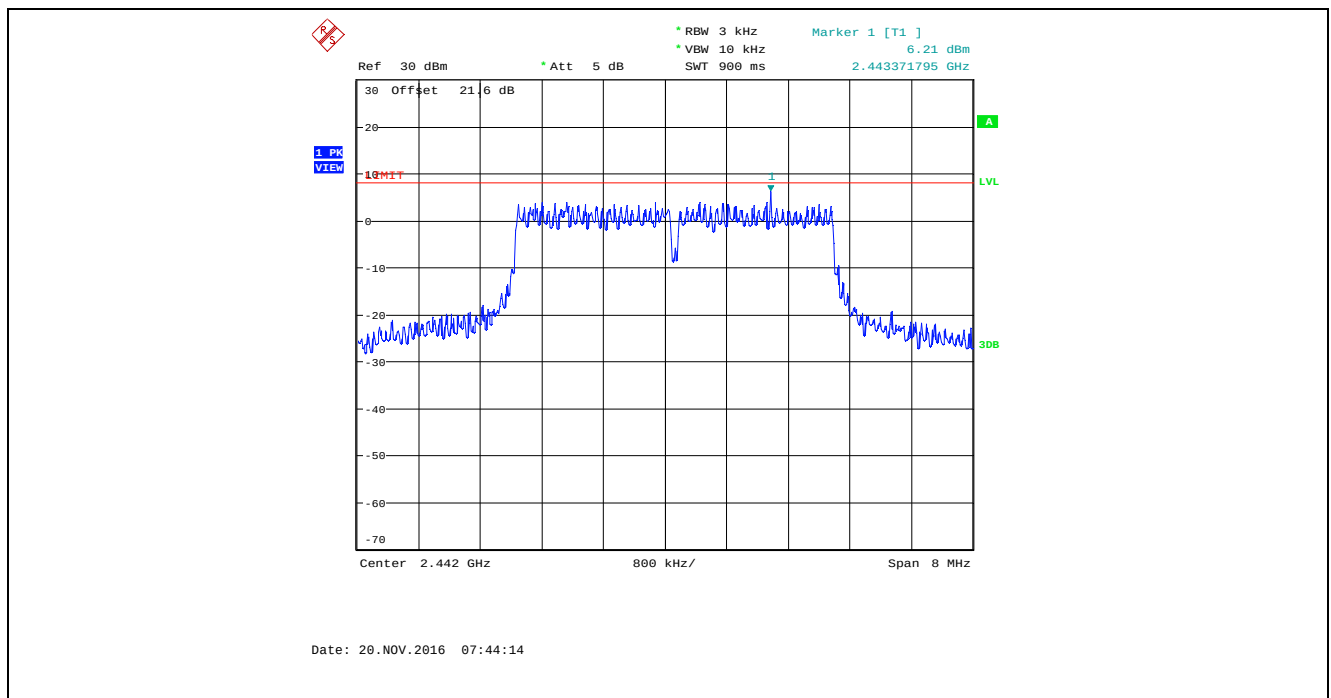
Plot 5.6.4.59. Power Spectral Density, Bandwidth: 4 MHz, TX Gain Setting: 50, Data Rate 4, 2442 MHz
