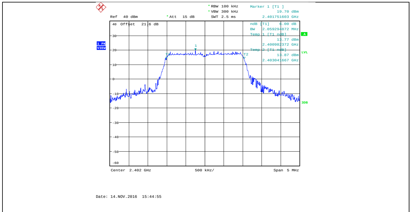
Plot 5.2.4.49. 6 dB Bandwidth, Bandwidth: 2 MHz, TX Gain: 45, Data Rate 5, 2402 MHz
