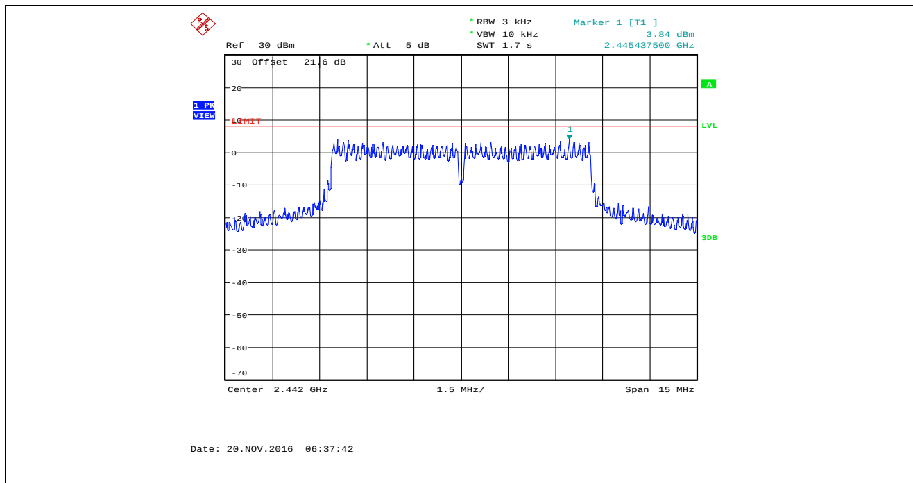
Plot 5.6.4.77. Power Spectral Density, Bandwidth: 8 MHz, TX Gain Setting: 55, Data Rate 6, 2442 MHz
