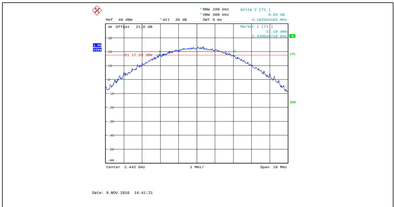
Plot 5.2.4.32. 6 dB Bandwidth, Bandwidth: 8 MHz, TX Gain: 50, Data Rate 3, 2442 MHz
