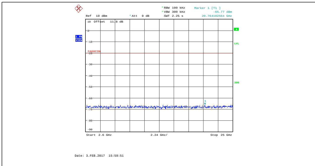
Plot 5.4.4.2.18. Conducted Spurious Emissions in Non-restricted Frequency Bands Bandwidth: 8 MHz, TX Gain: 0, Data Rate 1, 2477 MHz, 2.6 GHz – 25 GHz
