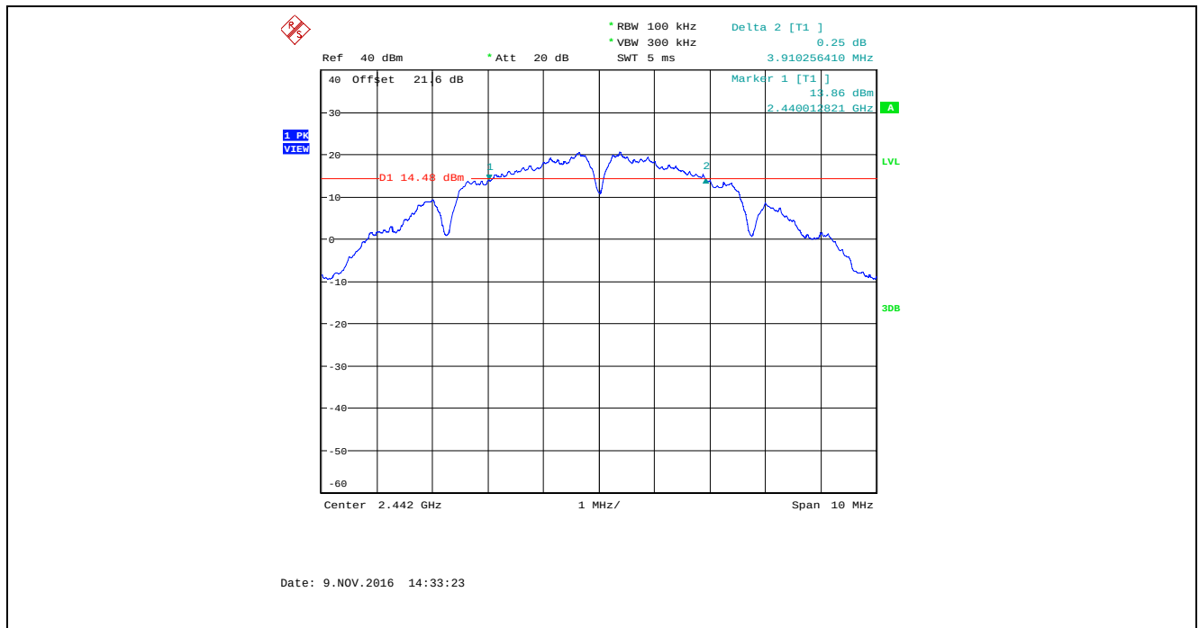
Plot 5.2.4.29. 6 dB Bandwidth, Bandwidth: 8 MHz, TX Gain: 50, Data Rate 2, 2442 MHz
