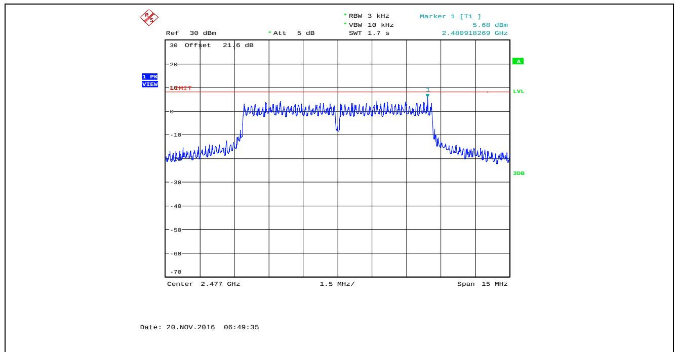
Plot 5.6.4.75. Power Spectral Density, Bandwidth: 8 MHz, TX Gain Setting: 55, Data Rate 5, 2477 MHz
