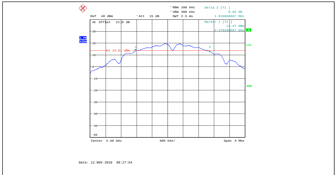
Plot 5.2.4.21. 6 dB Bandwidth, Bandwidth: 4 MHz, TX Gain: 43, Data Rate 2, 2480 MHz
