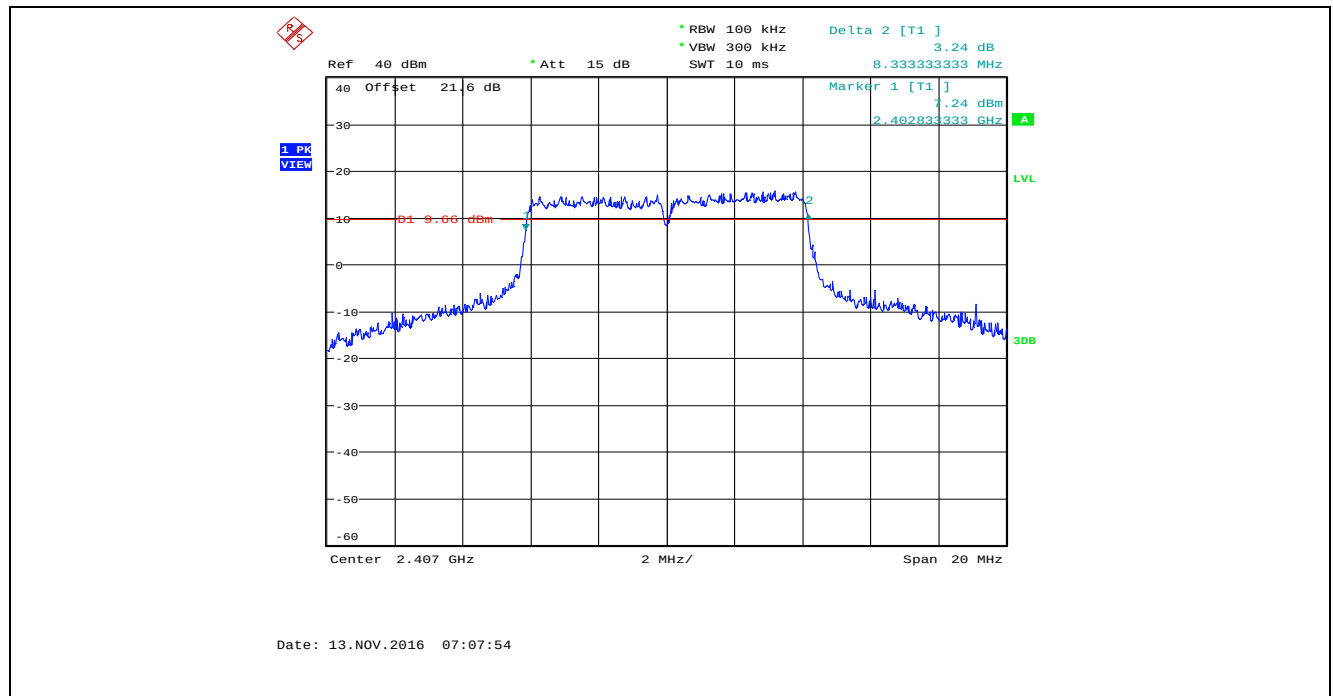
Plot 5.2.4.76. 6 dB Bandwidth, Bandwidth: 8 MHz, TX Gain: 55, Data Rate 6, 2407 MHz
