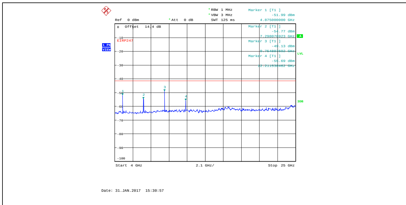
Plot 5.4.4.10. Conducted Spurious Emissions in Restricted Frequency Bands Bandwidth: 8 MHz, TX Gain Setting 25, Data Rate 1, 2442 MHz, 4 GHz - 25 GHz, Peak Detector
