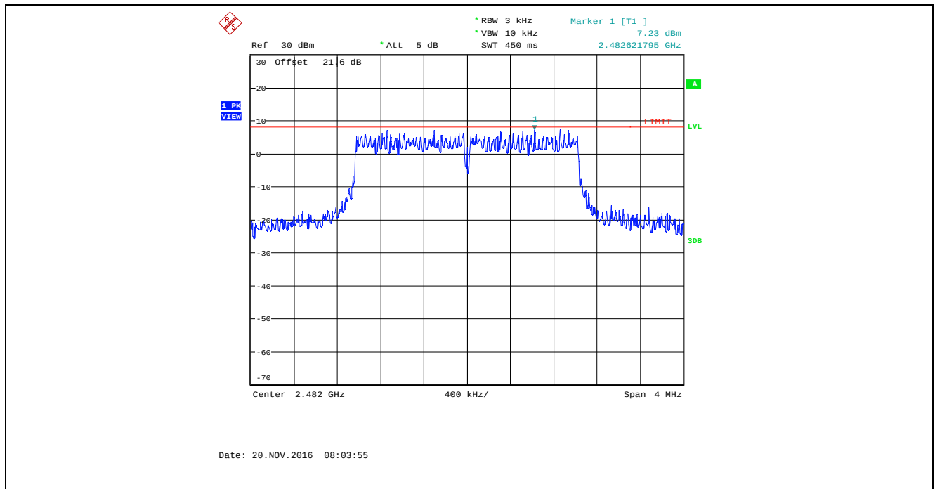
Plot 5.6.4.57. Power Spectral Density, Bandwidth: 2 MHz, TX Gain Setting: 45, Data Rate 7, 2482 MHz
