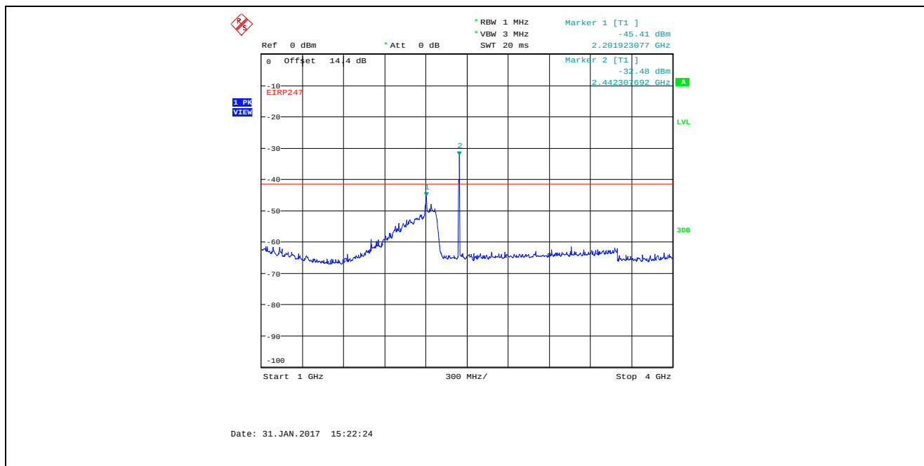
Plot 5.4.4.9. Conducted Spurious Emissions in Restricted Frequency Bands Bandwidth: 8 MHz, TX Gain Setting 25, Data Rate 1, 2442 MHz, 1 GHz - 4 GHz, Peak Detector Marker 2 is the Fundamental
