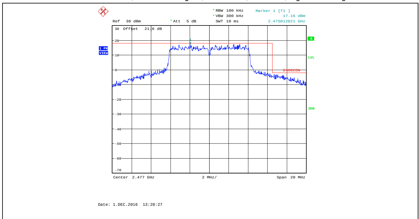
Plot 5.4.4.1.16. Band-Edge RF Conducted Emissions Bandwidth: 8 MHz, TX Gain Setting: 55, Data Rate 7, 2477 MHz, Higher Band-edge
