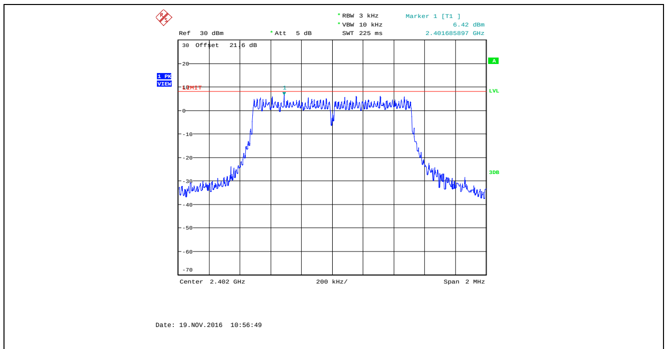
Plot 5.6.4.37. Power Spectral Density, Bandwidth: 1 MHz, TX Gain Setting: 43, Data Rate 5, 2402 MHz
