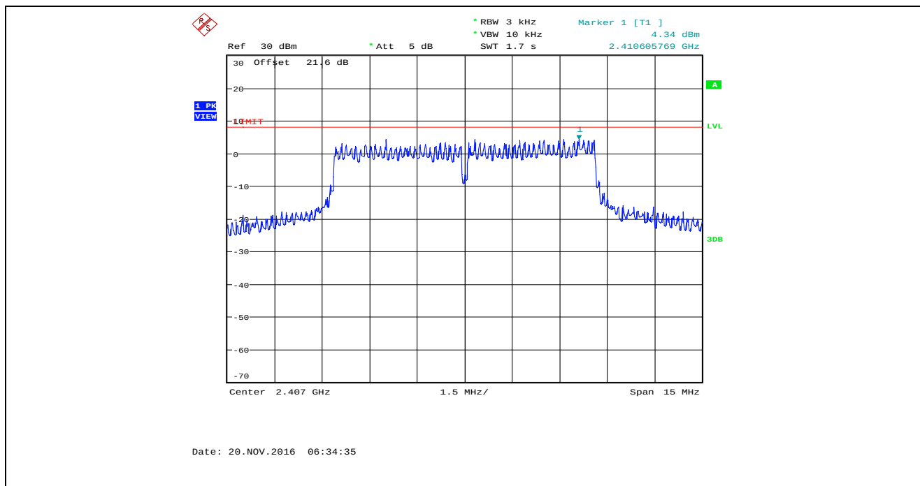
Plot 5.6.4.76. Power Spectral Density, Bandwidth: 8 MHz, TX Gain Setting: 55, Data Rate 6, 2407 MHz
