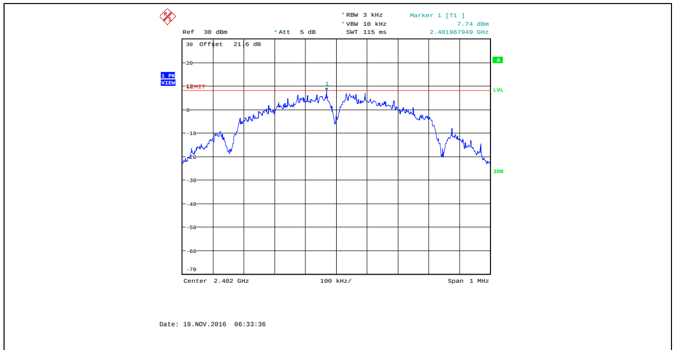
Plot 5.6.4.1. Power Spectral Density, Bandwidth: 1 MHz, TX Gain Setting: 26, Data Rate 1, 2402 MHz
