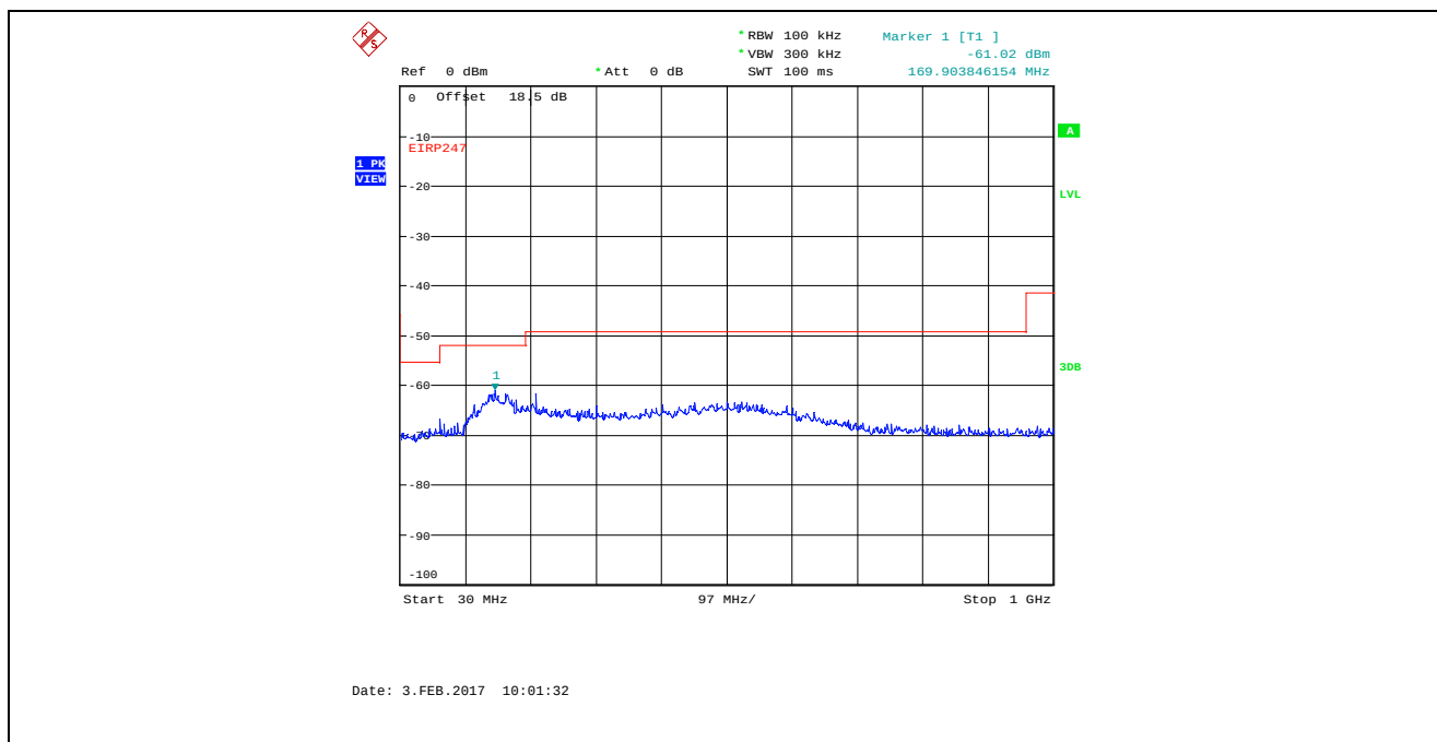
Plot 5.4.4.3.18. Conducted Spurious Emissions in Restricted Frequency Bands Bandwidth: 8 MHz, TX Gain Setting 55, Data Rate 4, 2407 MHz, 30 MHz - 1 GHz, Peak Detector
