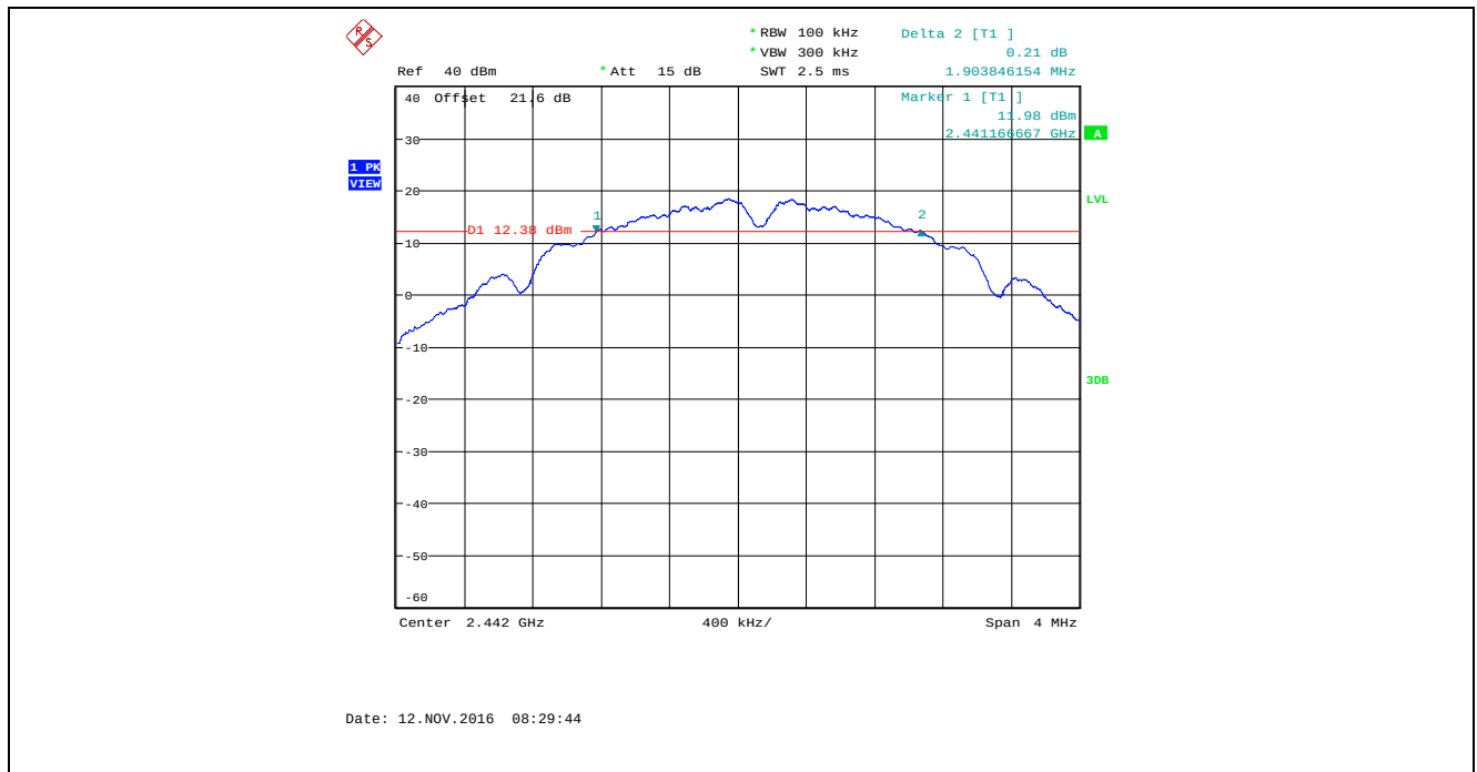
Plot 5.2.4.20. 6 dB Bandwidth, Bandwidth: 4 MHz, TX Gain: 43, Data Rate 2, 2442 MHz
