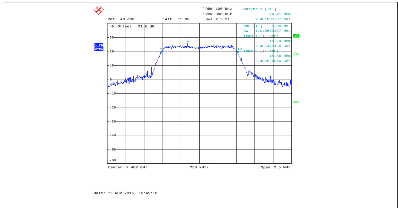
Plot 5.2.4.36. 6 dB Bandwidth, Bandwidth: 1 MHz, TX Gain: 43, Data Rate 4, 2482 MHz
