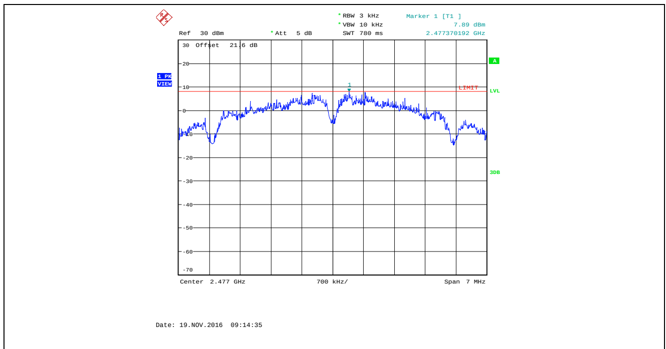
Plot 5.6.4.30. Power Spectral Density, Bandwidth: 8 MHz, TX Gain Setting: 50, Data Rate 2, 2477 MHz
