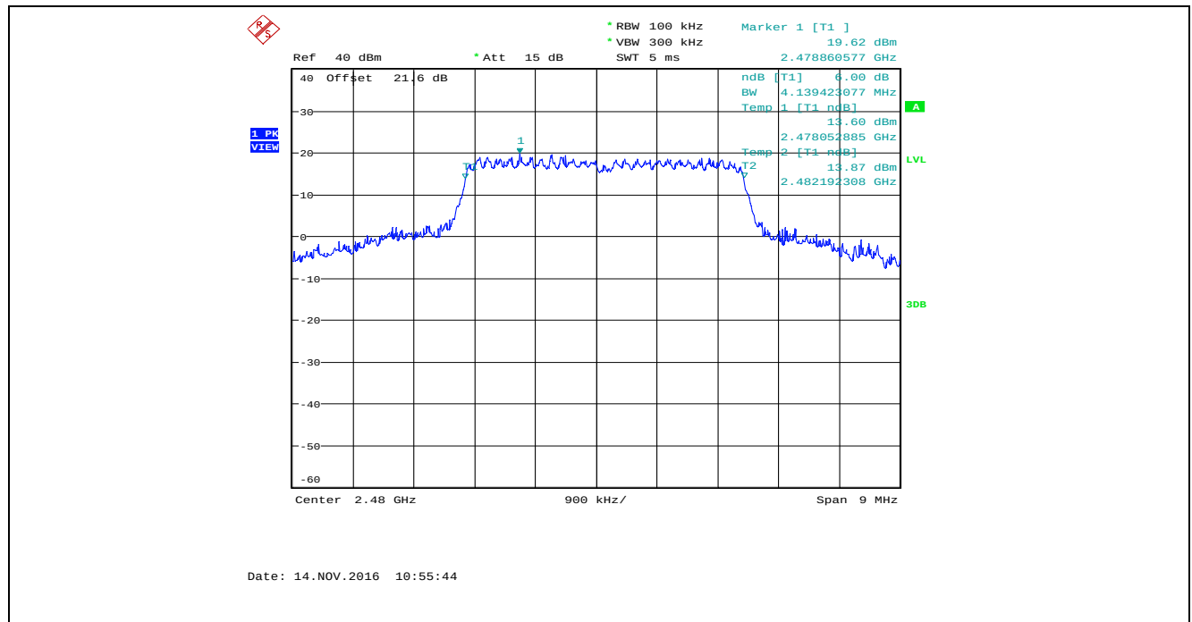
Plot 5.2.4.60. 6 dB Bandwidth, Bandwidth: 4 MHz, TX Gain: 50, Data Rate 4, 2480 MHz
