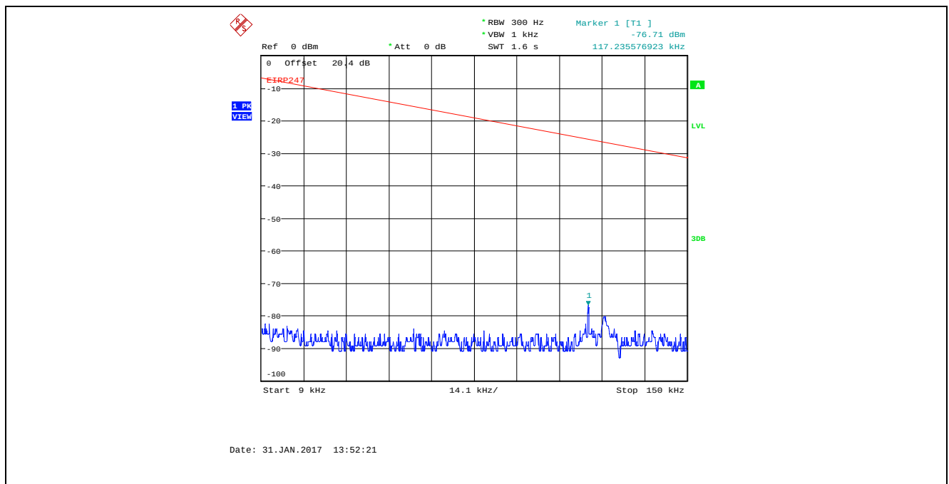
Plot 5.4.4.23. Conducted Spurious Emissions in Restricted Frequency Bands Bandwidth: 8 MHz, TX Gain Setting 25, Data Rate 4, 2442 MHz, 9 kHz - 150 kHz, Peak Detector
