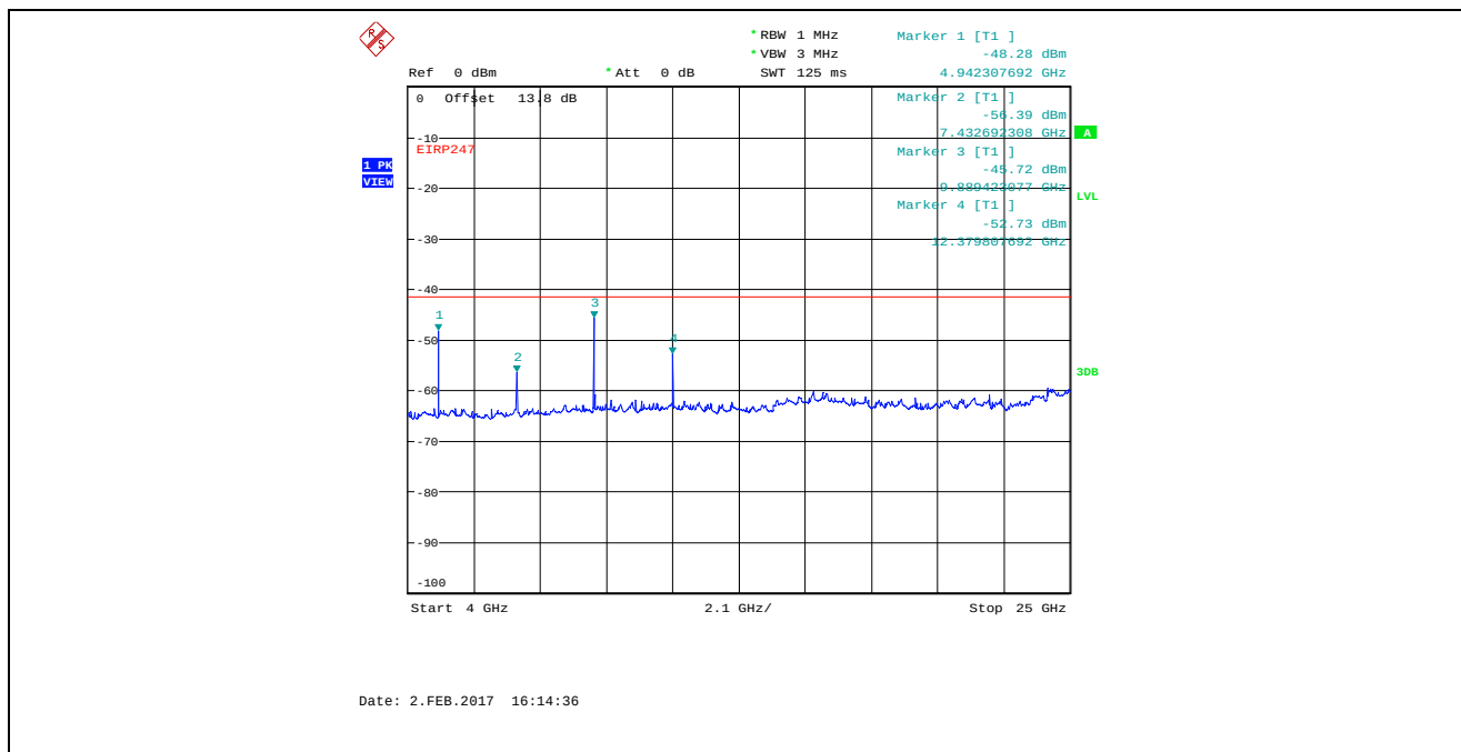
Plot 5.4.4.3.15. Conducted Spurious Emissions in Restricted Frequency Bands Bandwidth: 8 MHz, TX Gain Setting 50, Data Rate 1, 2477 MHz, 4 GHz - 25 GHz, Peak Detector
