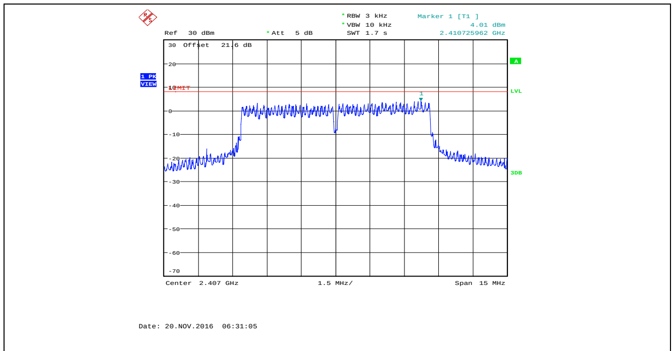
Plot 5.6.4.79. Power Spectral Density, Bandwidth: 8 MHz, TX Gain Setting: 55, Data Rate 7, 2407 MHz
