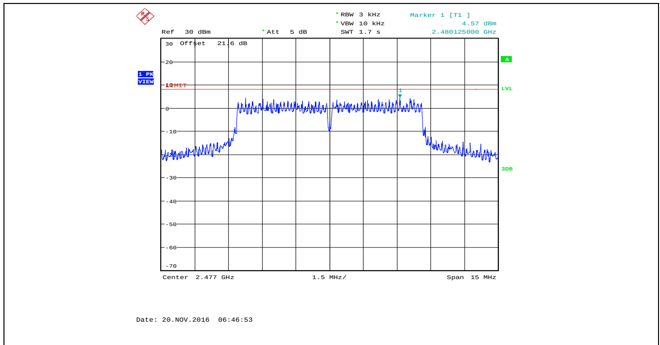
Plot 5.6.4.78. Power Spectral Density, Bandwidth: 8 MHz, TX Gain Setting: 55, Data Rate 6, 2477 MHz
