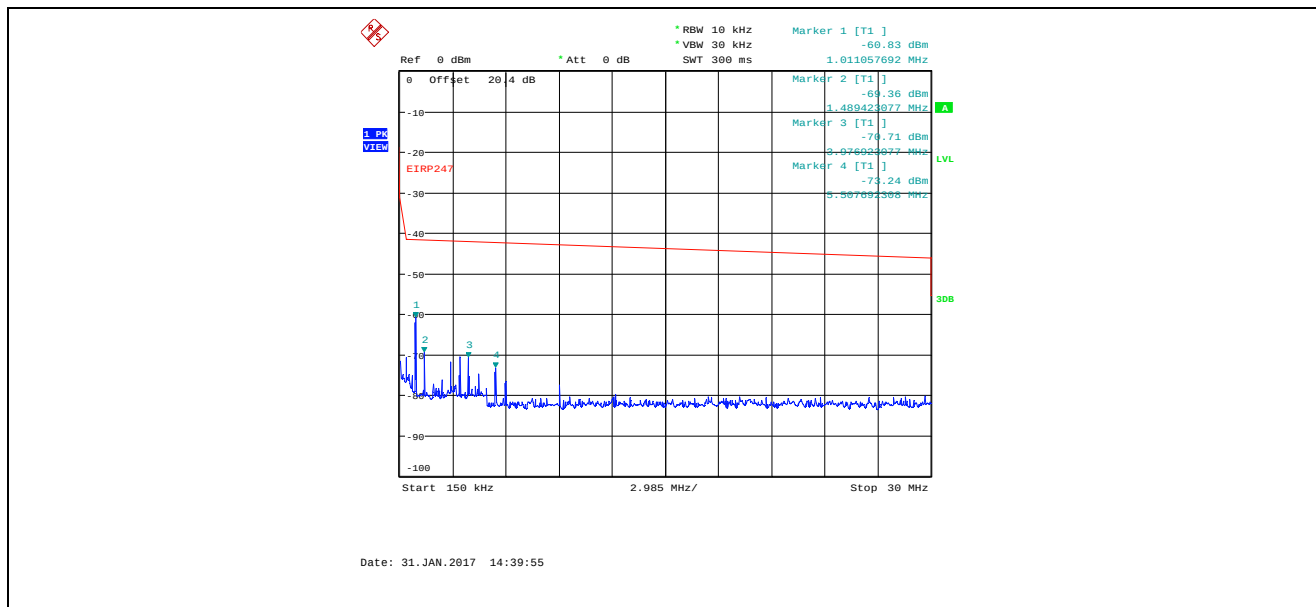
Plot 5.4.4.4.2. Conducted Spurious Emissions in Restricted Frequency Bands Bandwidth: 8 MHz, TX Gain Setting 25, Data Rate 1, 2407 MHz, 150 kHz - 30 MHz, Peak Detector
