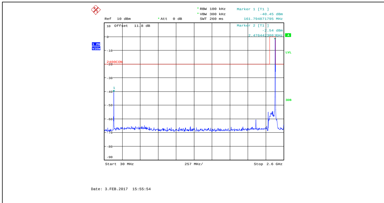
Plot 5.4.4.2.17. Conducted Spurious Emissions in Non-restricted Frequency Bands Bandwidth: 8 MHz, TX Gain: 0, Data Rate 1, 2477 MHz, 30 MHz – 2.6 GHz
