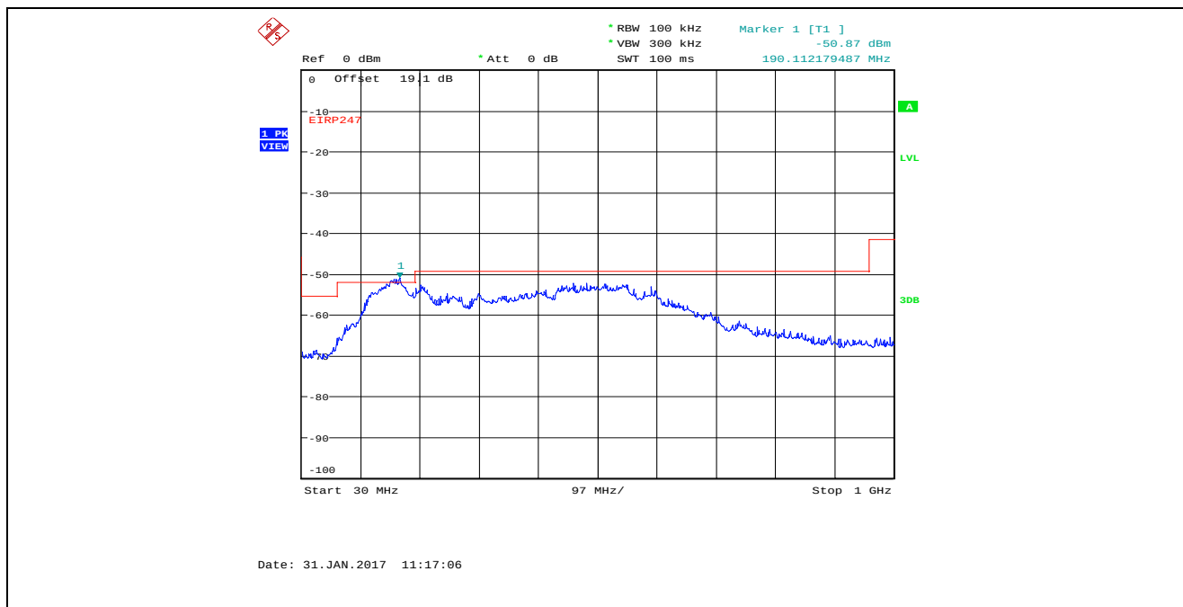
Plot 5.4.4.25. Conducted Spurious Emissions in Restricted Frequency Bands Bandwidth: 8 MHz, TX Gain Setting 25, Data Rate 4, 2442 MHz, 30 MHz - 1 GHz, Peak Detector
