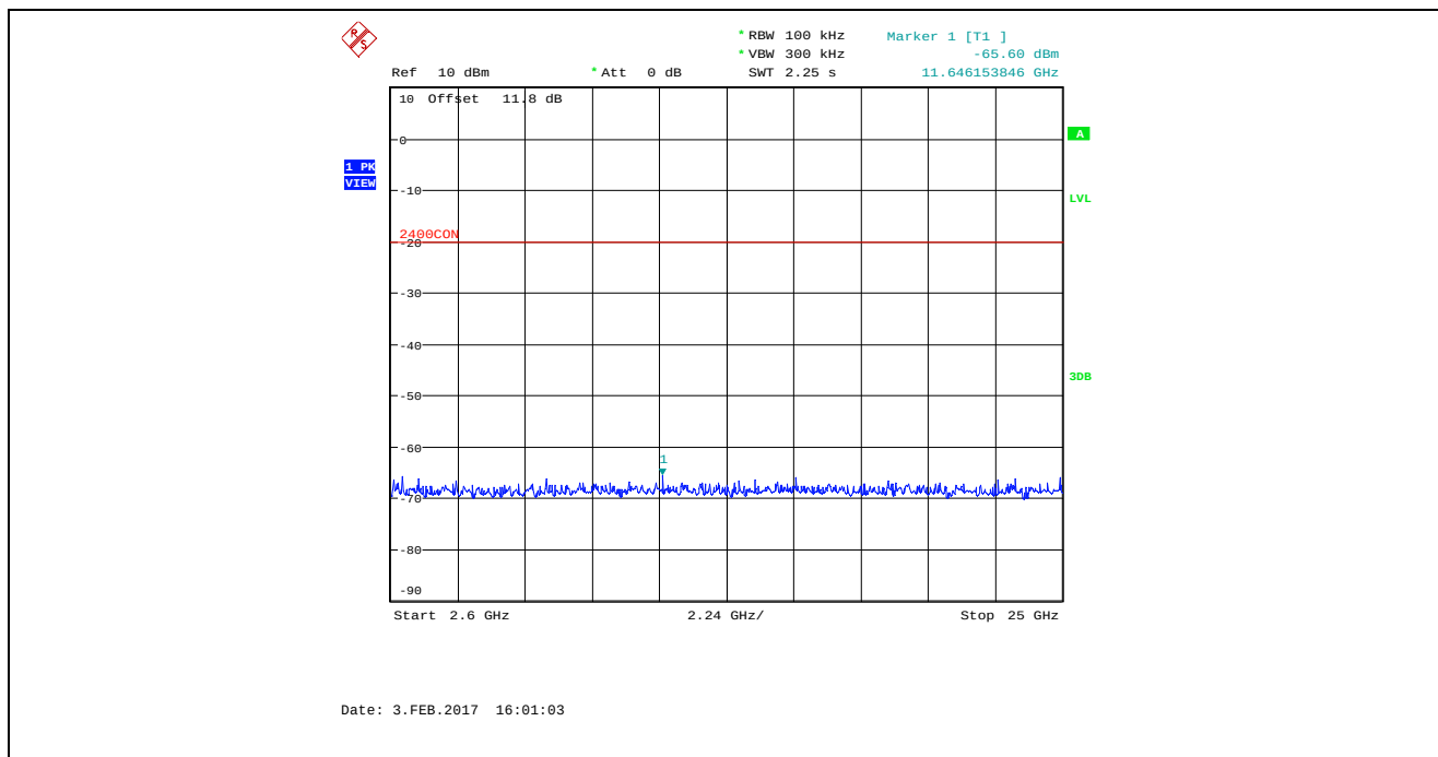
Plot 5.4.4.2.16. Conducted Spurious Emissions in Non-restricted Frequency Bands Bandwidth: 8 MHz, TX Gain: 0, Data Rate 1, 2442 MHz, 2.6 GHz – 25 GHz
