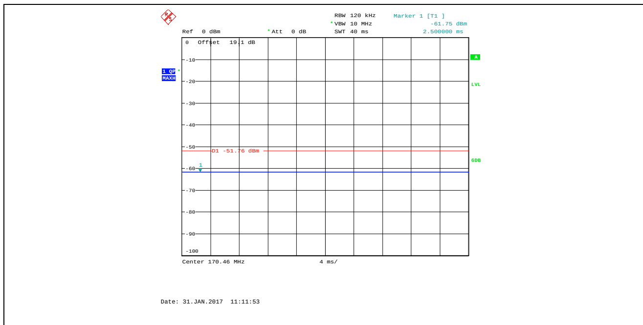
Plot 5.4.4.4.20. Conducted Spurious Emissions in Restricted Frequency Bands Bandwidth: 8 MHz, TX Gain Setting 25, Data Rate 4, 2407 MHz, RB 167.72-173.2 MHz, QP Detector QP at 170.44 MHz (RB 167.72-173.2 MHz) is -61.62dBm (limit is -51.76dBm)
