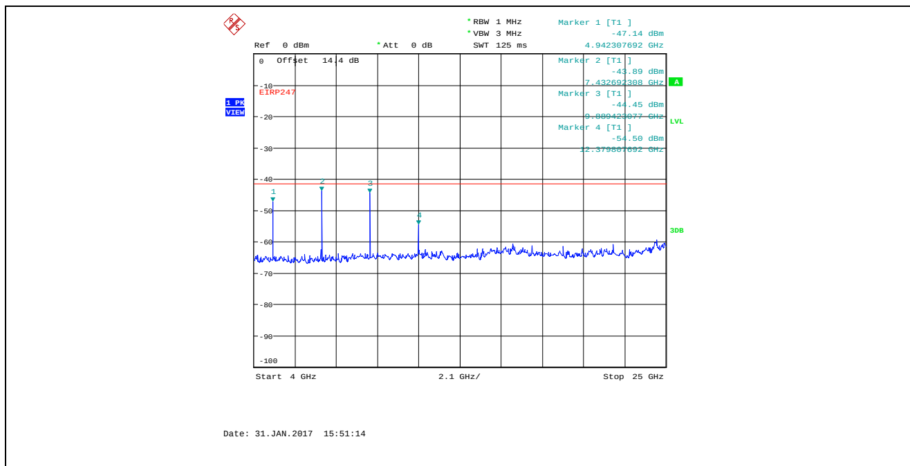
Plot 5.4.4.4.15. Conducted Spurious Emissions in Restricted Frequency Bands Bandwidth: 8 MHz, TX Gain Setting 25, Data Rate 1, 2477 MHz, 4 GHz - 25 GHz, Peak Detector
