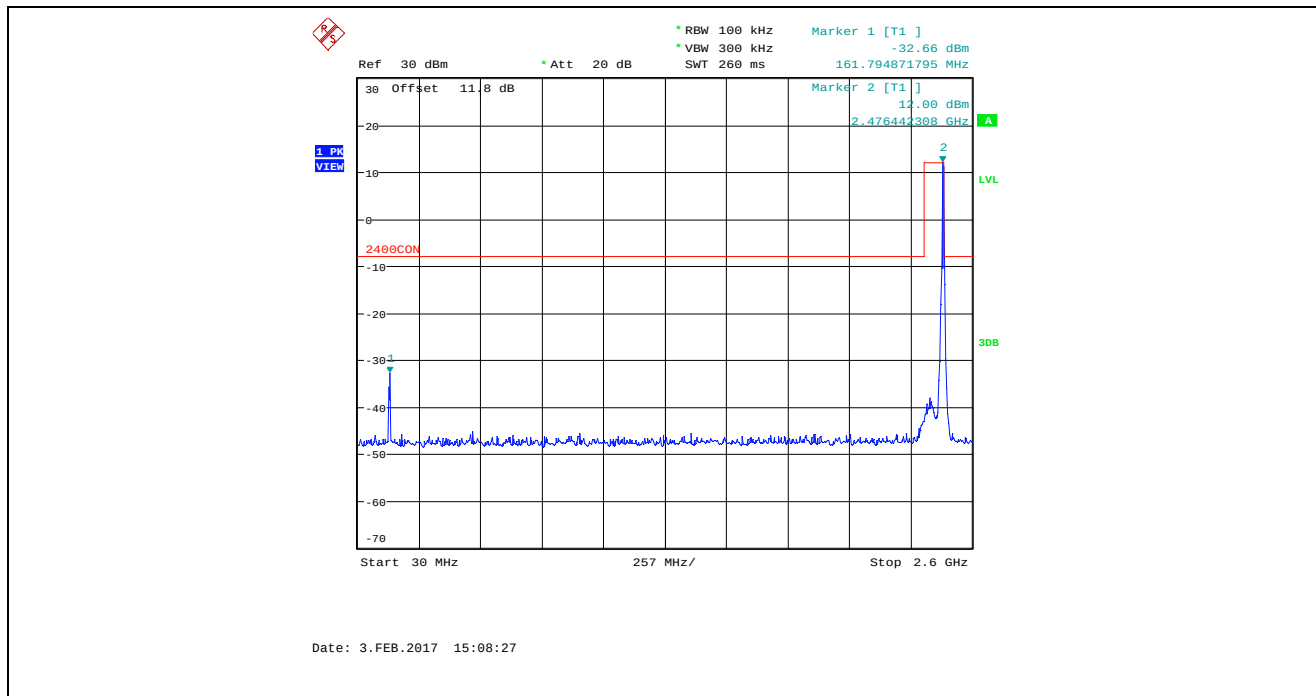
Plot 5.4.4.2.11. Conducted Spurious Emissions in Non-restricted Frequency Bands Bandwidth: 8 MHz, TX Gain: 55, Data Rate 4, 2477 MHz, 30 MHz – 2.6 GHz
