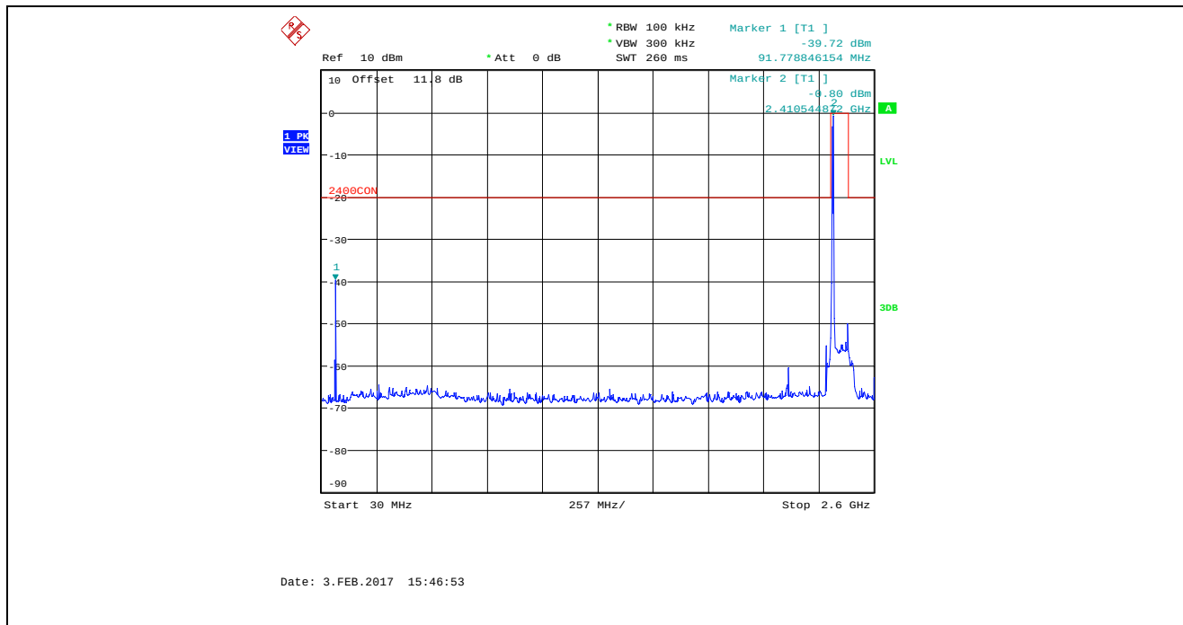
Plot 5.4.4.2.13. Conducted Spurious Emissions in Non-restricted Frequency Bands Bandwidth: 8 MHz, TX Gain: 0, Data Rate 1, 2407 MHz, 30 MHz – 2.6 GHz
