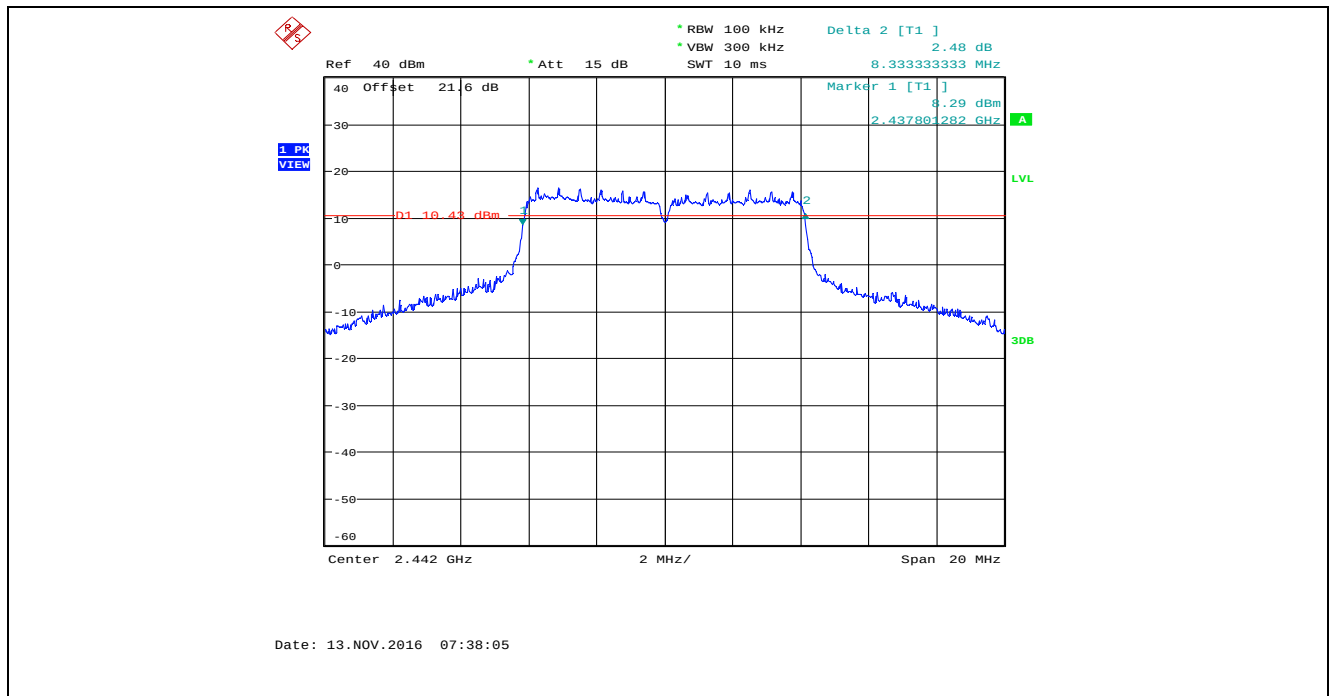
Plot 5.2.4.74. 6 dB Bandwidth, Bandwidth: 8 MHz, TX Gain: 55, Data Rate 5, 2442 MHz
