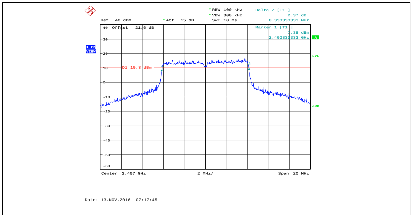
Plot 5.2.4.73. 6 dB Bandwidth, Bandwidth: 8 MHz, TX Gain: 55, Data Rate 5, 2407 MHz
