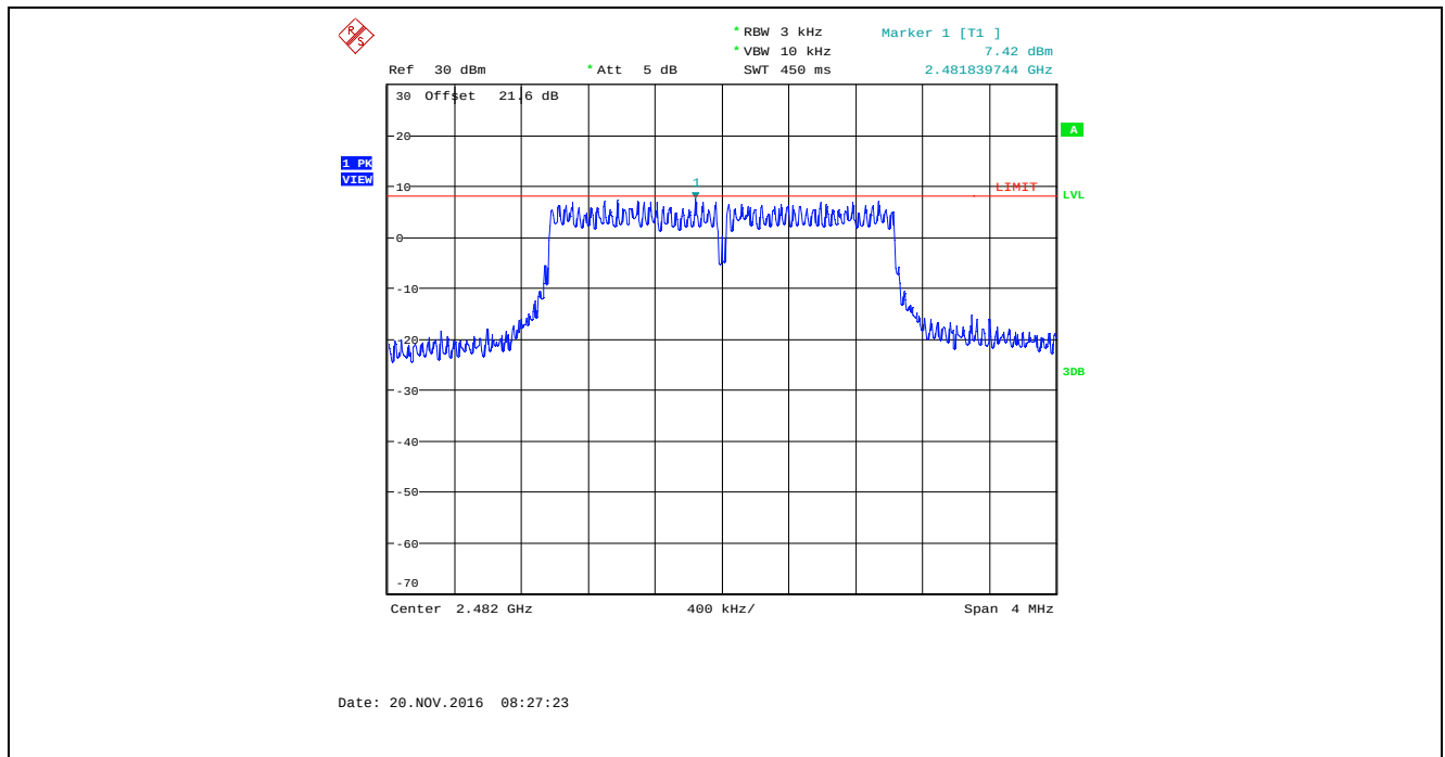
Plot 5.6.4.54. Power Spectral Density, Bandwidth: 2 MHz, TX Gain Setting: 45, Data Rate 6, 2482 MHz
