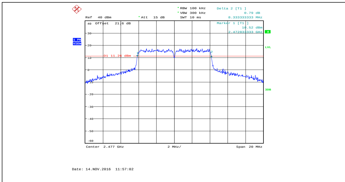
Plot 5.2.4.78. 6 dB Bandwidth, Bandwidth: 8 MHz, TX Gain: 55, Data Rate 6, 2477 MHz
