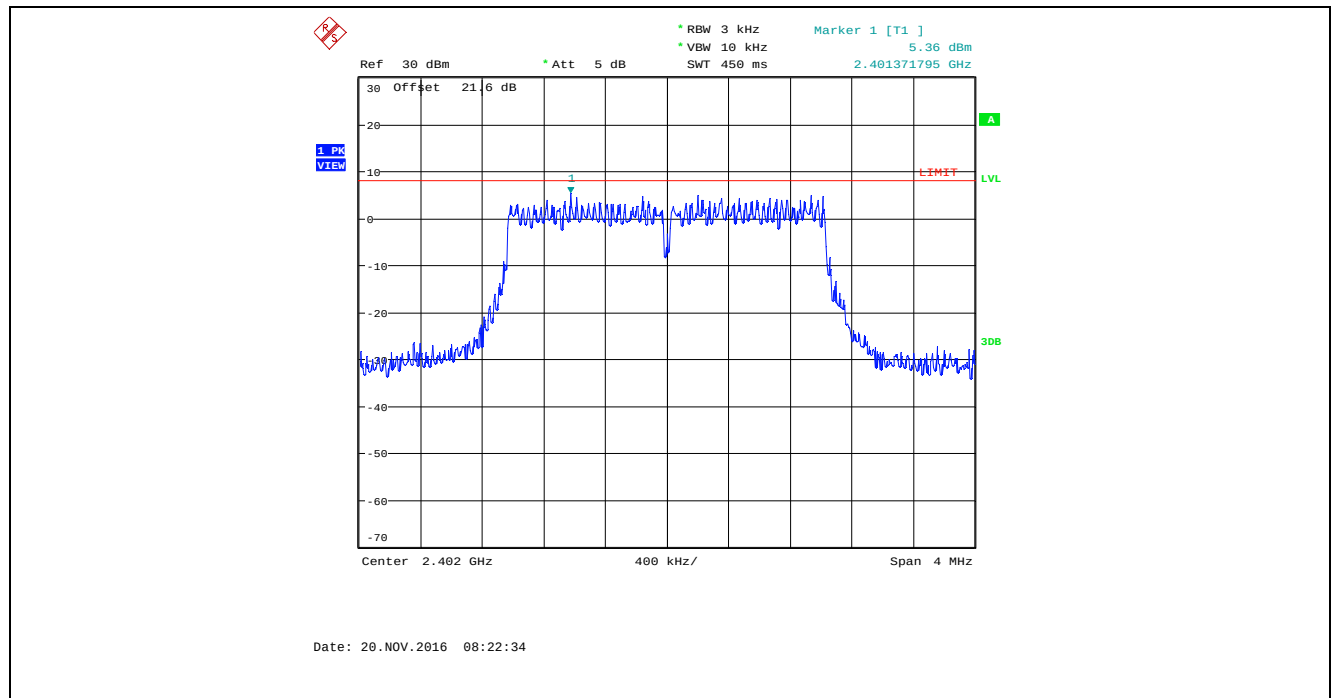
Plot 5.6.4.52. Power Spectral Density, Bandwidth: 2 MHz, TX Gain Setting: 45, Data Rate 6, 2402 MHz
