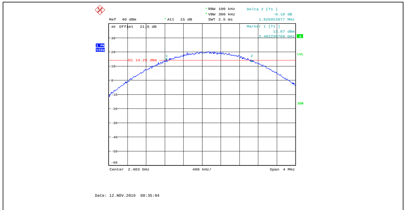
Plot 5.2.4.22. 6 dB Bandwidth, Bandwidth: 4 MHz, TX Gain: 43, Data Rate 3, 2403 MHz
