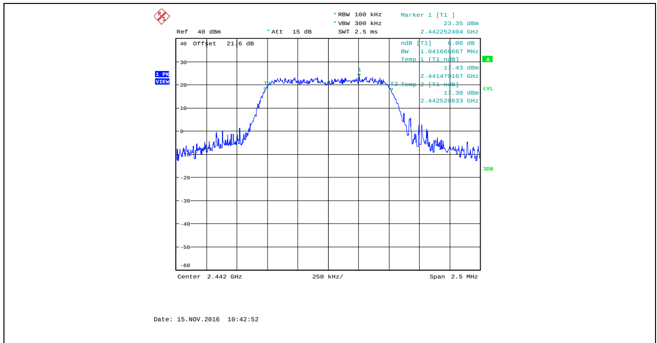
Plot 5.2.4.35. 6 dB Bandwidth, Bandwidth: 1 MHz, TX Gain: 43, Data Rate 4, 2442 MHz
