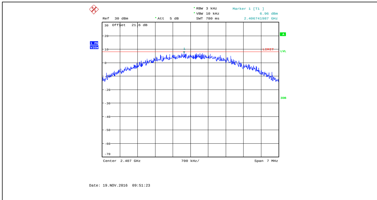
Plot 5.6.4.31. Power Spectral Density, Bandwidth: 8 MHz, TX Gain Setting: 50, Data Rate 3, 2407 MHz
