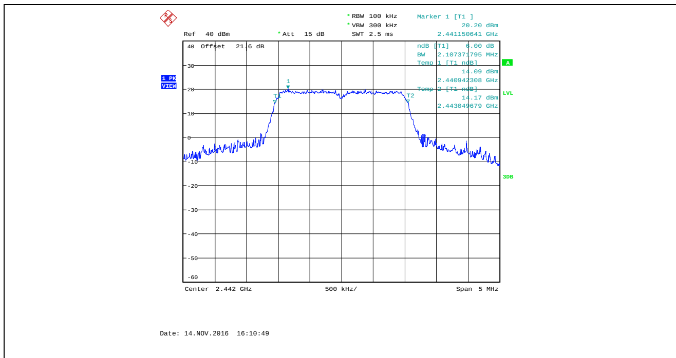
Plot 5.2.4.47. 6 dB Bandwidth, Bandwidth: 2 MHz, TX Gain: 45, Data Rate 4, 2442 MHz
