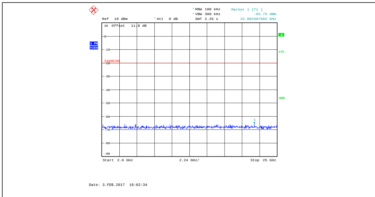
Plot 5.4.4.2.14. Conducted Spurious Emissions in Non-restricted Frequency Bands Bandwidth: 8 MHz, TX Gain: 0, Data Rate 1, 2407 MHz, 2.6 GHz – 25 GHz
