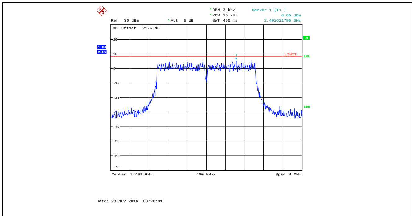
Plot 5.6.4.55. Power Spectral Density, Bandwidth: 2 MHz, TX Gain Setting: 45, Data Rate 7, 2402 MHz
