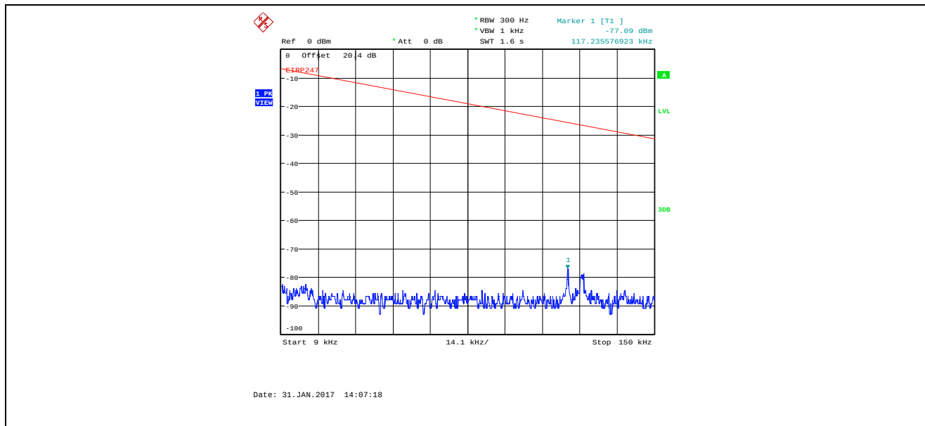
Plot 5.4.4.4.1. Conducted Spurious Emissions in Restricted Frequency Bands Bandwidth: 8 MHz, TX Gain Setting 25, Data Rate 1, 2407 MHz, 9 kHz - 150 kHz, Peak Detector
