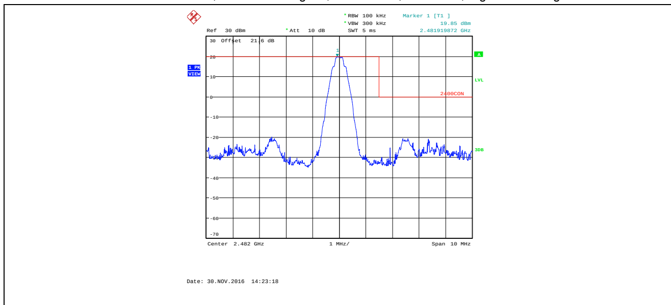
Plot 5.4.4.1.2. Band-Edge RF Conducted Emissions
