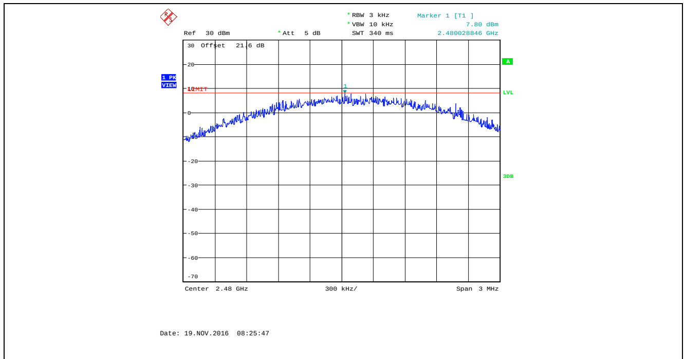
Plot 5.6.4.24. Power Spectral Density, Bandwidth: 4 MHz, TX Gain Setting: 43, Data Rate 3, 2480 MHz
