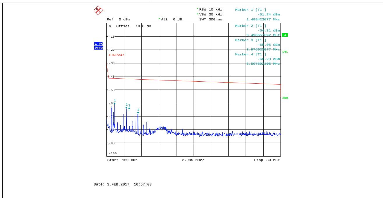
Plot 5.4.4.3.12. Conducted Spurious Emissions in Restricted Frequency Bands Bandwidth: 8 MHz, TX Gain Setting 50, Data Rate 1, 2477 MHz, 150 kHz - 30 MHz, Peak Detector
