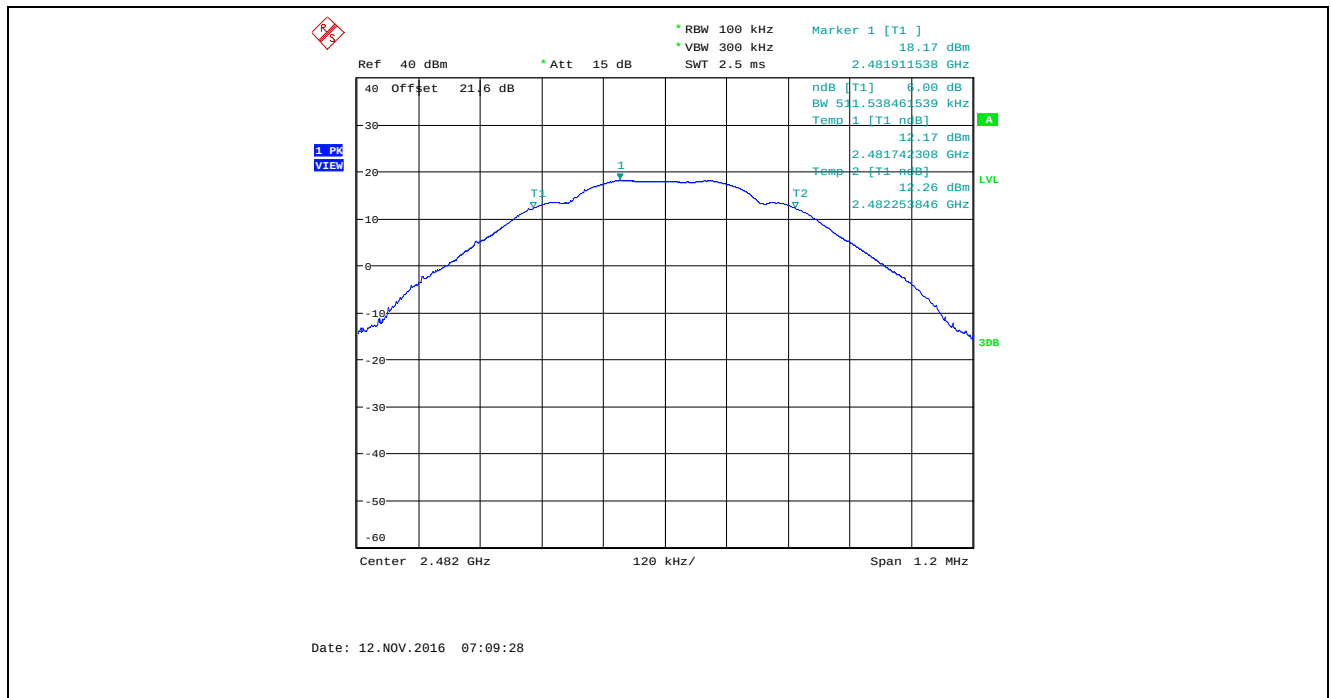
Plot 5.2.4.3. 6 dB Bandwidth, Bandwidth: 1 MHz, TX Gain: 26, Data Rate 1, 2482 MHz
