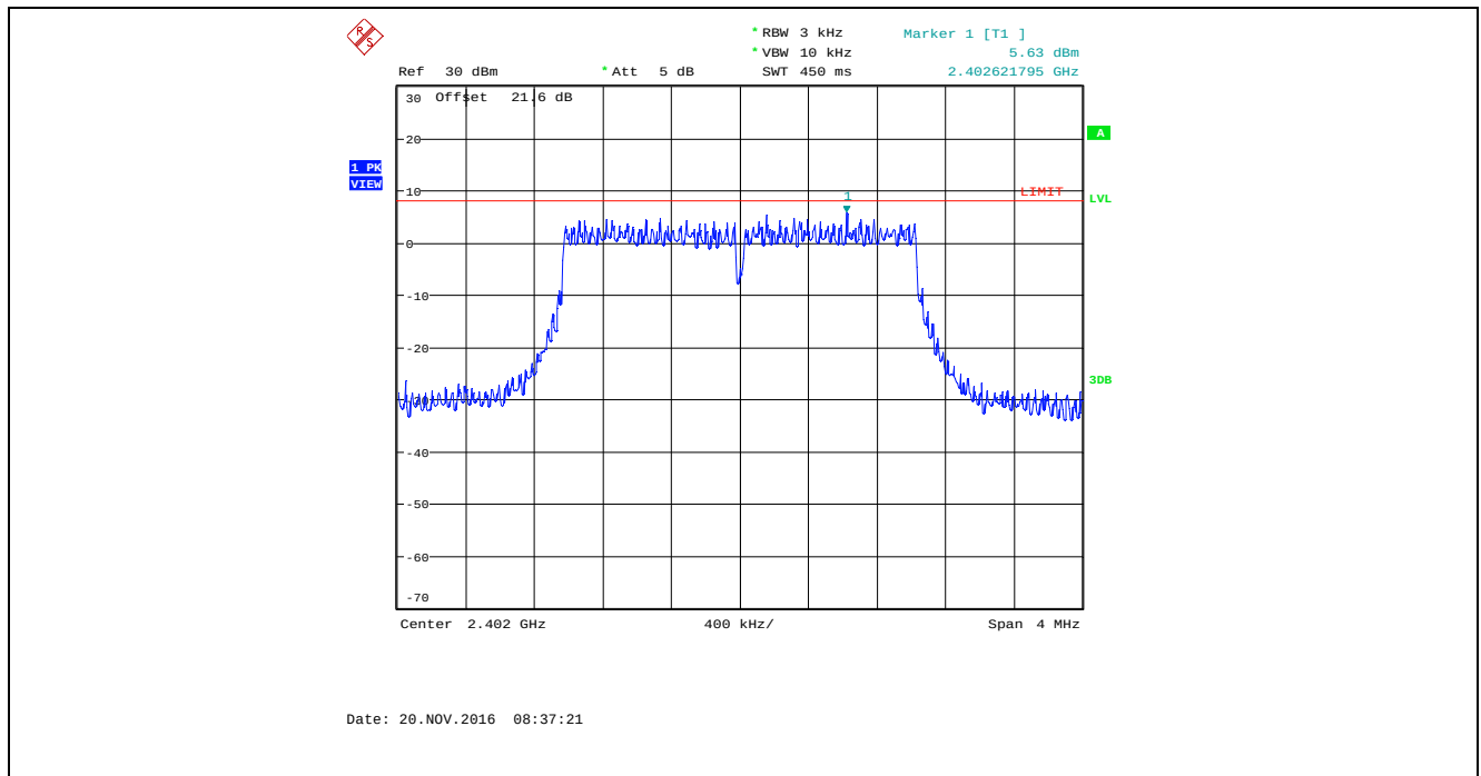
Plot 5.6.4.46. Power Spectral Density, Bandwidth: 2 MHz, TX Gain Setting: 45, Data Rate 4, 2402 MHz
