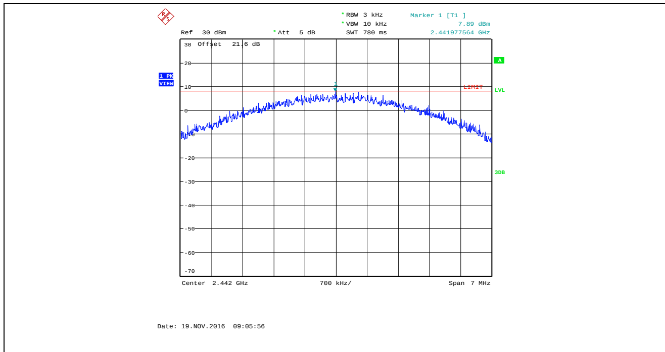
Plot 5.6.4.32. Power Spectral Density, Bandwidth: 8 MHz, TX Gain Setting: 50, Data Rate 3, 2442 MHz
