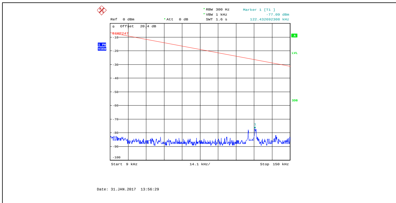
Plot 5.4.4.4.30. Conducted Spurious Emissions in Restricted Frequency Bands Bandwidth: 8 MHz, TX Gain Setting 25, Data Rate 4, 2477 MHz, 9 kHz - 150 kHz, Peak Detector
