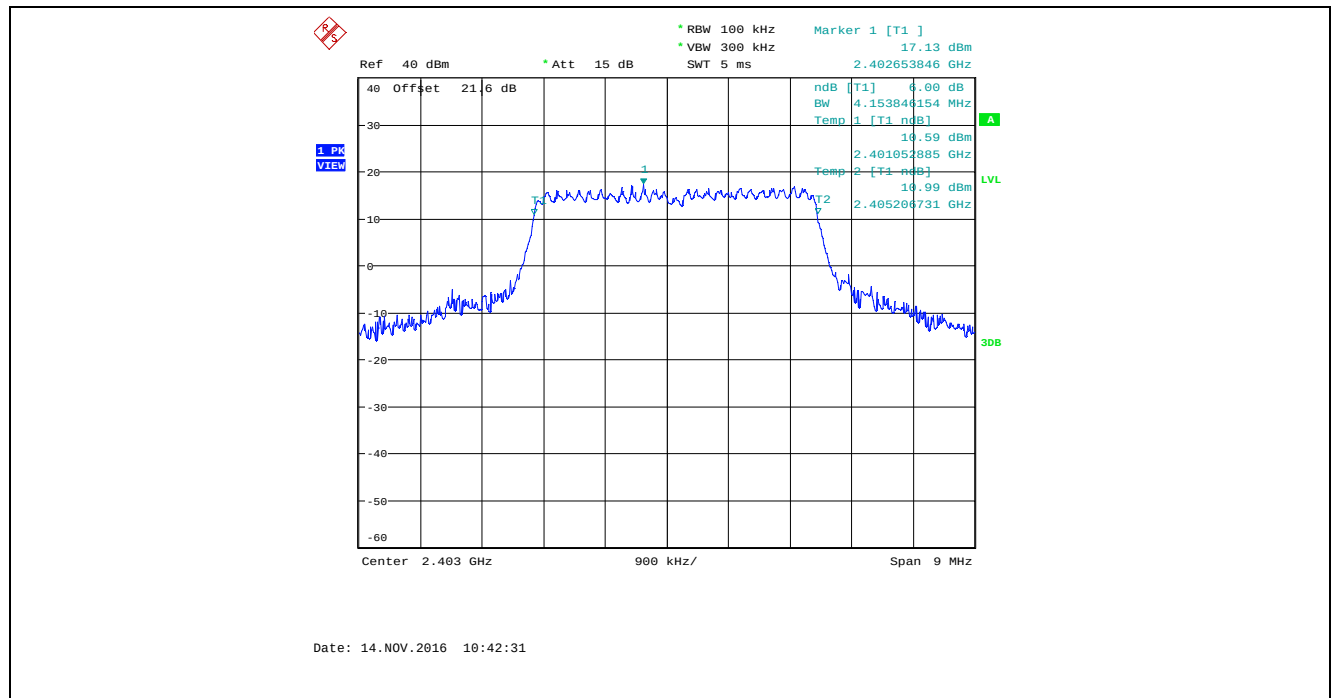
Plot 5.2.4.58. 6 dB Bandwidth, Bandwidth: 4 MHz, TX Gain: 50, Data Rate 4, 2403 MHz
