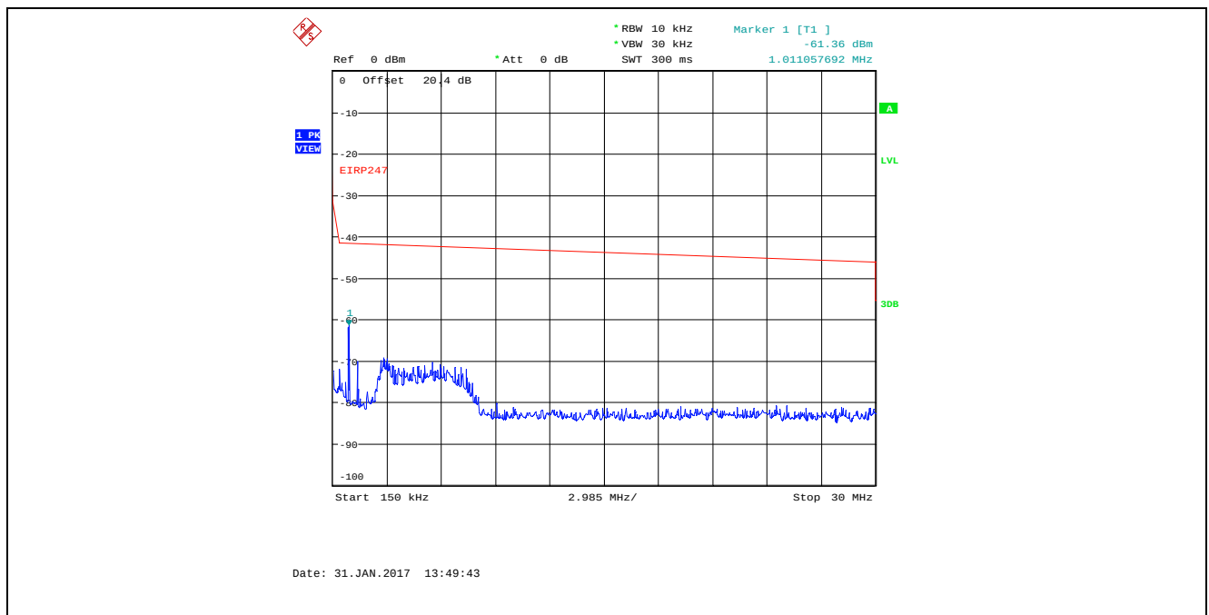
Plot 5.4.4.24. Conducted Spurious Emissions in Restricted Frequency Bands Bandwidth: 8 MHz, TX Gain Setting 25, Data Rate 4, 2442 MHz, 150 kHz - 30 MHz, Peak Detector
