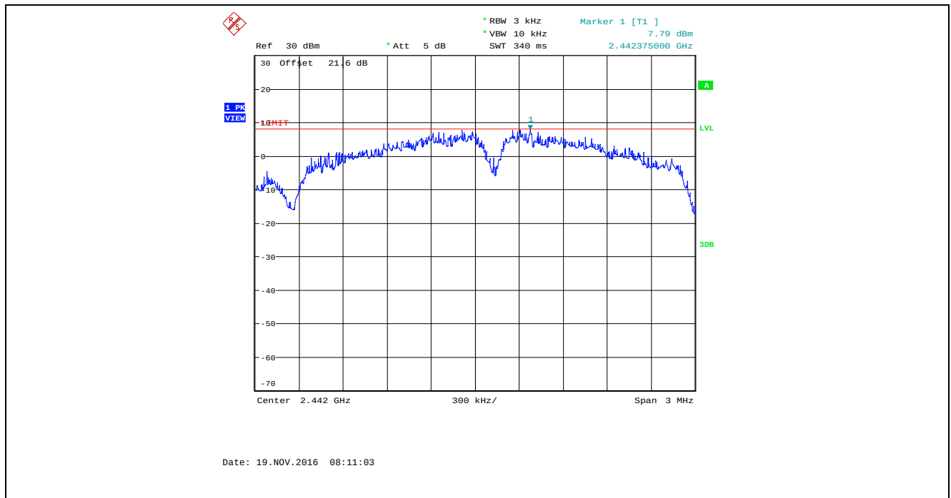
Plot 5.6.4.17. Power Spectral Density, Bandwidth: 4 MHz, TX Gain Setting: 43, Data Rate 1, 2442 MHz
