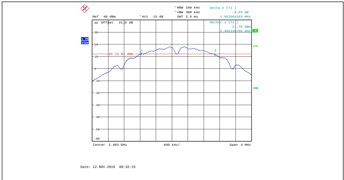
Plot 5.2.4.19. 6 dB Bandwidth, Bandwidth: 4 MHz, TX Gain: 43, Data Rate 2, 2403 MHz
