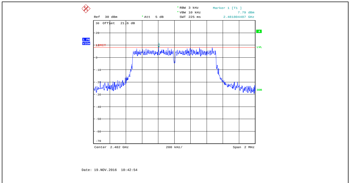
Plot 5.6.4.36. Power Spectral Density, Bandwidth: 1 MHz, TX Gain Setting: 43, Data Rate 4, 2482 MHz
