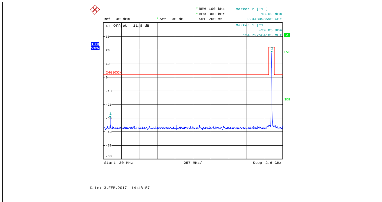
Plot 5.4.4.2.3. Conducted Spurious Emissions in Non-restricted Frequency Bands Bandwidth: 8 MHz, TX Gain: 50, Data Rate 1, 2442 MHz, 30 MHz – 2.6 GHz
