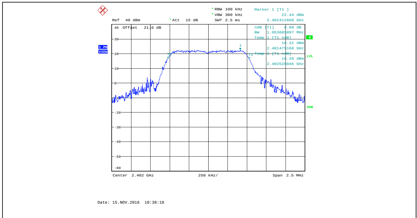
Plot 5.2.4.34. 6 dB Bandwidth, Bandwidth: 1 MHz, TX Gain: 43, Data Rate 4, 2402 MHz
