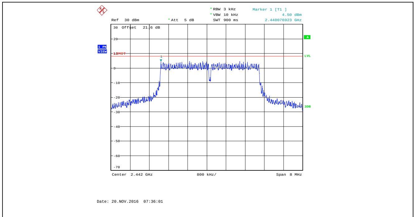
Plot 5.6.4.62. Power Spectral Density, Bandwidth: 4 MHz, TX Gain Setting: 50, Data Rate 5, 2442 MHz
