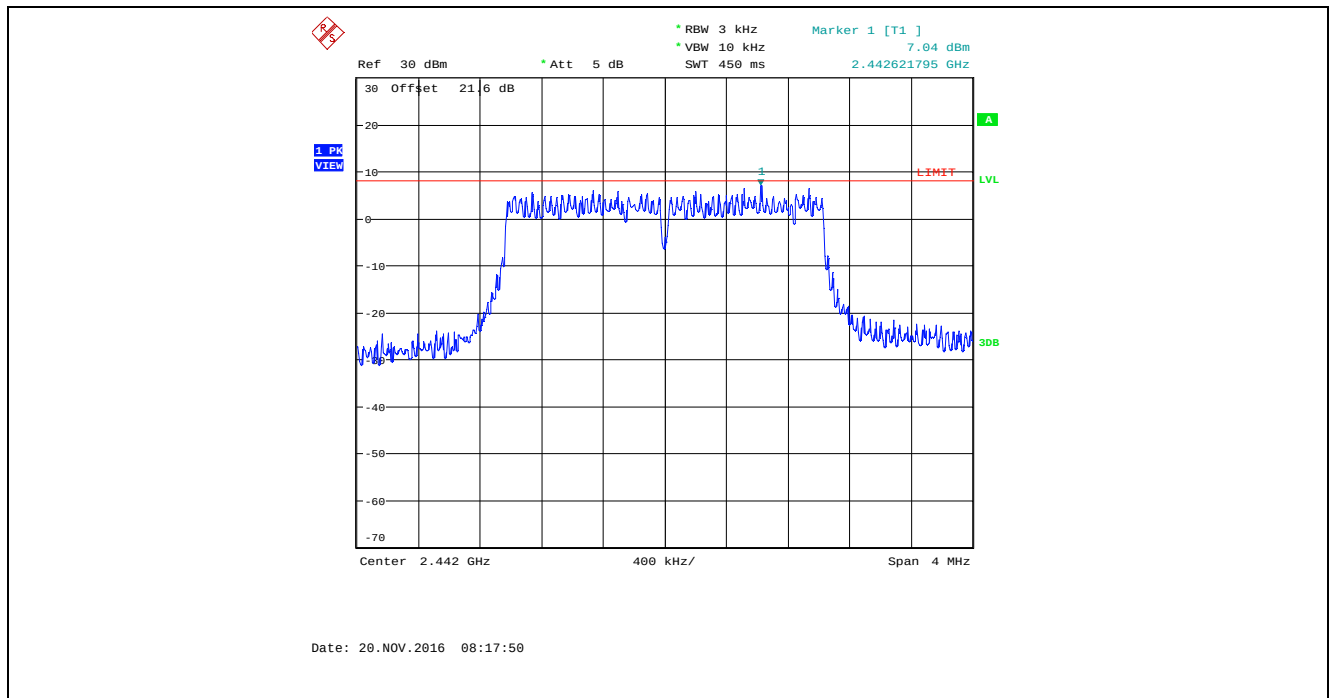
Plot 5.6.4.56. Power Spectral Density, Bandwidth: 2 MHz, TX Gain Setting: 45, Data Rate 7, 2442 MHz
