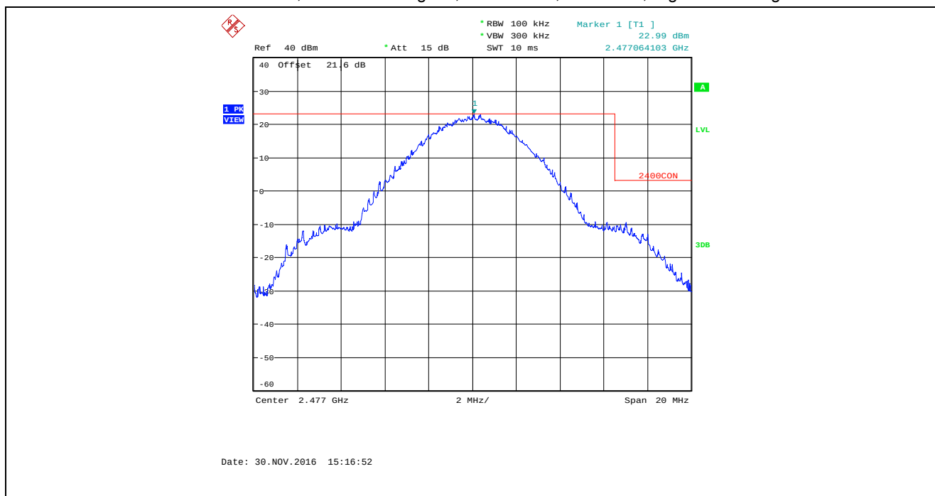
Plot 5.4.4.1.8. Band-Edge RF Conducted Emissions Bandwidth: 8 MHz, TX Gain Setting: 50, Data Rate 3, 2477 MHz, Higher Band-edge
