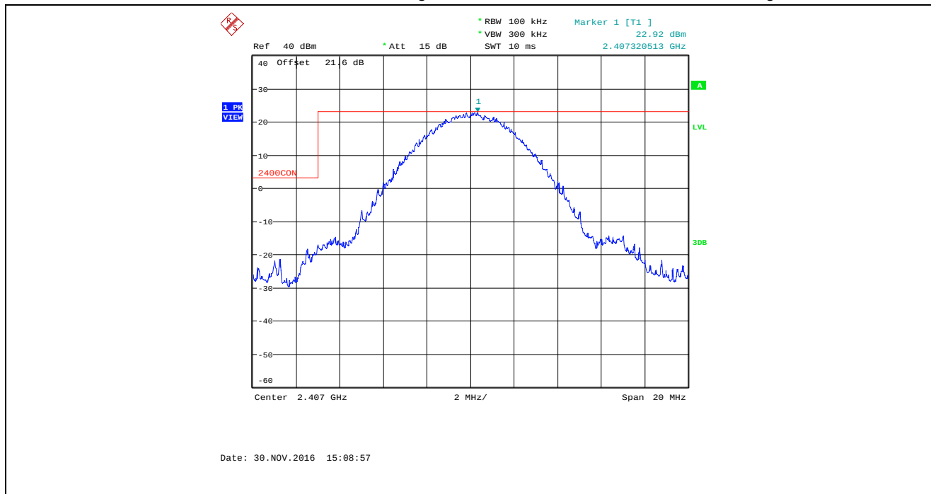
Plot 5.4.4.1.7. Band-Edge RF Conducted Emissions Bandwidth: 8 MHz, TX Gain Setting: 50, Data Rate 3, 2407 MHz, Lower Band-edge
