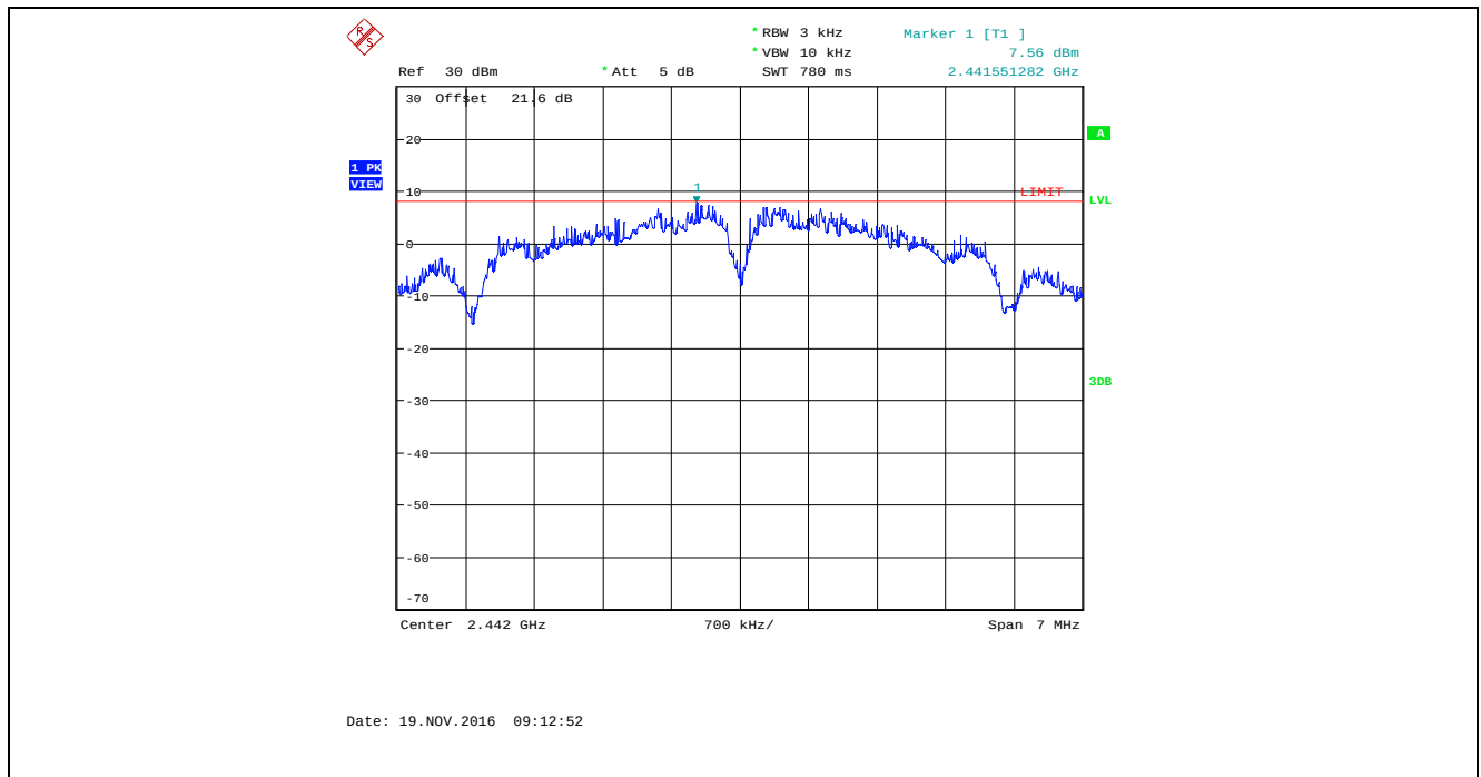
Plot 5.6.4.29. Power Spectral Density, Bandwidth: 8 MHz, TX Gain Setting: 50, Data Rate 2, 2442 MHz
