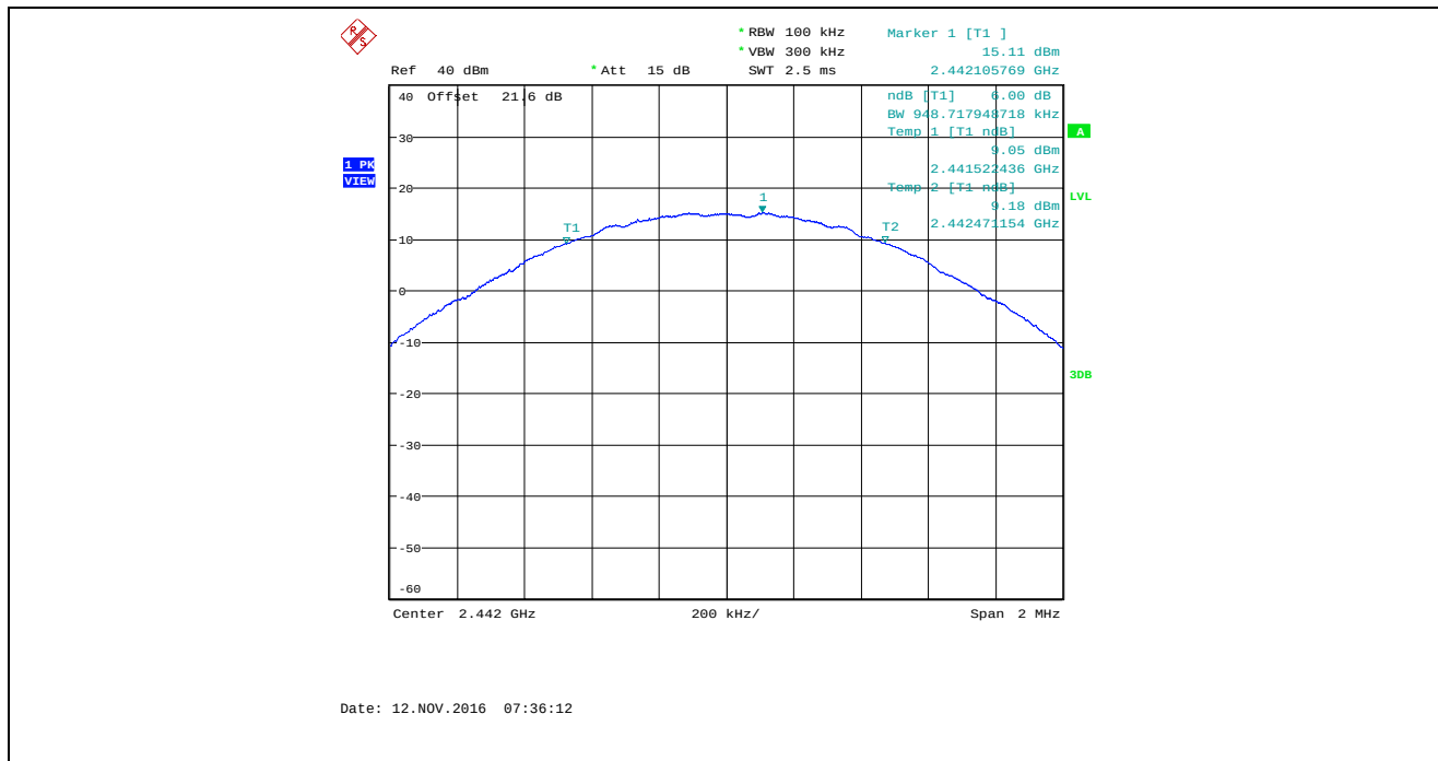
Plot 5.2.4.8. 6 dB Bandwidth, Bandwidth: 2 MHz, TX Gain: 32, Data Rate 1, 2442 MHz
