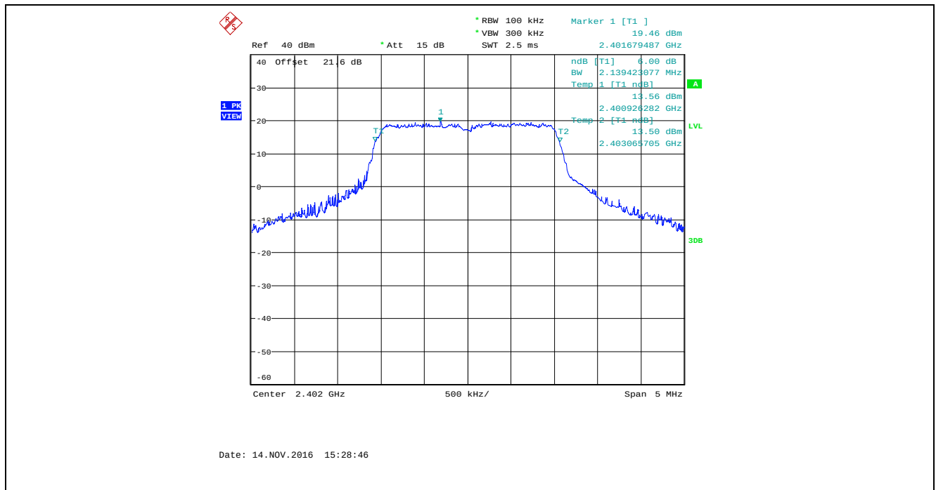
Plot 5.2.4.52. 6 dB Bandwidth, Bandwidth: 2 MHz, TX Gain: 45, Data Rate 6, 2402 MHz
