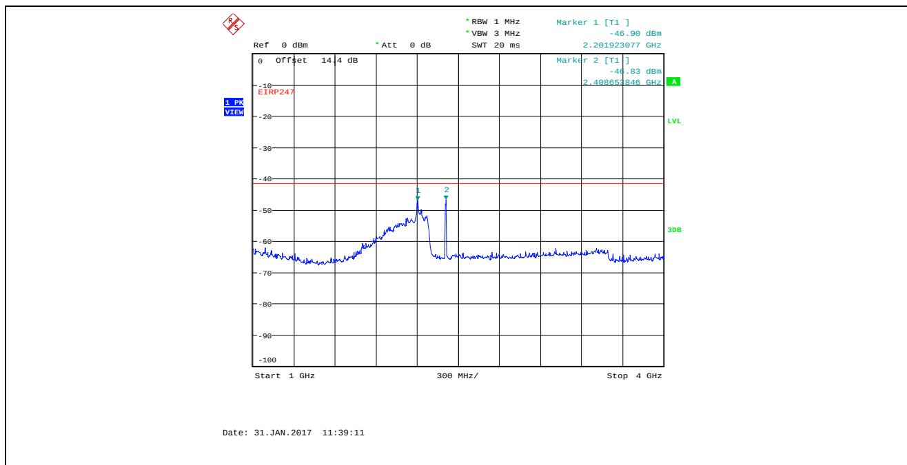
Plot 5.4.4.4.21. Conducted Spurious Emissions in Restricted Frequency Bands Bandwidth: 8 MHz, TX Gain Setting 25, Data Rate 4, 2407 MHz, 1 GHz - 4 GHz, Peak Detector
