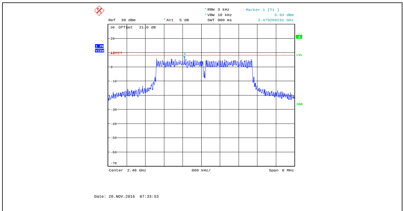
Plot 5.6.4.63. Power Spectral Density, Bandwidth: 4 MHz, TX Gain Setting: 50, Data Rate 5, 2480 MHz
