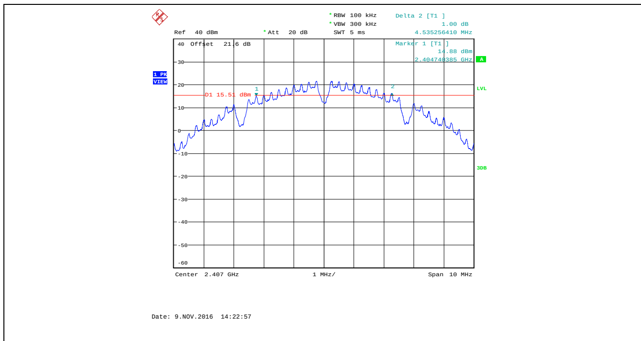
Plot 5.2.4.25. 6 dB Bandwidth, Bandwidth: 8 MHz, TX Gain: 50, Data Rate 1, 2407 MHz
