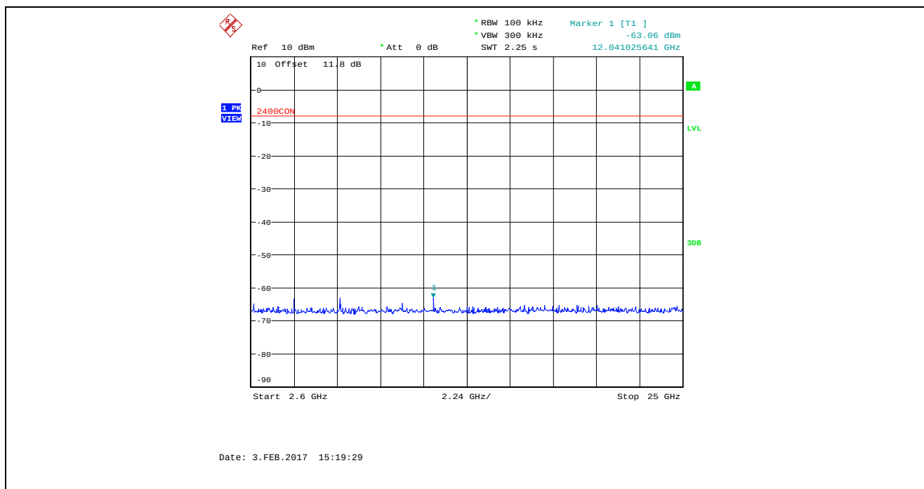
Plot 5.4.4.2.8. Conducted Spurious Emissions in Non-restricted Frequency Bands Bandwidth: 8 MHz, TX Gain: 55, Data Rate 4, 2407 MHz, 2.6 GHz – 25 GHz
