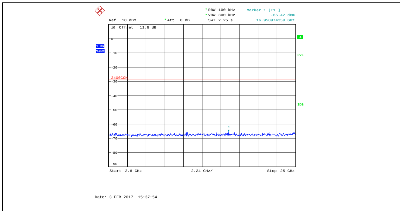
Plot 5.4.4.2.22. Conducted Spurious Emissions in Non-restricted Frequency Bands Bandwidth: 8 MHz, TX Gain: 0, Data Rate 4, 2442 MHz, 2.6 GHz – 25 GHz
