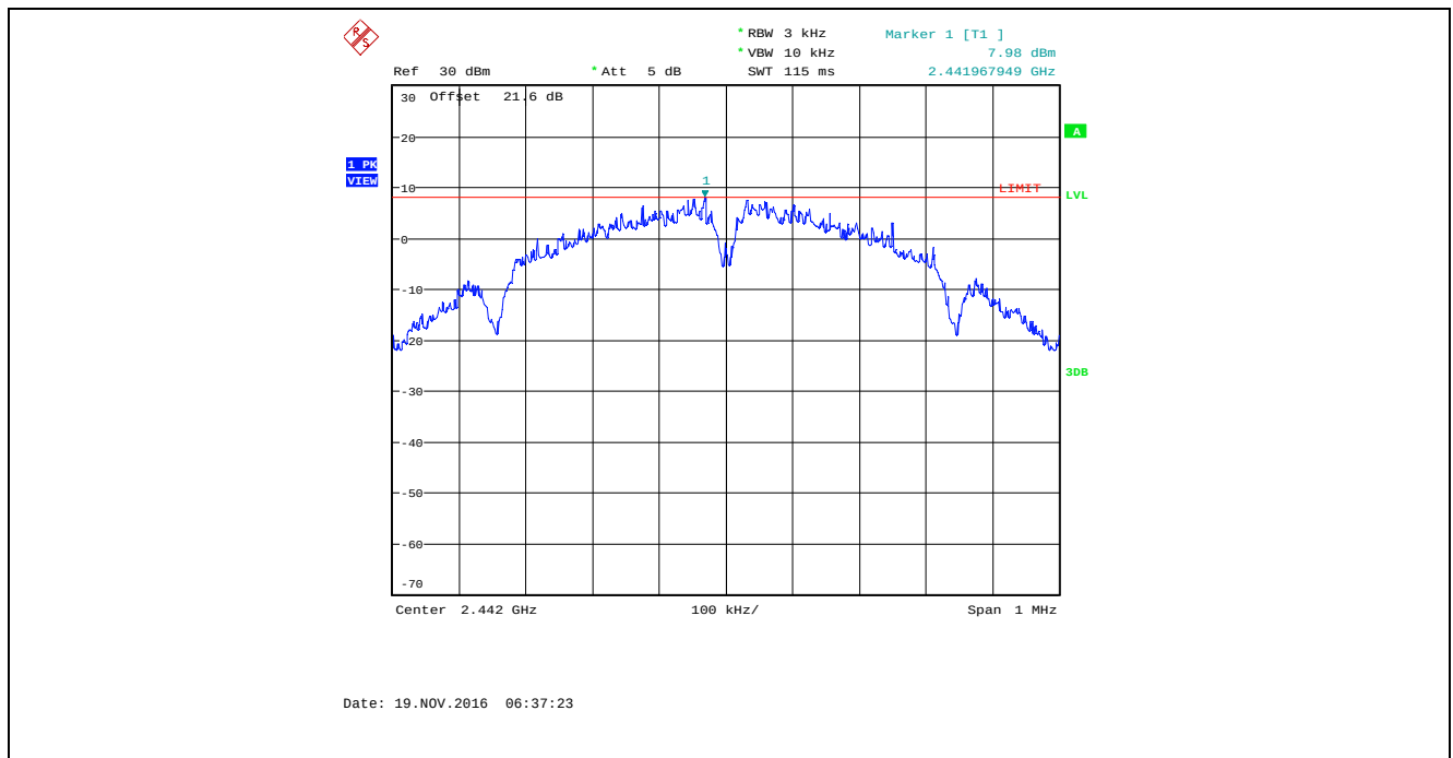
Plot 5.6.4.2. Power Spectral Density, Bandwidth: 1 MHz, TX Gain Setting: 26, Data Rate 1, 2442 MHz
