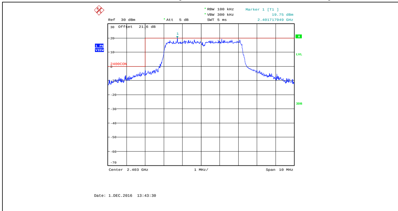
Plot 5.4.4.1.13. Band-Edge RF Conducted Emissions Bandwidth: 4 MHz, TX Gain Setting: 50, Data Rate 7, 2403 MHz, Lower Band-edge
