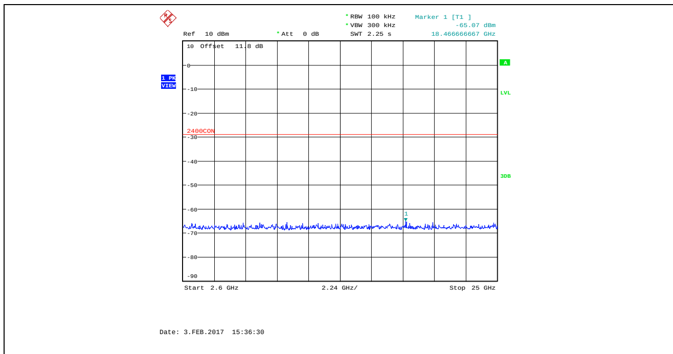
Plot 5.4.4.2.24. Conducted Spurious Emissions in Non-restricted Frequency Bands Bandwidth: 8 MHz, TX Gain: 0, Data Rate 4, 2477 MHz, 2.6 GHz – 25 GHz
