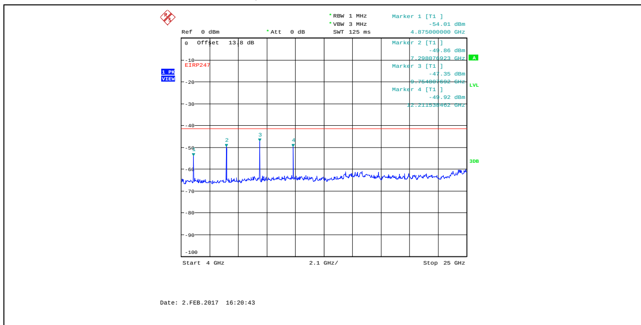
Plot 5.4.4.3.10. Conducted Spurious Emissions in Restricted Frequency Bands Bandwidth: 8 MHz, TX Gain Setting 50, Data Rate 1, 2442 MHz, 4 GHz - 25 GHz, Peak Detector
