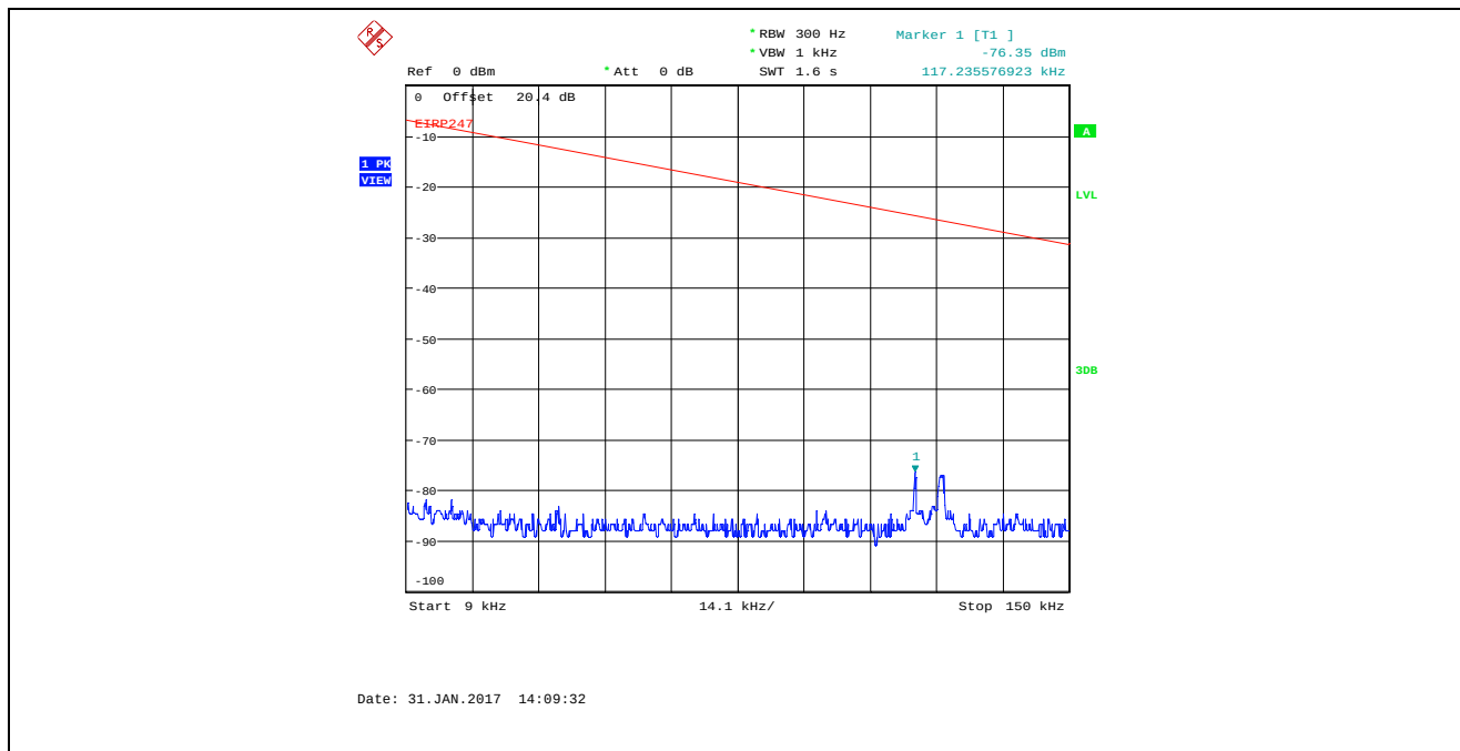
Plot 5.4.4.4.6. Conducted Spurious Emissions in Restricted Frequency Bands Bandwidth: 8 MHz, TX Gain Setting 25, Data Rate 1, 2442 MHz, 9 kHz - 150 kHz, Peak Detector
