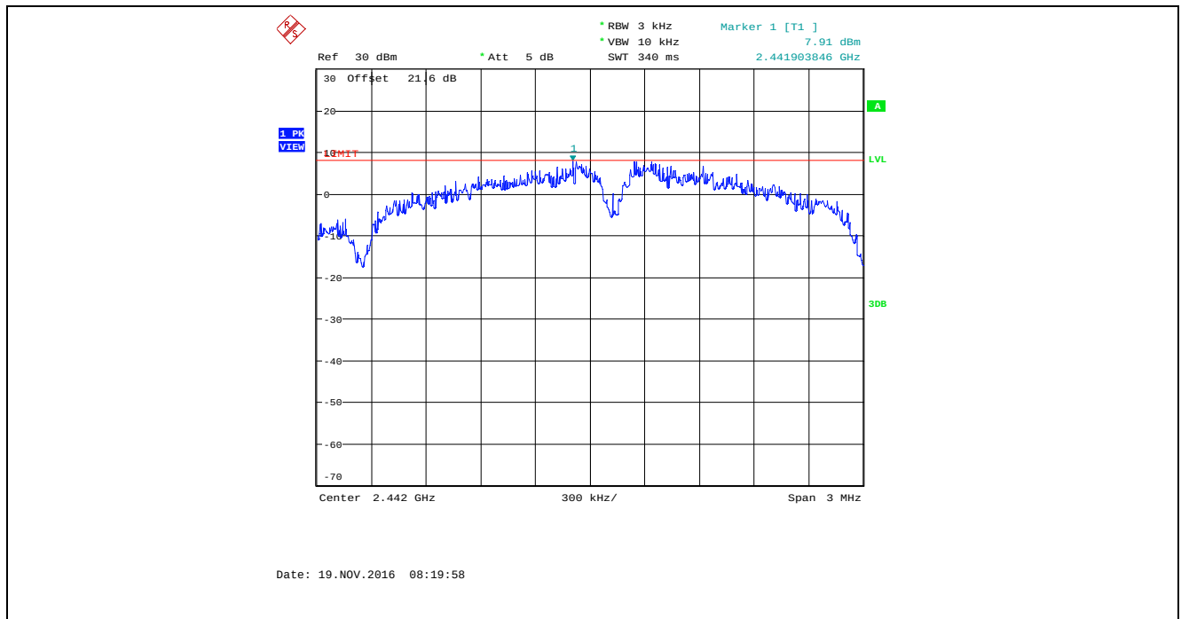
Plot 5.6.4.20. Power Spectral Density, Bandwidth: 4 MHz, TX Gain Setting: 43, Data Rate 2, 2442 MHz
