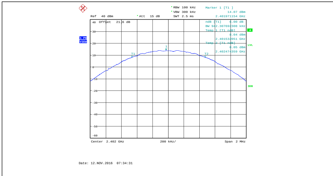
Plot 5.2.4.7. 6 dB Bandwidth, Bandwidth: 2 MHz, TX Gain: 32, Data Rate 1, 2402 MHz
