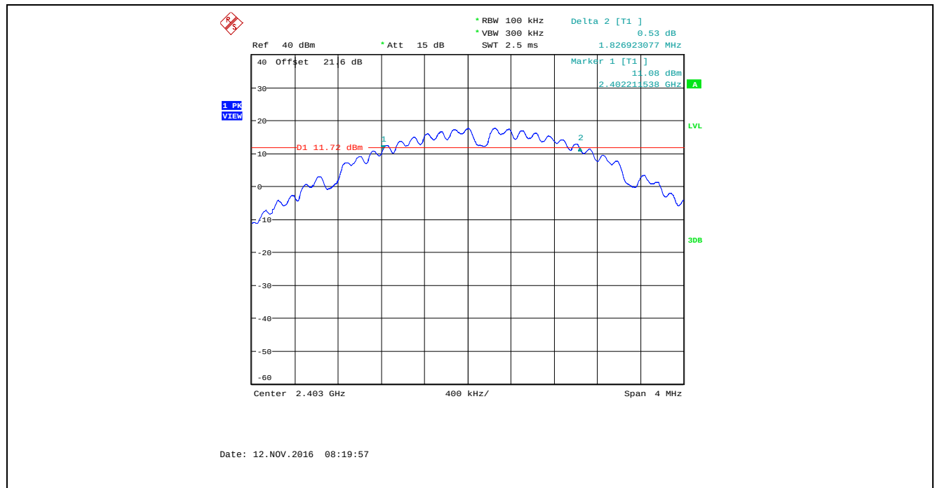
Plot 5.2.4.16. 6 dB Bandwidth, Bandwidth: 4 MHz, TX Gain: 43, Data Rate 1, 2403 MHz
