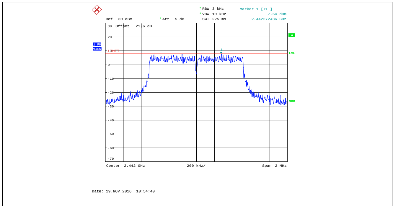
Plot 5.6.4.38. Power Spectral Density, Bandwidth: 1 MHz, TX Gain Setting: 43, Data Rate 5, 2442 MHz
