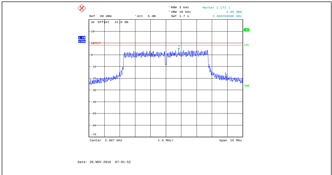
Plot 5.6.4.70. Power Spectral Density, Bandwidth: 8 MHz, TX Gain Setting: 55, Data Rate 4, 2407 MHz
