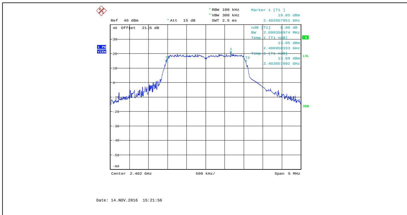
Plot 5.2.4.55. 6 dB Bandwidth, Bandwidth: 2 MHz, TX Gain: 45, Data Rate 7, 2402 MHz
