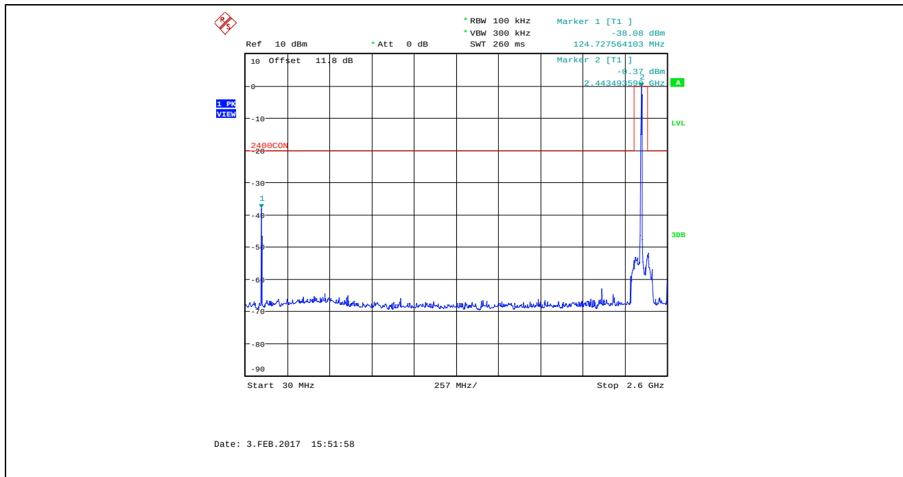
Plot 5.4.4.2.15. Conducted Spurious Emissions in Non-restricted Frequency Bands Bandwidth: 8 MHz, TX Gain: 0, Data Rate 1, 2442 MHz, 30 MHz – 2.6 GHz
