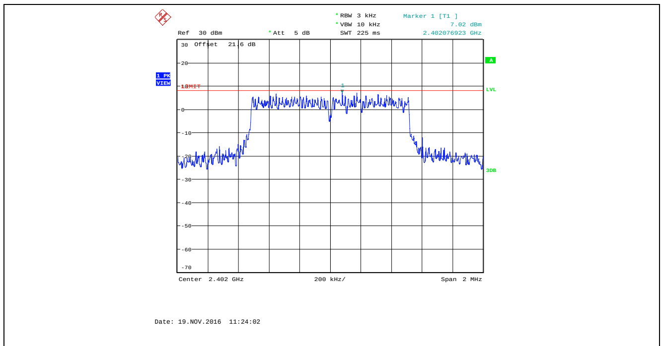
Plot 5.6.4.43. Power Spectral Density, Bandwidth: 1 MHz, TX Gain Setting: 43, Data Rate 7, 2402 MHz
