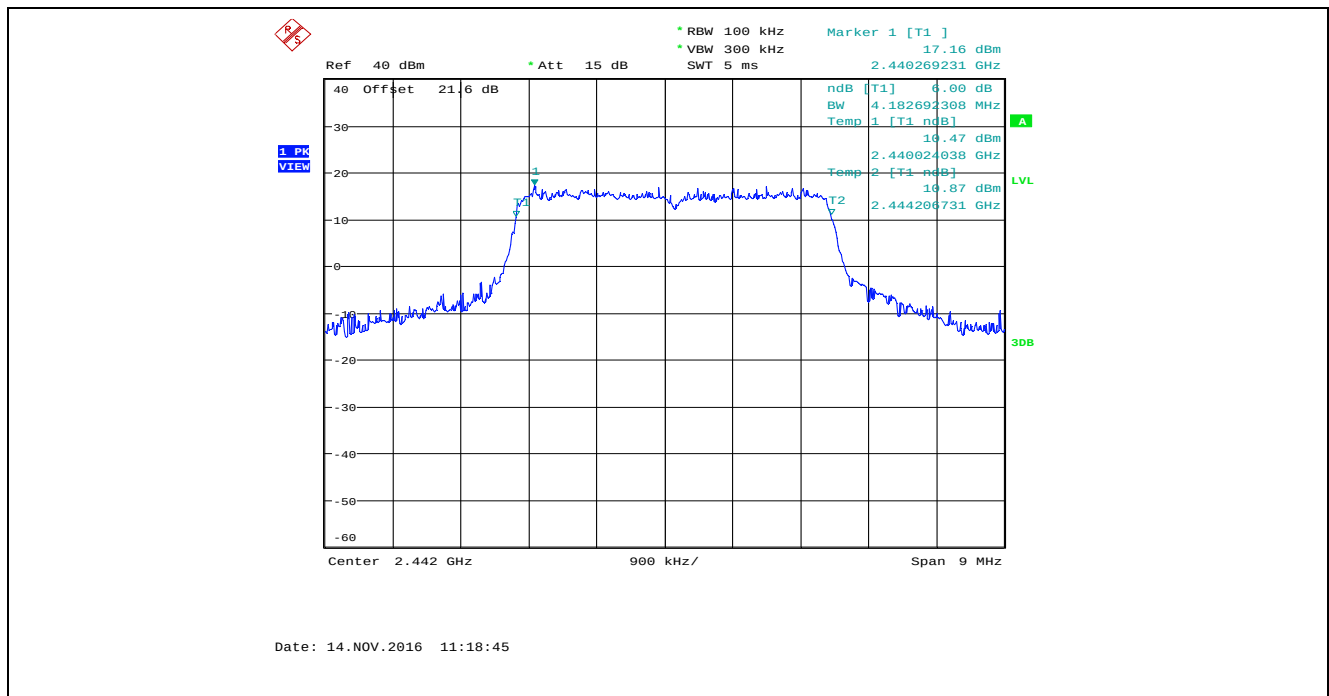
Plot 5.2.4.65. 6 dB Bandwidth, Bandwidth: 4 MHz, TX Gain: 50, Data Rate 6, 2442 MHz
