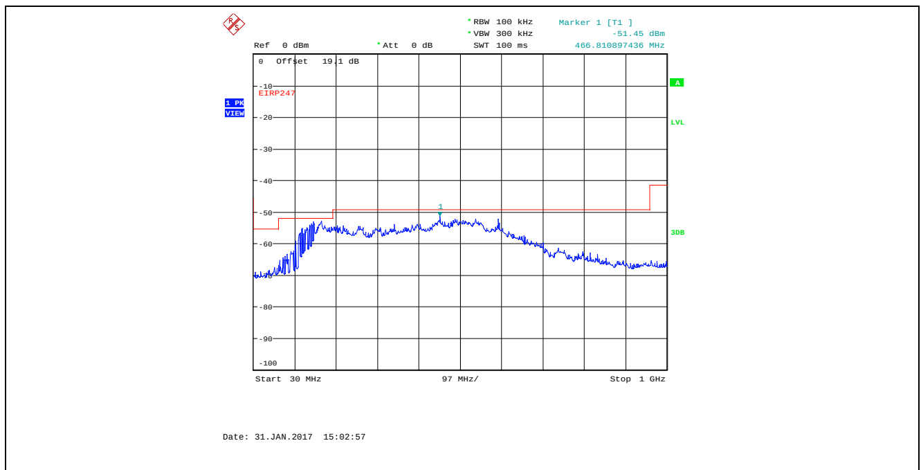
Plot 5.4.4.4.3. Conducted Spurious Emissions in Restricted Frequency Bands Bandwidth: 8 MHz, TX Gain Setting 25, Data Rate 1, 2407 MHz, 30 MHz - 1 GHz, Peak Detector
