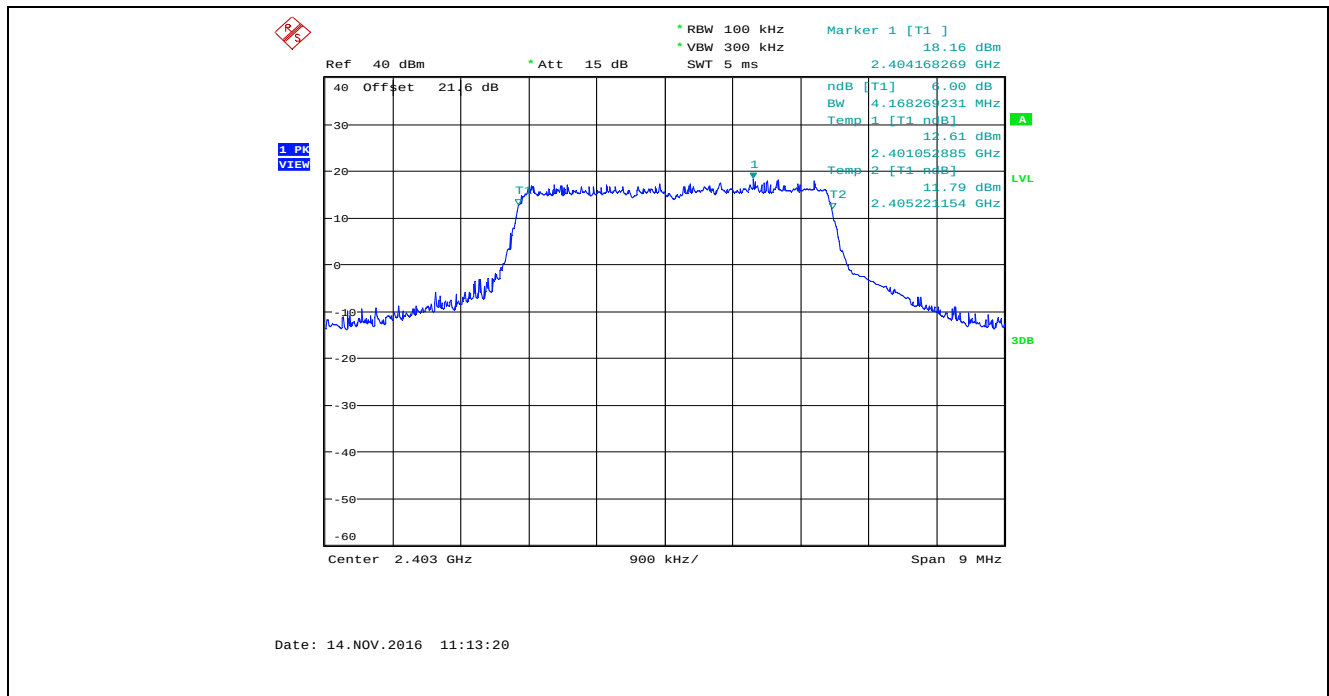
Plot 5.2.4.64. 6 dB Bandwidth, Bandwidth: 4 MHz, TX Gain: 50, Data Rate 6, 2403 MHz,
