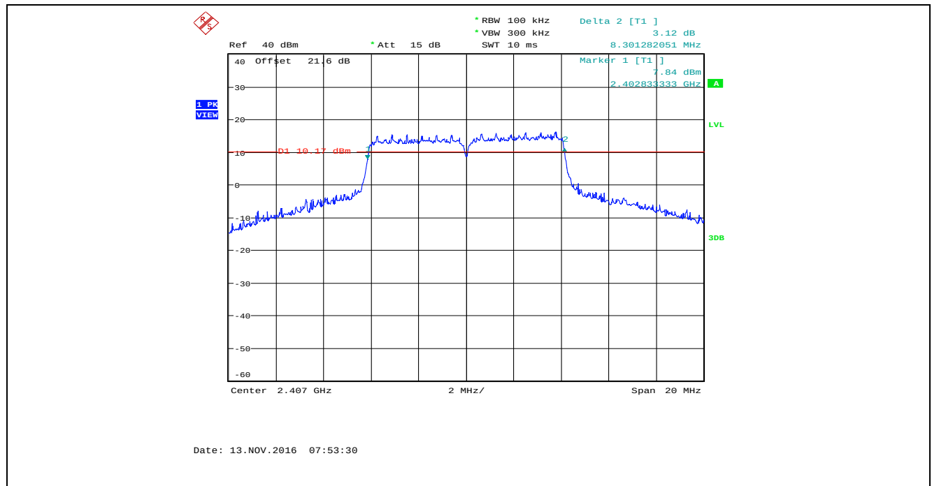
Plot 5.2.4.70. 6 dB Bandwidth, Bandwidth: 8 MHz, TX Gain: 55, Data Rate 4, 2407 MHz
