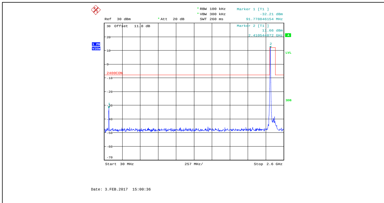
Plot 5.4.4.2.7. Conducted Spurious Emissions in Non-restricted Frequency Bands Bandwidth: 8 MHz, TX Gain: 55, Data Rate 4, 2407 MHz, 30 MHz – 2.6 GHz
