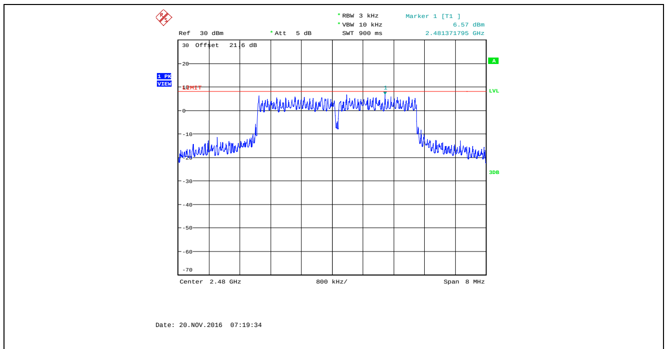
Plot 5.6.4.69. Power Spectral Density, Bandwidth: 4 MHz, TX Gain Setting: 50, Data Rate 7, 2480 MHz
