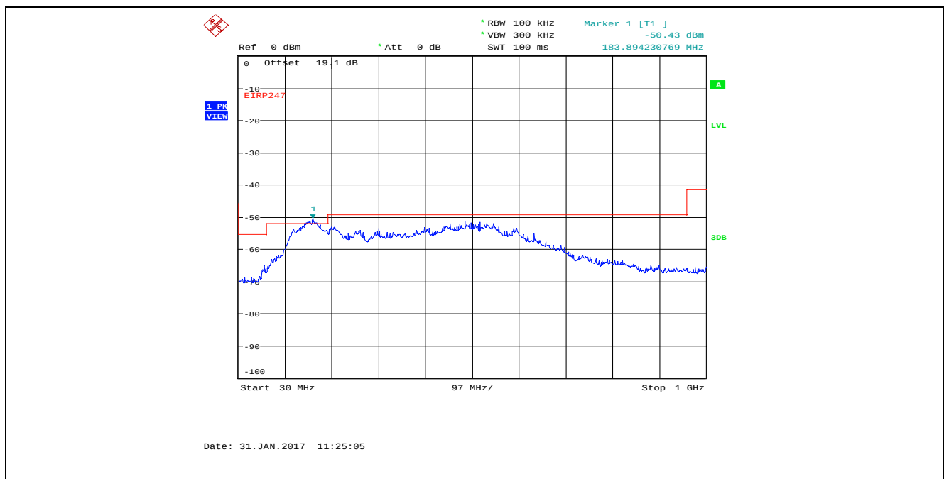
Plot 5.4.4.4.32. Conducted Spurious Emissions in Restricted Frequency Bands Bandwidth: 8 MHz, TX Gain Setting 25, Data Rate 4, 2477 MHz, 30 MHz - 1 GHz, Peak Detector
