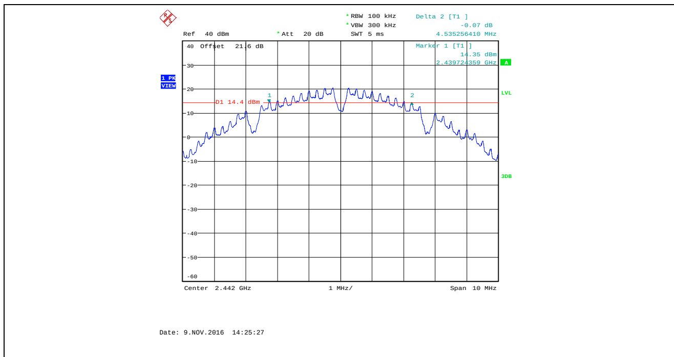
Plot 5.2.4.26. 6 dB Bandwidth, Bandwidth: 8 MHz, TX Gain: 50, Data Rate 1, 2442 MHz
