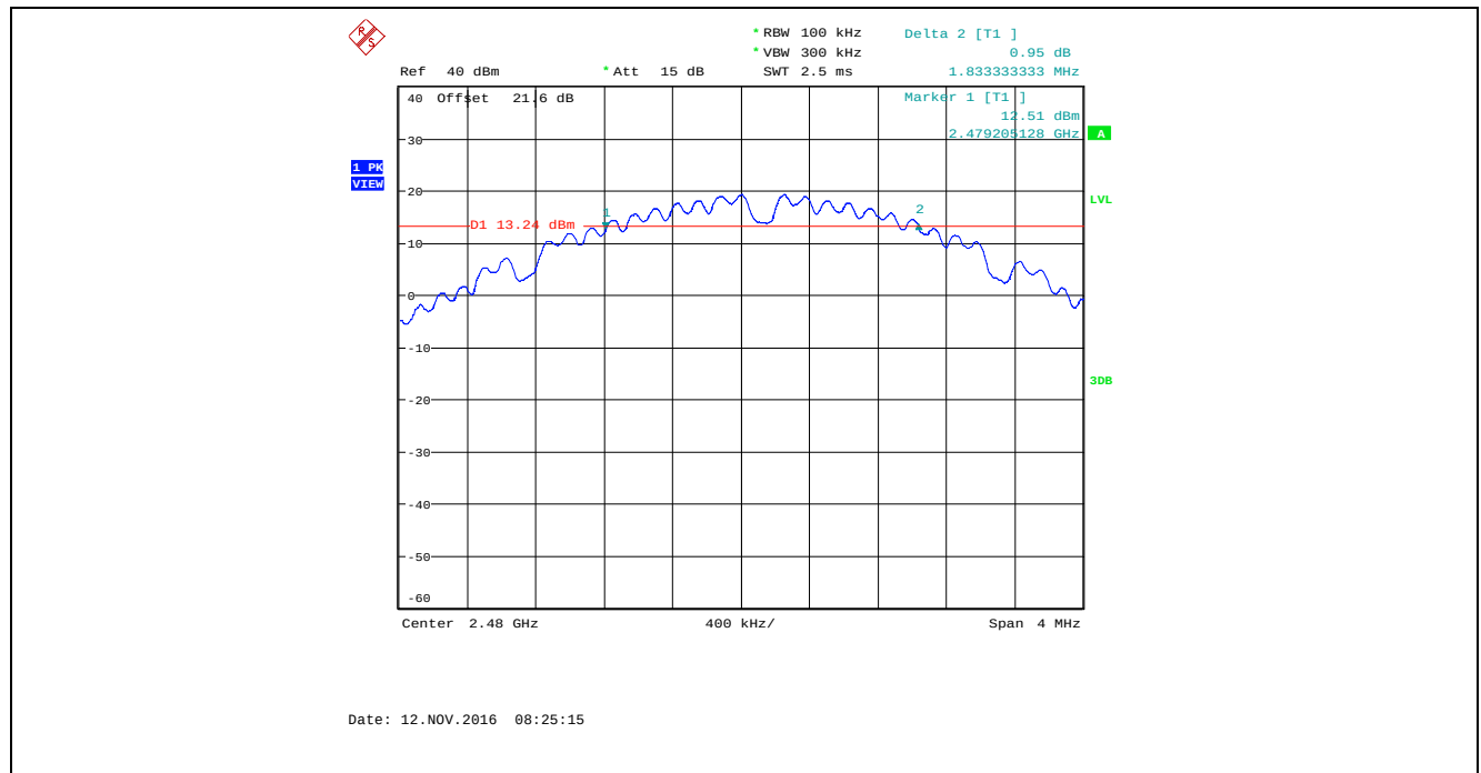
Plot 5.2.4.18. 6 dB Bandwidth, Bandwidth: 4 MHz, TX Gain: 43, Data Rate 1, 2480 MHz
