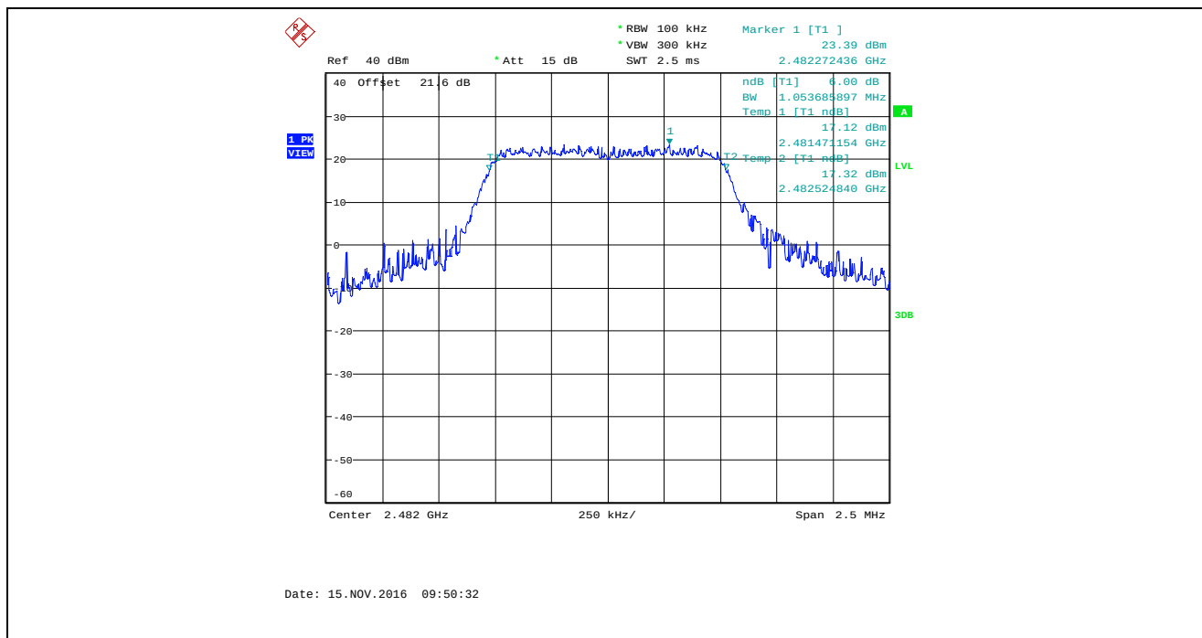
Plot 5.2.4.45. 6 dB Bandwidth, Bandwidth: 1 MHz, TX Gain: 43, Data Rate 7, 2482 MHz
