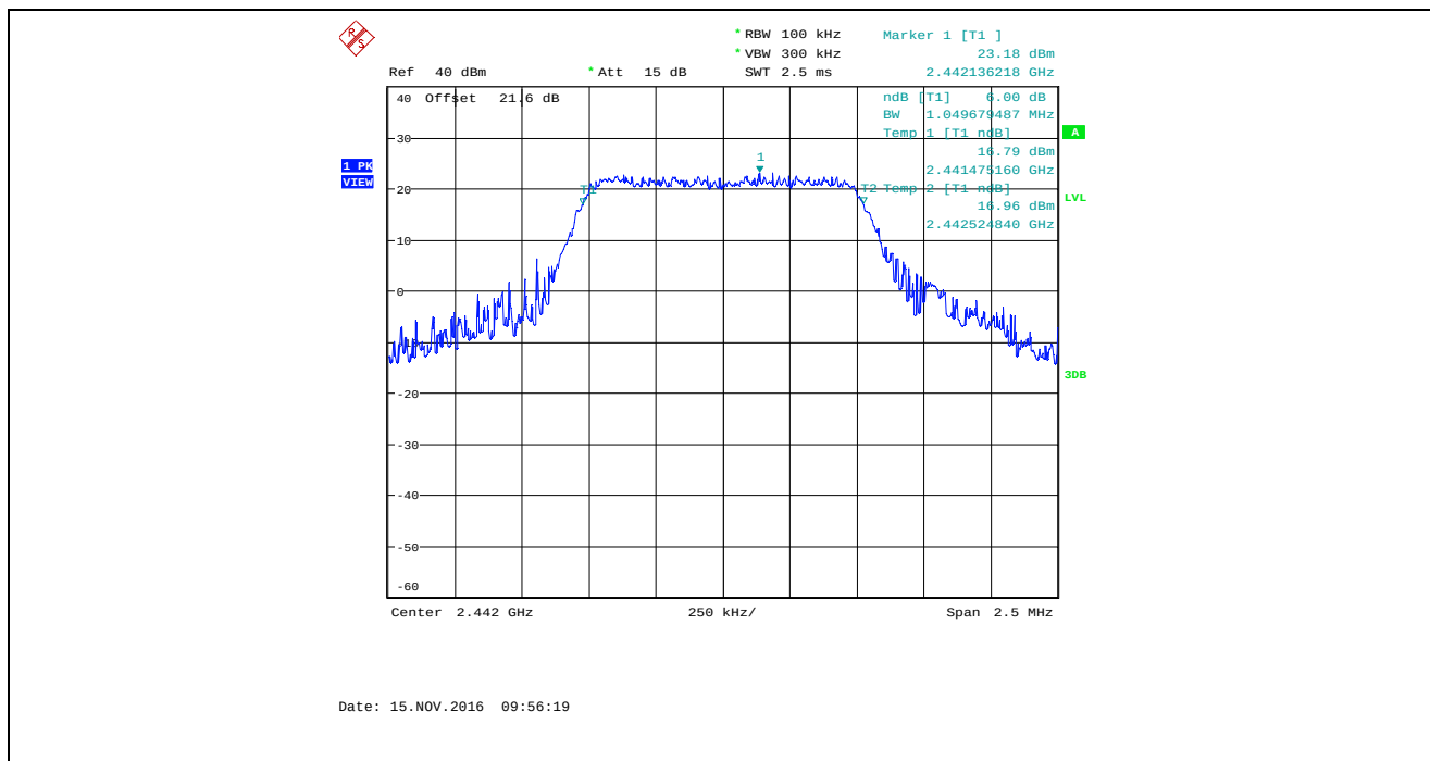
Plot 5.2.4.44. 6 dB Bandwidth, Bandwidth: 1 MHz, TX Gain: 43, Data Rate 7, 2442 MHz
