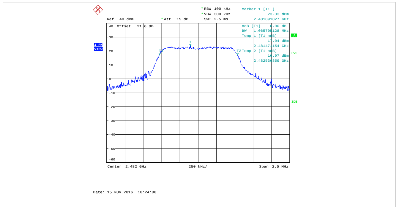
Plot 5.2.4.42. 6 dB Bandwidth, Bandwidth: 1 MHz, TX Gain: 43, Data Rate 6, 2482 MHz
