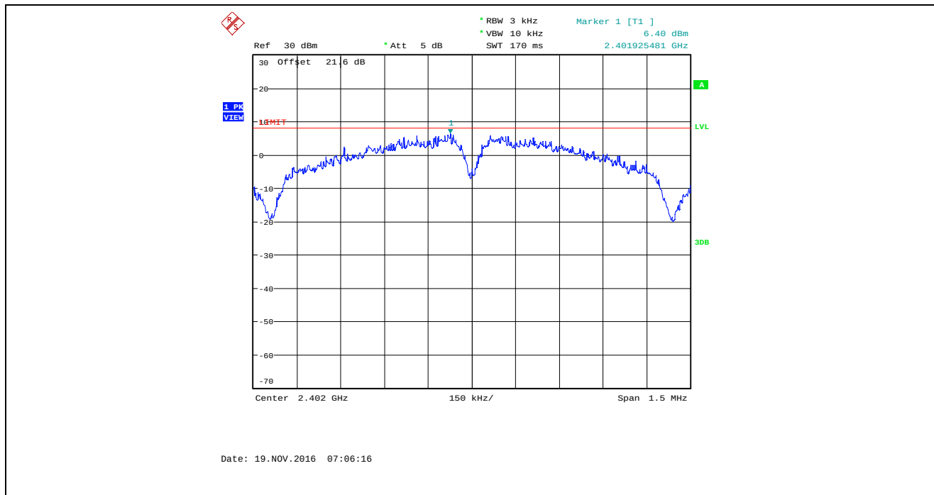
Plot 5.6.4.7. Power Spectral Density, Bandwidth: 2 MHz, TX Gain Setting: 32, Data Rate 1, 2402 MHz
