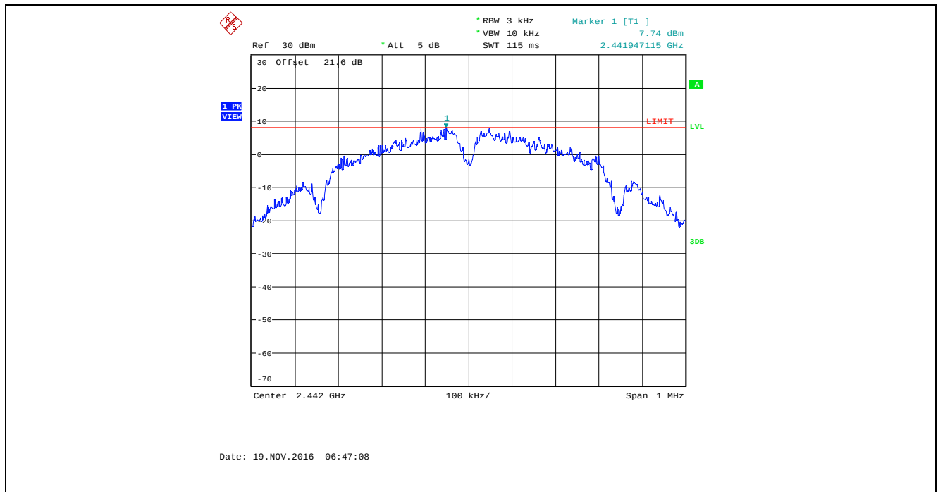
Plot 5.6.4.5. Power Spectral Density, Bandwidth: 1 MHz, TX Gain Setting: 26, Data Rate 2, 2442 MHz
