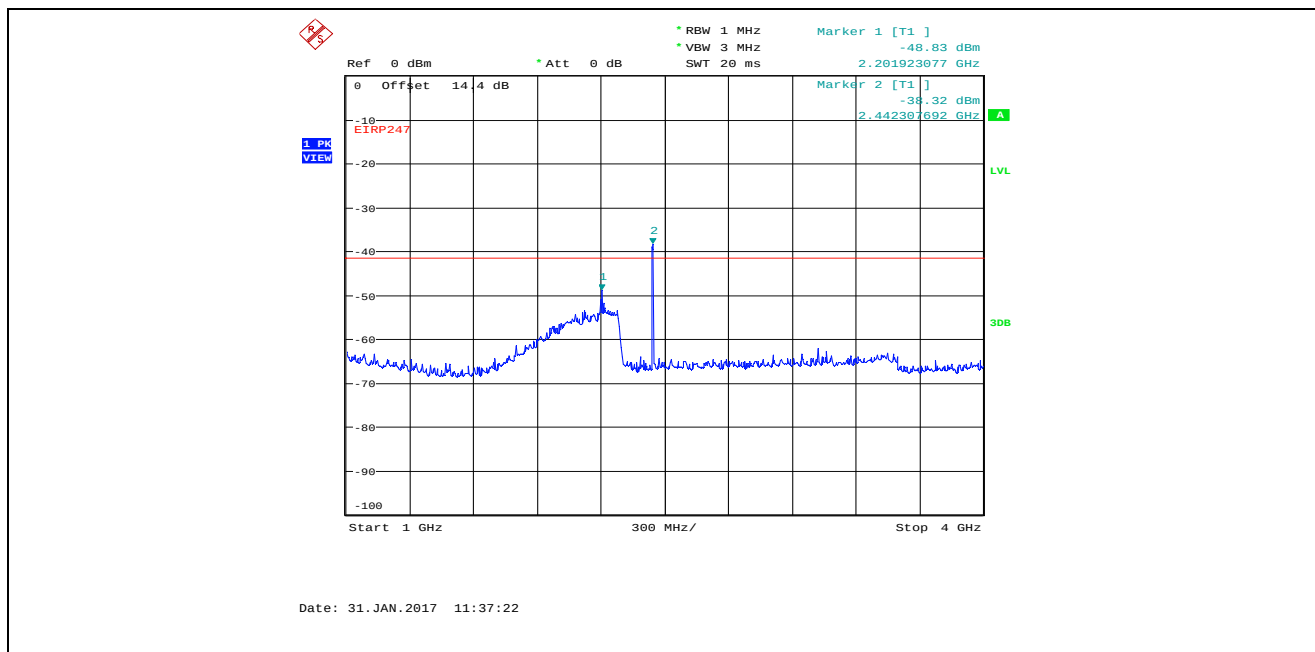
Plot 5.4.4.4.28. Conducted Spurious Emissions in Restricted Frequency Bands Bandwidth: 8 MHz, TX Gain Setting 25, Data Rate 4, 2442 MHz, 1 GHz - 4 GHz, Peak Detector Marker 2 is the Fundamental
