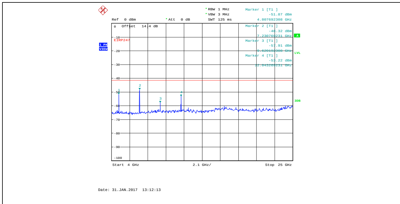
Plot 5.4.4.4.22. Conducted Spurious Emissions in Restricted Frequency Bands Bandwidth: 8 MHz, TX Gain Setting 25, Data Rate 4, 2407 MHz, 4 GHz - 25 GHz, Peak Detector
