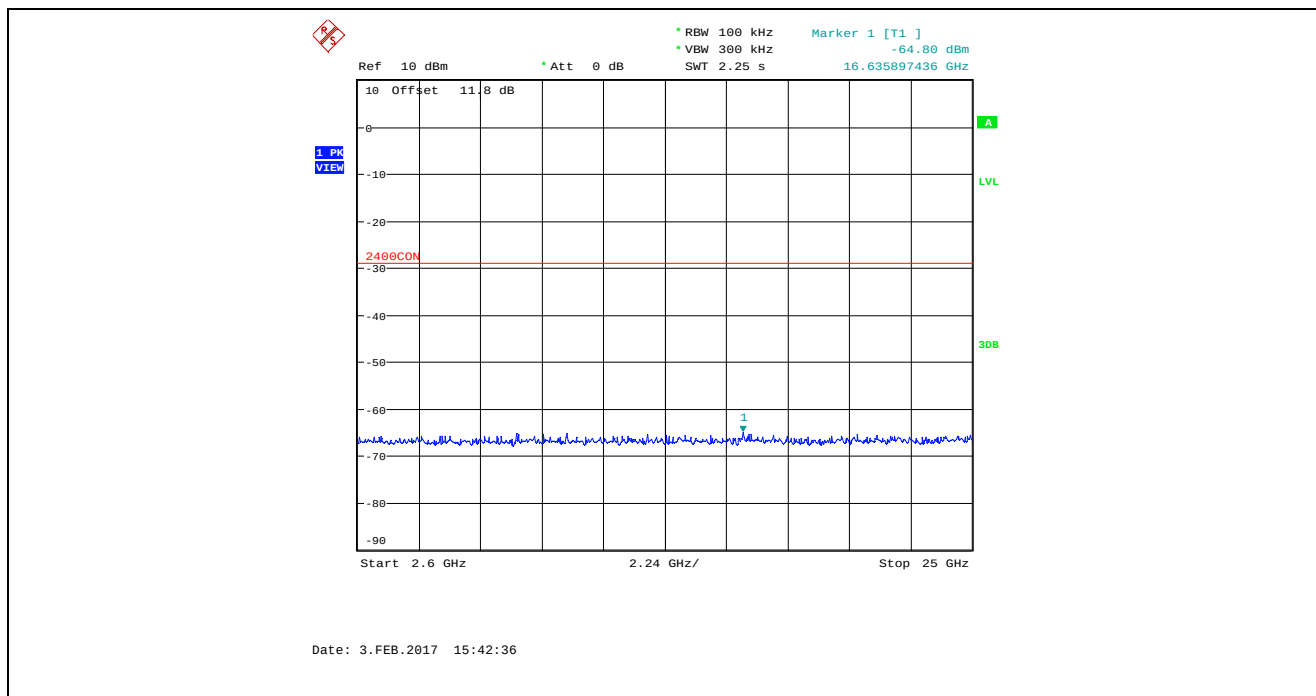
Plot 5.4.4.2.20. Conducted Spurious Emissions in Non-restricted Frequency Bands Bandwidth: 8 MHz, TX Gain: 0, Data Rate 4, 2407 MHz, 2.6 GHz – 25 GHz
