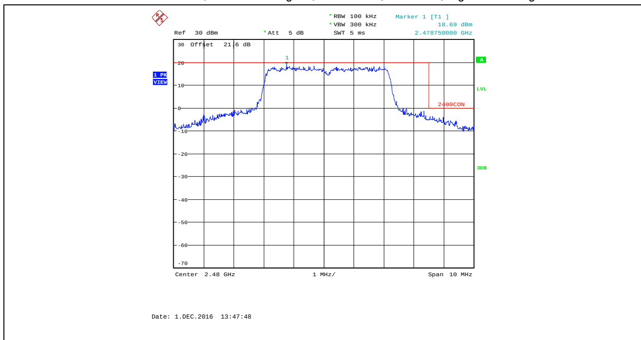
Plot 5.4.4.1.14. Band-Edge RF Conducted Emissions Bandwidth: 4 MHz, TX Gain Setting: 50, Data Rate 7, 2480 MHz, Higher Band-edge
