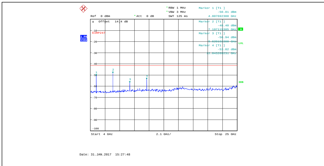
Plot 5.4.4.4.5. Conducted Spurious Emissions in Restricted Frequency Bands Bandwidth: 8 MHz, TX Gain Setting 25, Data Rate 1, 2407 MHz, 4 GHz - 25 GHz, Peak Detector
