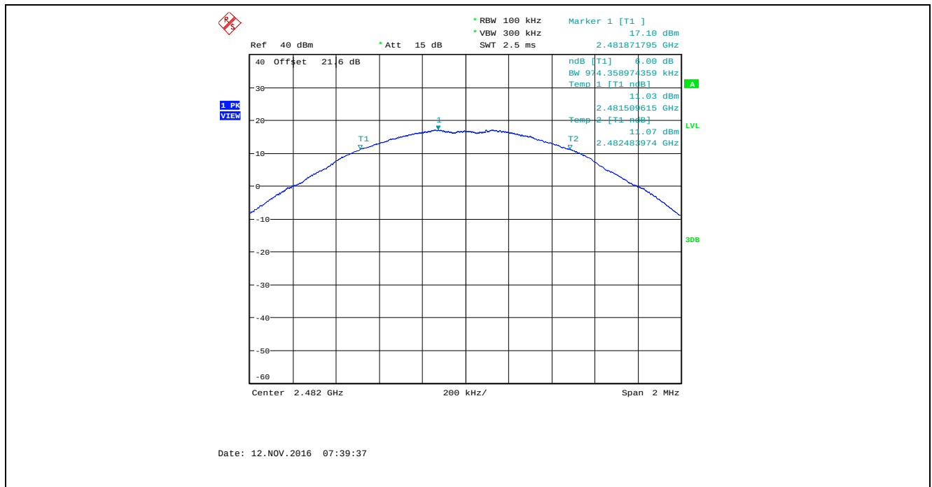
Plot 5.2.4.12. 6 dB Bandwidth, Bandwidth: 2 MHz, TX Gain: 32, Data Rate 2, 2482 MHz
