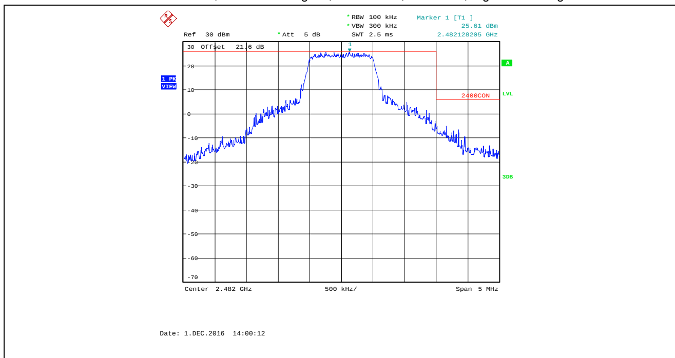
Plot 5.4.4.1.10. Band-Edge RF Conducted Emissions Bandwidth: 1 MHz, TX Gain Setting: 43, Data Rate 7, 2482 MHz, Higher Band-edge
