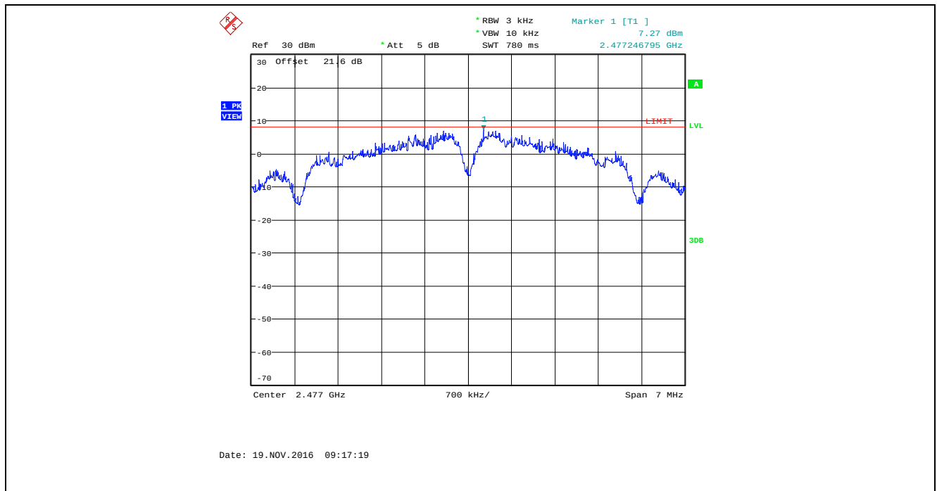
Plot 5.6.4.27. Power Spectral Density, Bandwidth: 8 MHz, TX Gain Setting: 50, Data Rate 1, 2477 MHz
