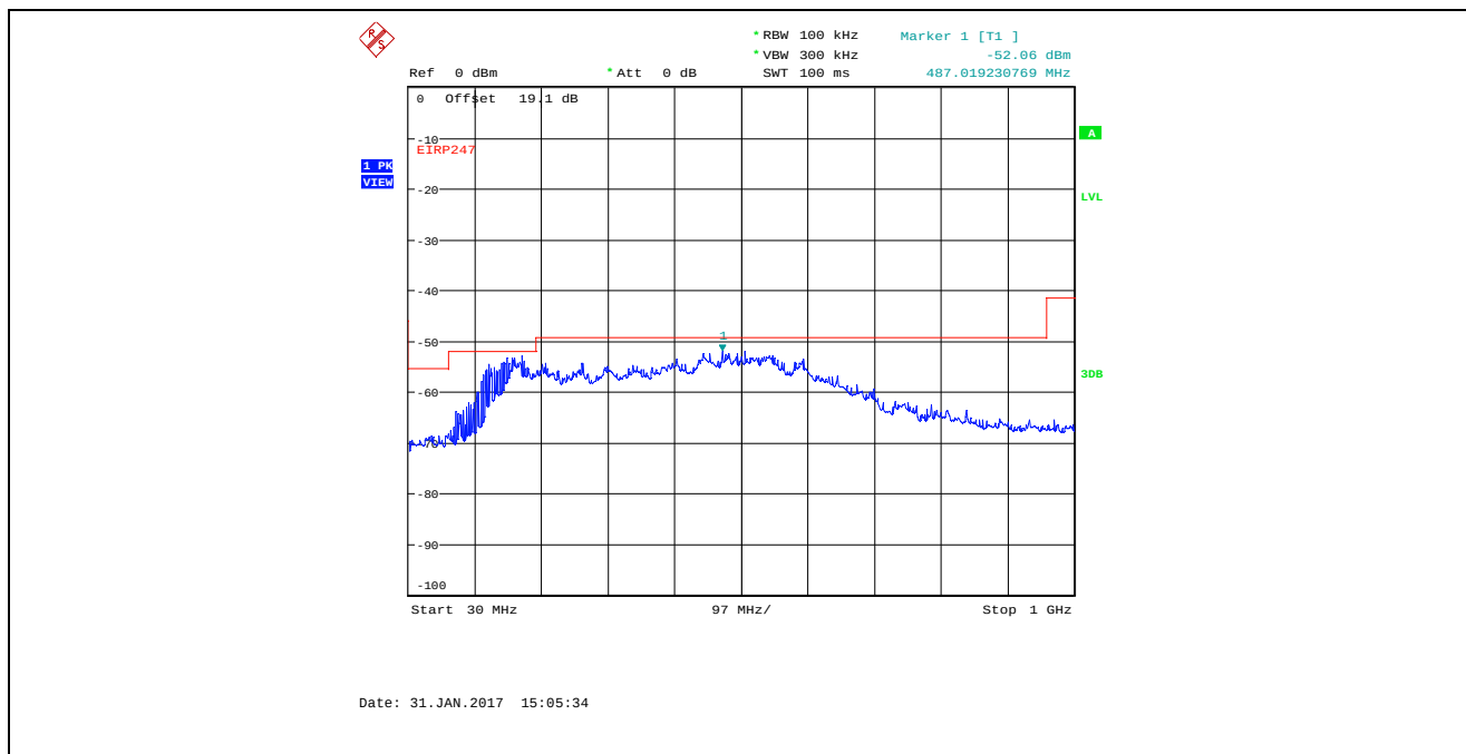
Plot 5.4.4.4.8. Conducted Spurious Emissions in Restricted Frequency Bands Bandwidth: 8 MHz, TX Gain Setting 25, Data Rate 1, 2442 MHz, 30 MHz - 1 GHz, Peak Detector
