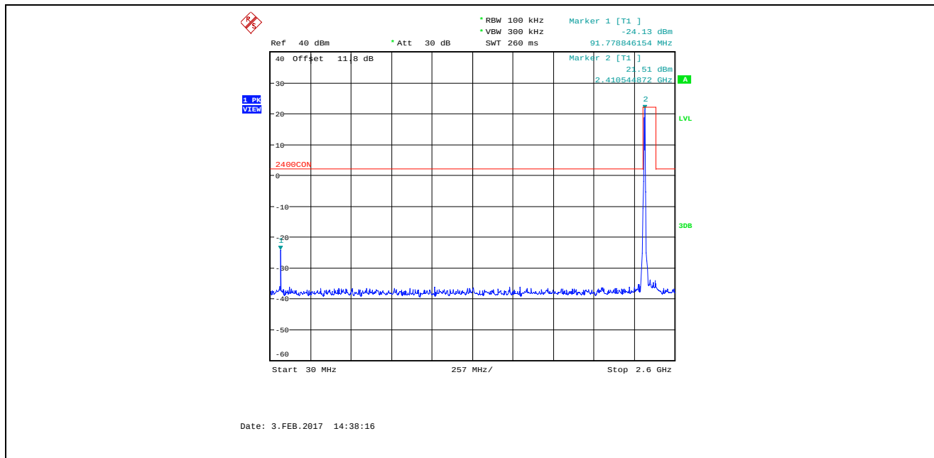
Plot 5.4.4.2.1. Conducted Spurious Emissions in Non-restricted Frequency Bands Bandwidth: 8, TX Gain: 50, Data Rate 1, 2407 MHz, 30 MHz – 2.6 GHz
