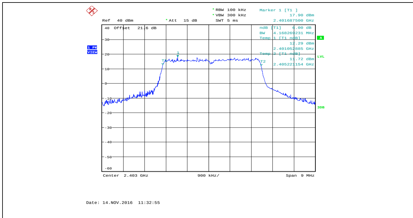
Plot 5.2.4.67. 6 dB Bandwidth, Bandwidth: 4 MHz, TX Gain: 50, Data Rate 7, 2403 MHz
