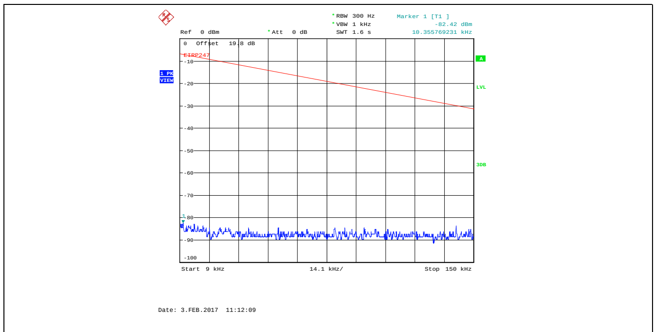
Plot 5.4.4.3.21. Conducted Spurious Emissions in Restricted Frequency Bands Bandwidth: 8 MHz, TX Gain Setting 55, Data Rate 4, 2442 MHz, 9 kHz - 150 kHz, Peak Detector
