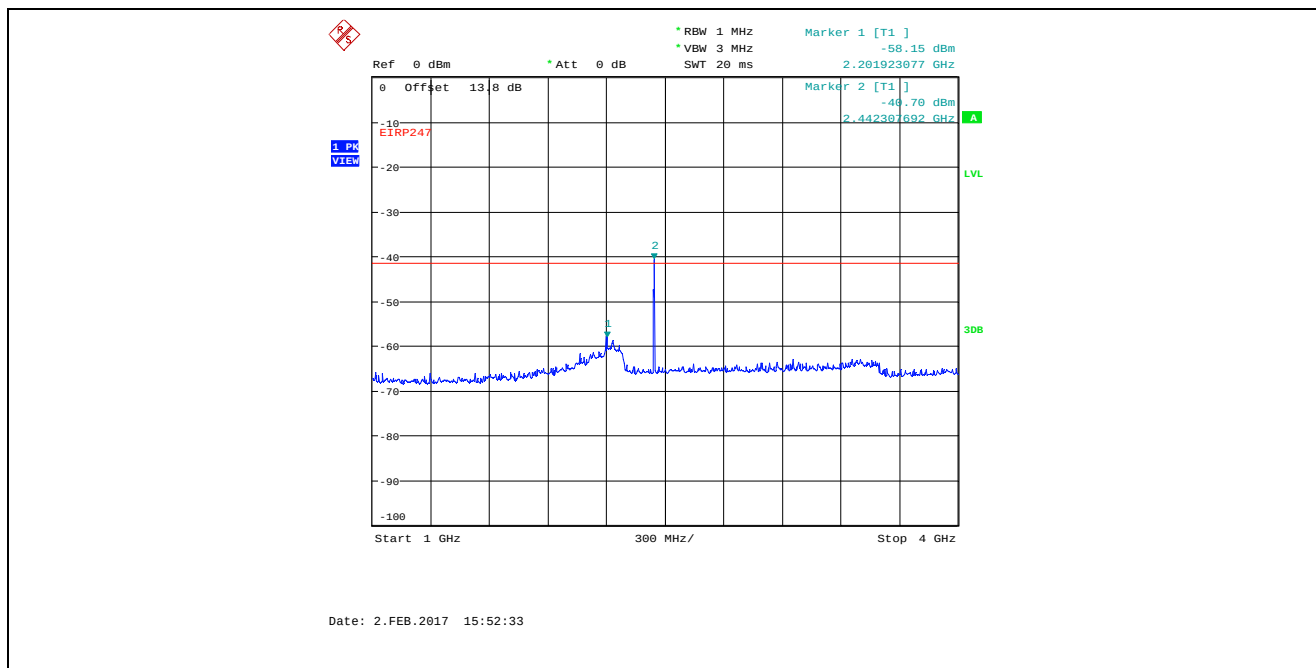
Plot 5.4.4.3.9. Conducted Spurious Emissions in Restricted Frequency Bands Bandwidth: 8 MHz, TX Gain Setting 50, Data Rate 1, 2442 MHz, 1 GHz - 4 GHz, Peak Detector Marker 2 is the Fundamental
