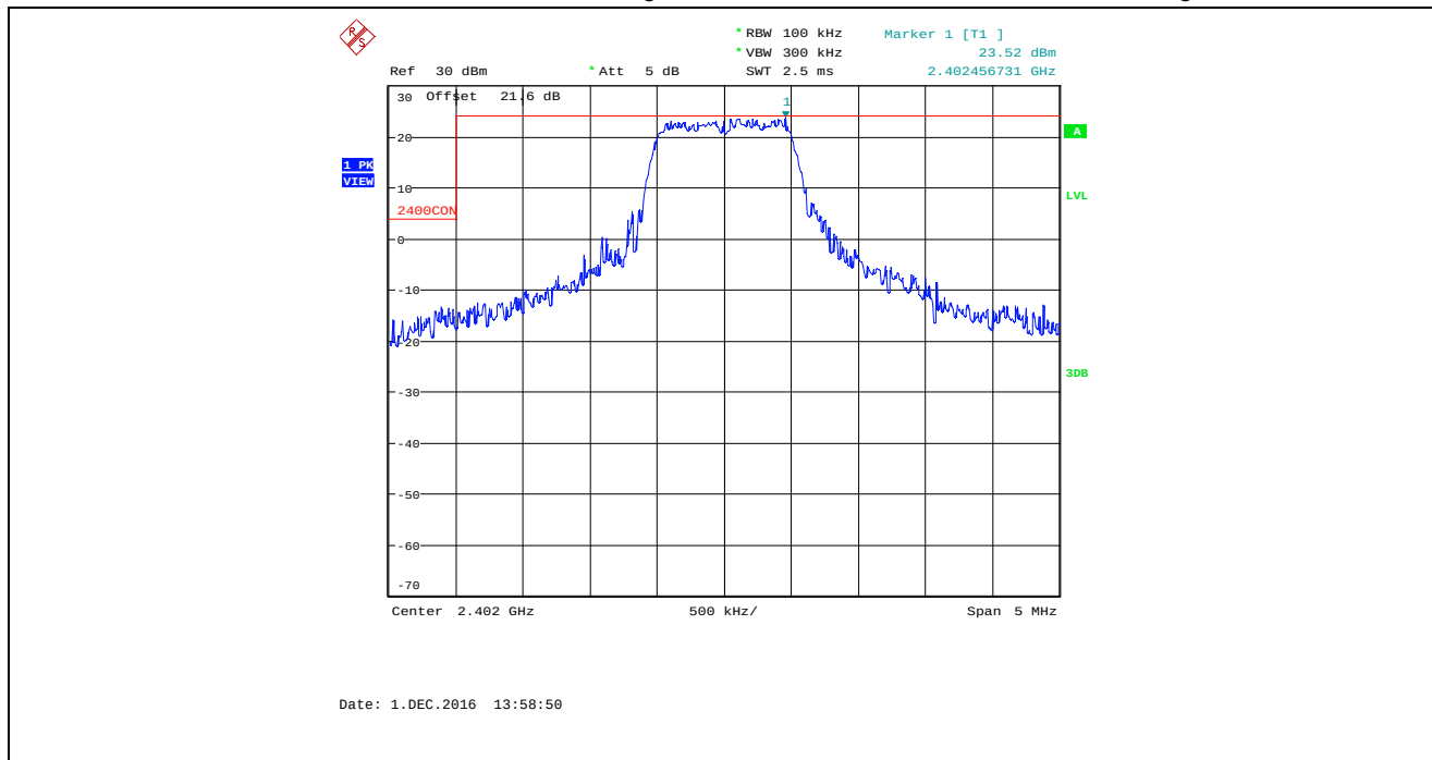
Plot 5.4.4.1.9. Band-Edge RF Conducted Emissions Bandwidth: 1 MHz, TX Gain Setting: 43, Data Rate 7, 2402 MHz, Lower Band-edge
