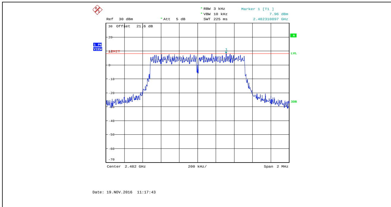
Plot 5.6.4.45. Power Spectral Density, Bandwidth: 1 MHz, TX Gain Setting: 43, Data Rate 7, 2482 MHz
