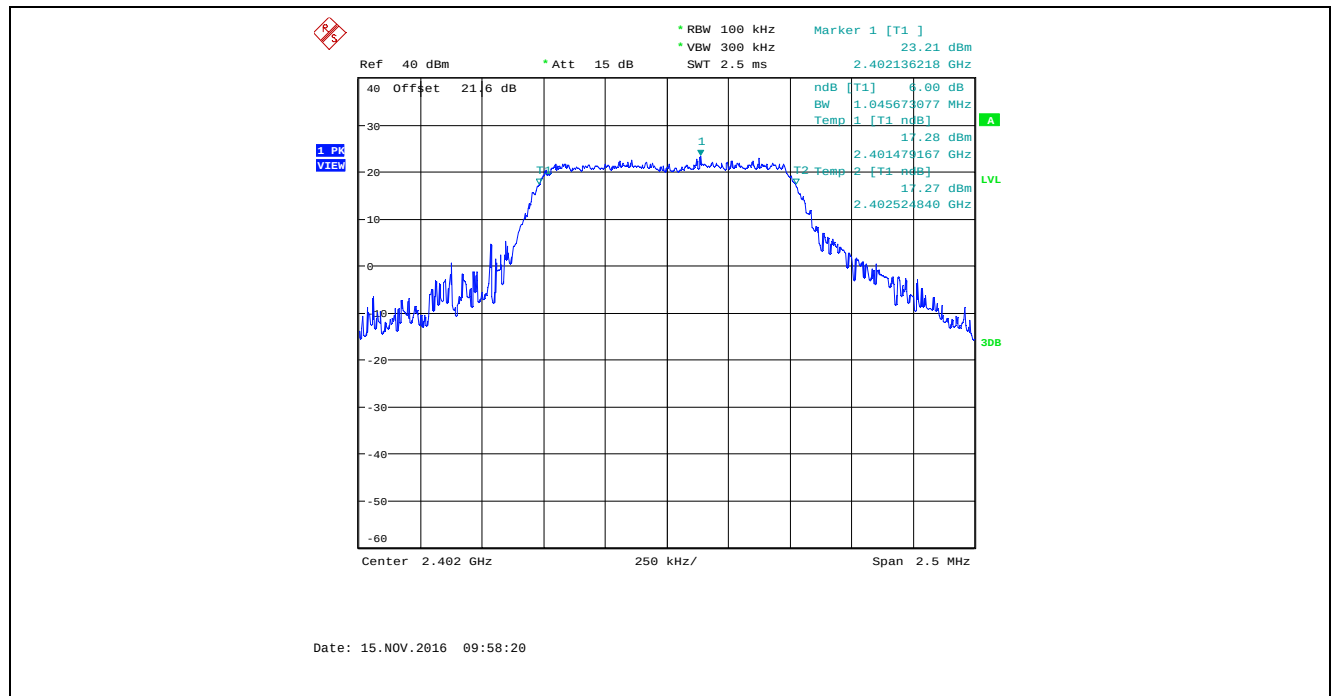
Plot 5.2.4.43. 6 dB Bandwidth, Bandwidth: 1 MHz, TX Gain: 43, Data Rate 7, 2402 MHz
