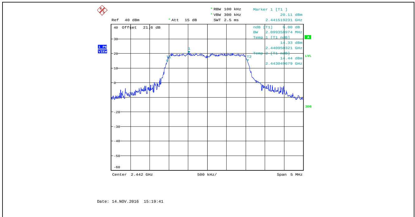
Plot 5.2.4.56. 6 dB Bandwidth, Bandwidth: 2 MHz, TX Gain: 45, Data Rate 7, 2442 MHz
