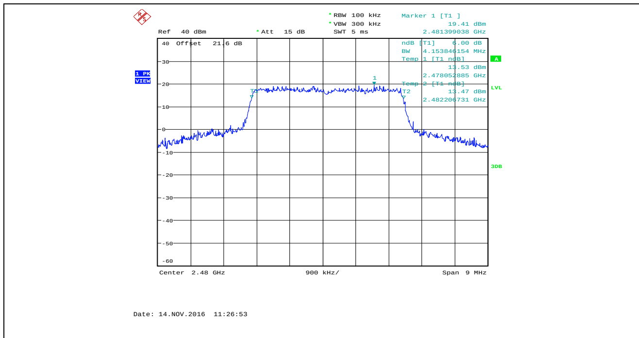
Plot 5.2.4.69. 6 dB Bandwidth, Bandwidth: 4 MHz, TX Gain: 50, Data Rate 7, 2480 MHz
