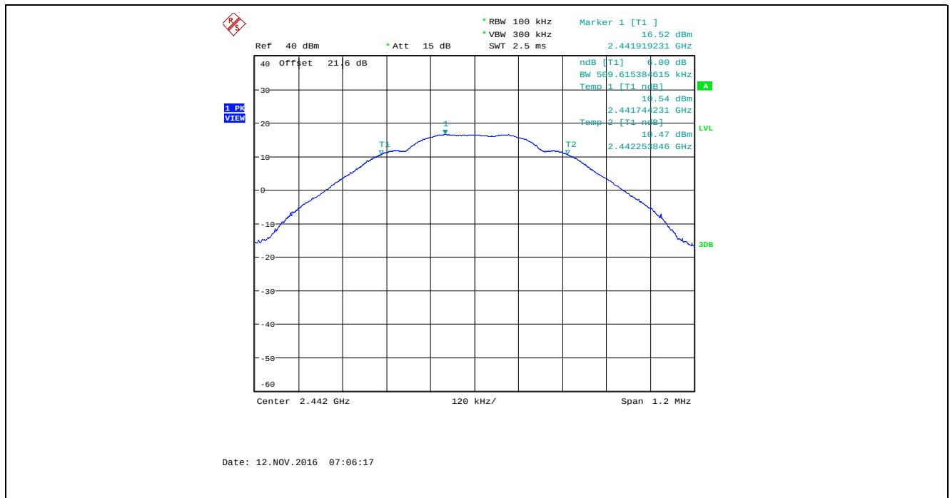
Plot 5.2.4.2. 6 dB Bandwidth, Bandwidth: 1 MHz, TX Gain: 26, Data Rate 1, 2442 MHz
