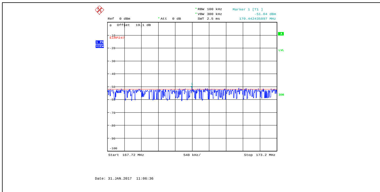
Plot 5.4.4.4.19. Conducted Spurious Emissions in Restricted Frequency Bands Bandwidth: 8 MHz, TX Gain Setting 25, Data Rate 4, 2407 MHz, RB 167.72-173.2 MHz, QP Detector
