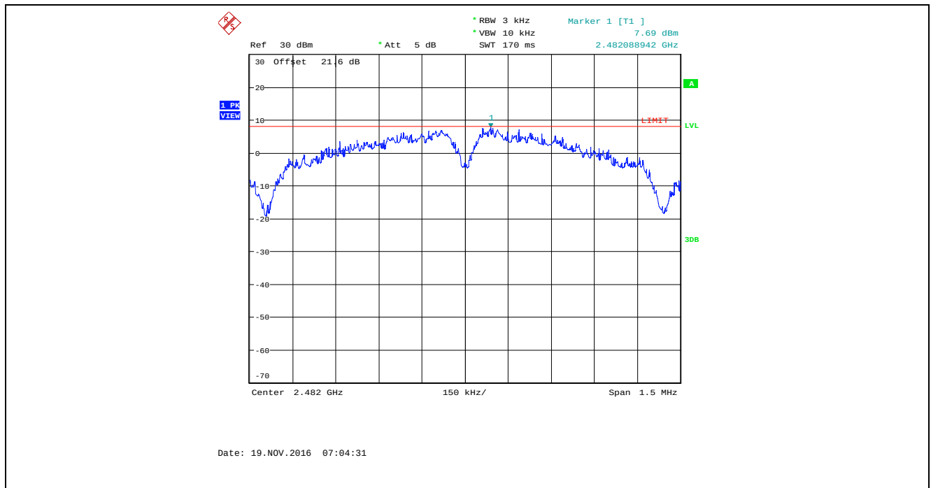
Plot 5.6.4.9. Power Spectral Density, Bandwidth: 2 MHz, TX Gain Setting: 32, Data Rate 1, 2482 MHz
