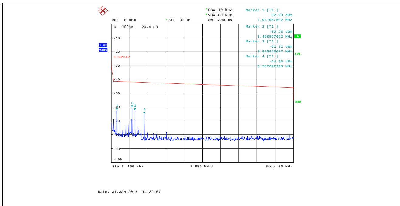
Plot 5.4.4.4.12. Conducted Spurious Emissions in Restricted Frequency Bands Bandwidth: 8 MHz, TX Gain Setting 25, Data Rate 1, 2477 MHz, 150 kHz - 30 MHz, Peak Detector
