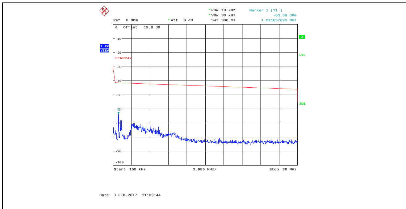
Plot 5.4.4.3.27. Conducted Spurious Emissions in Restricted Frequency Bands Bandwidth: 8 MHz, TX Gain Setting 55, Data Rate 4, 2477 MHz, 150 kHz - 30 MHz, Peak Detector
