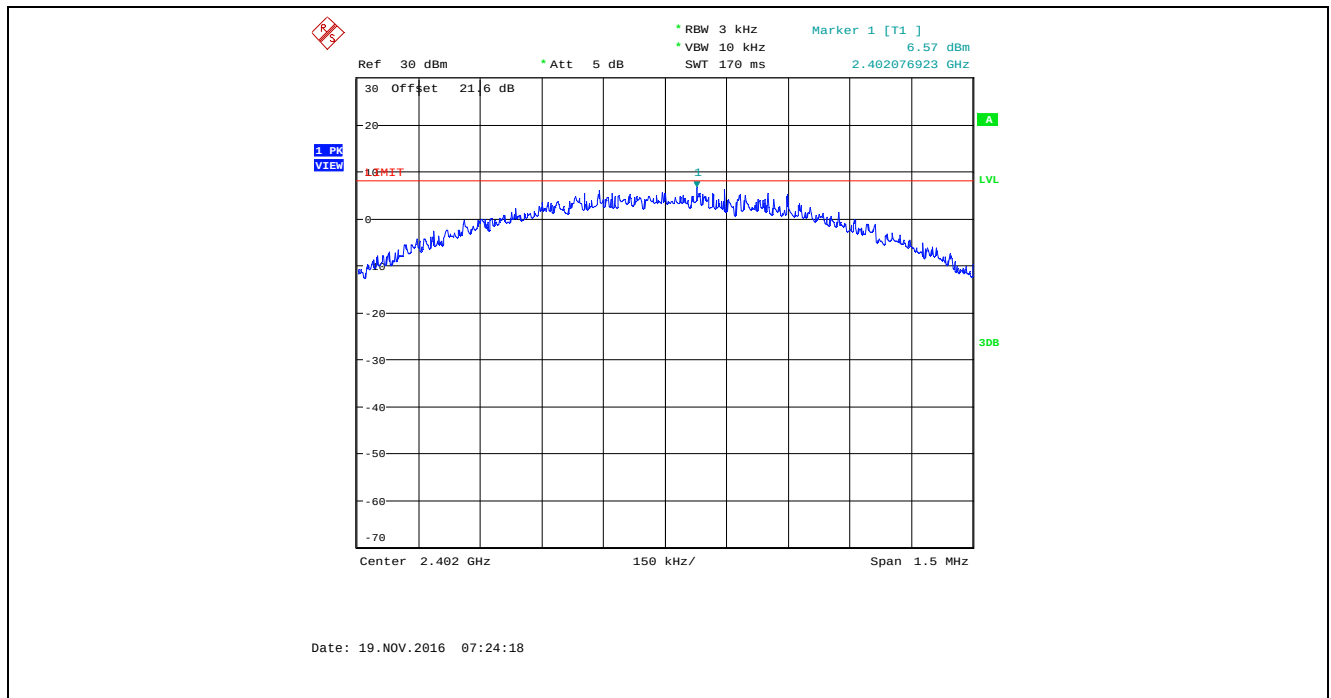
Plot 5.6.4.13. Power Spectral Density, Bandwidth: 2 MHz, TX Gain Setting: 32, Data Rate 3, 2402 MHz
