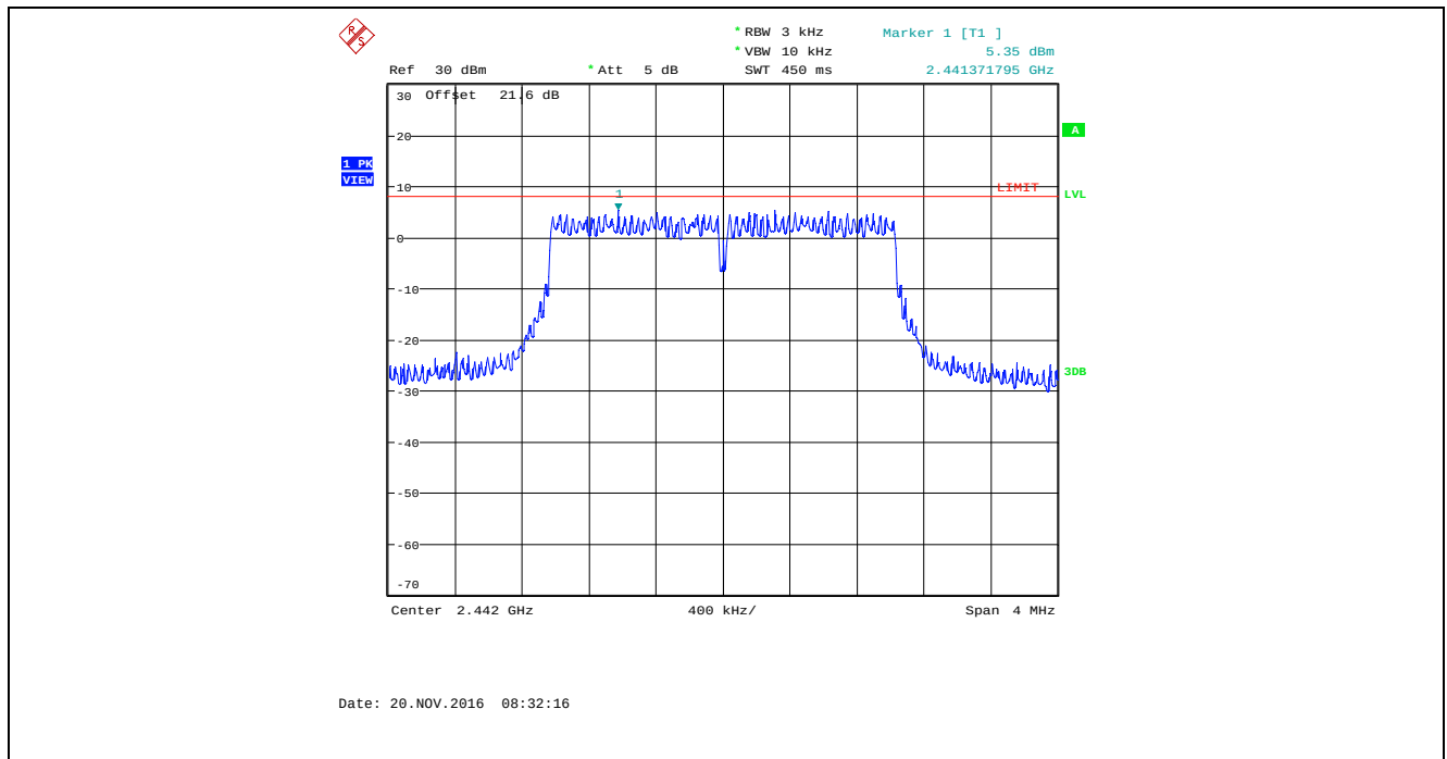
Plot 5.6.4.50. Power Spectral Density, Bandwidth: 2 MHz, TX Gain Setting: 45, Data Rate 5, 2442 MHz
