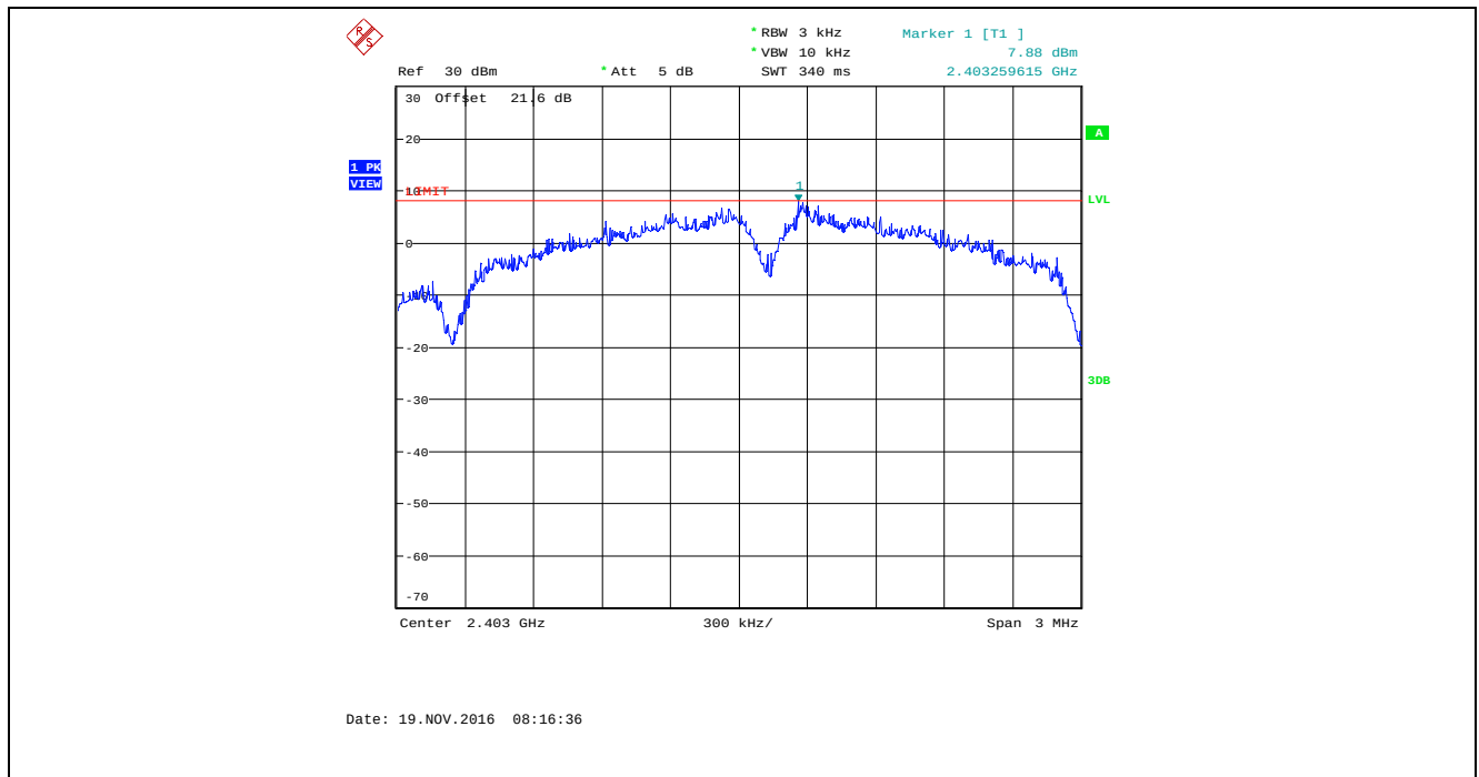
Plot 5.6.4.19. Power Spectral Density, Bandwidth: 4 MHz, TX Gain Setting: 43, Data Rate 2, 2403 MHz
