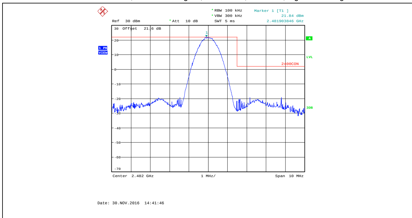
Plot 5.4.4.1.4. Band-Edge RF Conducted Emissions Bandwidth: 2 MHz, TX Gain Setting: 32, Data Rate 3, 2482 MHz, Higher Band-edge
