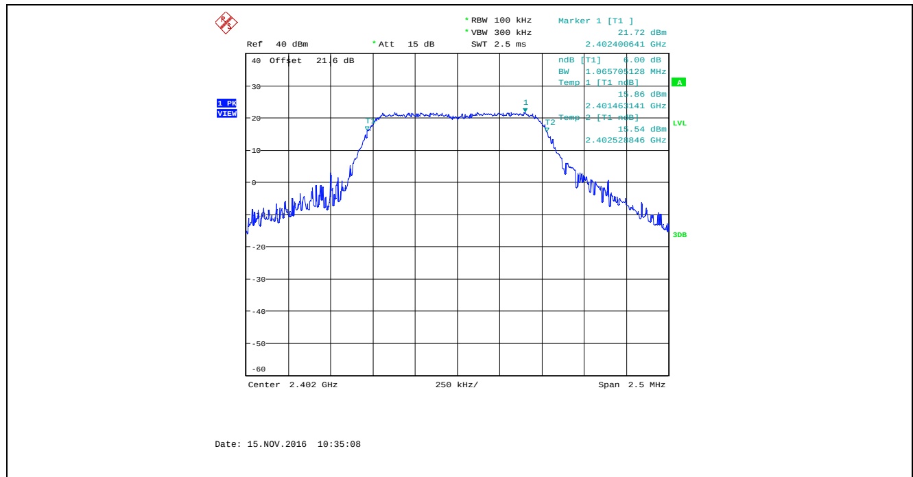
Plot 5.2.4.37. 6 dB Bandwidth, Bandwidth: 1 MHz, TX Gain: 43, Data Rate 5, 2402 MHz
