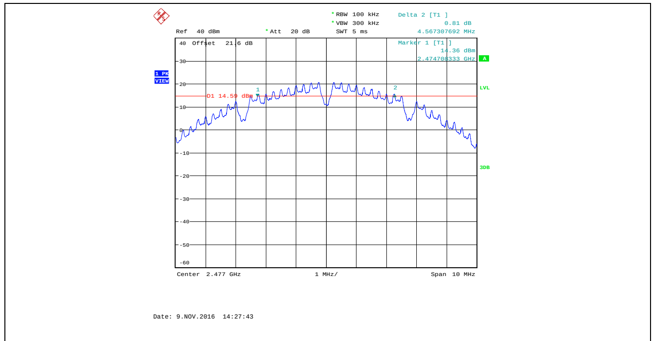
Plot 5.2.4.27. 6 dB Bandwidth, Bandwidth: 8 MHz, TX Gain: 50, Data Rate 1, 2477 MHz
