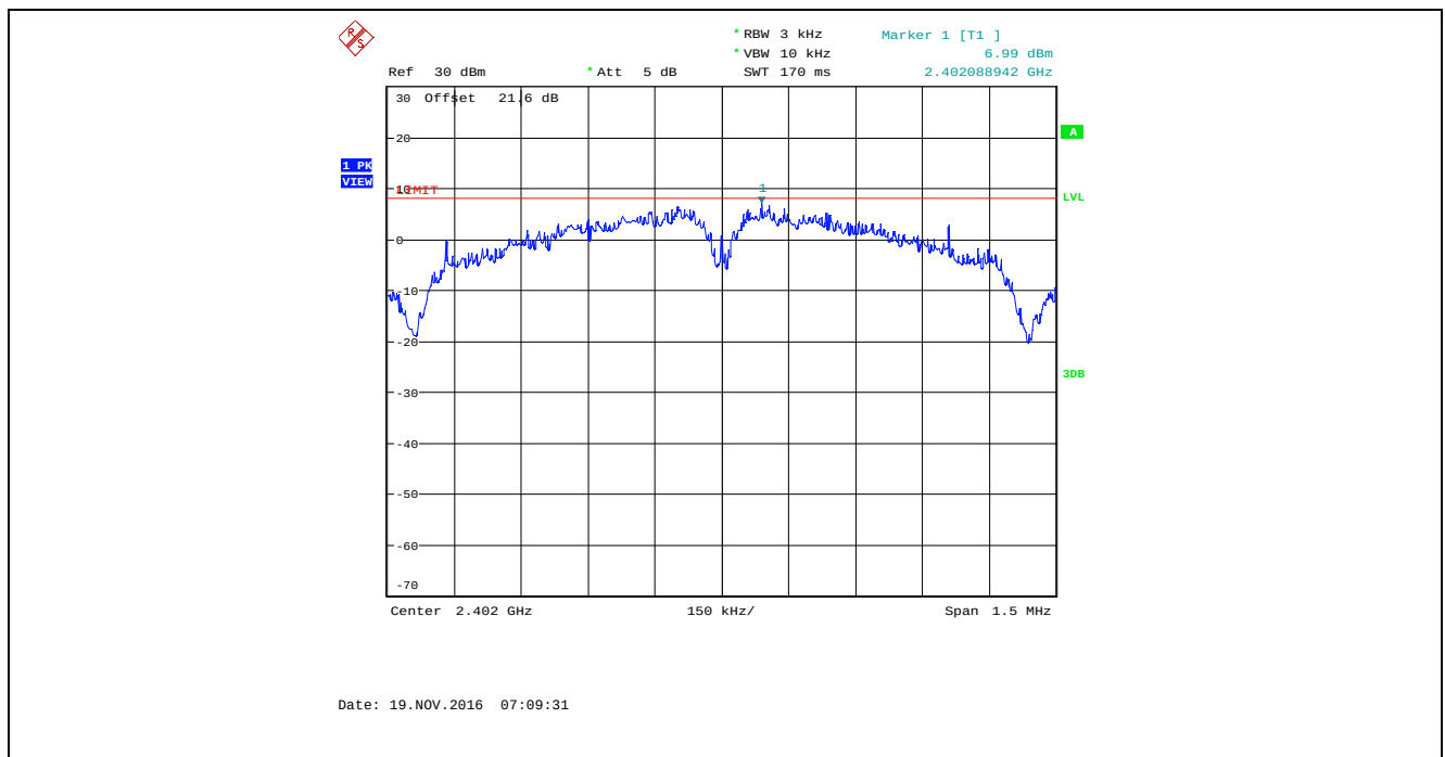
Plot 5.6.4.10. Power Spectral Density, Bandwidth: 2 MHz, TX Gain Setting: 32, Data Rate 2, 2402 MHz
