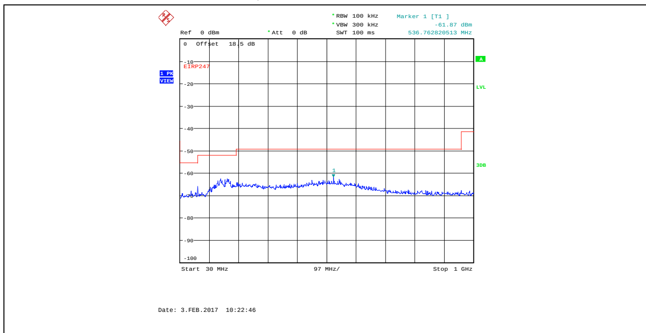
Plot 5.4.4.3.28. Conducted Spurious Emissions in Restricted Frequency Bands Bandwidth: 8 MHz, TX Gain Setting 55, Data Rate 4, 2477 MHz, 30 MHz - 1 GHz, Peak Detector
