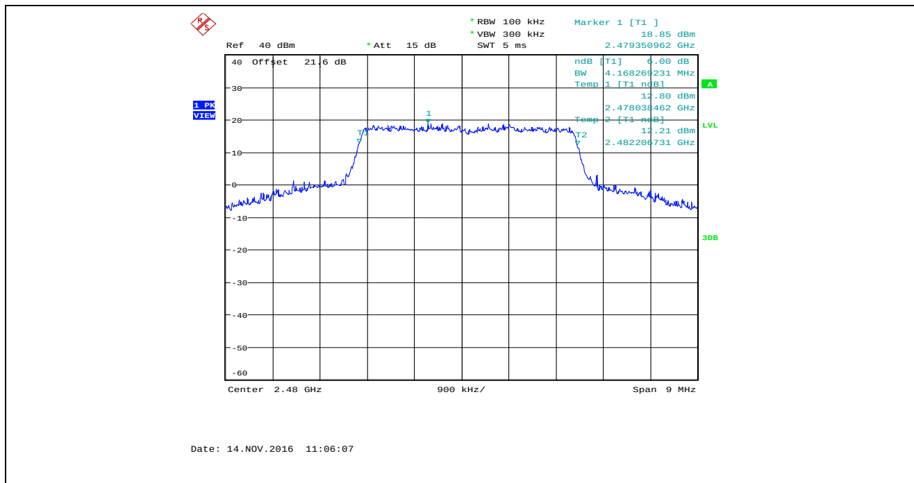
Plot 5.2.4.63. 6 dB Bandwidth, Bandwidth: 4 MHz, TX Gain: 50, Data Rate 5, 2480 MHz
