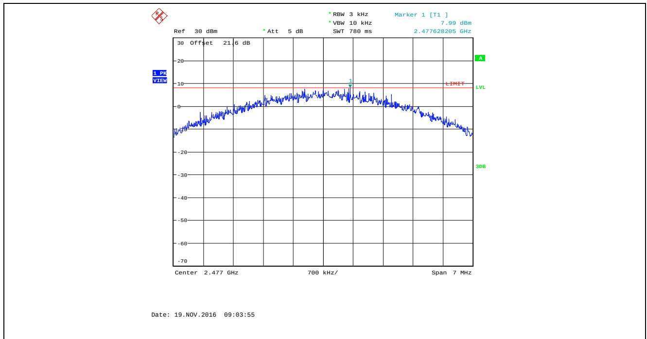
Plot 5.6.4.33. Power Spectral Density, Bandwidth: 8 MHz, TX Gain Setting: 50, Data Rate 3, 2477 MHz
