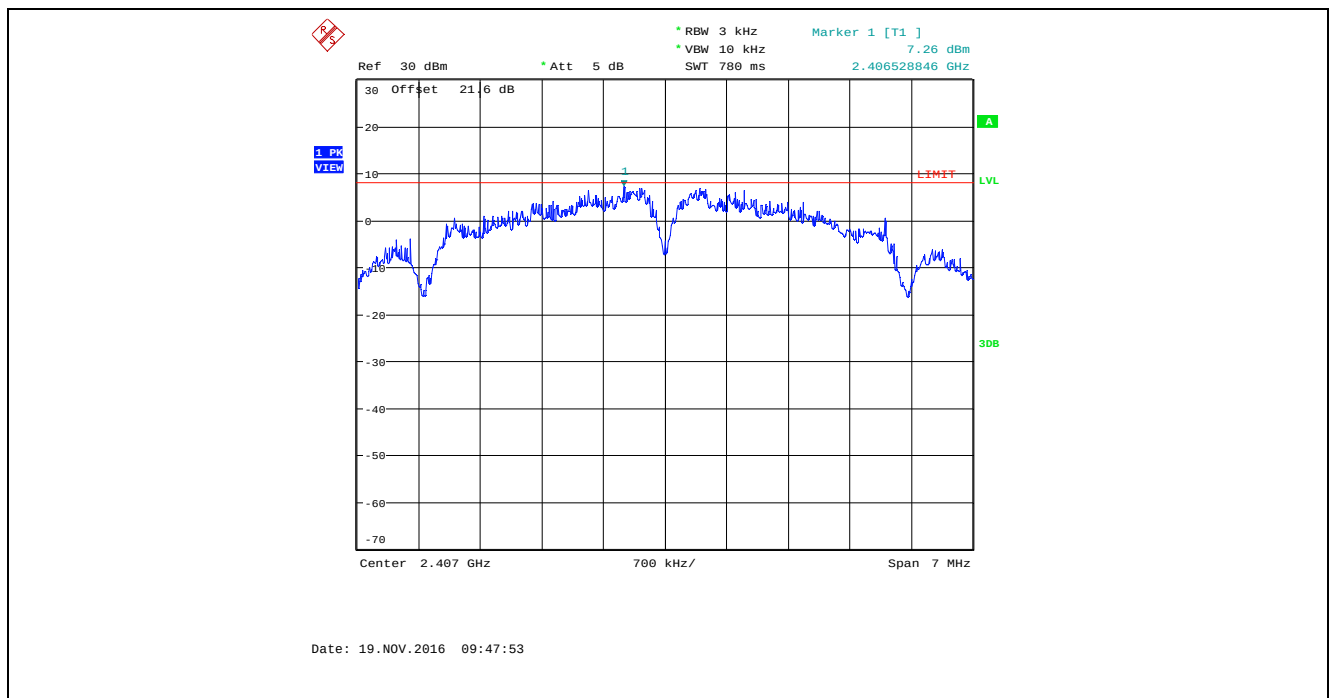
Plot 5.6.4.28. Power Spectral Density, Bandwidth: 8 MHz, TX Gain Setting: 50, Data Rate 2, 2407 MHz
