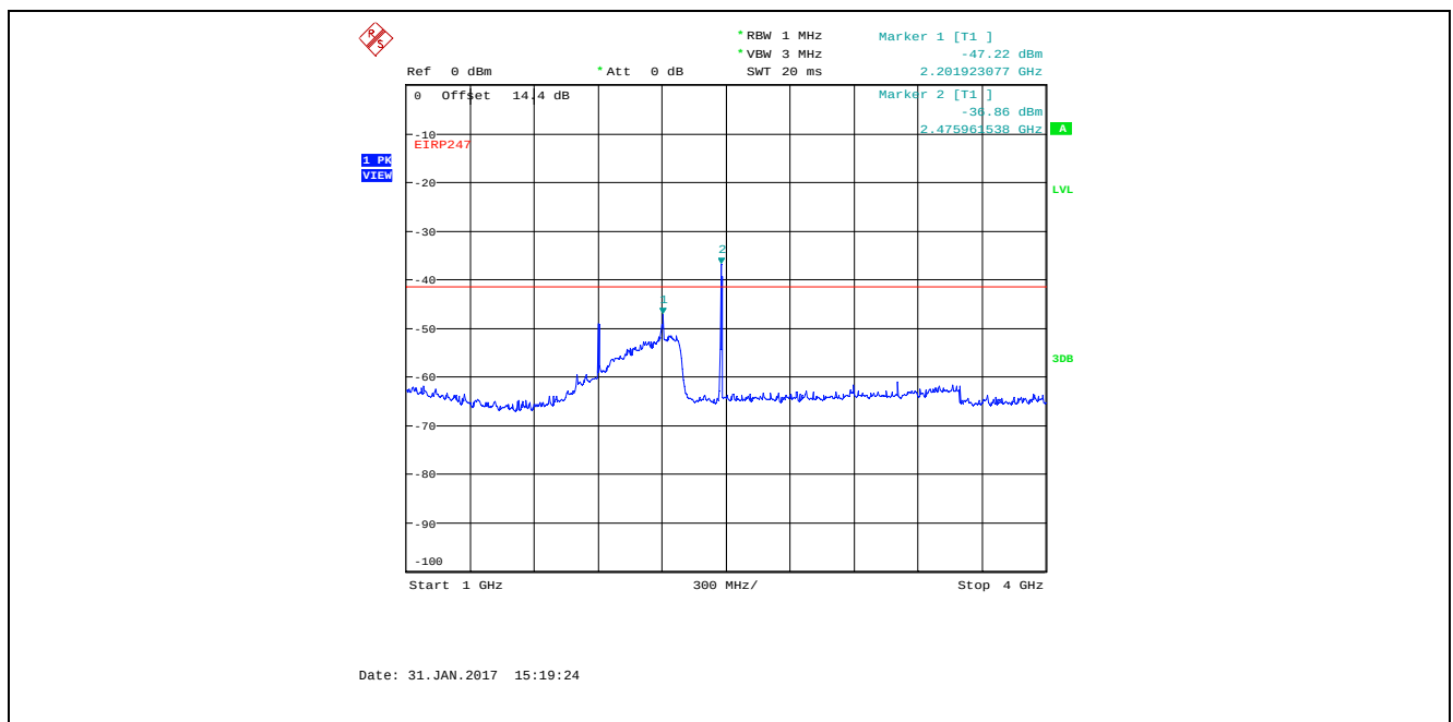
Plot 5.4.4.4.14. Conducted Spurious Emissions in Restricted Frequency Bands Bandwidth: 8 MHz, TX Gain Setting 25, Data Rate 1, 2477 MHz, 1 GHz - 4 GHz, Peak Detector Marker 2 is the Fundamental
