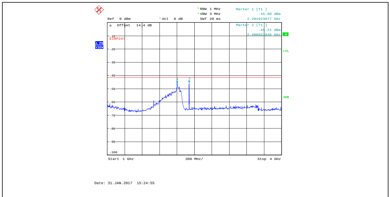
Plot 5.4.4.4.4. Conducted Spurious Emissions in Restricted Frequency Bands Bandwidth: 8 MHz, TX Gain Setting 25, Data Rate 1, 2407 MHz, 1 GHz - 4 GHz, Peak Detector
