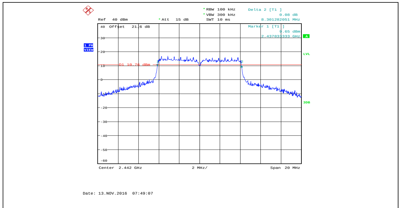
Plot 5.2.4.71. 6 dB Bandwidth, Bandwidth: 8 MHz, TX Gain: 55, Data Rate 4, 2442 MHz
