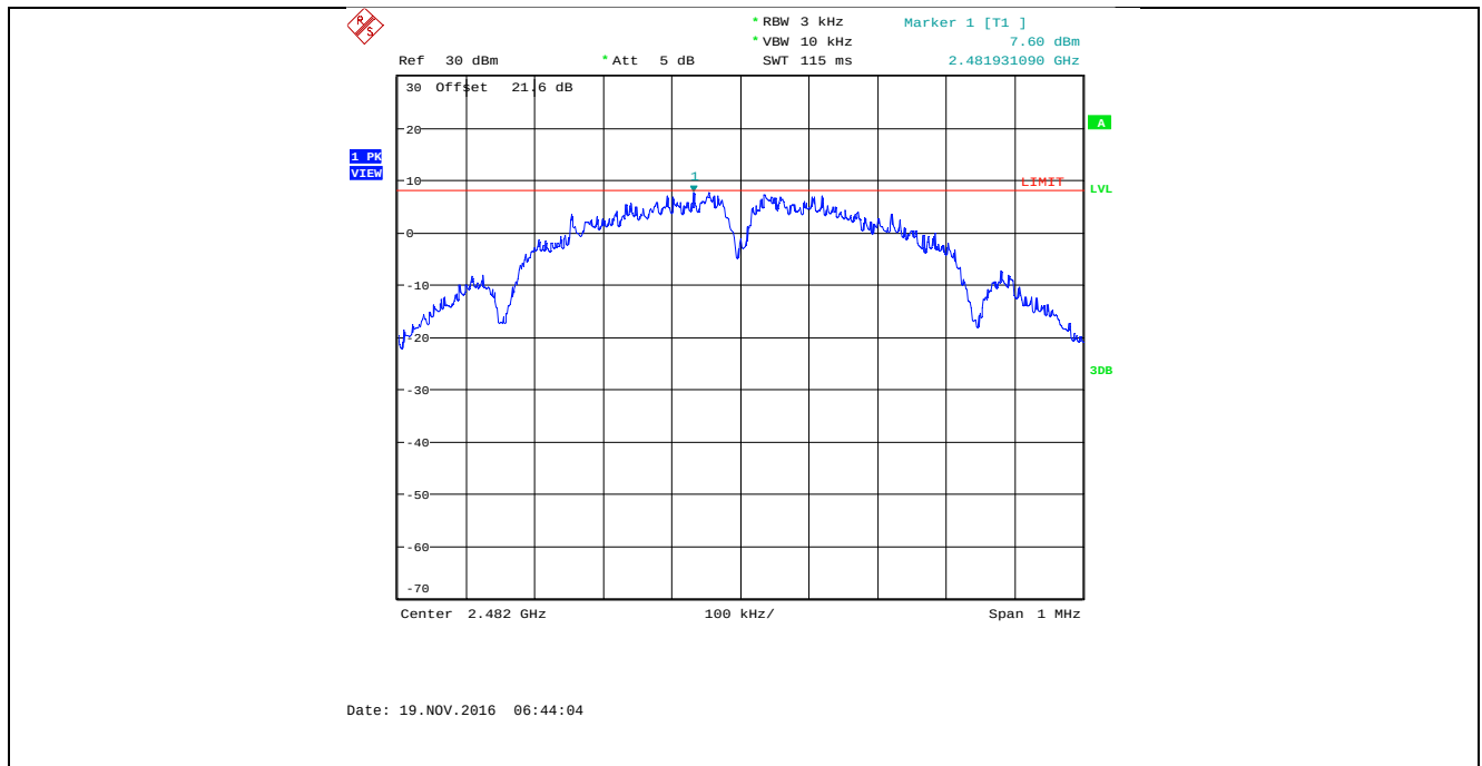
Plot 5.6.4.6. Power Spectral Density, Bandwidth: 1 MHz, TX Gain Setting: 26, Data Rate 2, 2482 MHz
