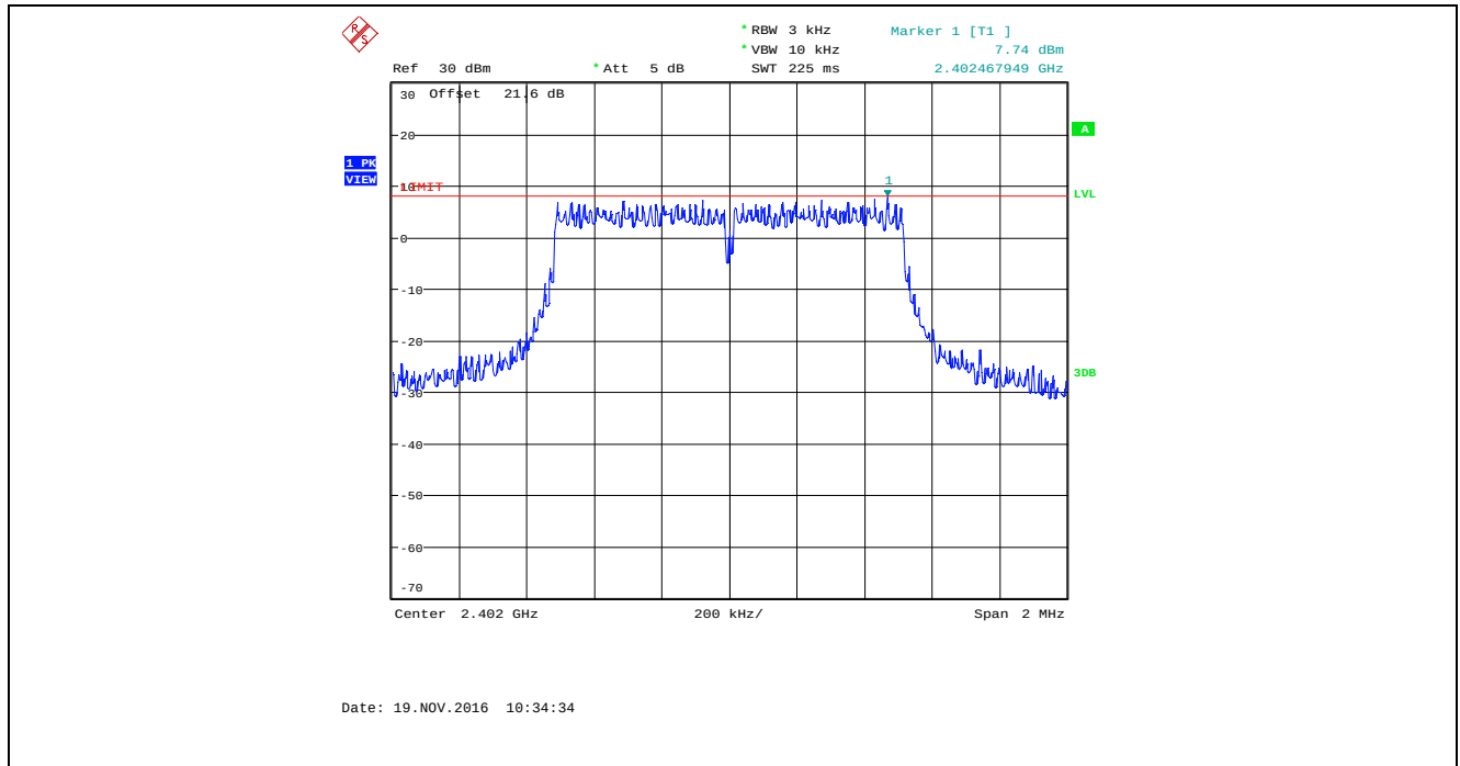
Plot 5.6.4.34. Power Spectral Density, Bandwidth: 1 MHz, TX Gain Setting: 43, Data Rate 4, 2402 MHz
