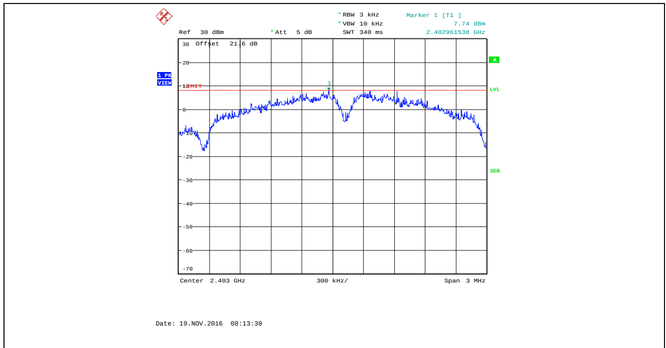
Plot 5.6.4.16. Power Spectral Density, Bandwidth: 4 MHz, TX Gain Setting: 43, Data Rate 1, 2403 MHz
