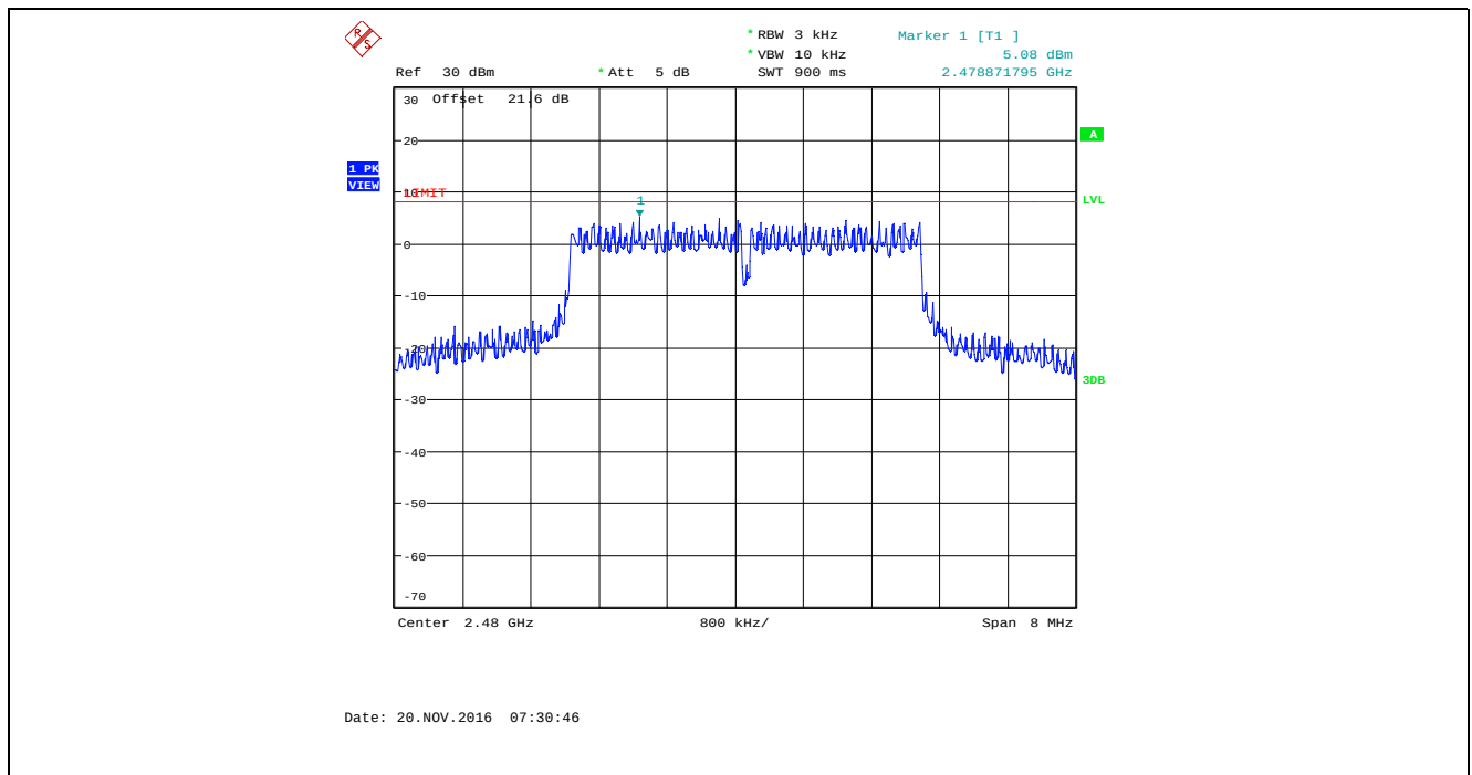
Plot 5.6.4.66. Power Spectral Density, Bandwidth: 4 MHz, TX Gain Setting: 50, Data Rate 6, 2480 MHz
