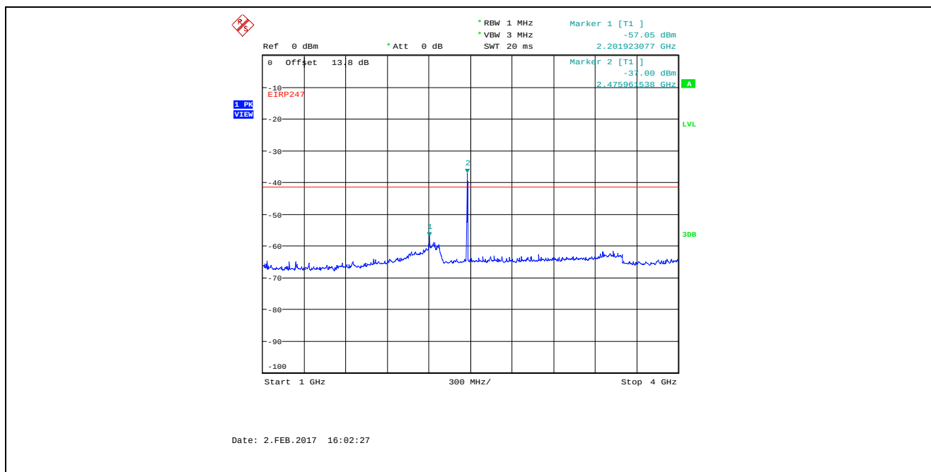
Plot 5.4.4.3.14. Conducted Spurious Emissions in Restricted Frequency Bands Bandwidth: 8 MHz, TX Gain Setting 50, Data Rate 1, 2477 MHz, 1 GHz - 4 GHz, Peak Detector Marker 2 is the Fundamental
