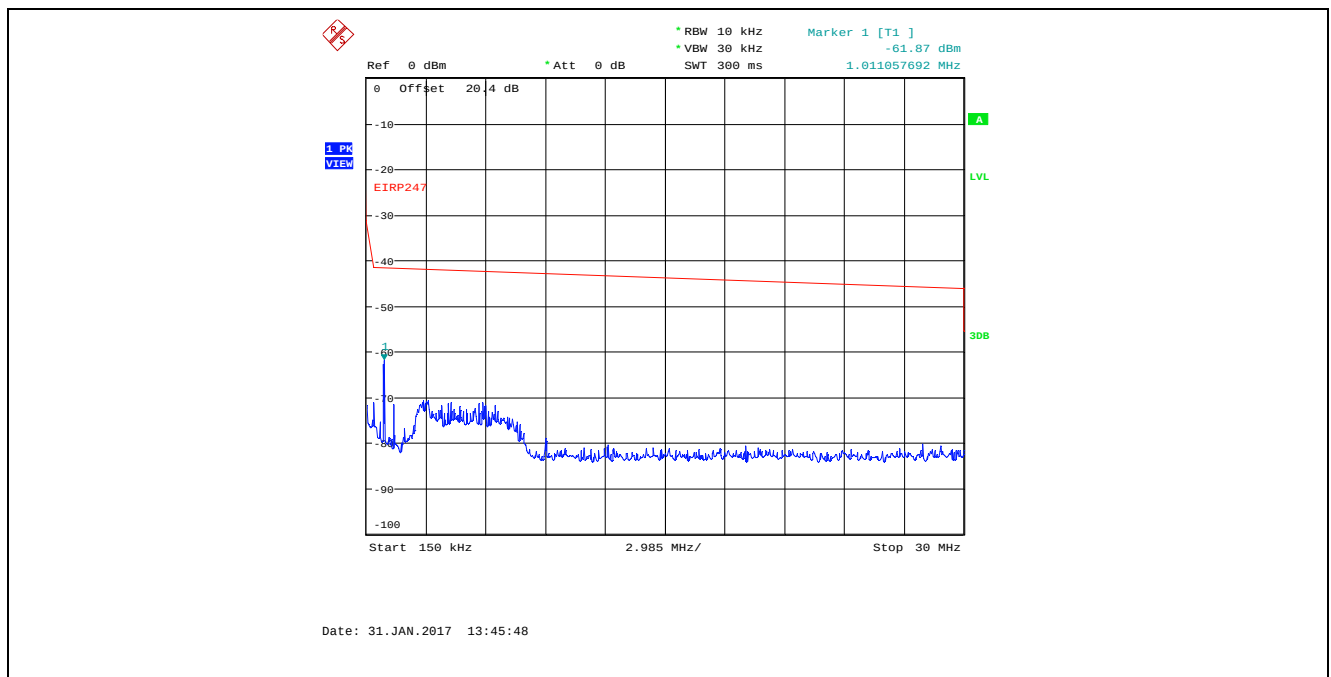
Plot 5.4.4.17. Conducted Spurious Emissions in Restricted Frequency Bands Bandwidth: 8 MHz, TX Gain Setting 25, Data Rate 4, 2407 MHz, 150 kHz - 30 MHz, Peak Detector
