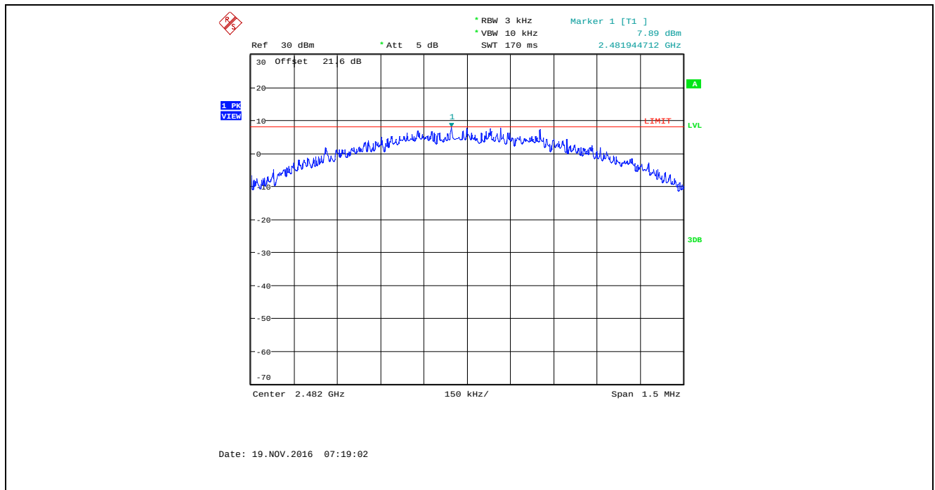
Plot 5.6.4.15. Power Spectral Density, Bandwidth: 2 MHz, TX Gain Setting: 32, Data Rate 3, 2482 MHz
