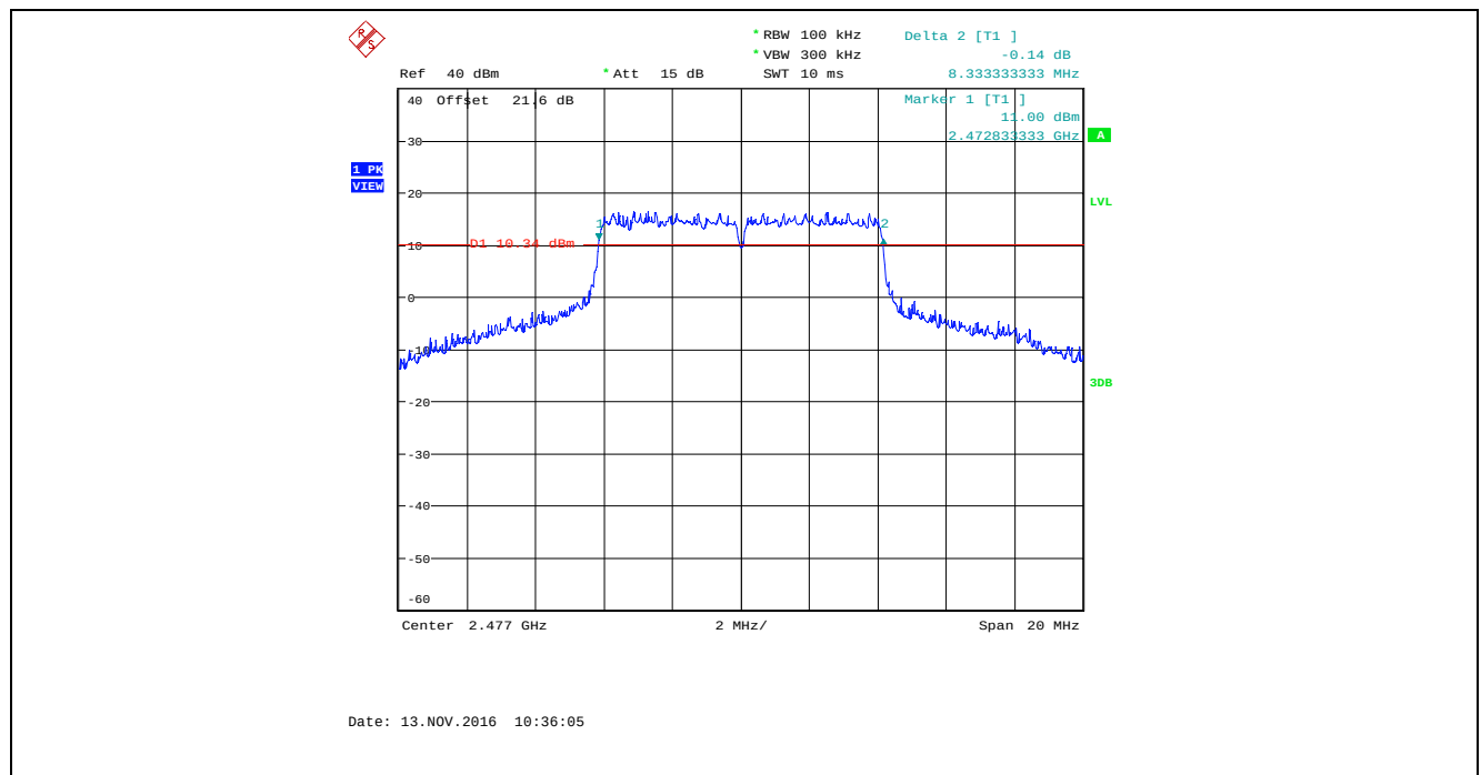
Plot 5.2.4.81. 6 dB Bandwidth, Bandwidth: 8 MHz, TX Gain: 55, Data Rate 7, 2477 MHz
