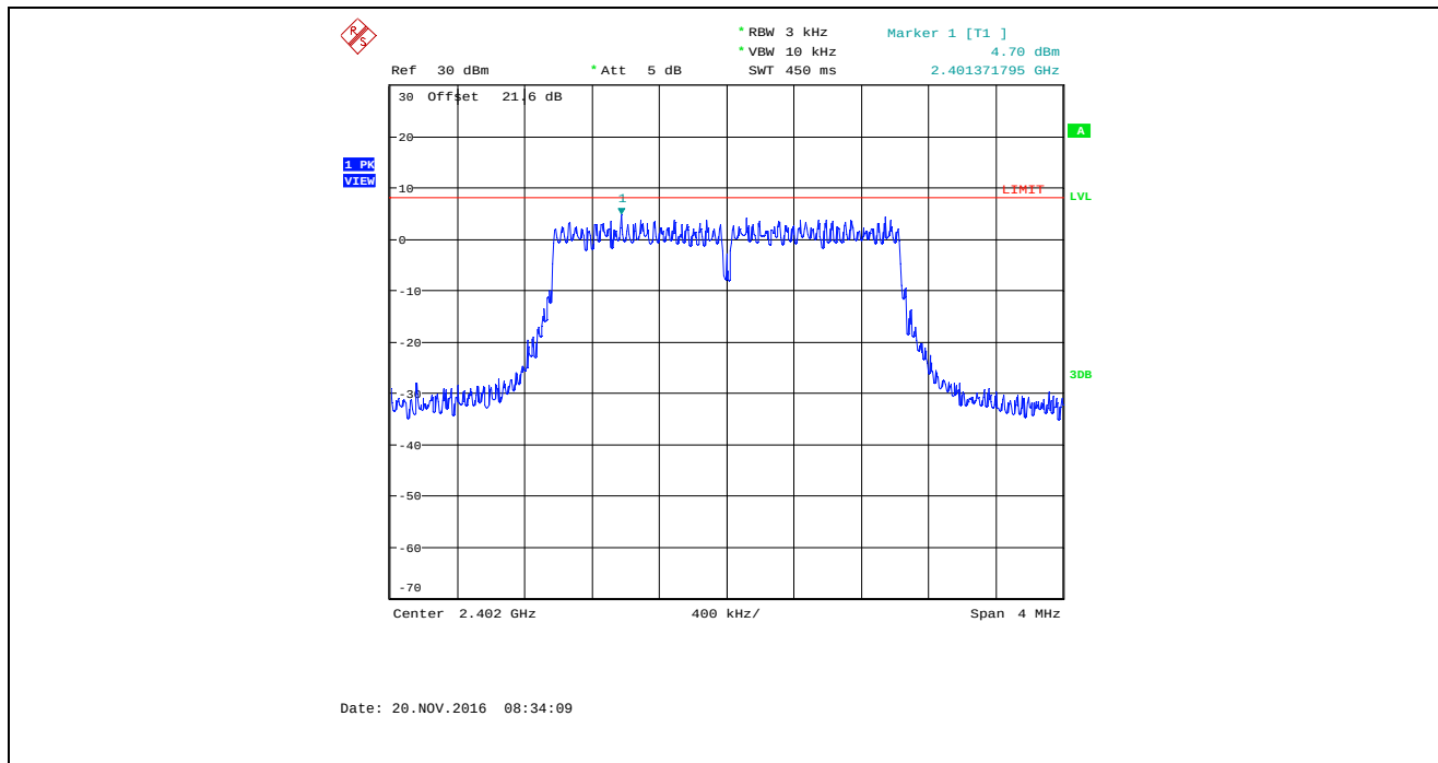
Plot 5.6.4.49. Power Spectral Density, Bandwidth: 2 MHz, TX Gain Setting: 45, Data Rate 5, 2402 MHz
