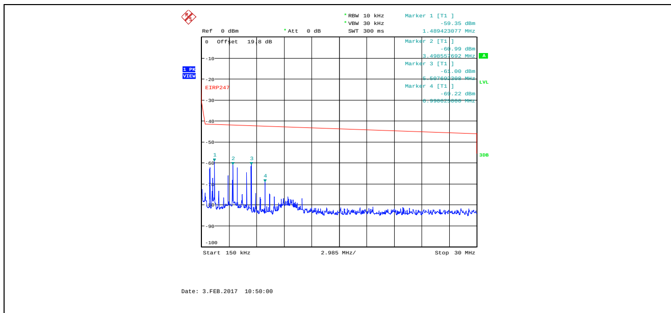
Plot 5.4.4.3.2. Conducted Spurious Emissions in Restricted Frequency Bands Bandwidth: 8 MHz, TX Gain Setting 50, Data Rate 1, 2407 MHz, 150 kHz - 30 MHz, Peak Detector
