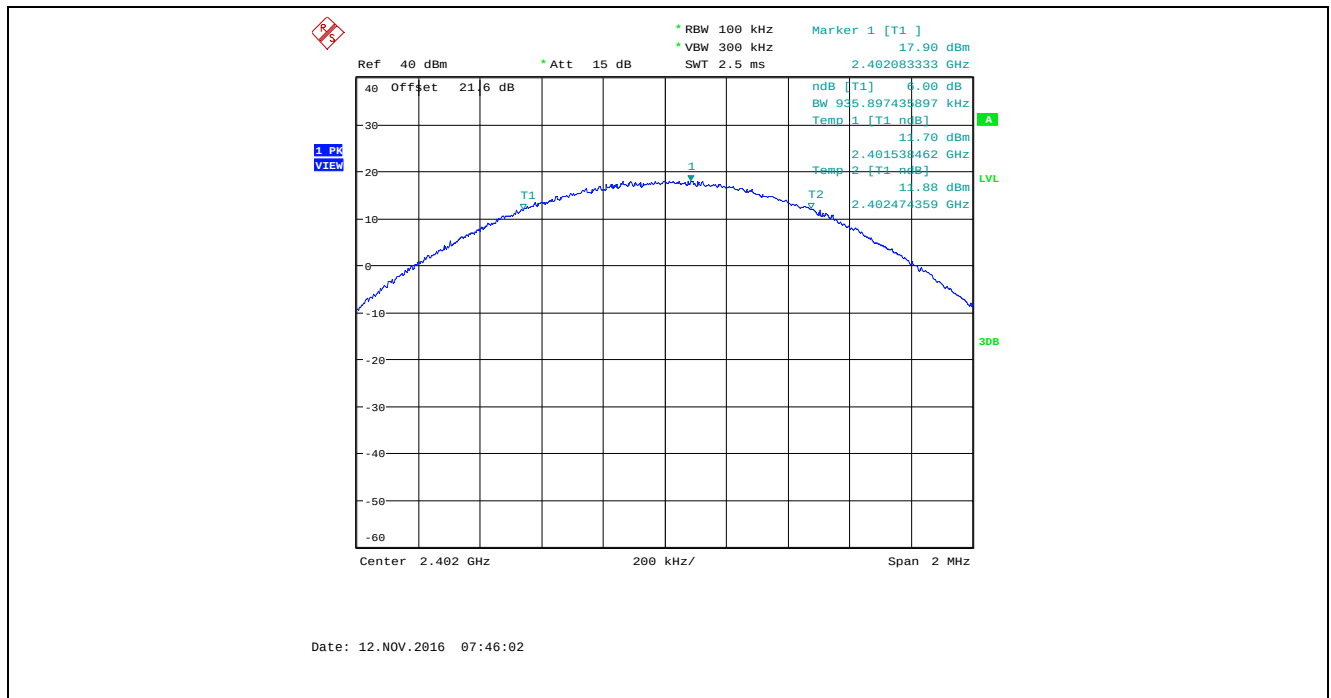
Plot 5.2.4.13. 6 dB Bandwidth, Bandwidth: 2 MHz, TX Gain: 32, Data Rate 3, 2402 MHz
