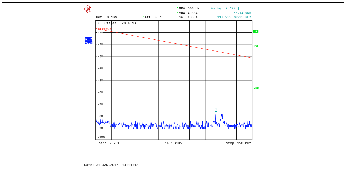
Plot 5.4.4.4.11. Conducted Spurious Emissions in Restricted Frequency Bands Bandwidth: 8 MHz, TX Gain Setting 25, Data Rate 1, 2477 MHz, 9 kHz - 150 kHz, Peak Detector
