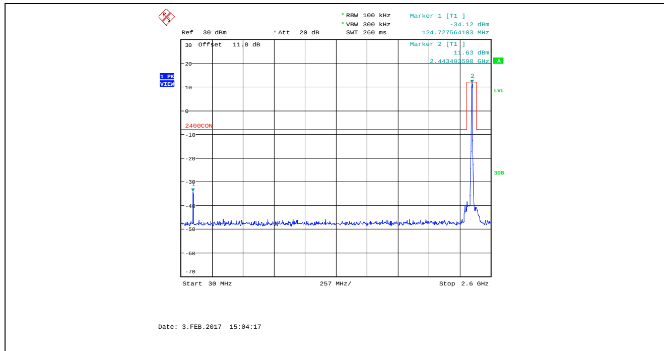
Plot 5.4.4.2.9. Conducted Spurious Emissions in Non-restricted Frequency Bands Bandwidth: 8 MHz, TX Gain: 55, Data Rate 4, 2442 MHz, 30 MHz – 2.6 GHz
