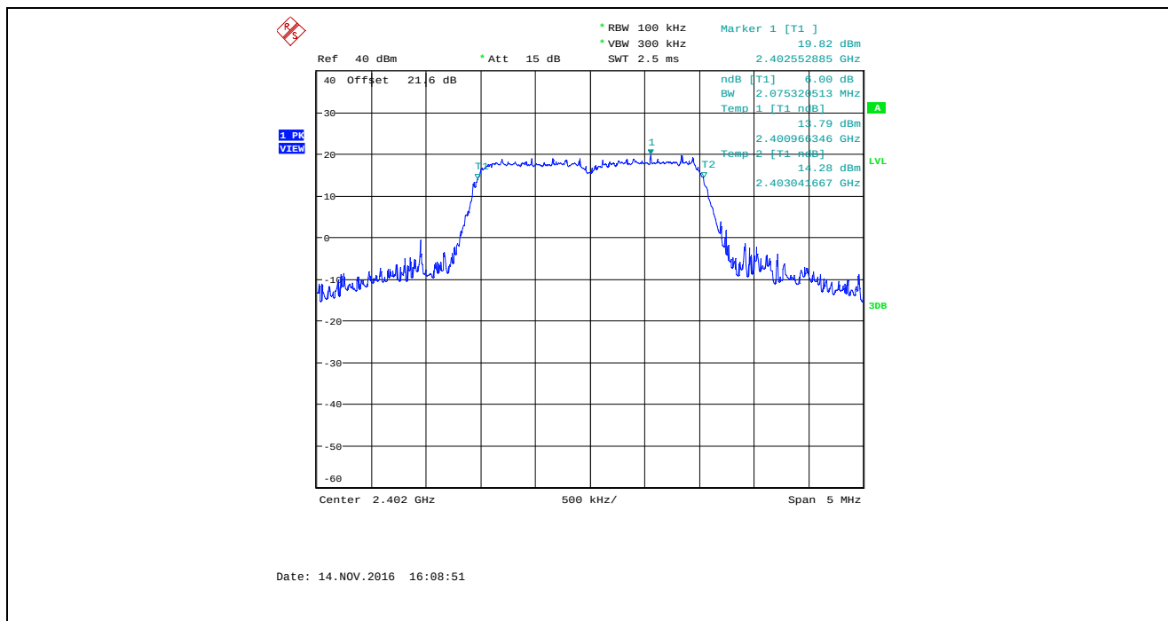
Plot 5.2.4.46. 6 dB Bandwidth, Bandwidth: 2 MHz, TX Gain: 45, Data Rate 4, 2402 MHz
