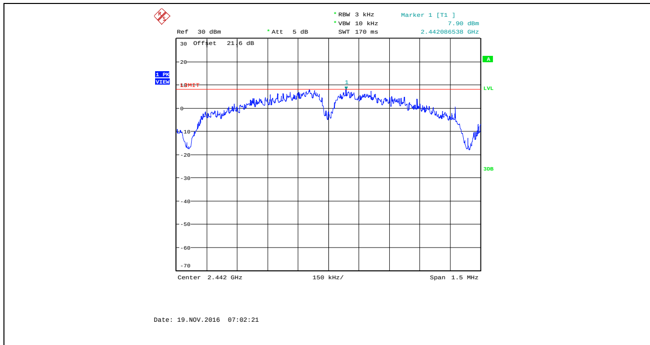
Plot 5.6.4.8. Power Spectral Density, Bandwidth: 2 MHz, TX Gain Setting: 32, Data Rate 1, 2442 MHz
