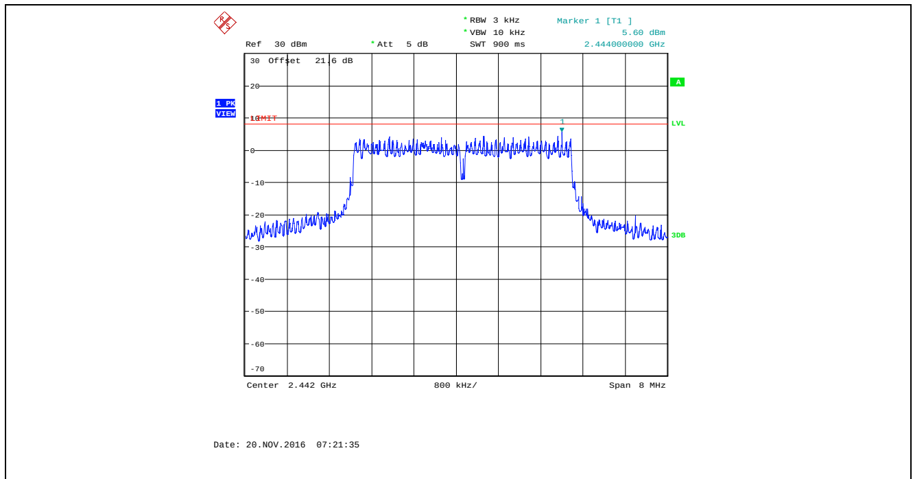
Plot 5.6.4.68. Power Spectral Density, Bandwidth: 4 MHz, TX Gain Setting: 50, Data Rate 7, 2442 MHz
