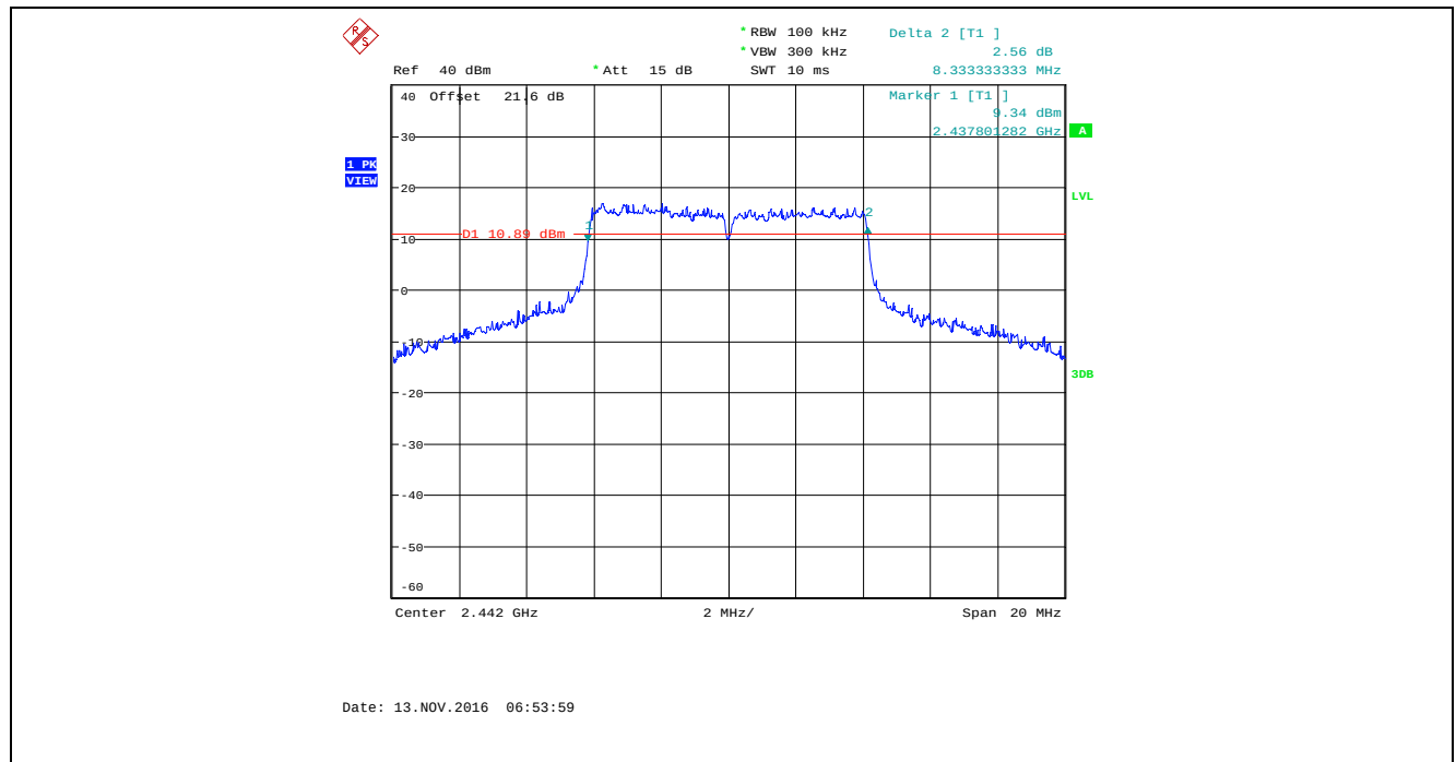
Plot 5.2.4.80. 6 dB Bandwidth, Bandwidth: 8 MHz, TX Gain: 55, Data Rate 7, 2442 MHz
