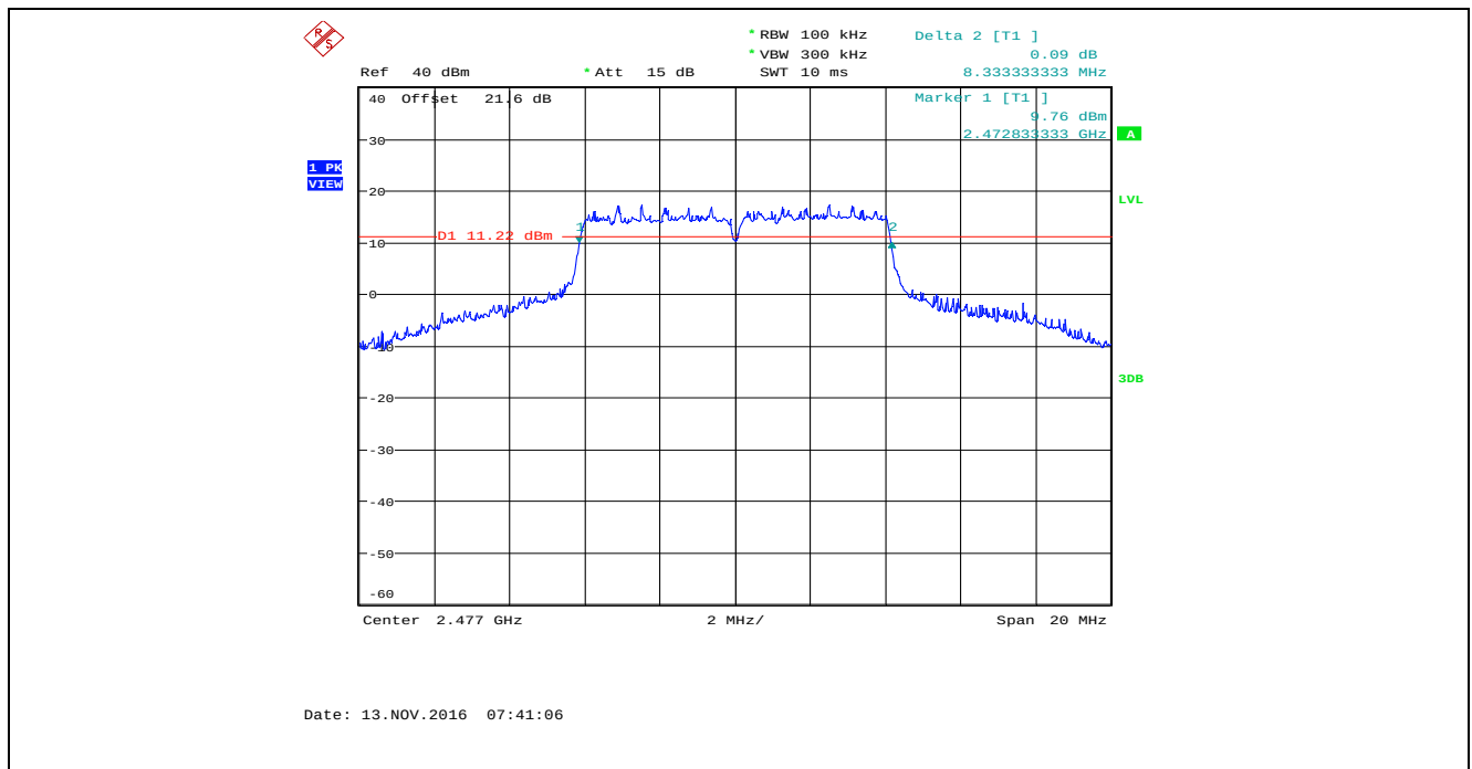
Plot 5.2.4.75. 6 dB Bandwidth, Bandwidth: 8 MHz, TX Gain: 55, Data Rate 5, 2477 MHz
