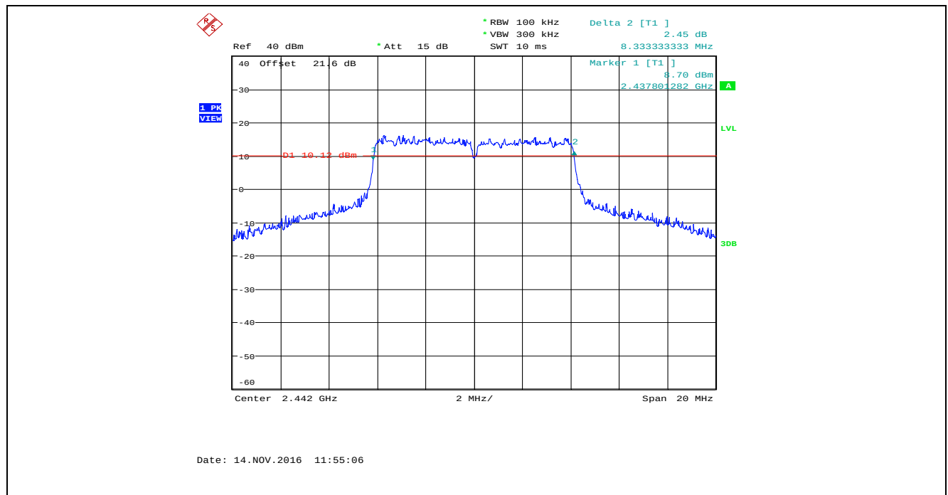
Plot 5.2.4.77. 6 dB Bandwidth, Bandwidth: 8 MHz, TX Gain: 55, Data Rate 6, 2442 MHz
