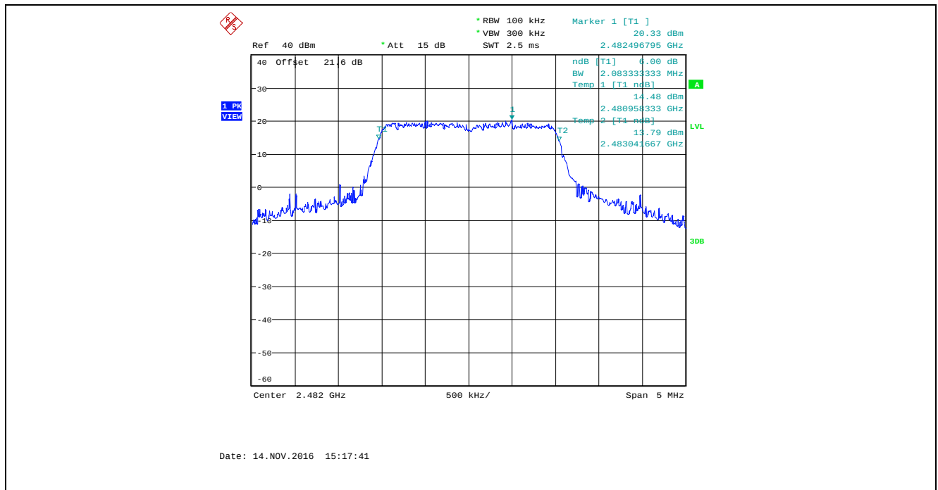
Plot 5.2.4.57. 6 dB Bandwidth, Bandwidth: 2 MHz, TX Gain: 45, Data Rate 7, 2482 MHz
