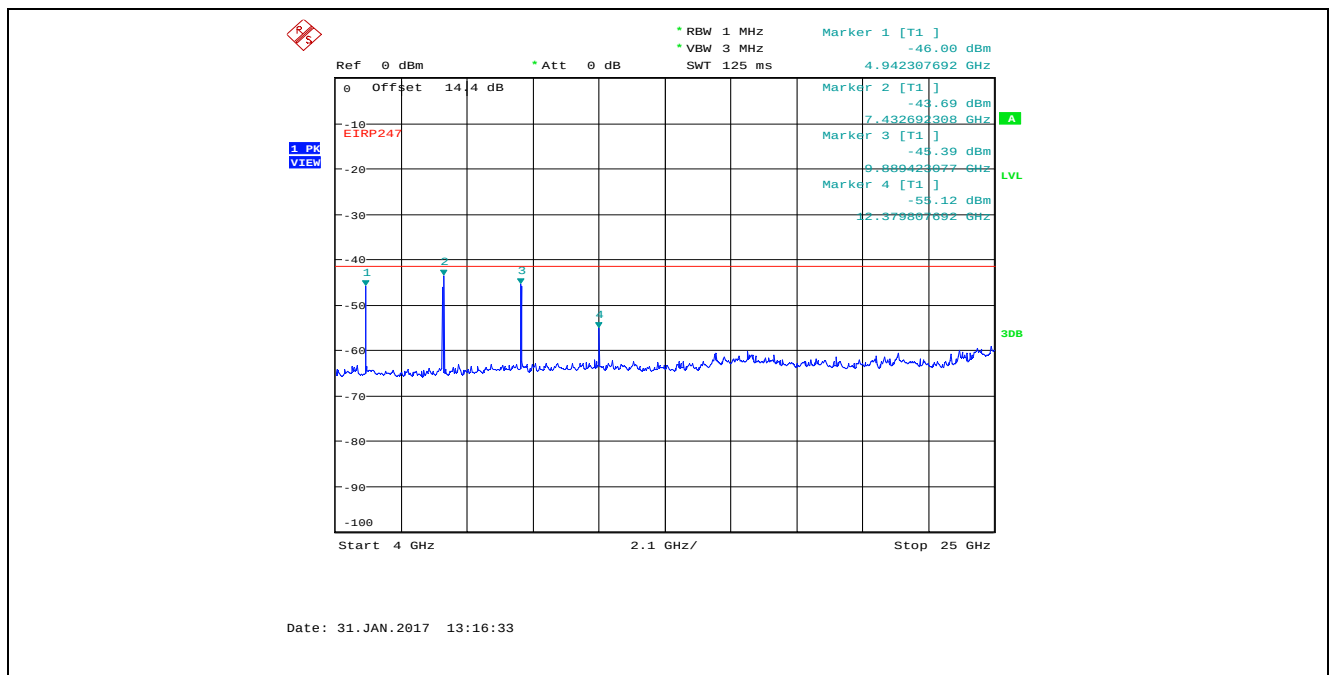
Plot 5.4.4.4.35. Conducted Spurious Emissions in Restricted Frequency Bands Bandwidth: 8 MHz, TX Gain Setting 25, Data Rate 4, 2477 MHz, 4 GHz - 25 GHz, Peak Detector
