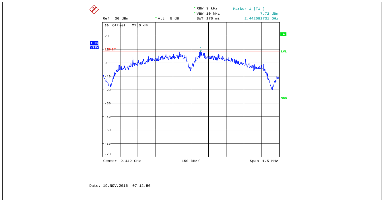
Plot 5.6.4.11. Power Spectral Density, Bandwidth: 2 MHz, TX Gain Setting: 32, Data Rate 2, 2442 MHz
