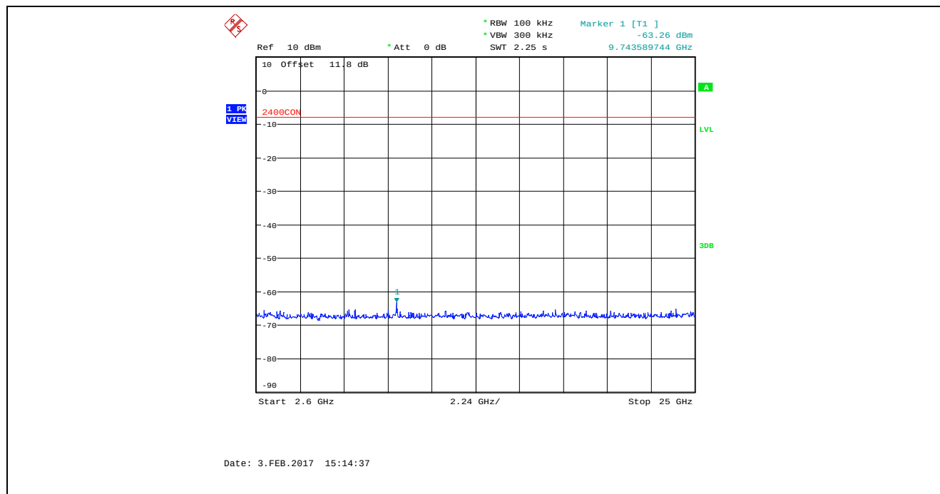
Plot 5.4.4.2.10. Conducted Spurious Emissions in Non-restricted Frequency Bands Bandwidth: 8 MHz, TX Gain: 55, Data Rate 4, 2442 MHz, 2.6 GHz – 25 GHz
