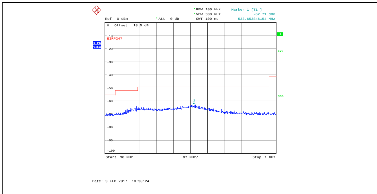
Plot 5.4.4.3.8. Conducted Spurious Emissions in Restricted Frequency Bands Bandwidth: 8 MHz, TX Gain Setting 50, Data Rate 1, 2442 MHz, 30 MHz - 1 GHz, Peak Detector
