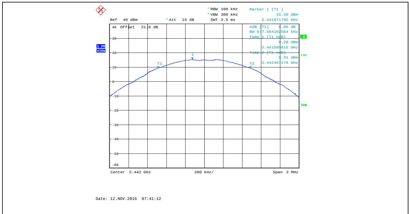
Plot 5.2.4.11. 6 dB Bandwidth, Bandwidth: 2 MHz, TX Gain: 32, Data Rate 2, 2442 MHz
