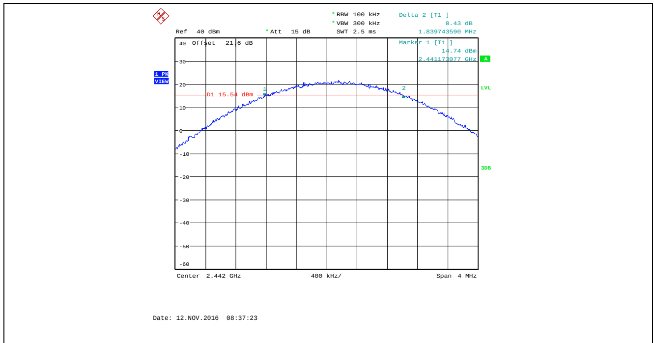
Plot 5.2.4.23. 6 dB Bandwidth, Bandwidth: 4 MHz, TX Gain: 43, Data Rate 3, 2442 MHz
