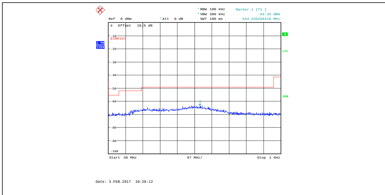
Plot 5.4.4.3.13. Conducted Spurious Emissions in Restricted Frequency Bands Bandwidth: 8 MHz, TX Gain Setting 50, Data Rate 1, 2477 MHz, 30 MHz - 1 GHz, Peak Detector
