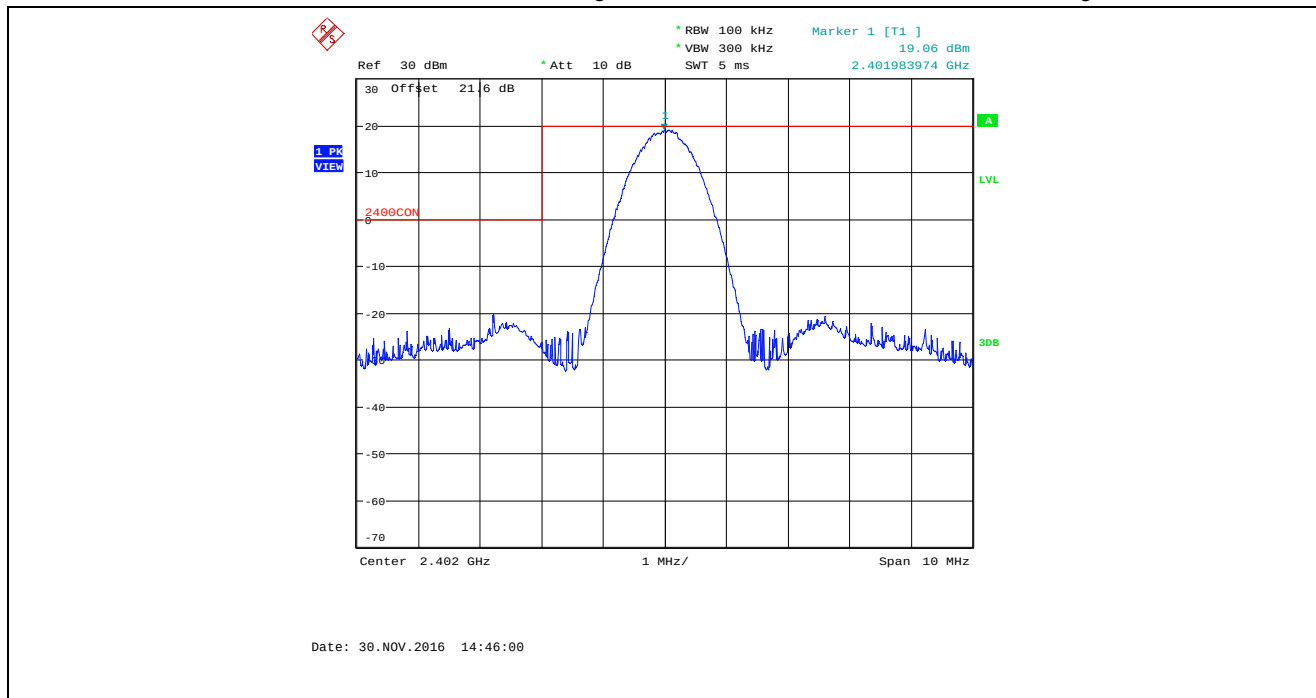
Plot 5.4.4.1.3. Band-Edge RF Conducted Emissions Bandwidth: 2 MHz, TX Gain Setting: 32 Data Rate 3, 2402 MHz, Lower Band-edge
