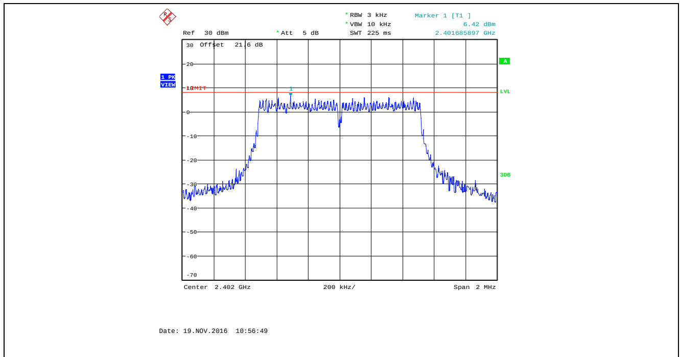
Plot 5.6.4.40. Power Spectral Density, Bandwidth: 1 MHz, TX Gain Setting: 43, Data Rate 6, 2402 MHz
