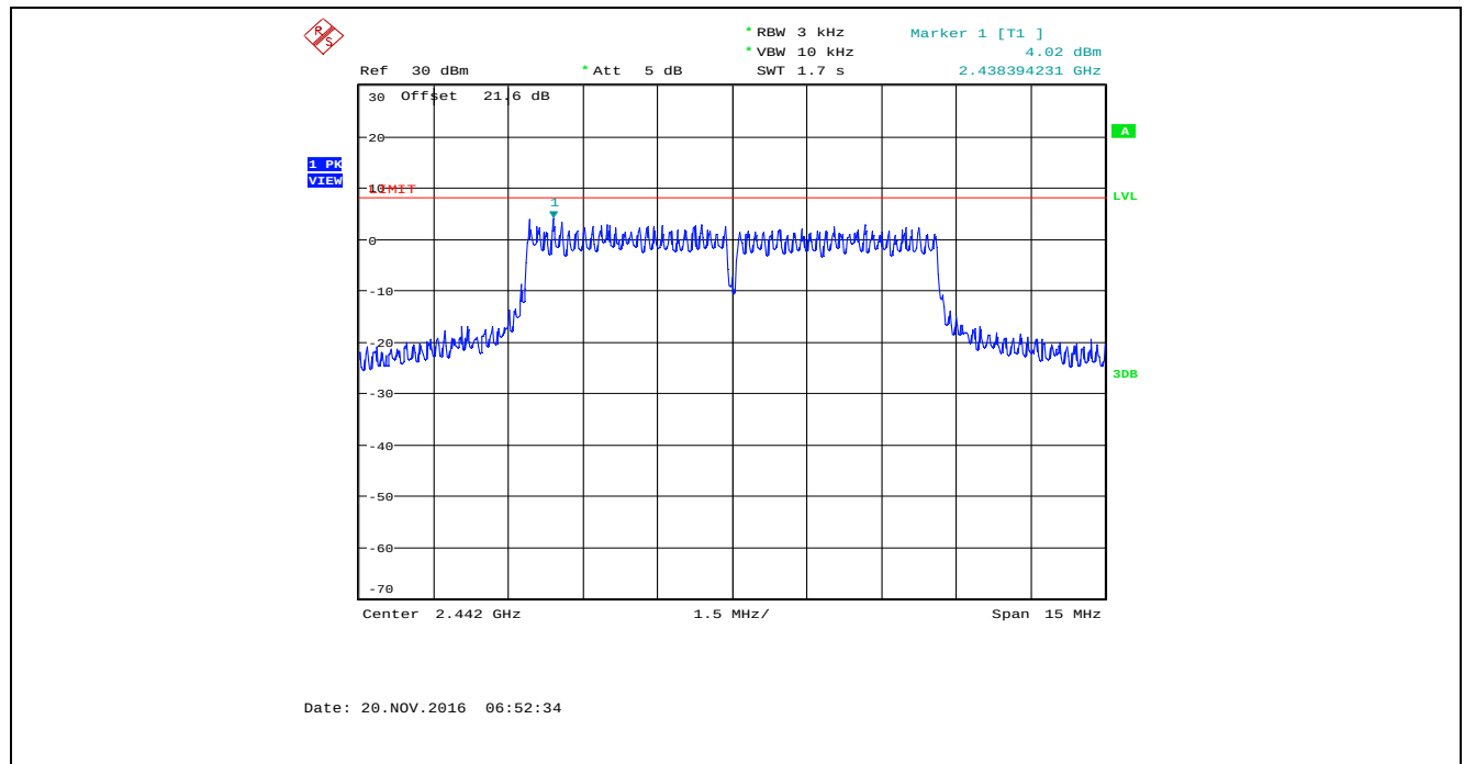
Plot 5.6.4.74. Power Spectral Density, Bandwidth: 8 MHz, TX Gain Setting: 55, Data Rate 5, 2442 MHz
