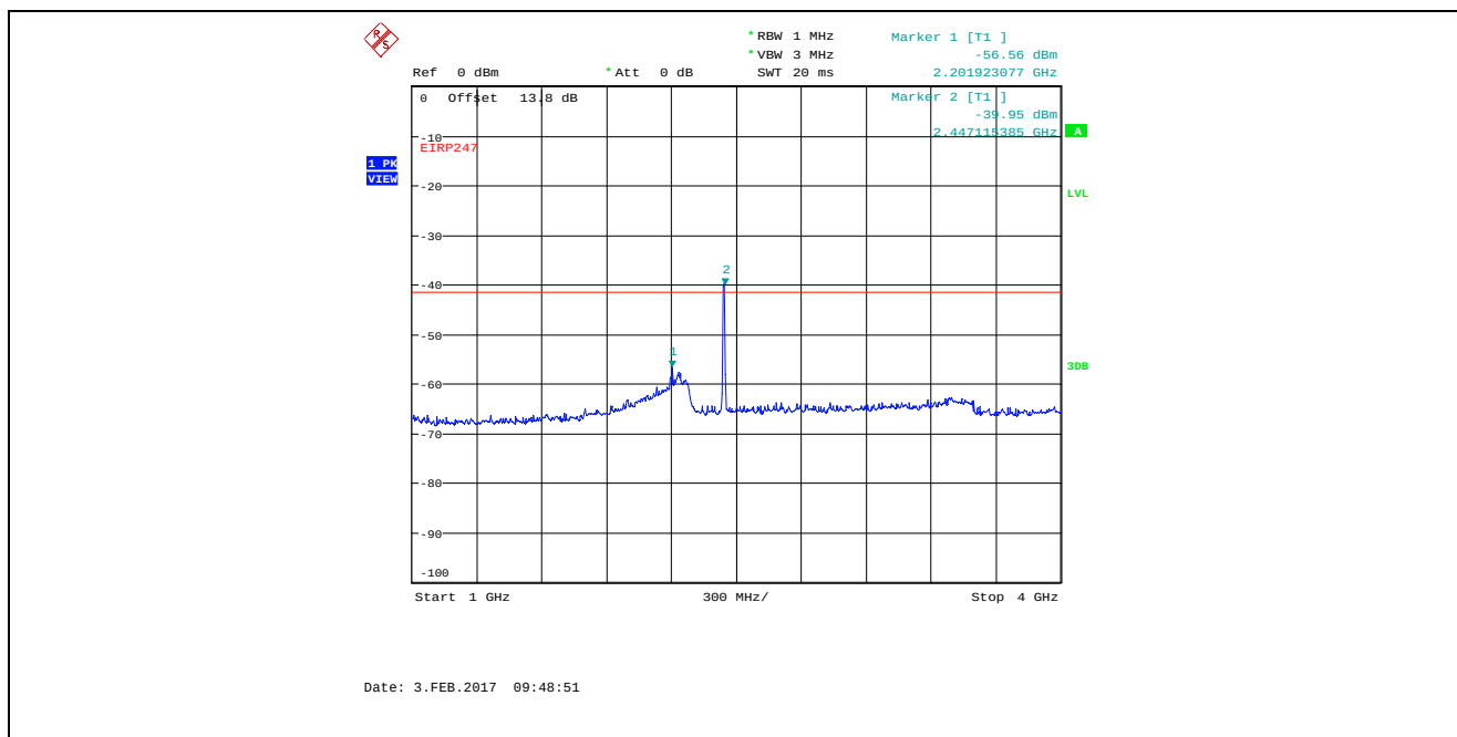
Plot 5.4.4.3.24. Conducted Spurious Emissions in Restricted Frequency Bands Bandwidth: 8 MHz, TX Gain Setting 55, Data Rate 4, 2442 MHz, 1 GHz - 4 GHz, Peak Detector Marker 2 is the Fundamental
