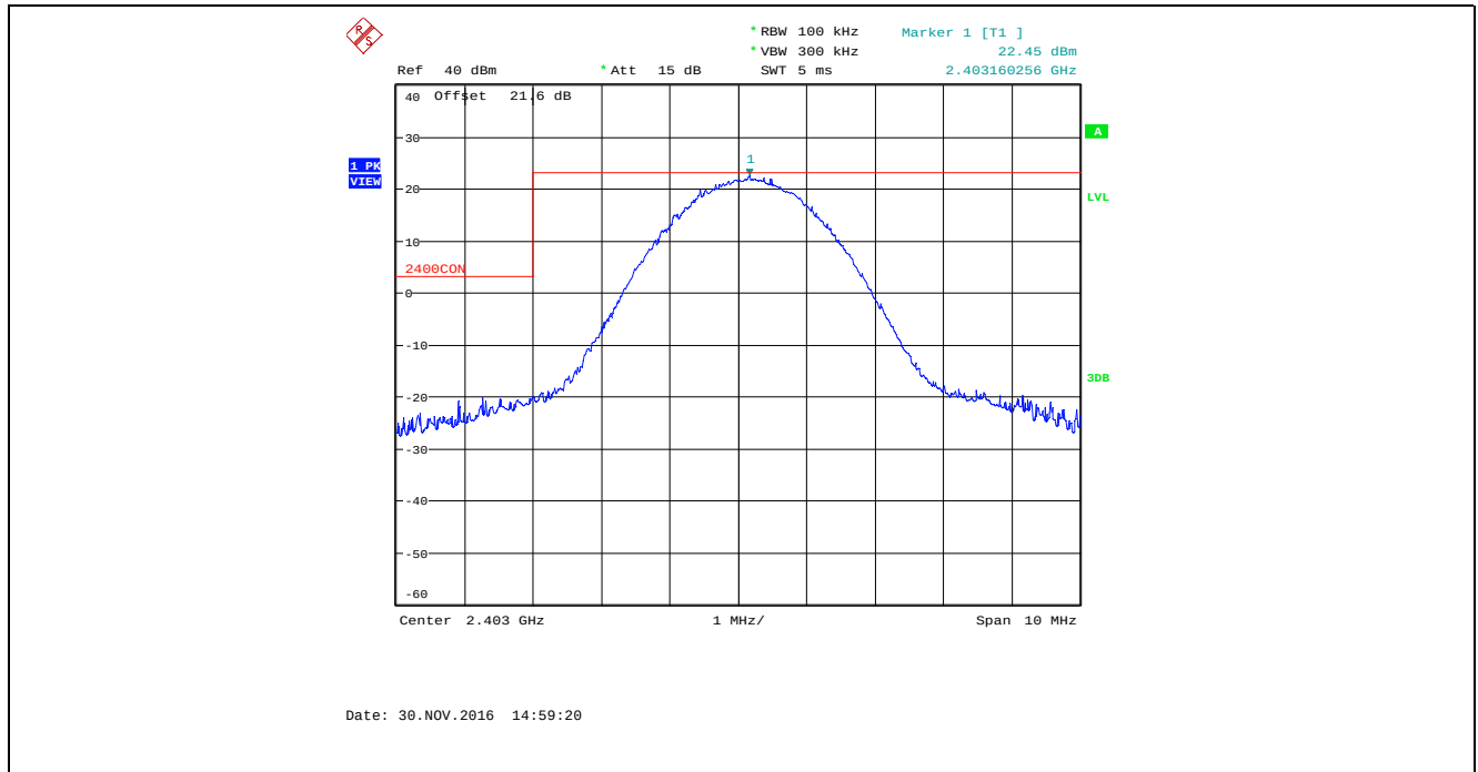
Plot 5.4.4.1.5. Band-Edge RF Conducted Emissions Bandwidth: 4 MHz, TX Gain Setting: 43, Data Rate 3, 2403 MHz, Lower Band-edge
