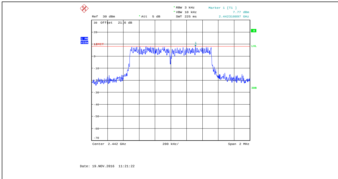
Plot 5.6.4.44. Power Spectral Density, Bandwidth: 1 MHz, TX Gain Setting: 43, Data Rate 7, 2442 MHz
