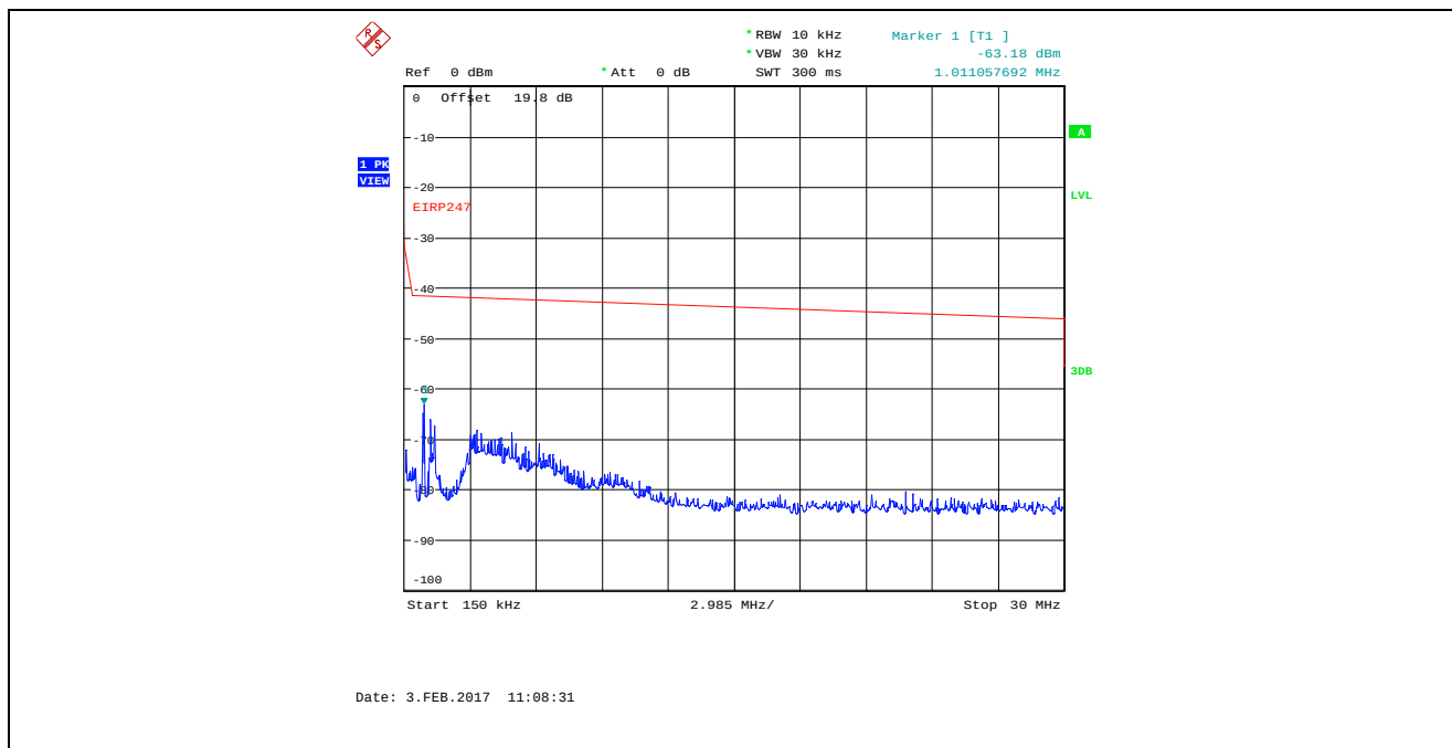
Plot 5.4.4.3.17. Conducted Spurious Emissions in Restricted Frequency Bands Bandwidth: 8 MHz, TX Gain Setting 55, Data Rate 4, 2407 MHz, 150 kHz - 30 MHz, Peak Detector
