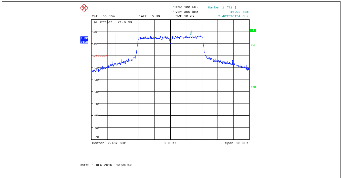
Plot 5.4.4.1.15. Band-Edge RF Conducted Emissions Bandwidth: 8 MHz, TX Gain Setting: 55, Data Rate 7, 2407 MHz, Lower Band-edge
