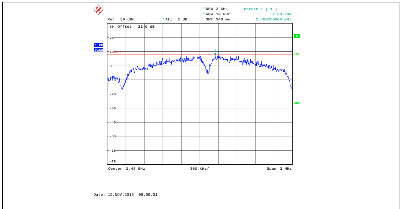
Plot 5.6.4.18. Power Spectral Density, Bandwidth: 4 MHz, TX Gain Setting: 43, Data Rate 1, 2480 MHz
