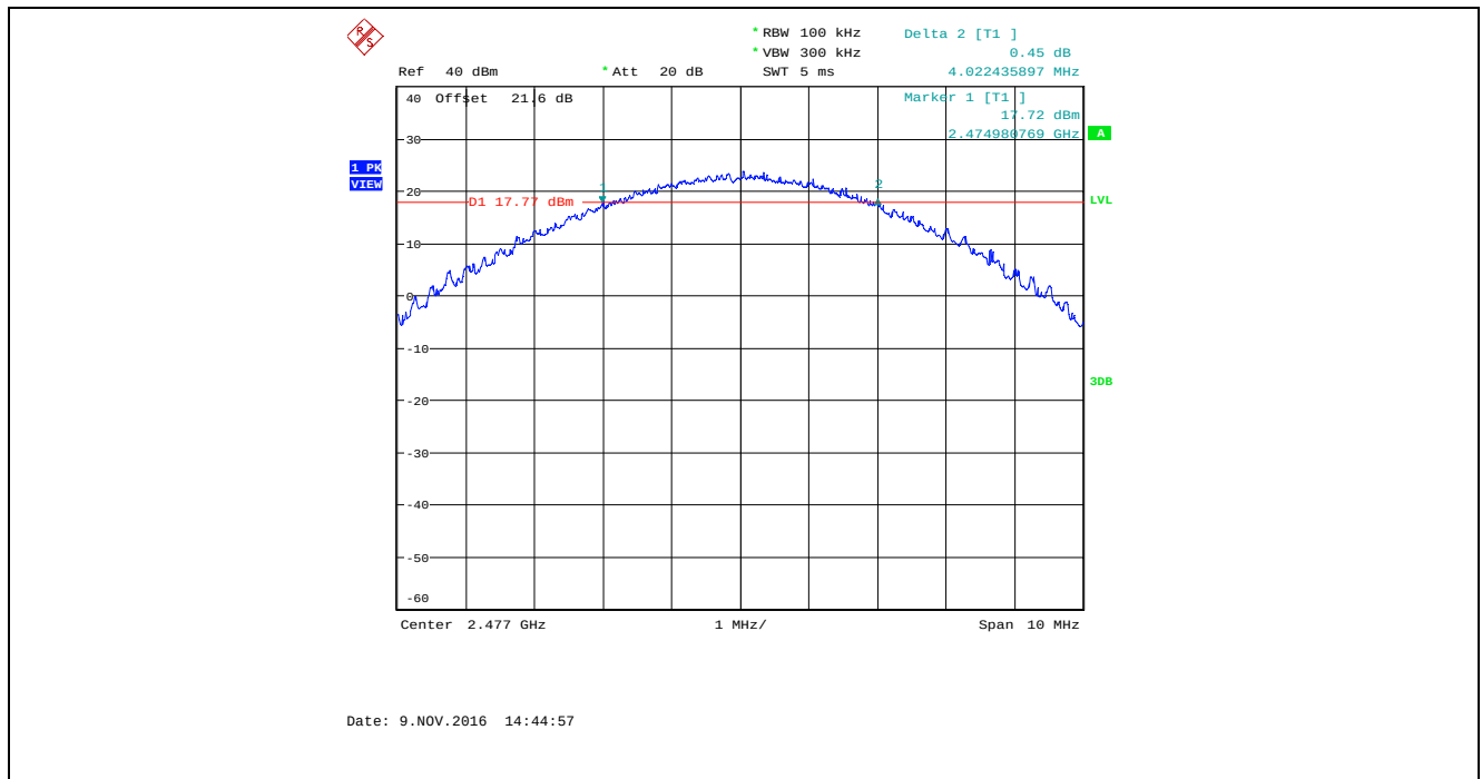
Plot 5.2.4.33. 6 dB Bandwidth, Bandwidth: 8 MHz, TX Gain: 50, Data Rate 3, 2477 MHz
