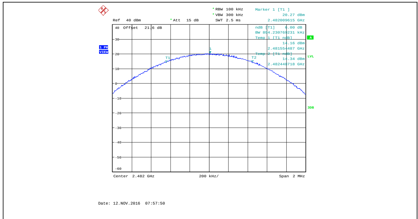
Plot 5.2.4.15. 6 dB Bandwidth, Bandwidth: 2 MHz, TX Gain: 32, Data Rate 3, 2482 MHz
