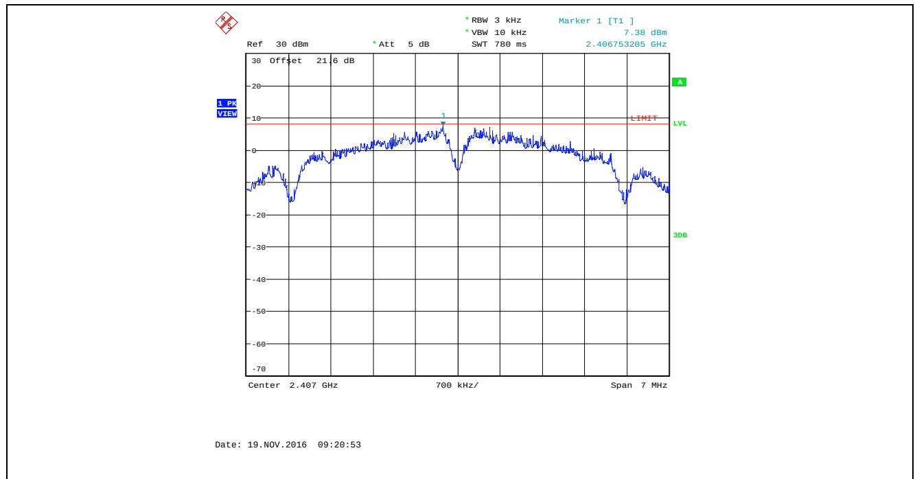
Plot 5.6.4.25. Power Spectral Density, Bandwidth: 8 MHz, TX Gain Setting: 50, Data Rate 1, 2407 MHz
