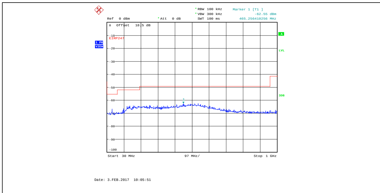
Plot 5.4.4.3.23. Conducted Spurious Emissions in Restricted Frequency Bands Bandwidth: 8 MHz, TX Gain Setting 55, Data Rate 4, 2442 MHz, 30 MHz - 1 GHz, Peak Detector
