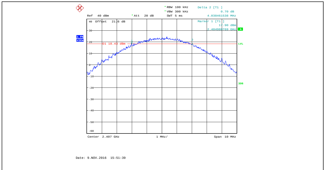
Plot 5.2.4.31. 6 dB Bandwidth, Bandwidth: 8 MHz, TX Gain: 50, Data Rate 3, 2407 MHz
