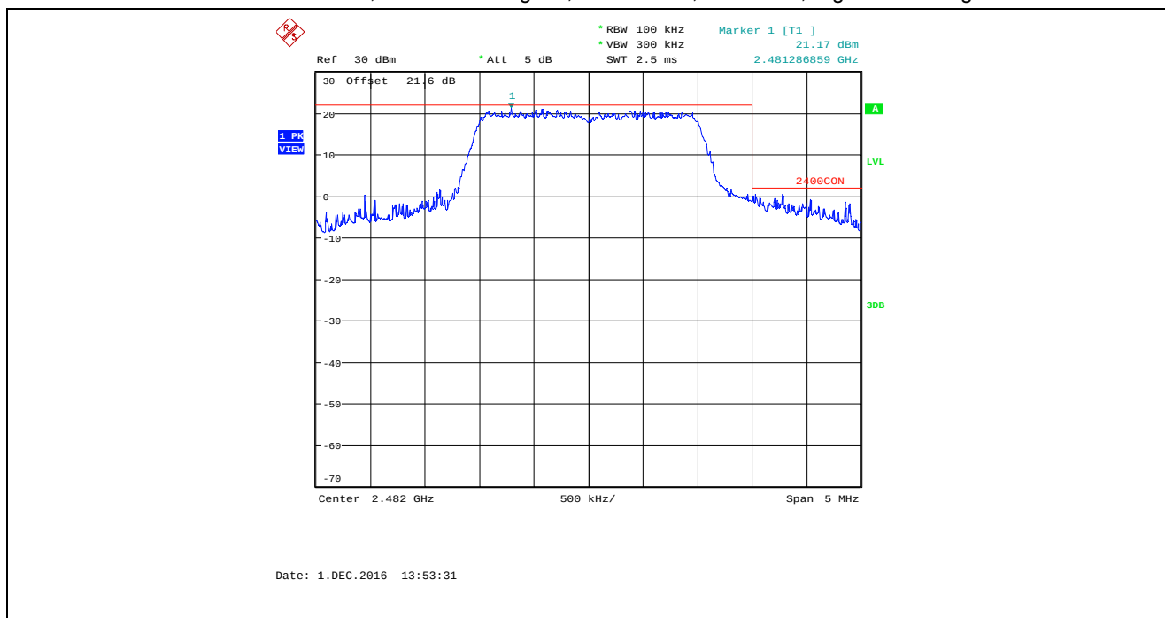
Plot 5.4.4.1.12. Band-Edge RF Conducted Emissions Bandwidth: 2 MHz, TX Gain Setting: 45, Data Rate 7, 2482 MHz, Higher Band-edge
