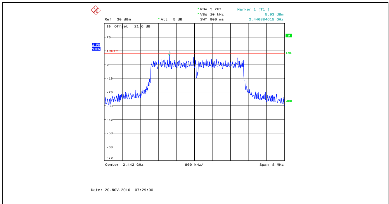
Plot 5.6.4.65. Power Spectral Density, Bandwidth: 4 MHz, TX Gain Setting: 50, Data Rate 6, 2442 MHz
