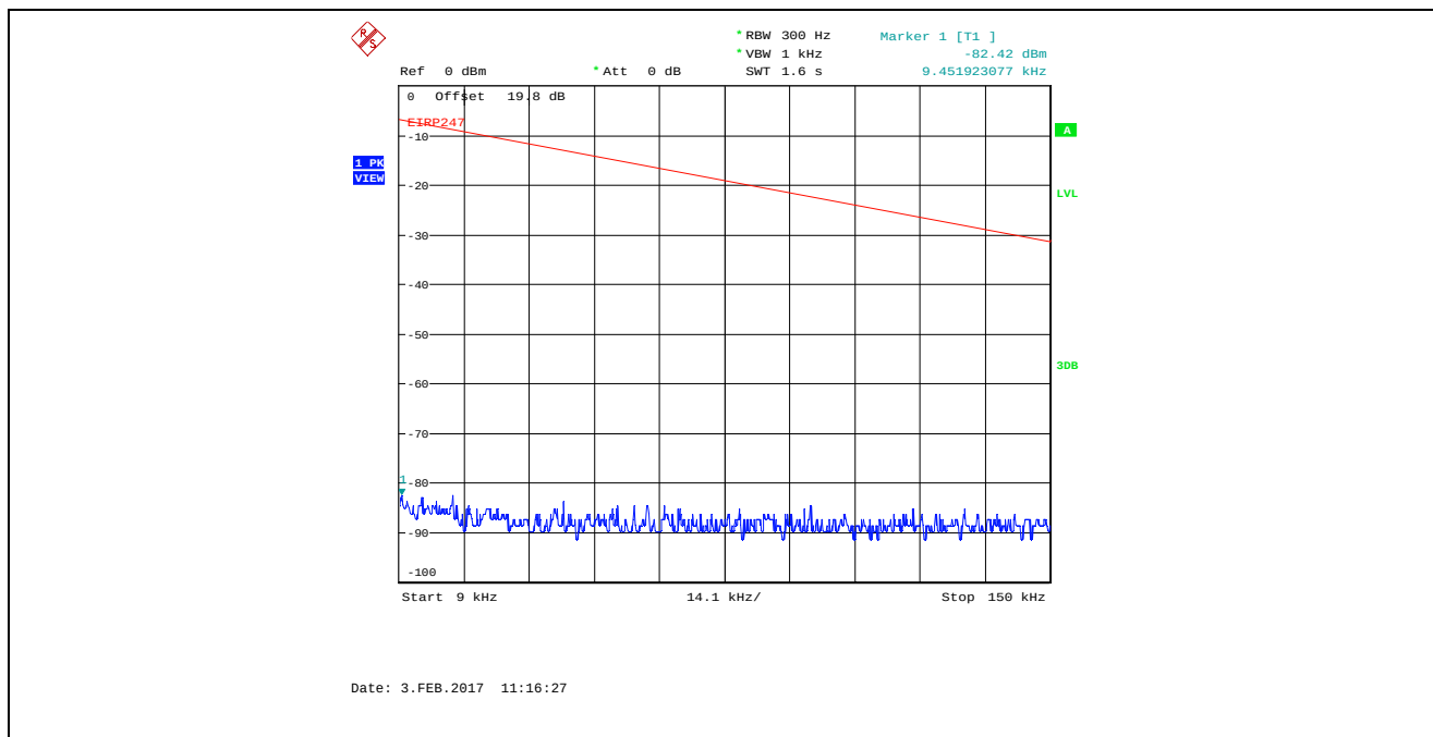
Plot 5.4.4.3.11. Conducted Spurious Emissions in Restricted Frequency Bands Bandwidth: 8 MHz, TX Gain Setting 50, Data Rate 1, 2477 MHz, 9 kHz - 150 kHz, Peak Detector
