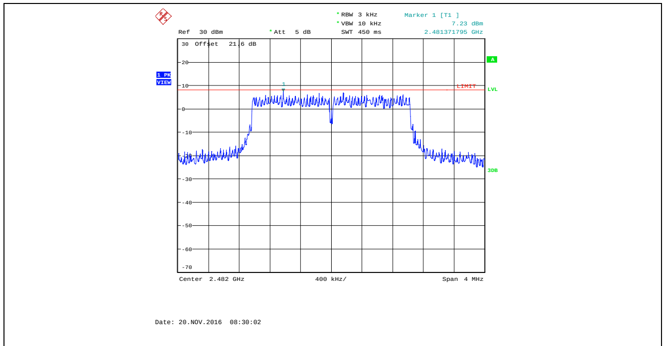
Plot 5.6.4.51. Power Spectral Density, Bandwidth: 2 MHz, TX Gain Setting: 45, Data Rate 5, 2482 MHz
