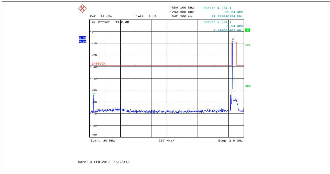
Plot 5.4.4.2.19. Conducted Spurious Emissions in Non-restricted Frequency Bands Bandwidth: 8 MHz, TX Gain: 0, Data Rate 4, 2407 MHz, 30 MHz – 2.6 GHz
