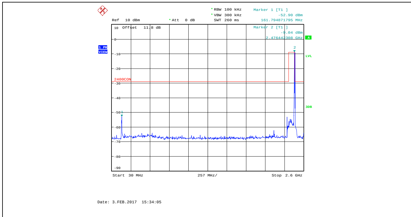
Plot 5.4.4.2.23. Conducted Spurious Emissions in Non-restricted Frequency Bands Bandwidth: 8 MHz, TX Gain: 0, Data Rate 4, 2477 MHz, 30 MHz – 2.6 GHz
