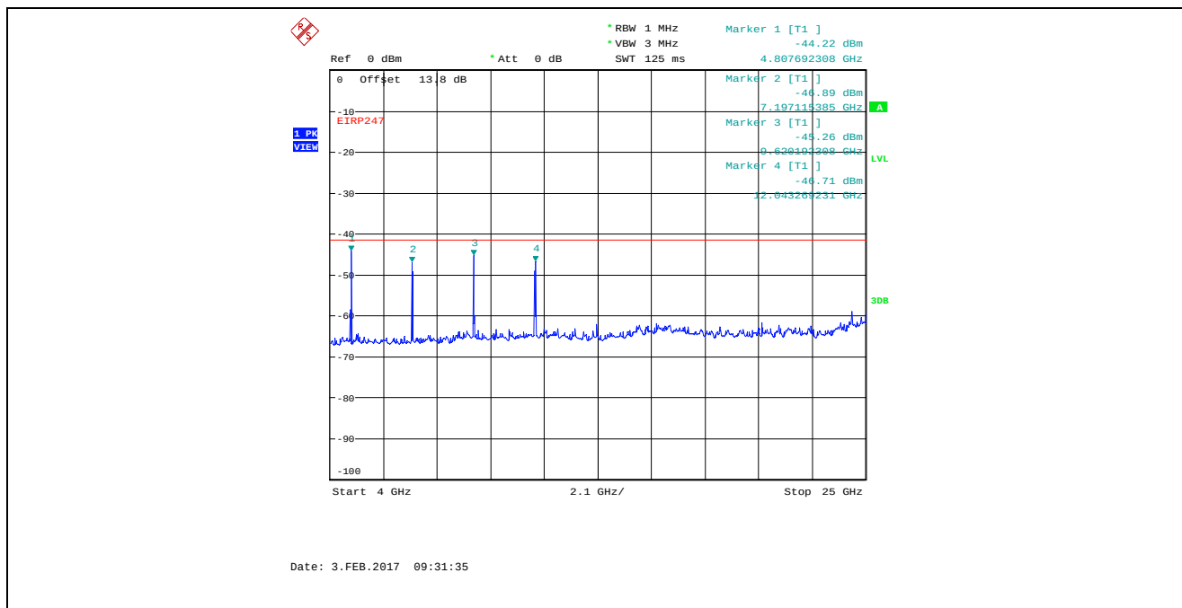
Plot 5.4.4.3.20. Conducted Spurious Emissions in Restricted Frequency Bands Bandwidth: 8 MHz, TX Gain Setting 55, Data Rate 4, 2407 MHz, 4 GHz - 25 GHz, Peak Detector
