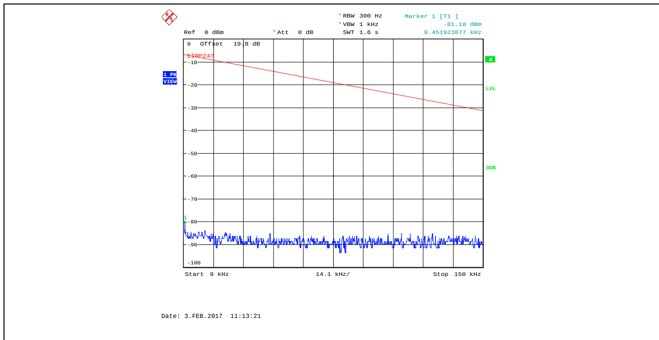
Plot 5.4.4.3.26. Conducted Spurious Emissions in Restricted Frequency Bands Bandwidth: 8 MHz, TX Gain Setting 55, Data Rate 4, 2477 MHz, 9 kHz - 150 kHz, Peak Detector
