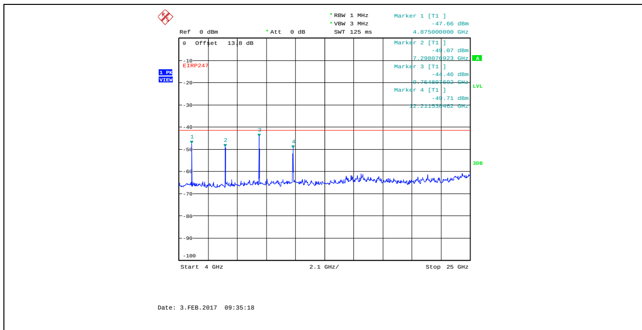
Plot 5.4.4.3.25. Conducted Spurious Emissions in Restricted Frequency Bands Bandwidth: 8 MHz, TX Gain Setting 55, Data Rate 4, 2442 MHz, 4 GHz - 25 GHz, Peak Detector
