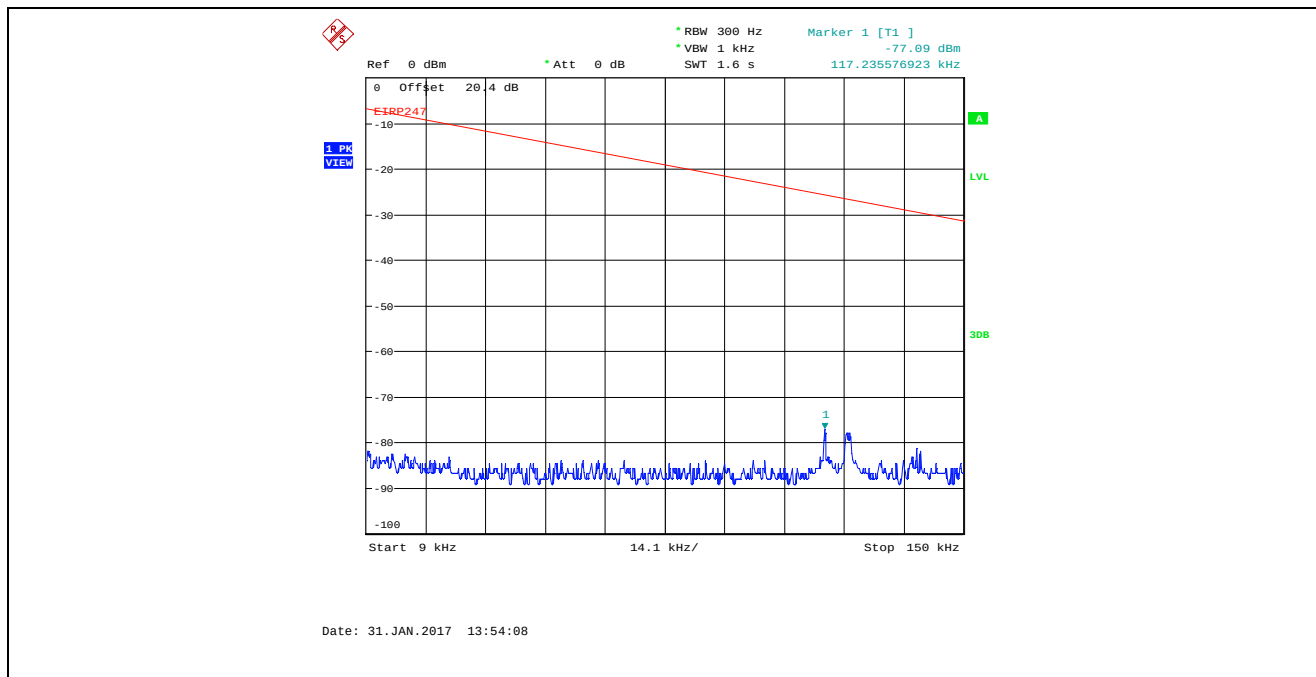
Plot 5.4.4.4.16. Conducted Spurious Emissions in Restricted Frequency Bands Bandwidth: 8 MHz, TX Gain Setting 25, Data Rate 4, 2407 MHz, 9 kHz - 150 kHz, Peak Detector
