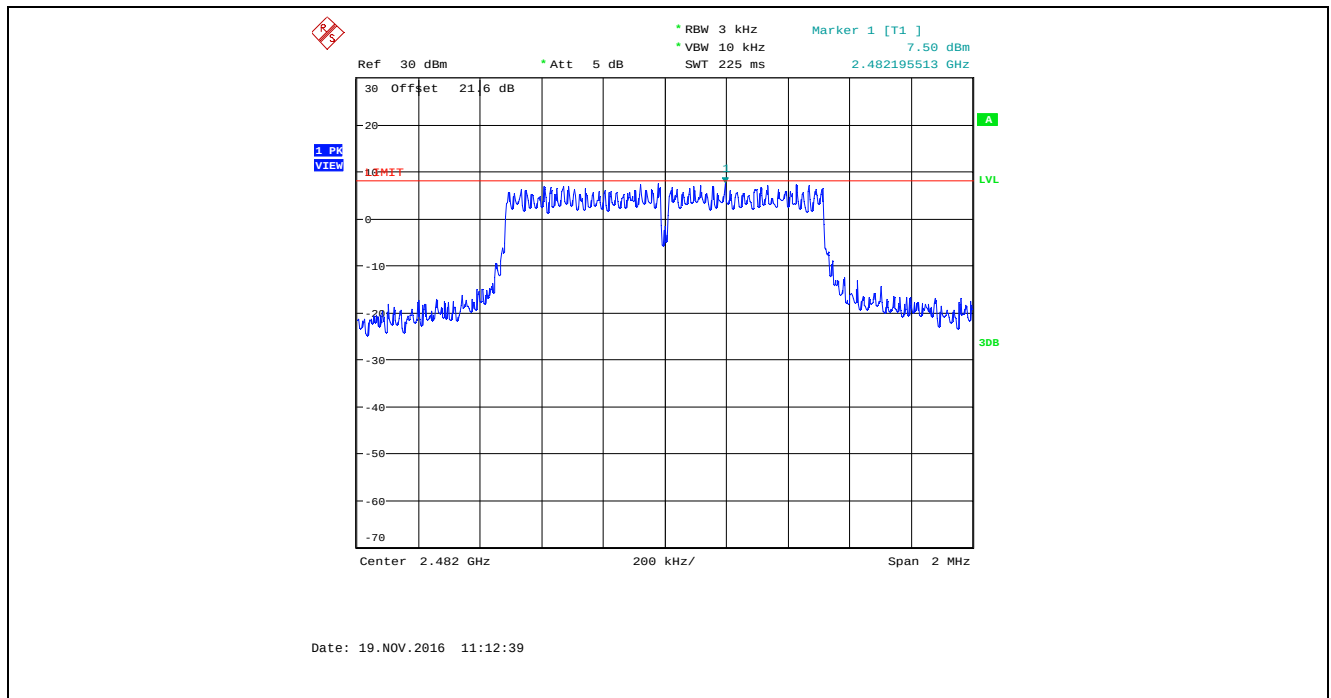
Plot 5.6.4.42. Power Spectral Density, Bandwidth: 1 MHz, TX Gain Setting: 43, Data Rate 6, 2482 MHz
