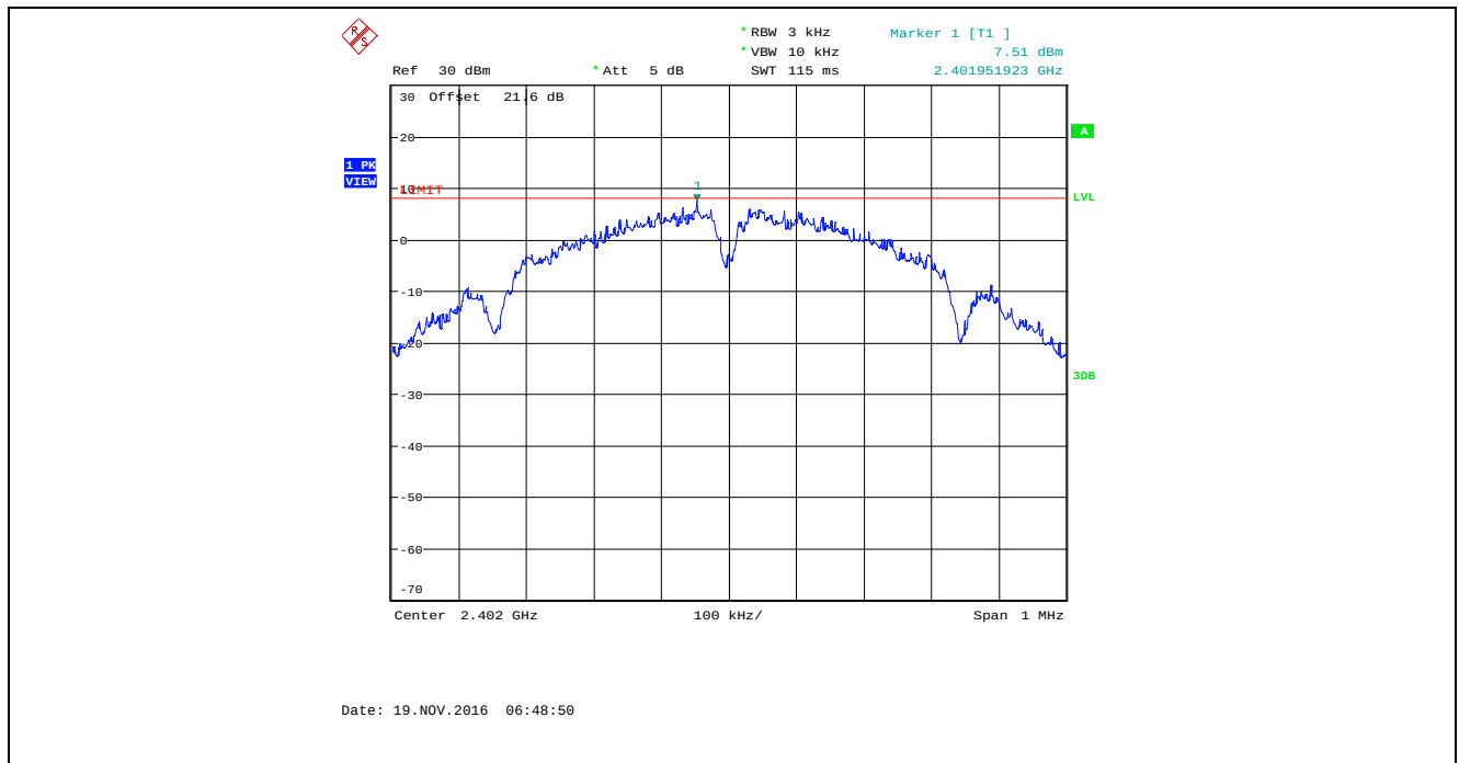
Plot 5.6.4.4. Power Spectral Density, Bandwidth: 1 MHz, TX Gain Setting: 26, Data Rate 2, 2402 MHz
