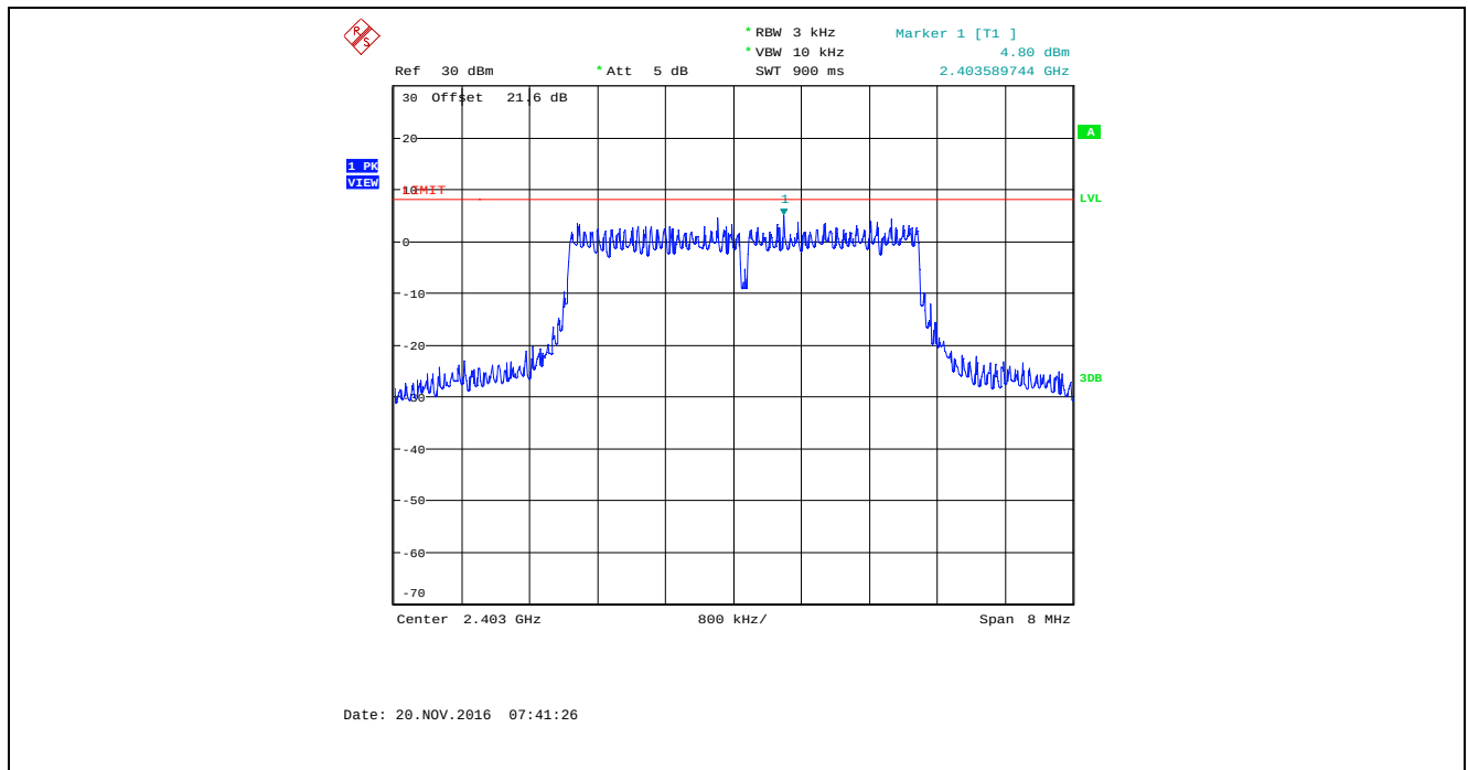
Plot 5.6.4.58. Power Spectral Density, Bandwidth: 4 MHz, TX Gain Setting: 50, Data Rate 4, 2403 MHz
