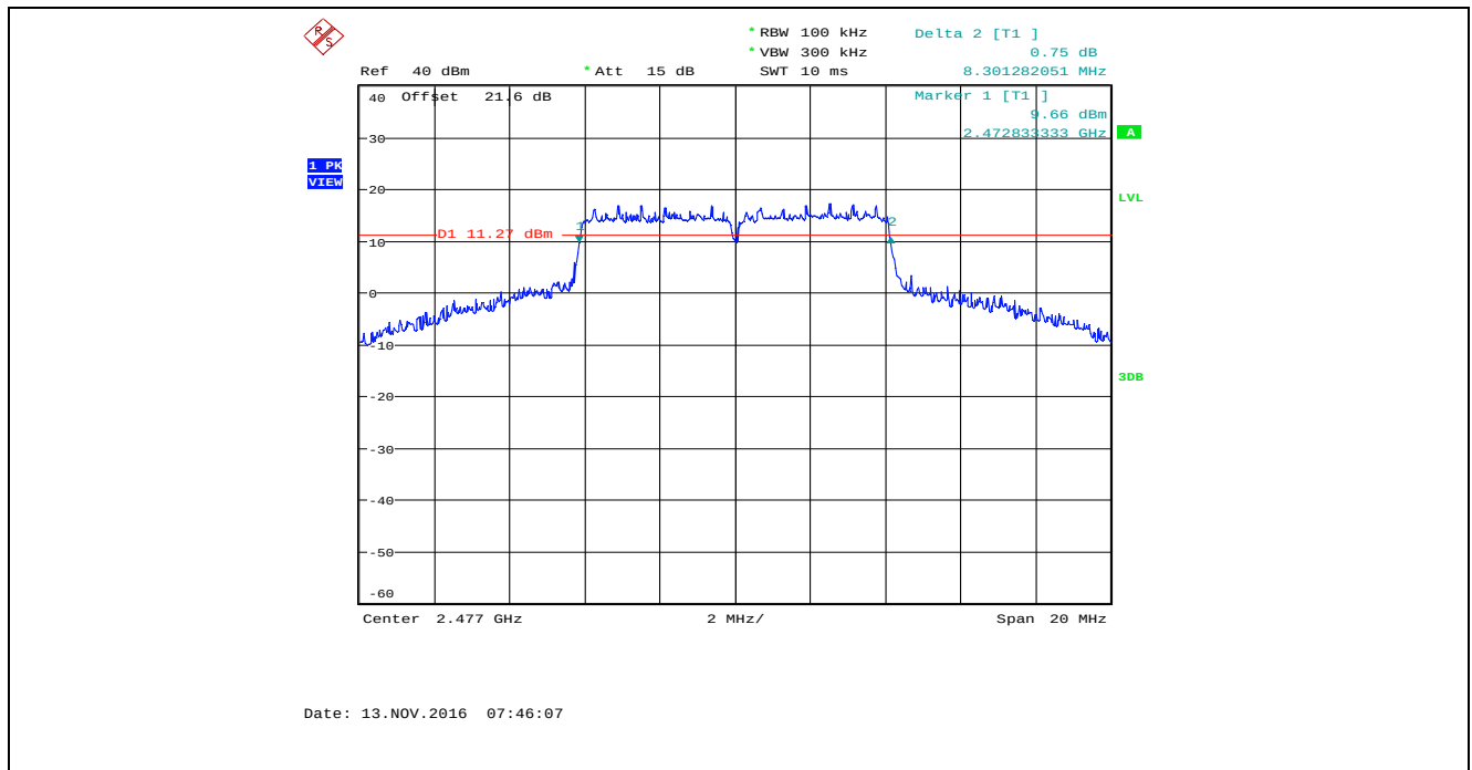
Plot 5.2.4.72. 6 dB Bandwidth, Bandwidth: 8 MHz, TX Gain: 55, Data Rate 4, 2477 MHz
