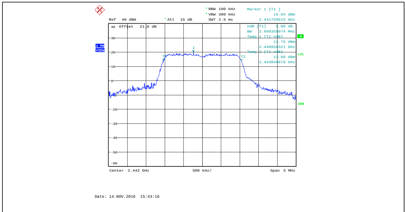
Plot 5.2.4.50. 6 dB Bandwidth, Bandwidth: 2 MHz, TX Gain: 45, Data Rate 5, 2442 MHz
