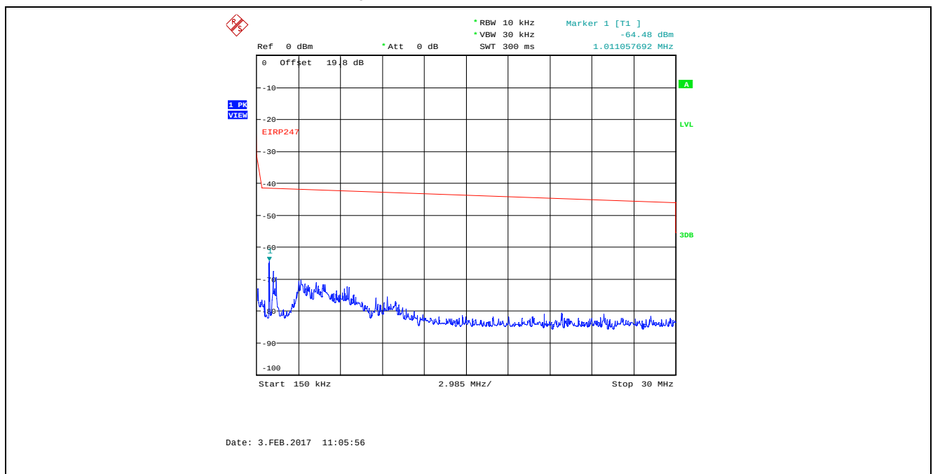
Plot 5.4.4.3.22. Conducted Spurious Emissions in Restricted Frequency Bands Bandwidth: 8 MHz, TX Gain Setting 55, Data Rate 4, 2442 MHz, 150 kHz - 30 MHz, Peak Detector
