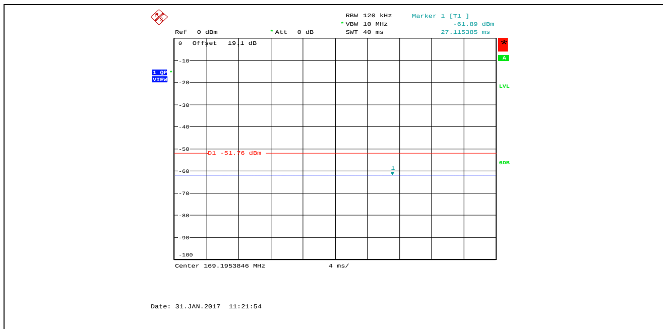
Plot 5.4.4.4.27. Conducted Spurious Emissions in Restricted Frequency Bands Bandwidth: 8 MHz, TX Gain Setting 25, Data Rate 4, 2442 MHz, RB 167.72-173.2 MHz, QP Detector QP at 169.19 MHz (RB 167.72-173.2 MHz) is -61.89dBm (limit -51.76dBm)
