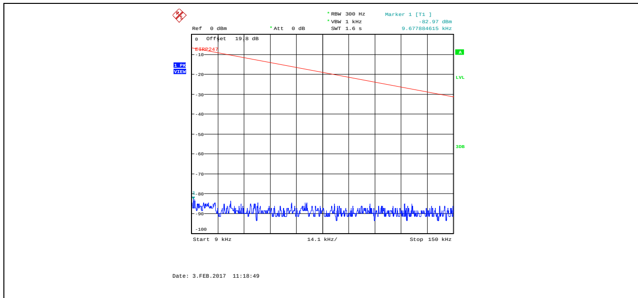
Plot 5.4.4.3.1. Conducted Spurious Emissions in Restricted Frequency Bands Bandwidth: 8 MHz, TX Gain Setting 50, Data Rate 1, 2407 MHz, 9 kHz - 150 kHz, Peak Detector
