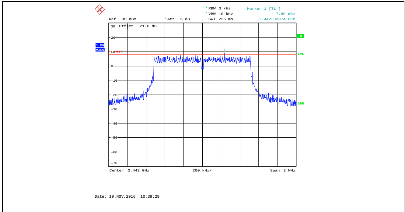
Plot 5.6.4.35. Power Spectral Density, Bandwidth: 1 MHz, TX Gain Setting: 43, Data Rate 4, 2442 MHz
