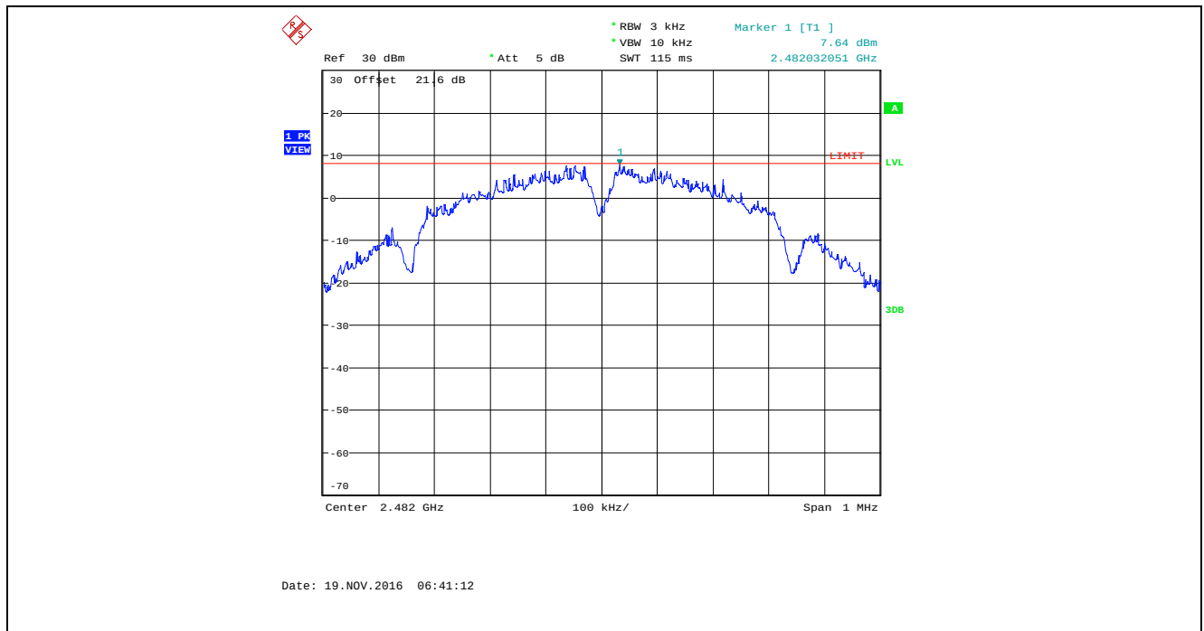
Plot 5.6.4.3. Power Spectral Density, Bandwidth: 1 MHz, TX Gain Setting: 26, Data Rate 1, 2482 MHz
