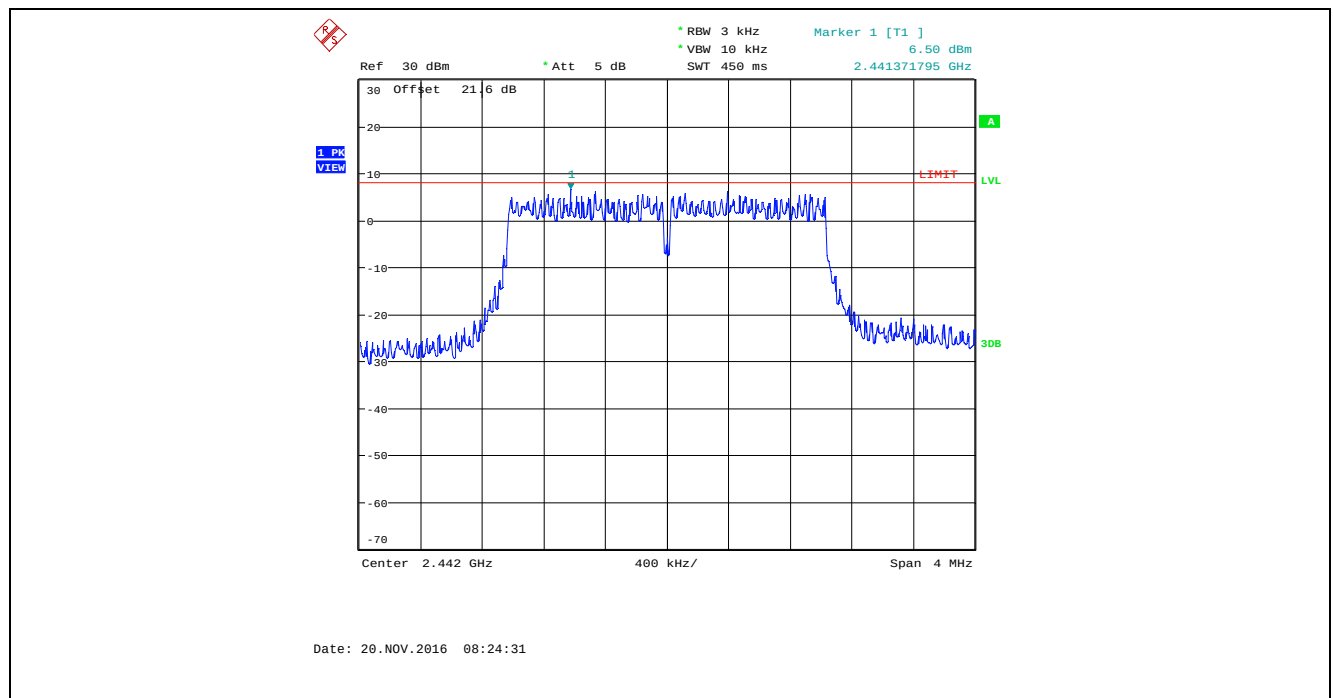
Plot 5.6.4.53. Power Spectral Density, Bandwidth: 2 MHz, TX Gain Setting: 45, Data Rate 6, 2442 MHz
