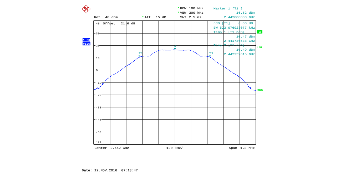
Plot 5.2.4.5. 6 dB Bandwidth, Bandwidth: 1 MHz, TX Gain: 26, Data Rate 2, 2442 MHz
