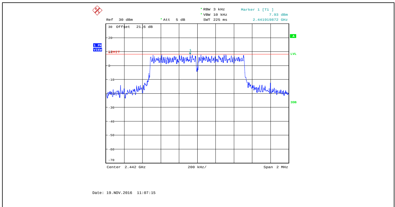
Plot 5.6.4.41. Power Spectral Density, Bandwidth: 1 MHz, TX Gain Setting: 43, Data Rate 6, 2442 MHz
