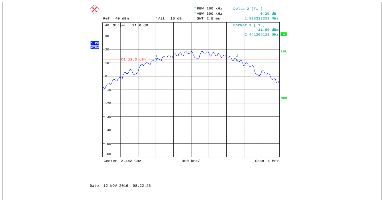
Plot 5.2.4.17. 6 dB Bandwidth, Bandwidth: 4 MHz, TX Gain: 43, Data Rate 1, 2442 MHz
