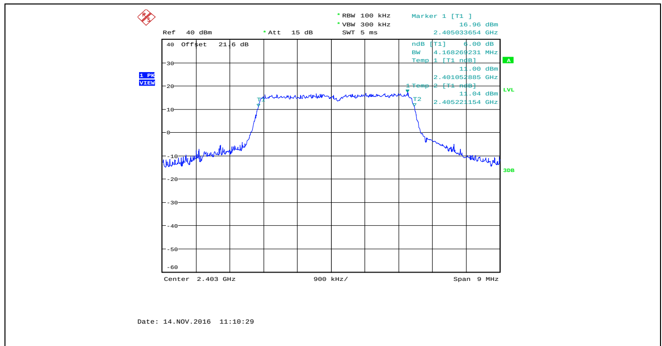
Plot 5.2.4.61. 6 dB Bandwidth, Bandwidth: 4 MHz, TX Gain: 50, Data Rate 5, 2403 MHz
