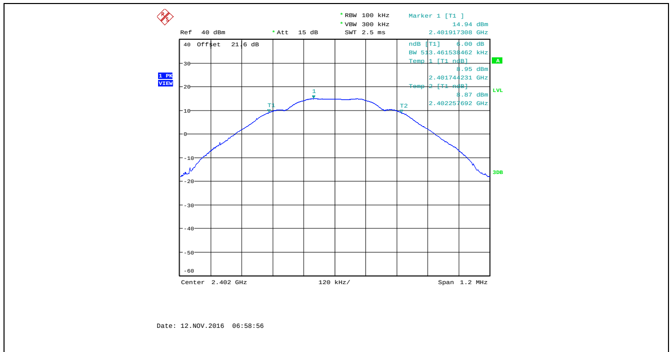
Plot 5.2.4.1. 6 dB Bandwidth, Bandwidth: 1 MHz, TX Gain: 26, Data Rate 1, 2402 MHz
