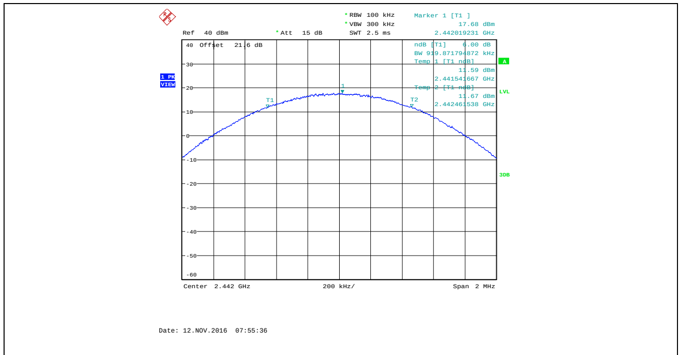
Plot 5.2.4.14. 6 dB Bandwidth, Bandwidth: 2 MHz, TX Gain: 32, Data Rate 3, 2442 MHz
