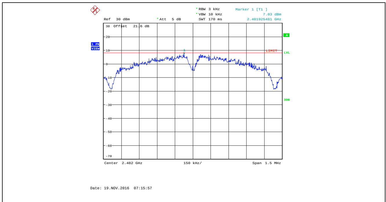
Plot 5.6.4.12. Power Spectral Density, Bandwidth: 2 MHz, TX Gain Setting: 32, Data Rate 2, 2482 MHz
