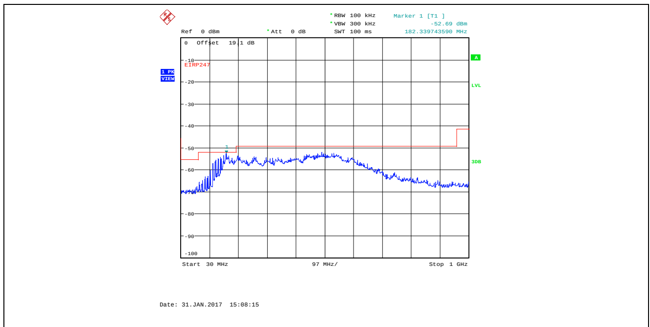
Plot 5.4.4.4.13. Conducted Spurious Emissions in Restricted Frequency Bands Bandwidth: 8 MHz, TX Gain Setting 25, Data Rate 1, 2477 MHz, 30 MHz - 1 GHz, Peak Detector
