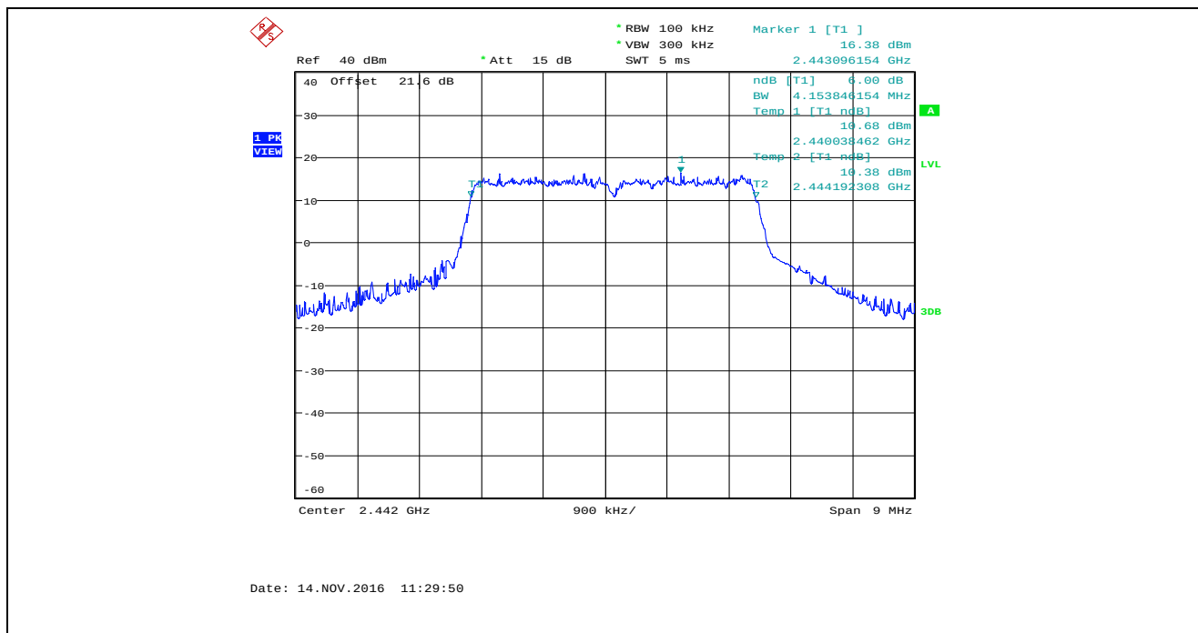
Plot 5.2.4.68. 6 dB Bandwidth, Bandwidth: 4 MHz, TX Gain: 50, Data Rate 7, 2442 MHz
