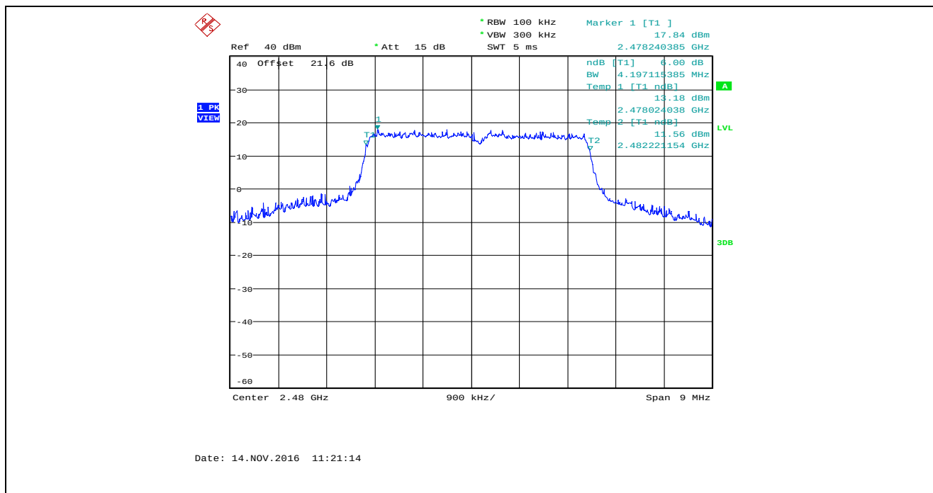
Plot 5.2.4.66. 6 dB Bandwidth, Bandwidth: 4 MHz, TX Gain: 50, Data Rate 6, 2480 MHz
