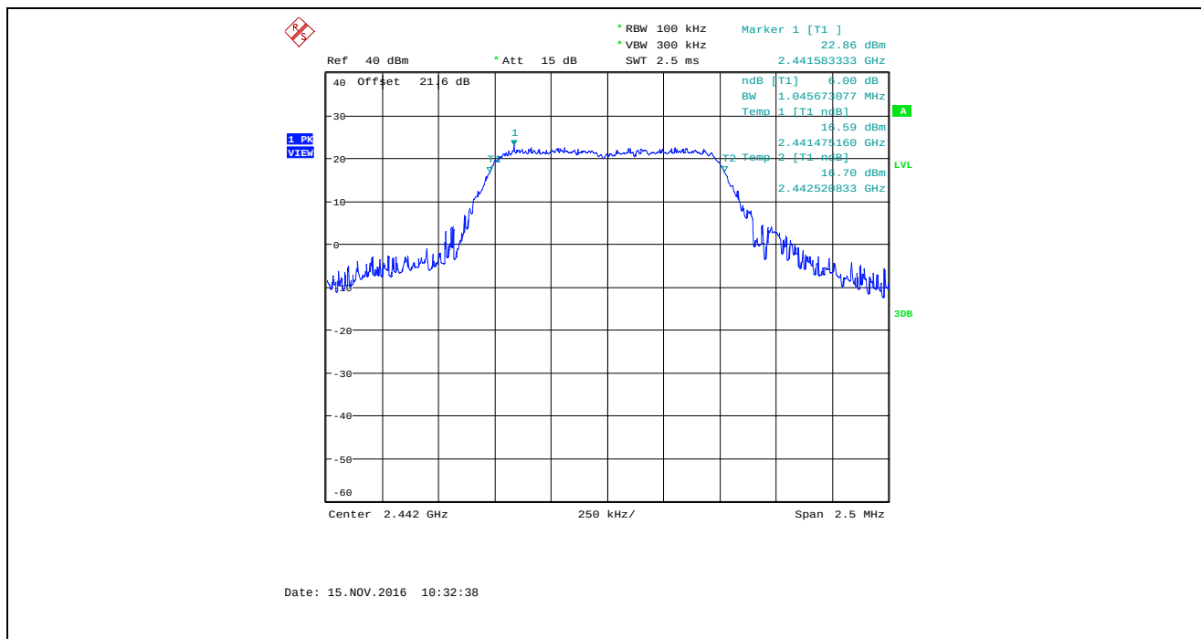
Plot 5.2.4.38. 6 dB Bandwidth, Bandwidth: 1 MHz, TX Gain: 43, Data Rate 5, 2442 MHz
