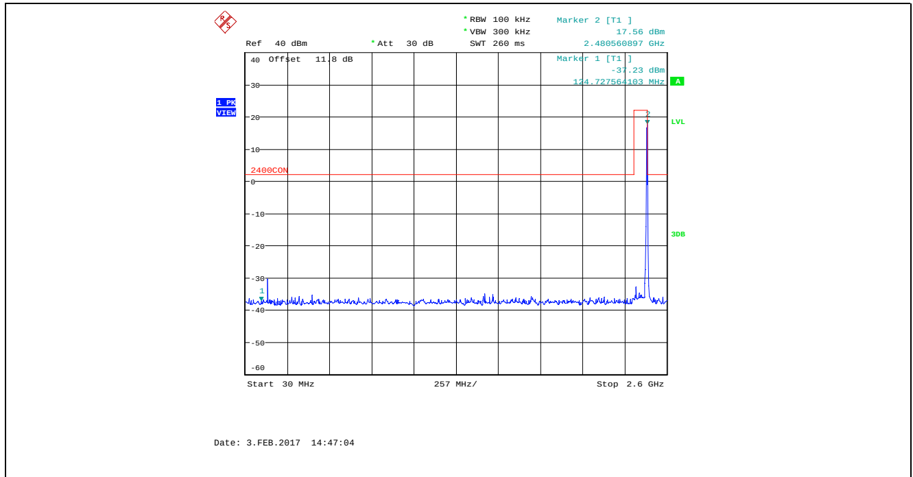
Plot 5.4.4.2.5. Conducted Spurious Emissions in Non-restricted Frequency Bands Bandwidth: 8 MHz, TX Gain: 50, Data Rate 1, 2477 MHz, 30 MHz – 2.6 GHz
