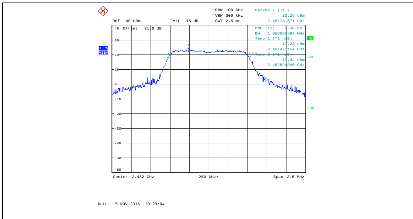
Plot 5.2.4.39. 6 dB Bandwidth, Bandwidth: 1 MHz, TX Gain: 43, Data Rate 5, 2482 MHz
