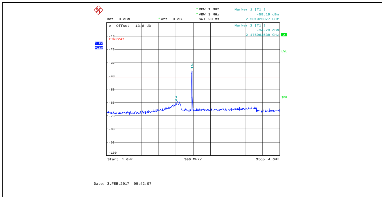
Plot 5.4.4.3.29. Conducted Spurious Emissions in Restricted Frequency Bands Bandwidth: 8 MHz, TX Gain Setting 55, Data Rate 4, 2477 MHz, 1 GHz - 4 GHz, Peak Detector Marker 2 is the Fundamental
