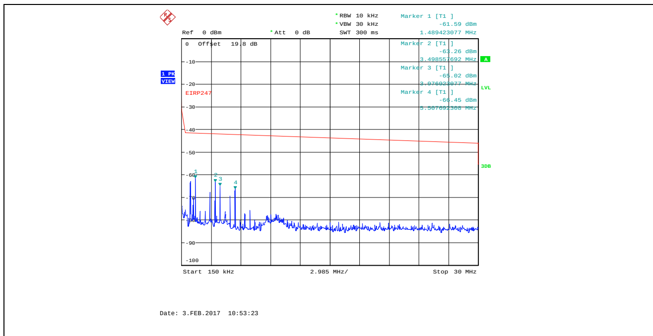
Plot 5.4.4.3.7. Conducted Spurious Emissions in Restricted Frequency Bands Bandwidth: 8 MHz, TX Gain Setting 50, Data Rate 1, 2442 MHz, 150 kHz - 30 MHz, Peak Detector
