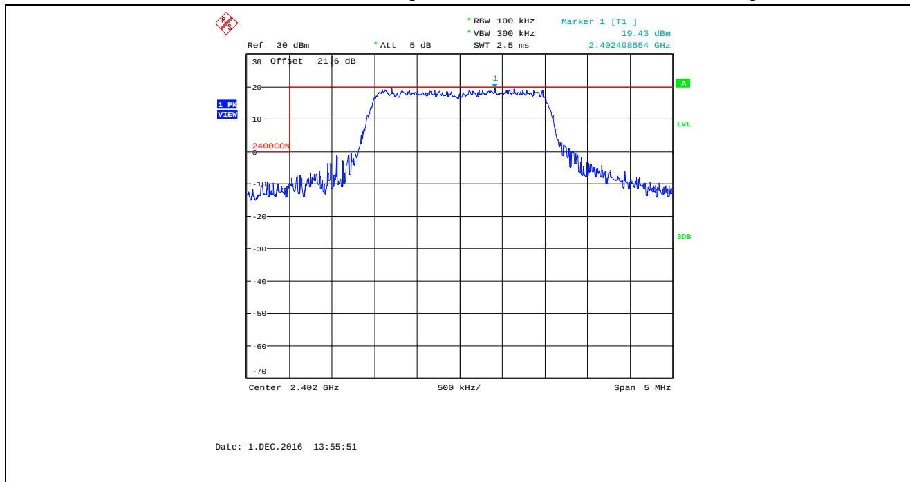
Plot 5.4.4.1.11. Band-Edge RF Conducted Emissions Bandwidth: 2 MHz, TX Gain Setting: 45, Data Rate 7, 2402 MHz, Lower Band-edge
