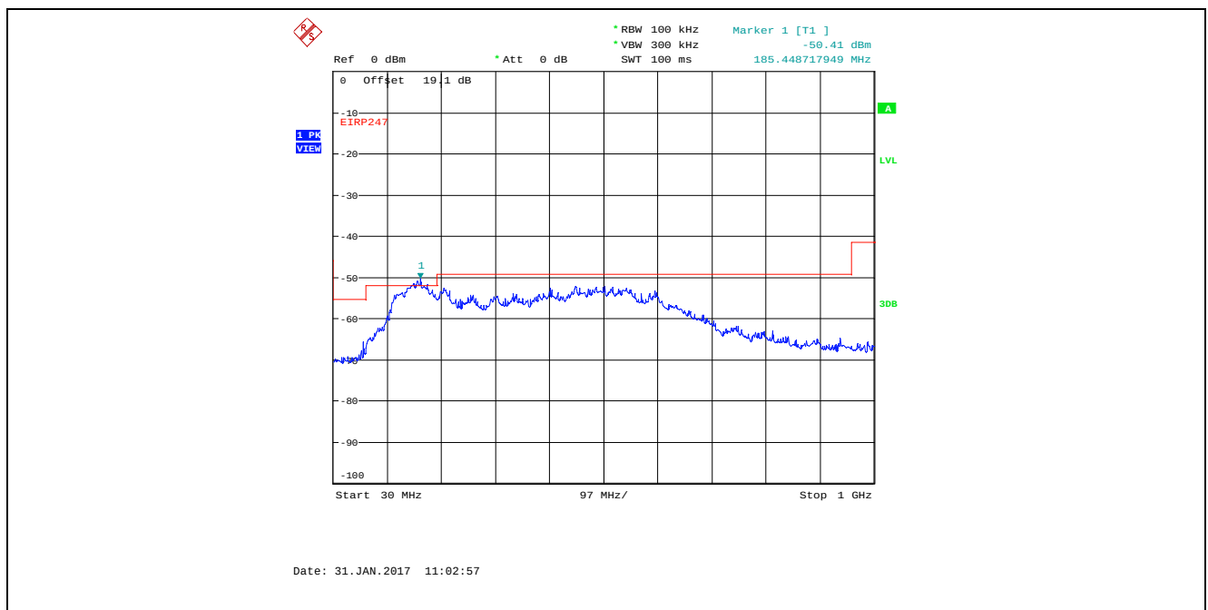
Plot 5.4.4.18. Conducted Spurious Emissions in Restricted Frequency Bands Bandwidth: 8 MHz, TX Gain Setting 25, Data Rate 4, 2407 MHz, 30 MHz - 1 GHz, Peak Detector
