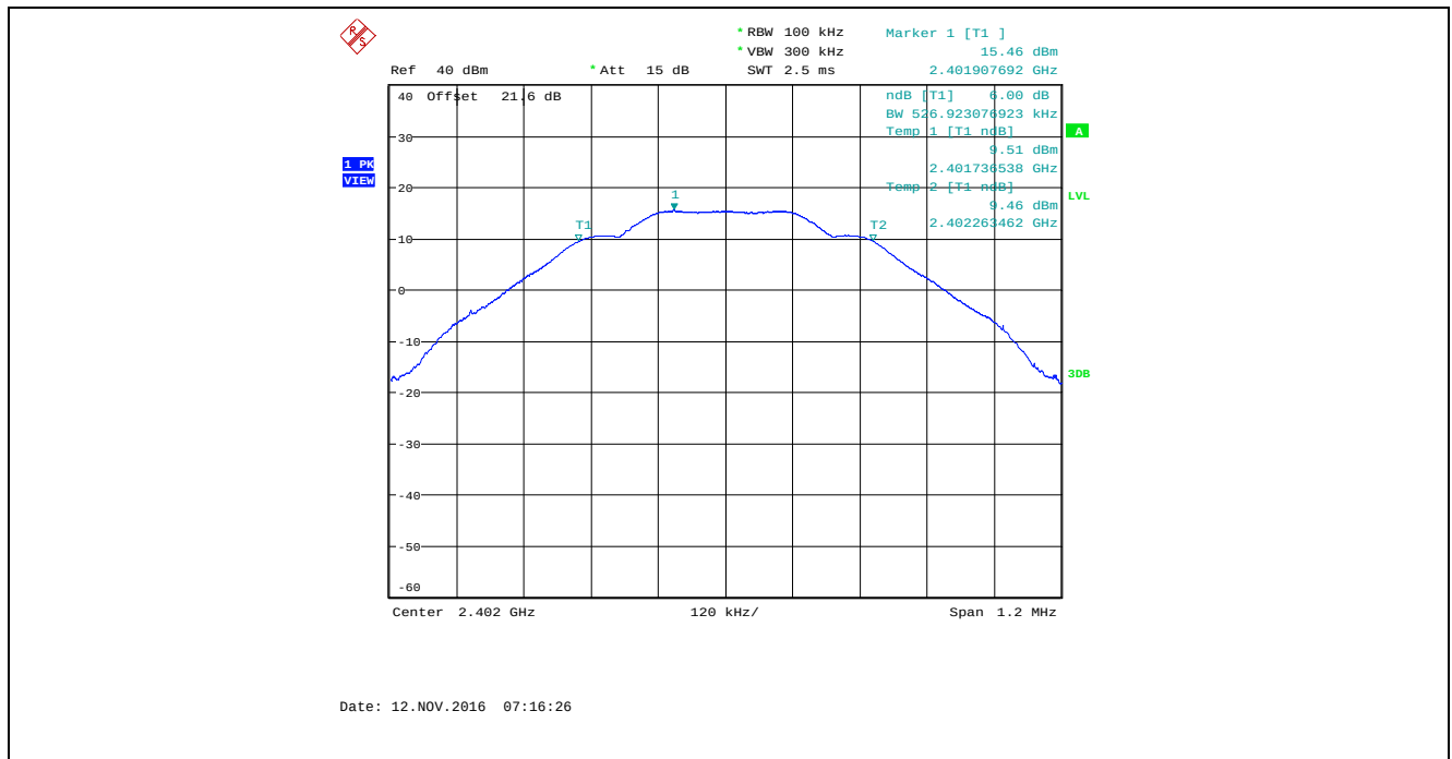
Plot 5.2.4.4. 6 dB Bandwidth, Bandwidth: 1 MHz, TX Gain: 26, Data Rate 2, 2402 MHz
