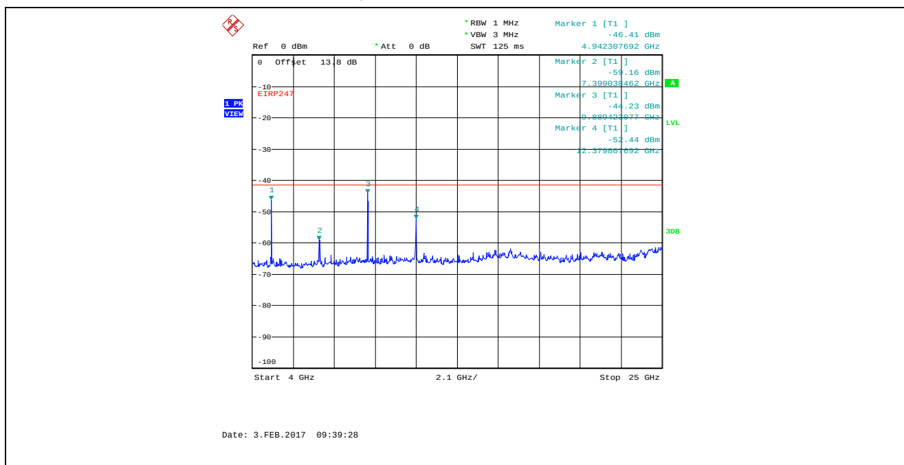
Plot 5.4.4.3.30. Conducted Spurious Emissions in Restricted Frequency Bands Bandwidth: 8 MHz, TX Gain Setting 55, Data Rate 4, 2477 MHz, 4 GHz - 25 GHz, Peak Detector
