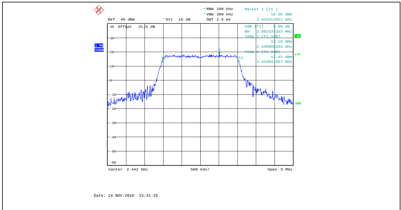
Plot 5.2.4.53. 6 dB Bandwidth, Bandwidth: 2 MHz, TX Gain: 45, Data Rate 6, 2442 MHz
