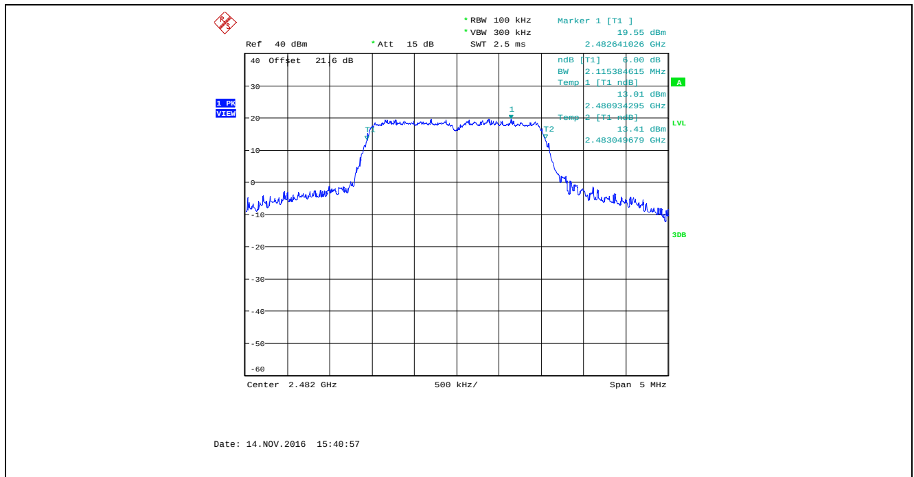
Plot 5.2.4.51. 6 dB Bandwidth, Bandwidth: 2 MHz, TX Gain: 45, Data Rate 5, 2482 MHz
