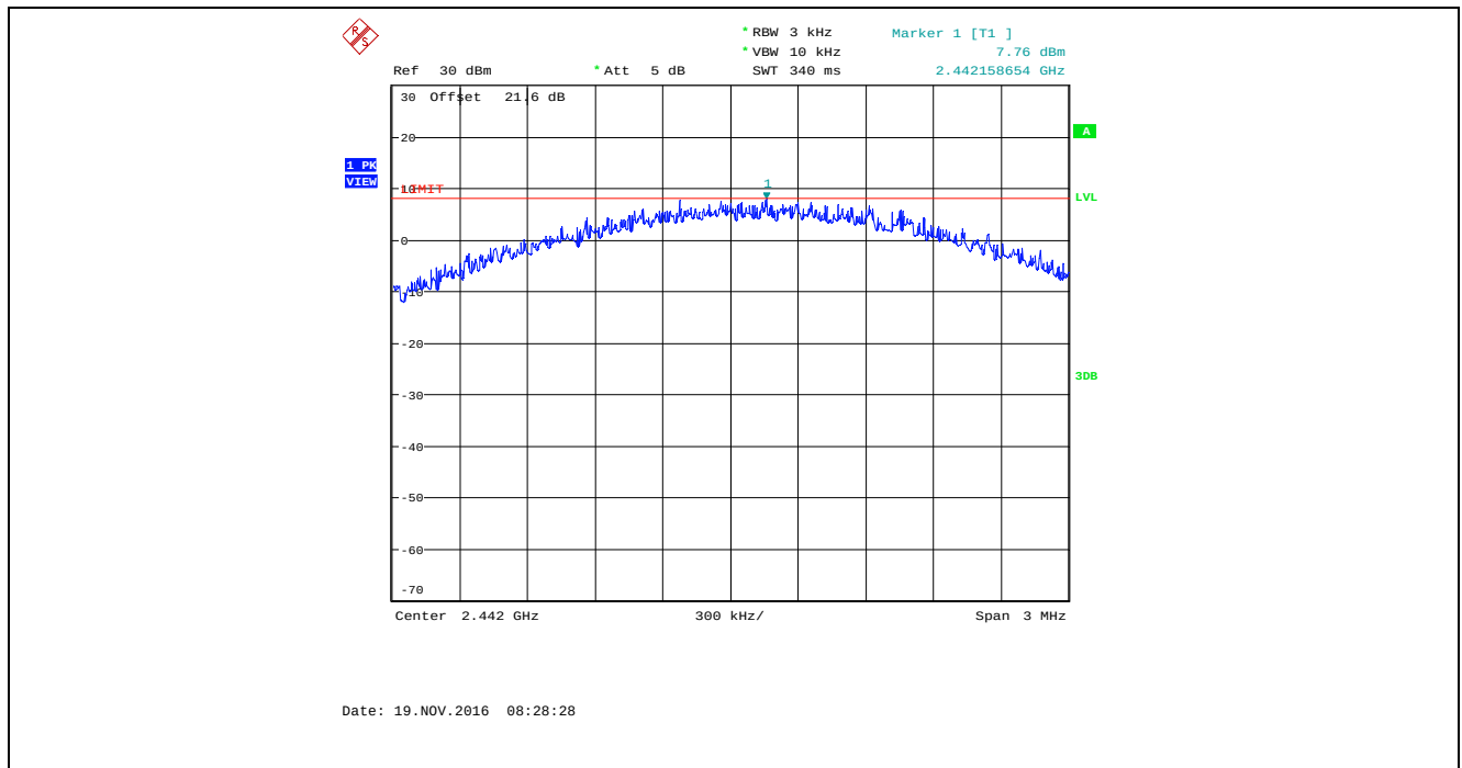
Plot 5.6.4.23. Power Spectral Density, Bandwidth: 4 MHz, TX Gain Setting: 43, Data Rate 3, 2442 MHz
