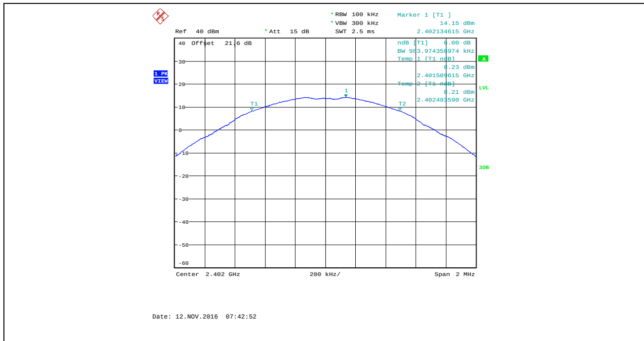
Plot 5.2.4.10. 6 dB Bandwidth, Bandwidth: 2 MHz, TX Gain: 32, Data Rate 2, 2402 MHz
