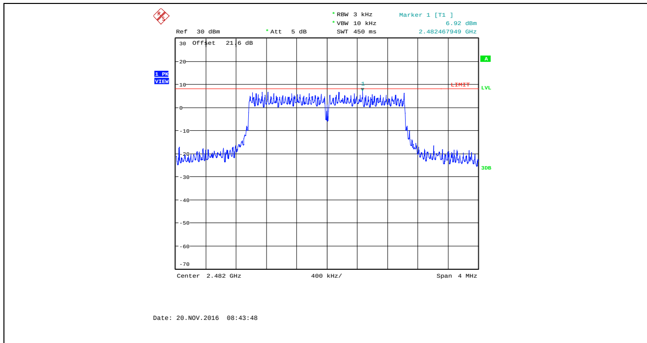
Plot 5.6.4.48. Power Spectral Density, Bandwidth: 2 MHz, TX Gain Setting: 45, Data Rate 4, 2482 MHz
