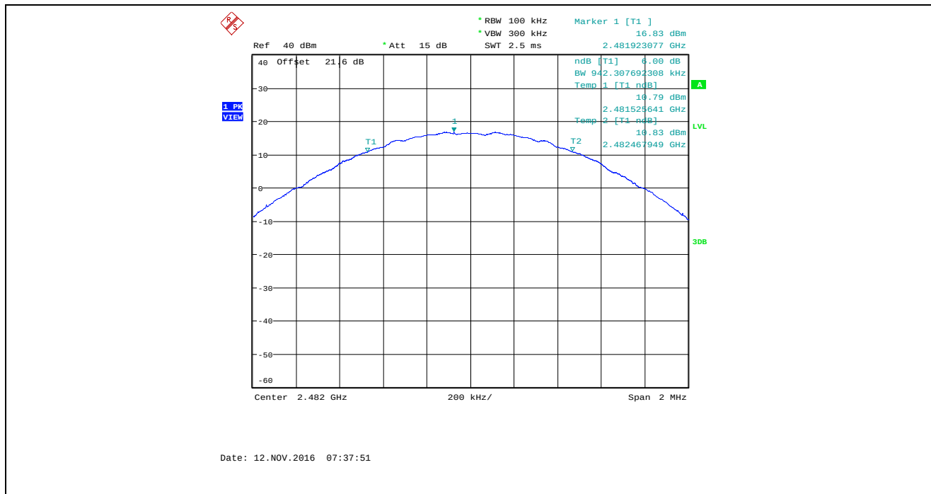
Plot 5.2.4.9. 6 dB Bandwidth, Bandwidth: 2 MHz, TX Gain: 32, Data Rate 1, 2482 MHz
