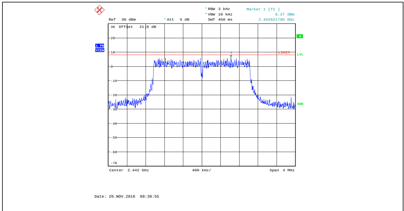
Plot 5.6.4.47. Power Spectral Density, Bandwidth: 2 MHz, TX Gain Setting: 45, Data Rate 4, 2442 MHz
