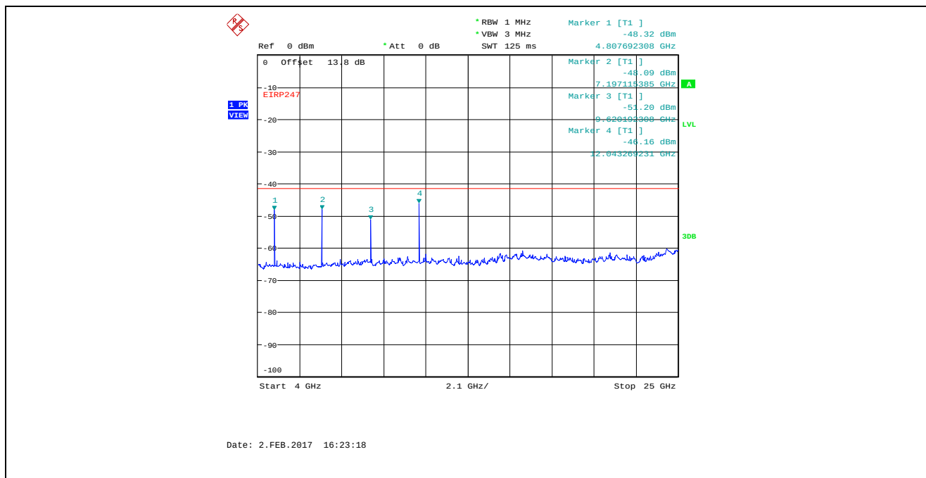
Plot 5.4.4.3.5. Conducted Spurious Emissions in Restricted Frequency Bands Bandwidth: 8 MHz, TX Gain Setting 50, Data Rate 1, 2407 MHz, 4 GHz - 25 GHz, Peak Detector
