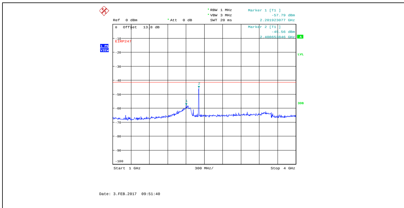
Plot 5.4.4.3.19. Conducted Spurious Emissions in Restricted Frequency Bands Bandwidth: 8 MHz, TX Gain Setting 55, Data Rate 4, 2407 MHz, 1 GHz - 4 GHz, Peak Detector
