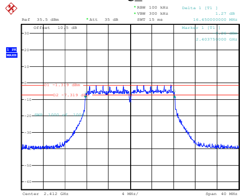
802.11g_2412MHz
