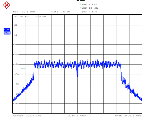
802.11g_2412MHz
