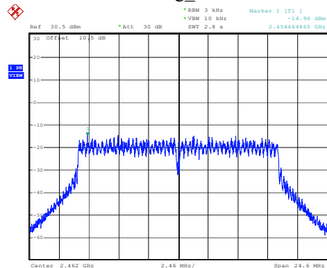
802.11g_2462MHz
