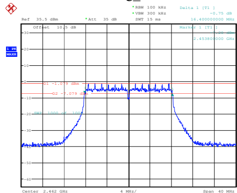
802.11g_2462MHz
