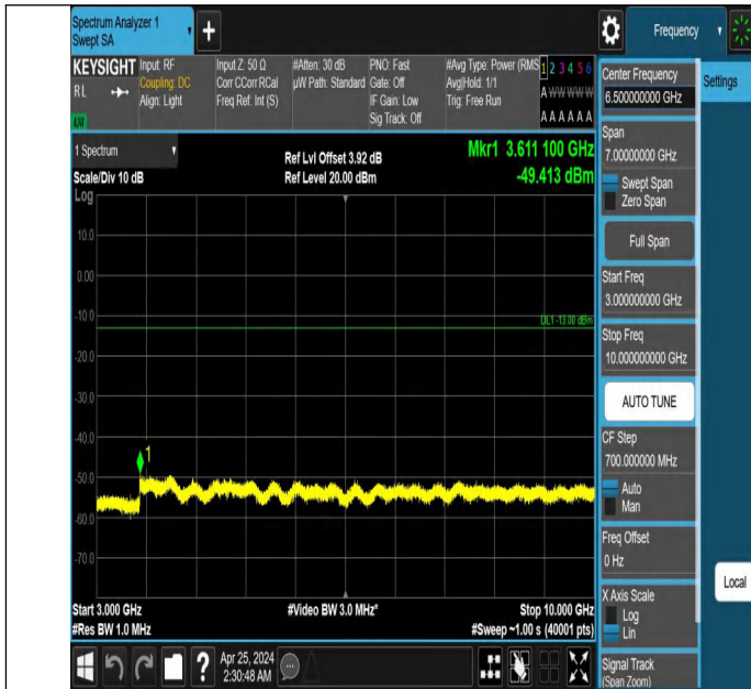
Band5_5MHz_QPSK_20425_1RB#0_3000~10000_3000~10000
