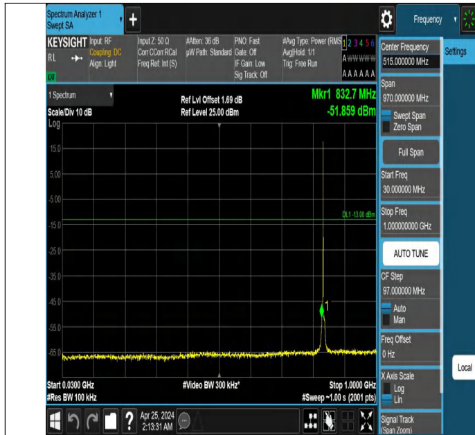
Band5_1.4MHz_QPSK_20525_1RB#0_30~1000_30~1000
