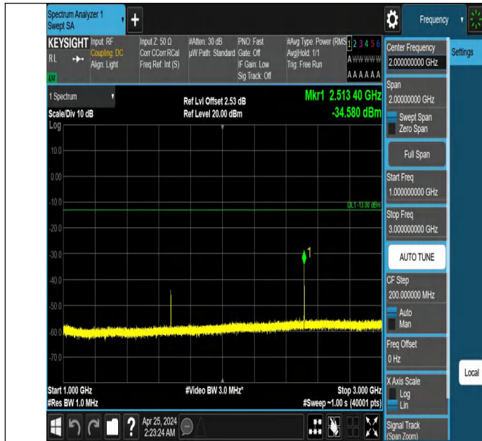
Band5_3MHz_QPSK_20525_1RB#14_1000~3000_1000~3000
