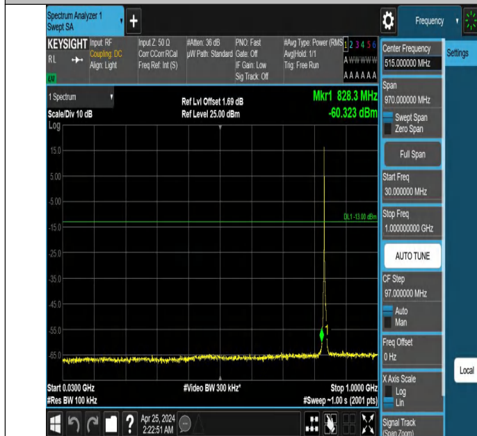
Band5_3MHz_QPSK_20525_1RB#0_30~1000_30~1000
