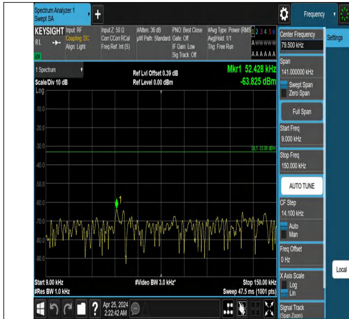
Band5_3MHz_QPSK_20525_1RB#0_0.009~0.15_0.009~0.15
