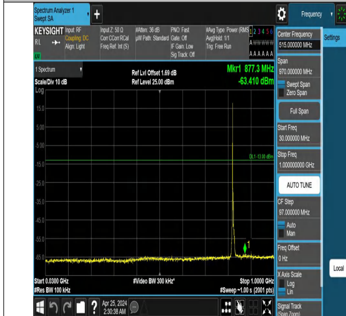
Band5_5MHz_QPSK_20425_1RB#0_30~1000_30~1000
