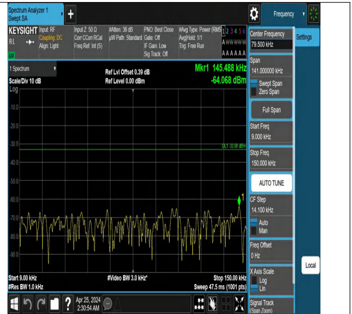
Band5_5MHz_QPSK_20425_1RB#24_0.009~0.15_0.009~0.15
