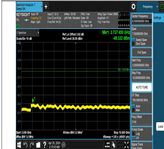
Band5_1.4MHz_QPSK_20525_1RB#0_3000~10000_3000~10000
