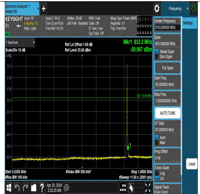
Band5_3MHz_QPSK_20415_1RB#14_30~1000_30~1000
