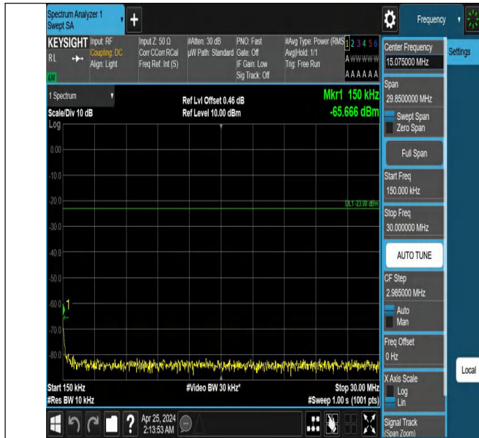
Band5_1.4MHz_QPSK_20525_1RB#5_0.15~30_0.15~30
