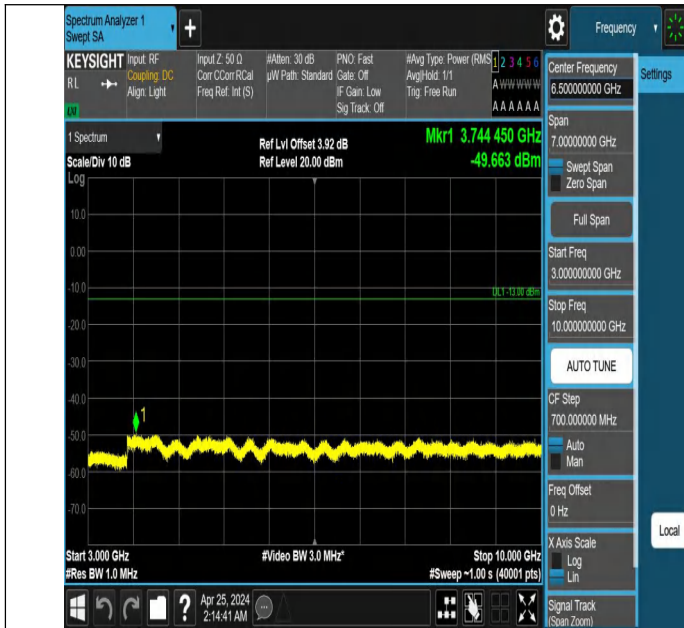
Band5_1.4MHz_QPSK_20643_1RB#0_3000~10000_3000~10000
