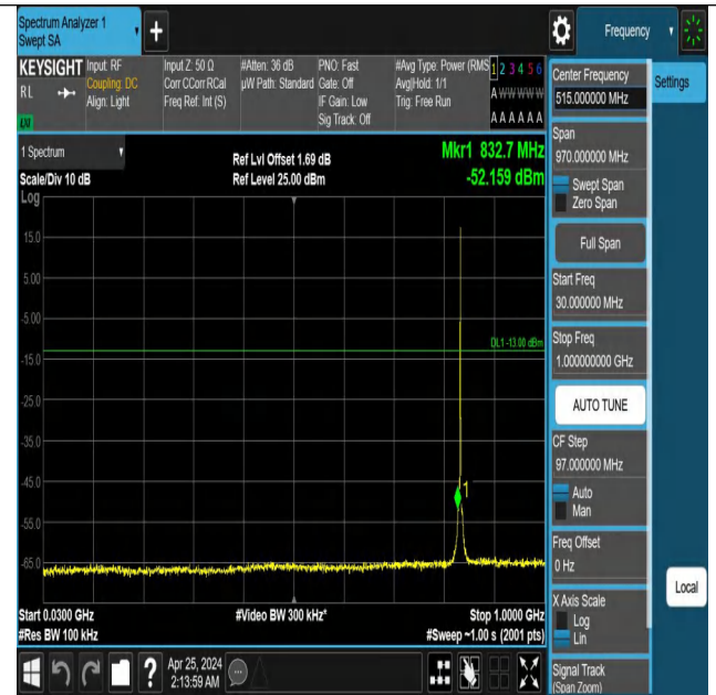
Band5_1.4MHz_QPSK_20525_1RB#5_30~1000_30~1000
