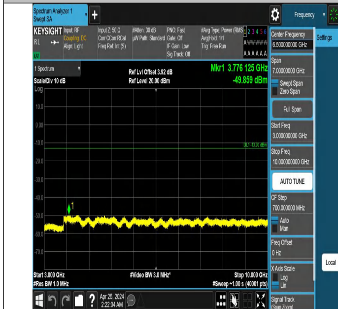
Band5_3MHz_QPSK_20415_1RB#0_3000~10000_3000~10000
