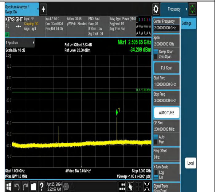
Band5_3MHz_QPSK_20525_1RB#0_1000~3000_1000~3000
