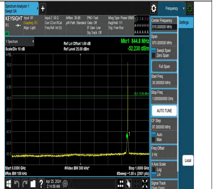
Band5_1.4MHz_QPSK_20643_1RB#5_30~1000_30~1000
