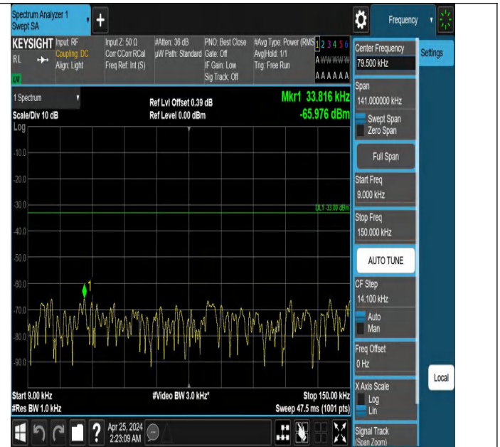
Band5_3MHz_QPSK_20525_1RB#14_0.009~0.15_0.009~0.15
