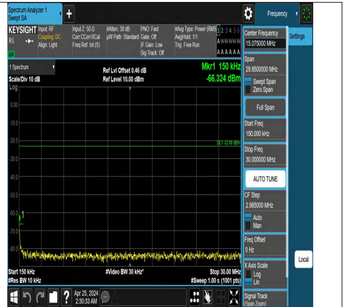
Band5_5MHz_QPSK_20425_1RB#0_0.15~30_0.15~30
