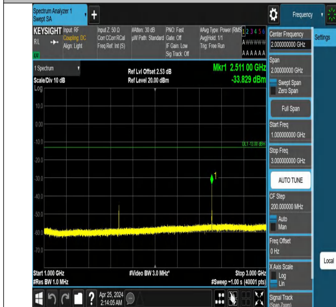
Band5_1.4MHz_QPSK_20525_1RB#5_1000~3000_1000~3000
