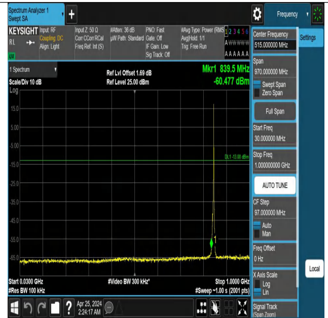
Band5_3MHz_QPSK_20635_1RB#14_30~1000_30~1000
