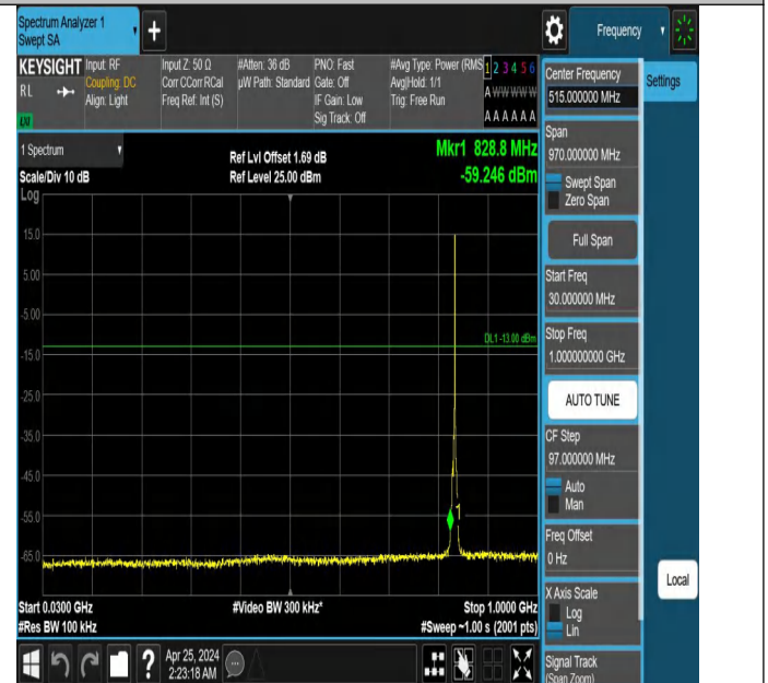
Band5_3MHz_QPSK_20525_1RB#14_30~1000_30~1000
