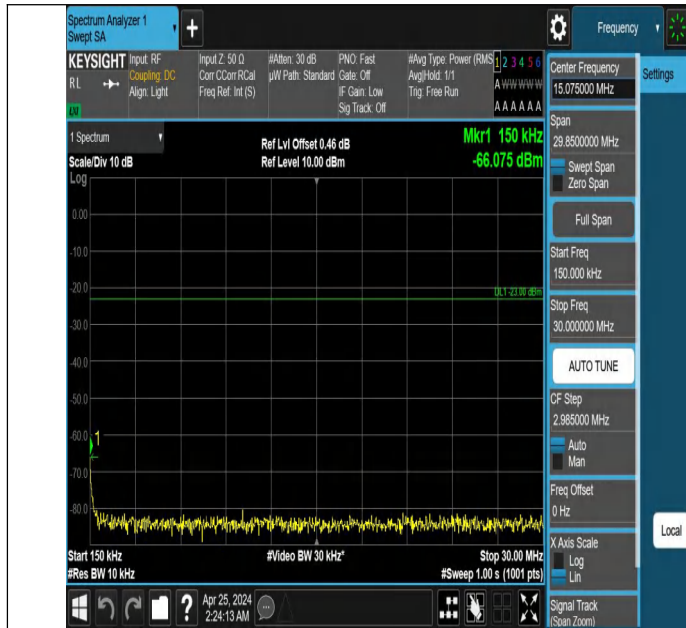
Band5_3MHz_QPSK_20635_1RB#14_0.15~30_0.15~30
