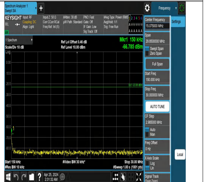
Band5_5MHz_QPSK_20525_1RB#0_0.15~30_0.15~30
