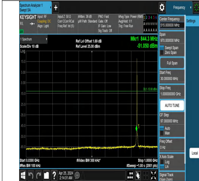
Band5_1.4MHz_QPSK_20643_1RB#0_30~1000_30~1000
