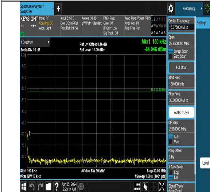
Band5_3MHz_QPSK_20525_1RB#14_0.15~30_0.15~30
