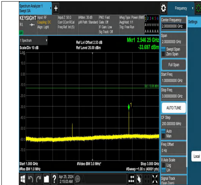
Band5_1.4MHz_QPSK_20643_1RB#5_1000~3000_1000~3000
