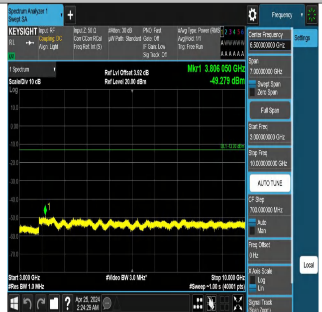
Band5_3MHz_QPSK_20635_1RB#14_3000~10000_3000~10000
