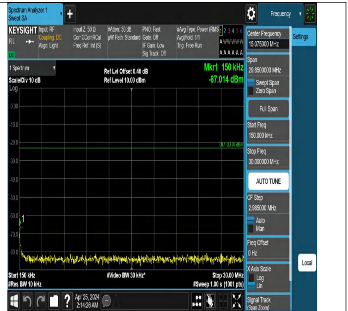
Band5_1.4MHz_QPSK_20643_1RB#0_0.15~30_0.15~30
