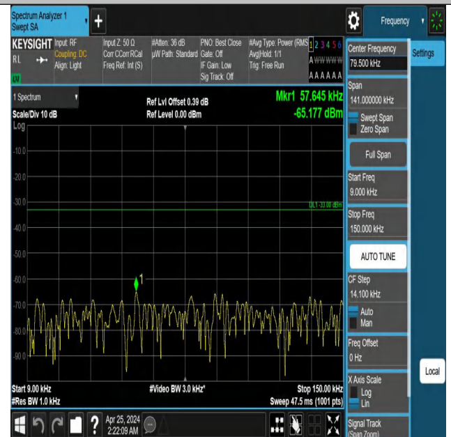
Band5_3MHz_QPSK_20415_1RB#14_0.009~0.15_0.009~0.15
