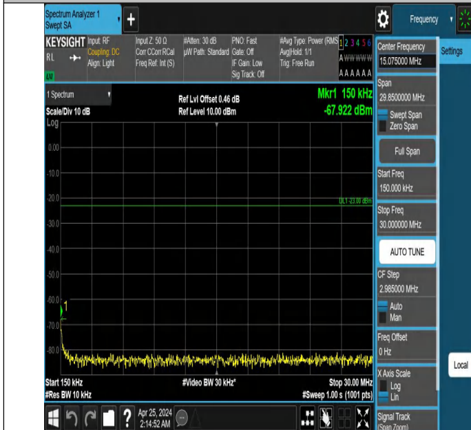
Band5_1.4MHz_QPSK_20643_1RB#5_0.15~30_0.15~30
