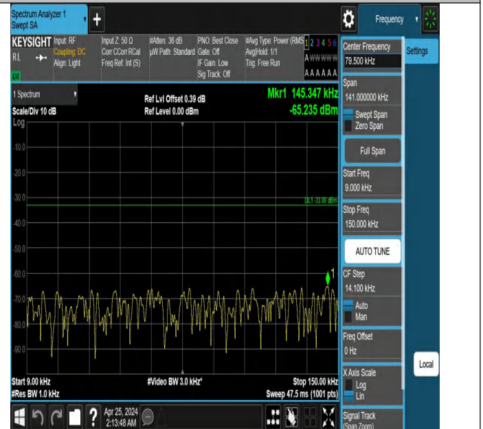
Band5_1.4MHz_QPSK_20525_1RB#5_0.009~0.15_0.009~0.15
