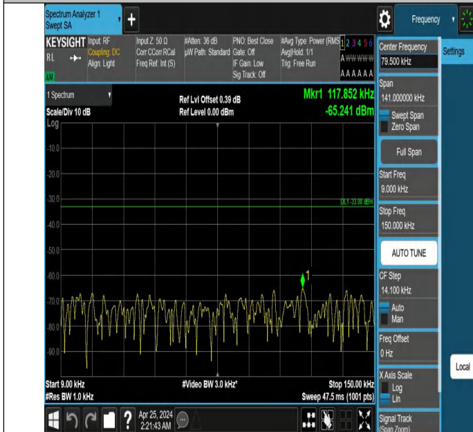
Band5_3MHz_QPSK_20415_1RB#0_0.009~0.15_0.009~0.15
