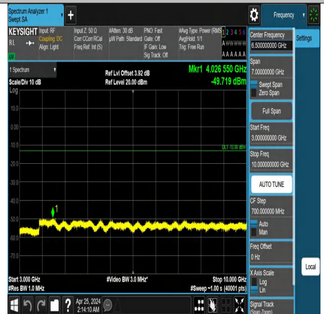
Band5_1.4MHz_QPSK_20525_1RB#5_3000~10000_3000~10000
