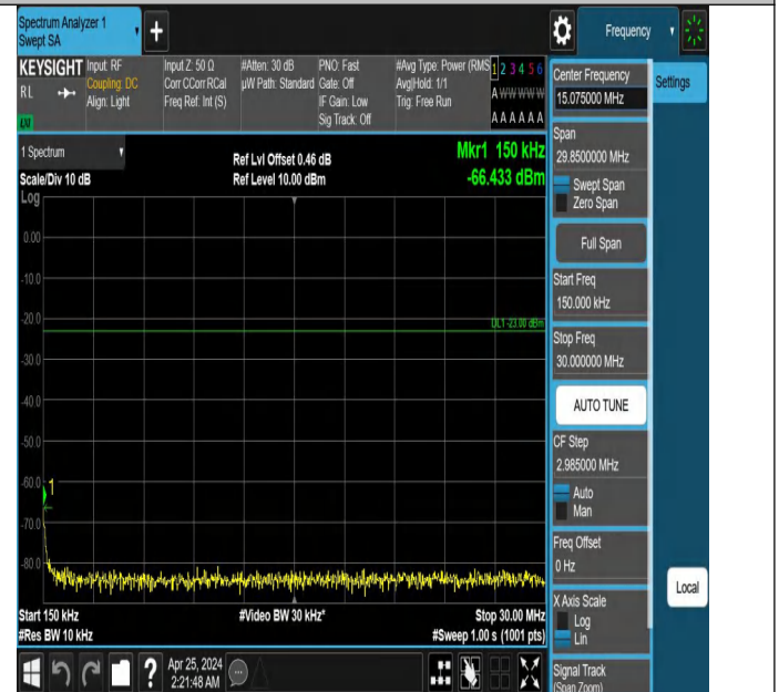
Band5_3MHz_QPSK_20415_1RB#0_0.15~30_0.15~30
