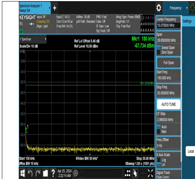
Band5_3MHz_QPSK_20415_1RB#14_0.15~30_0.15~30
