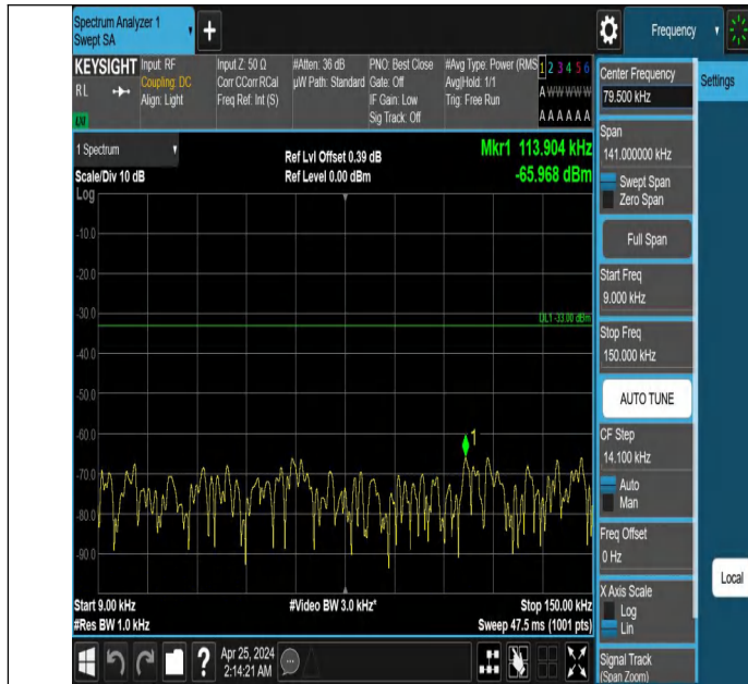
Band5_1.4MHz_QPSK_20643_1RB#0_0.009~0.15_0.009~0.15
