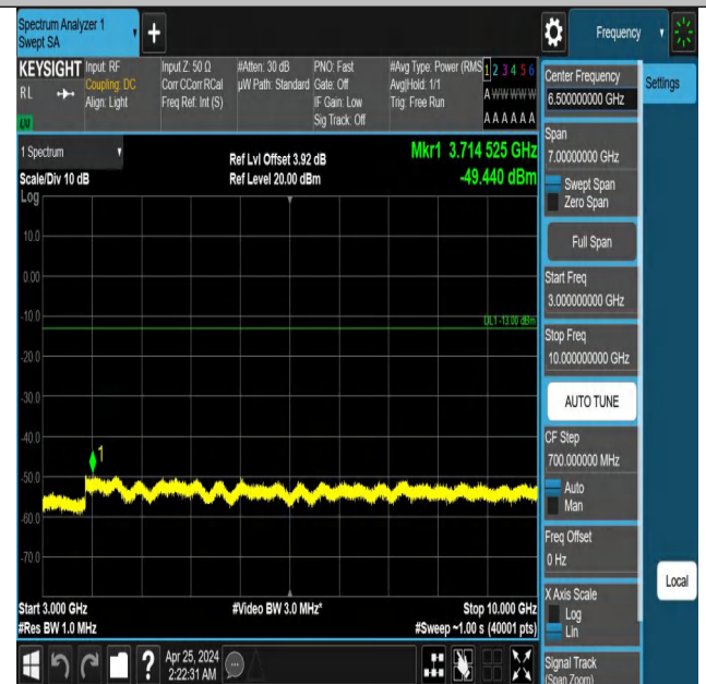
Band5_3MHz_QPSK_20415_1RB#14_3000~10000_3000~10000
