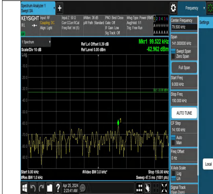
Band5_3MHz_QPSK_20635_1RB#0_0.009~0.15_0.009~0.15
