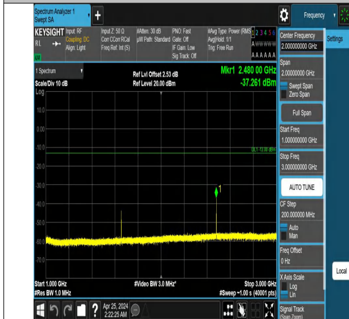
Band5_3MHz_QPSK_20415_1RB#14_1000~3000_1000~3000
