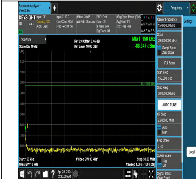
Band5_5MHz_QPSK_20425_1RB#24_0.15~30_0.15~30
