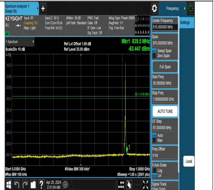
Band5_5MHz_QPSK_20425_1RB#24_30~1000_30~1000
