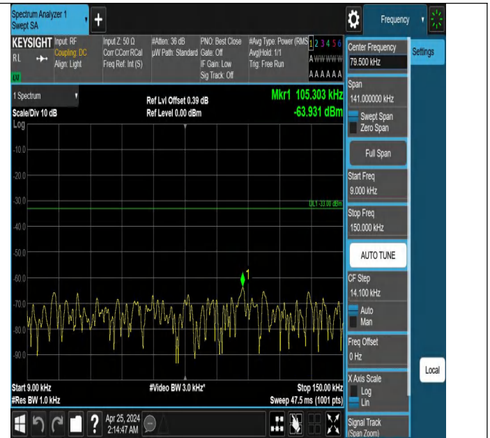
Band5_1.4MHz_QPSK_20643_1RB#5_0.009~0.15_0.009~0.15
