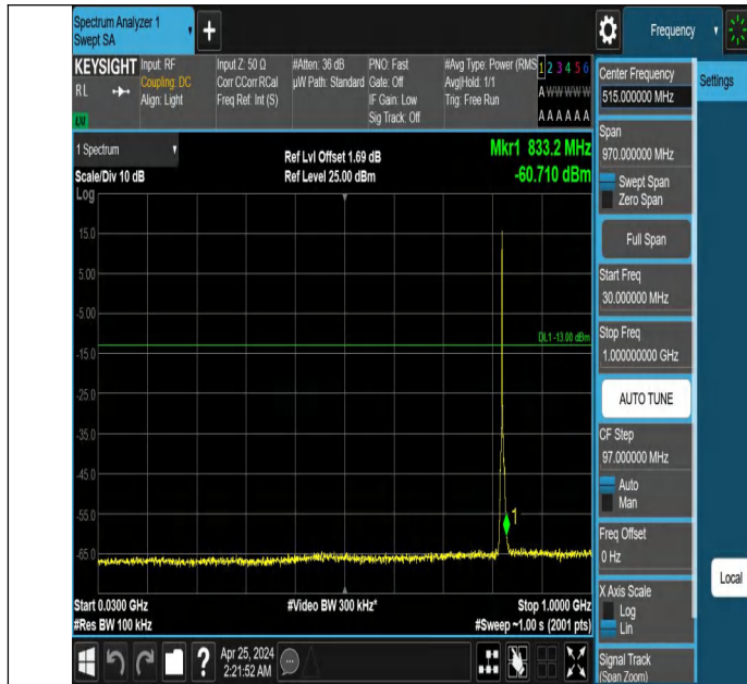
Band5_3MHz_QPSK_20415_1RB#0_30~1000_30~1000
