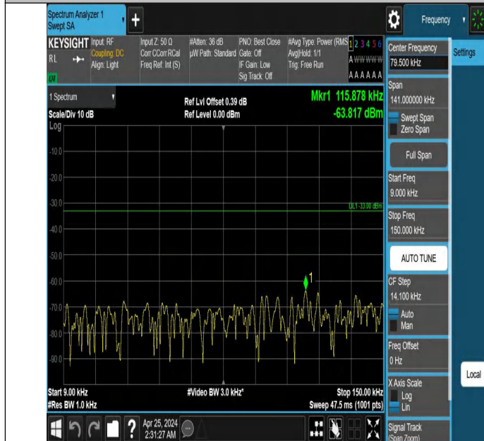
Band5_5MHz_QPSK_20525_1RB#0_0.009~0.15_0.009~0.15
